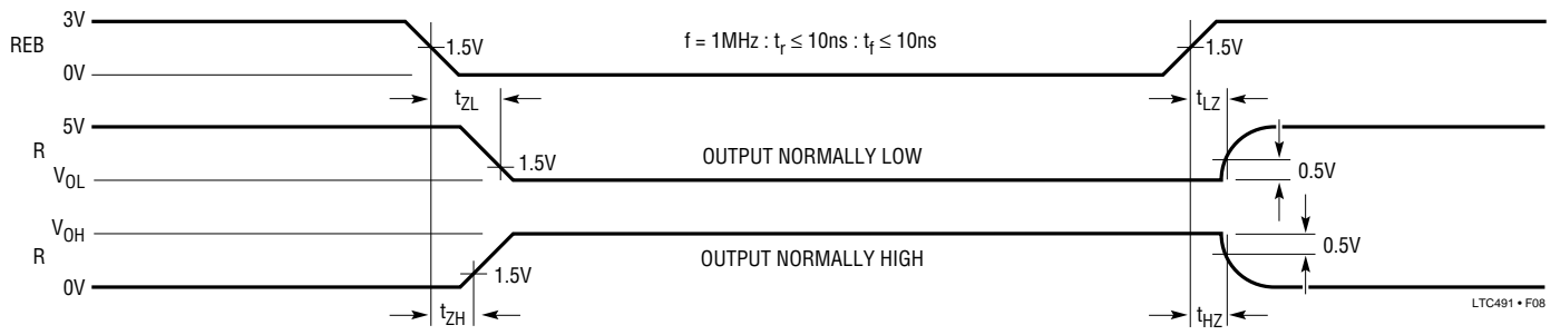
Figure 8. Receiver Enable and Disable Times
