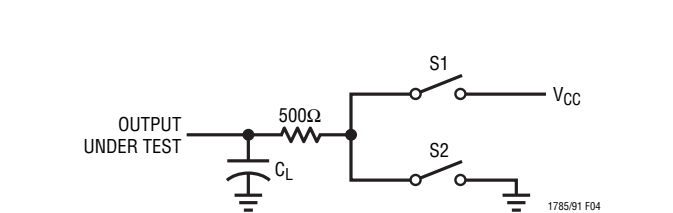
Figure 4. Driver Timing Test Load
