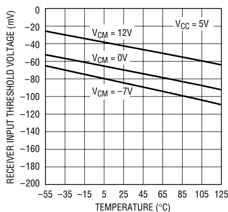
Receiver Input Threshold Voltage (Output High) vs Temperature
