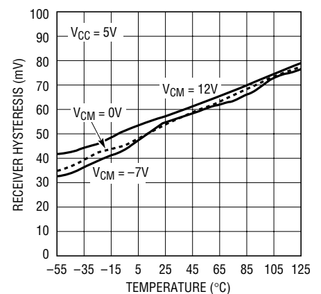
Receiver Hysteresis vs Temperature
