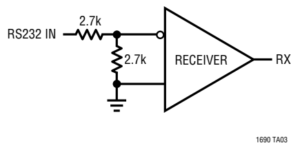
RS232 Receiver
