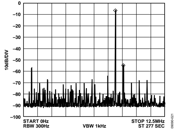
Figure 21. f_{CLK} = 25 MHz, f_{OUT} = 8.1 MHz, Frequency Word = 0x52F1A9FC
