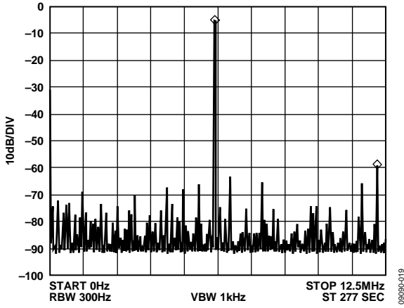
Figure 19. f_{CLK} = 25 MHz, f_{OUT} = 6.1 MHz, Frequency Word = 0x3E76C8B4
