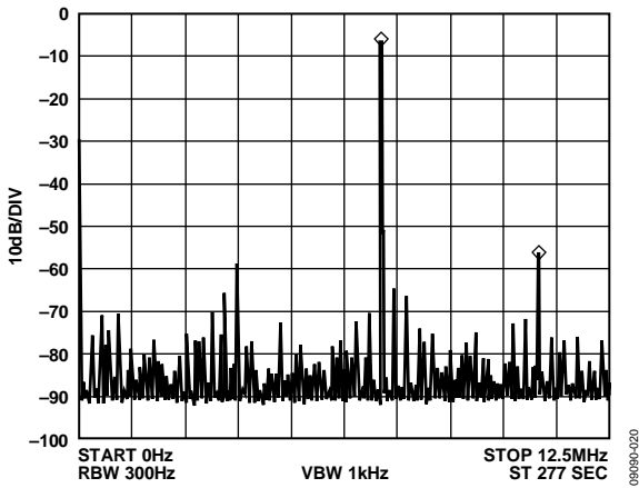
Figure 20. f_{CLK} = 25 MHz, f_{OUT} = 7.1 MHz, Frequency Word = 0x48B43958
