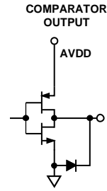
Figure 22. Comparator Outputs
