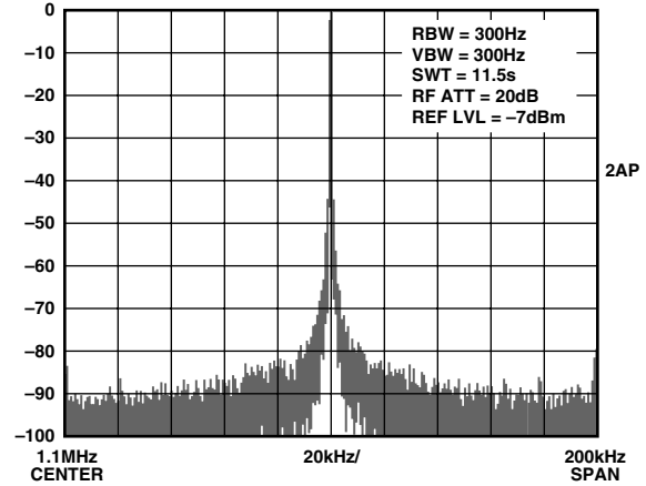
TPC 4. Narrowband ( 1.1 \pm 0.1 MHz) output SFDR for a 1.1 MHz fundamental output signal. System clock = 180 MHz ( 6\times REFCLK multiplier engaged), V_S = 5 V.
