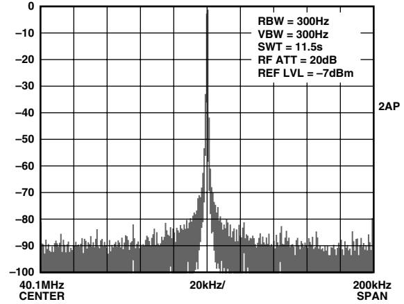
TPC 5. Narrowband ( 40.1 \pm 0.1 MHz) output SFDR for a 40.1 MHz fundamental output signal. System clock = 180 MHz ( 6\times REFCLK multiplier engaged), V_S = 5 V.
