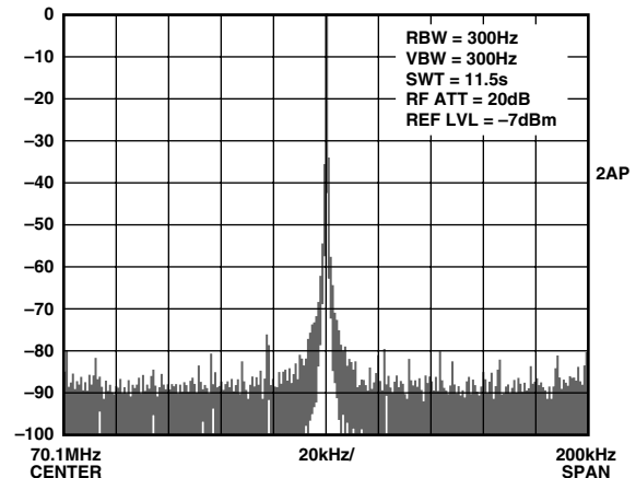
TPC 6. Narrowband ( 70.1 \pm 0.1 MHz) output SFDR for a 70.1 MHz fundamental output signal. System clock = 180 MHz ( 6\times REFCLK multiplier engaged), V_S = 5 V.
