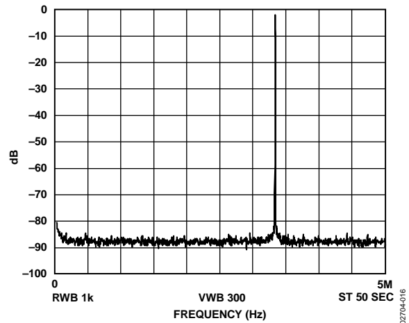
Figure 16. f_{MCLK} = 10 \text{ MHz} , f_{OUT} = 3.33 \text{ MHz} = f_{MCLK}/3 , Frequency Word = 0x5555555
