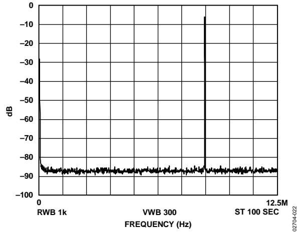
Figure 22. f_{MCLK} = 25 \text{ MHz} , f_{OUT} = 8.333 \text{ MHz} = f_{MCLK}/3 , Frequency Word = 0x5555555
