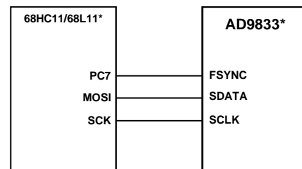
Figure 30. 68HC11/68L11 to AD9833 Interface
