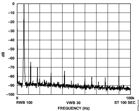
Figure 14. f_{MCLK} = 10 \text{ MHz} , f_{OUT} = 2.4 \text{ kHz} , Frequency Word = 0x000FBA9
