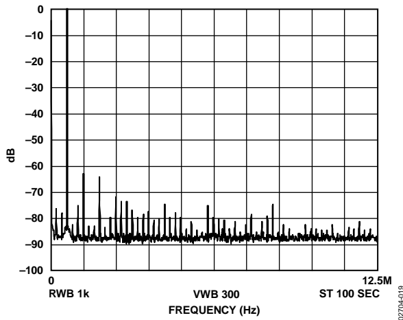
Figure 19. f_{MCLK} = 25 \text{ MHz} , f_{OUT} = 600 \text{ kHz} , Frequency Word = 0x0624DD3
