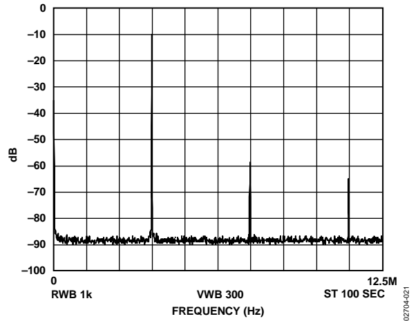
Figure 21. f_{MCLK} = 25 \text{ MHz} , f_{OUT} = 3.857 \text{ MHz} = f_{MCLK}/7 , Frequency Word = 0x2492492
