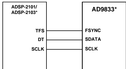
Figure 29. ADSP-2101/ADSP-2103 to AD9833 Interface
