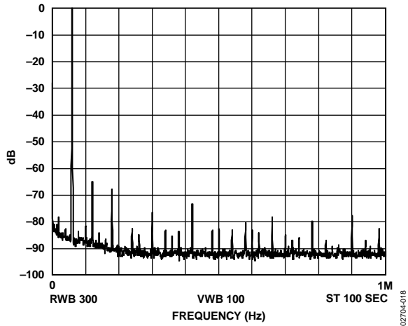
Figure 18. f_{MCLK} = 25 \text{ MHz} , f_{OUT} = 60 \text{ kHz} , Frequency Word = 0x009D495
