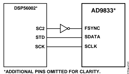
Figure 32. DSP56002 to AD9833 Interface
