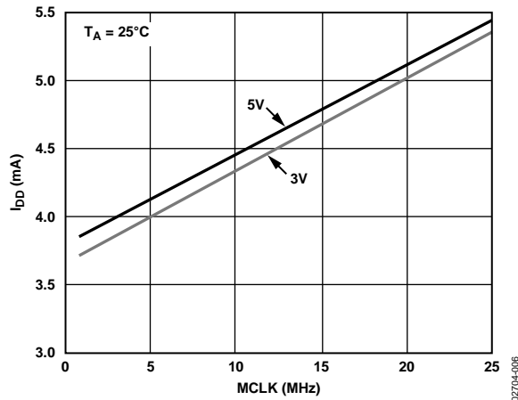
Figure 6. Typical Current Consumption vs. MCLK Frequency for f_{OUT} of MCLK/10
