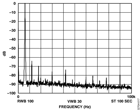
Figure 17. f_{MCLK} = 25 \text{ MHz} , f_{OUT} = 6 \text{ kHz} , Frequency Word = 0x000FBA9
