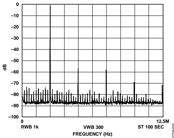
Figure 20. f_{MCLK} = 25 \text{ MHz} , f_{OUT} = 2.4 \text{ MHz} , Frequency Word = 0x189374D
