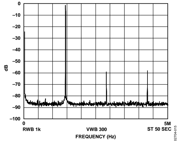
Figure 15. f_{MCLK} = 10 \text{ MHz} , f_{OUT} = 1.43 \text{ MHz} = f_{MCLK}/7 , Frequency Word = 0x2492492
