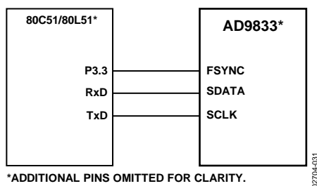
Figure 31. 80C51/80L51 to AD9833 Interface
