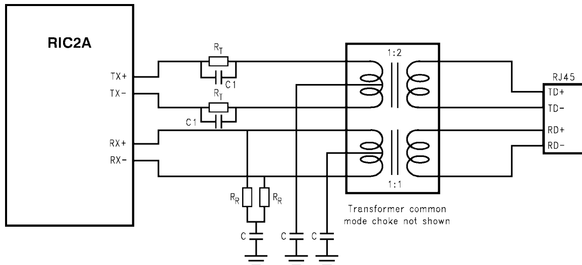
Figure 18. Magnetics Requirements
