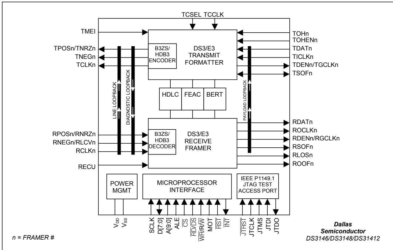
Figure 1-1. Block Diagram
