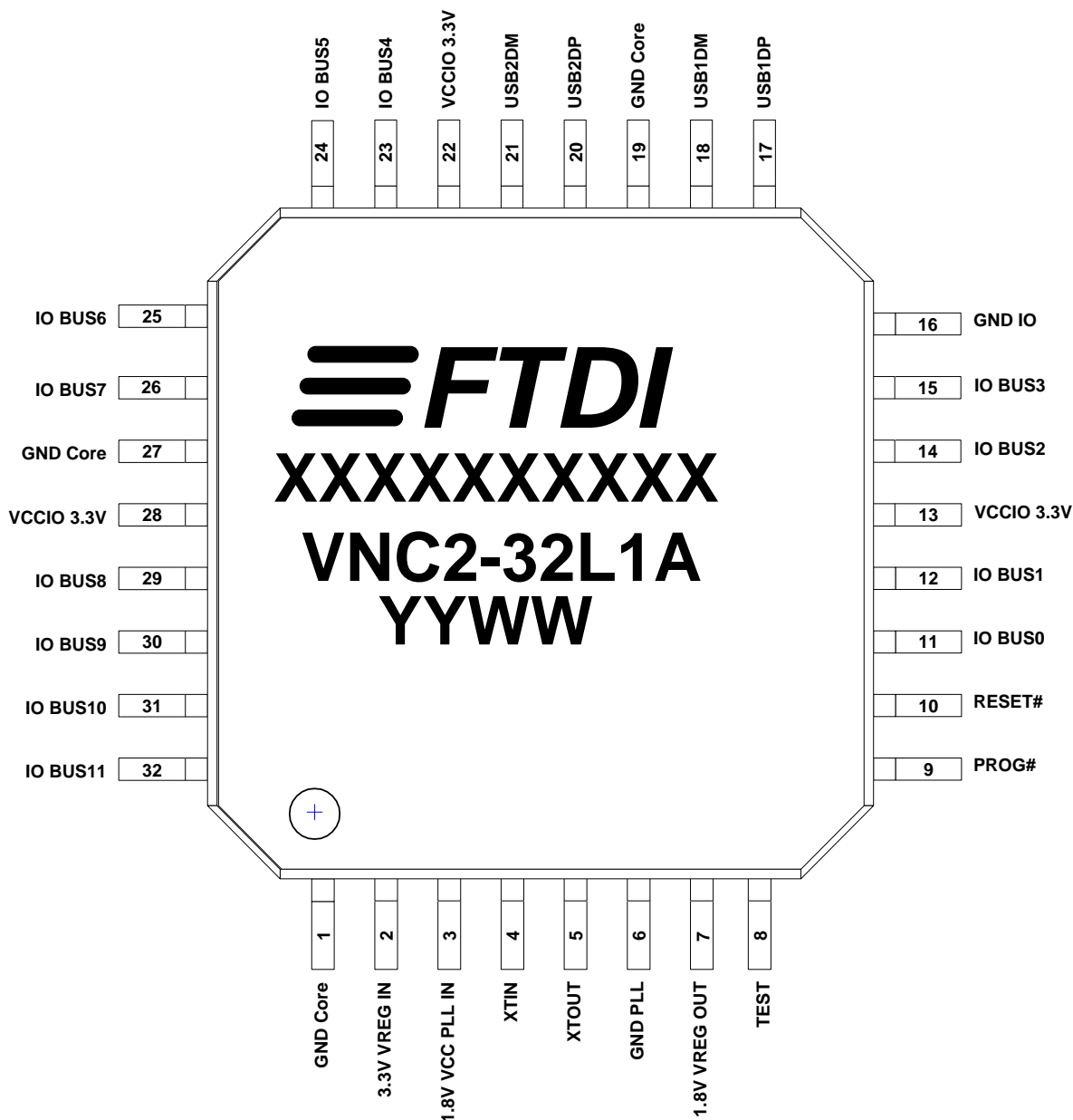
Figure 3-1 32 Pin LQFP – Top Down View
