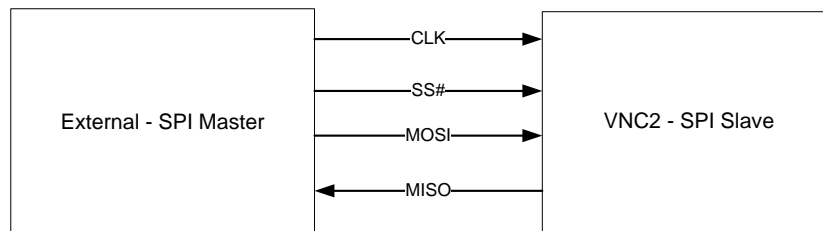
Figure 6-4 SPI Slave block diagram
