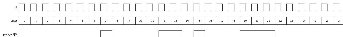
Figure 6-24 PWM – Timing Diagram
