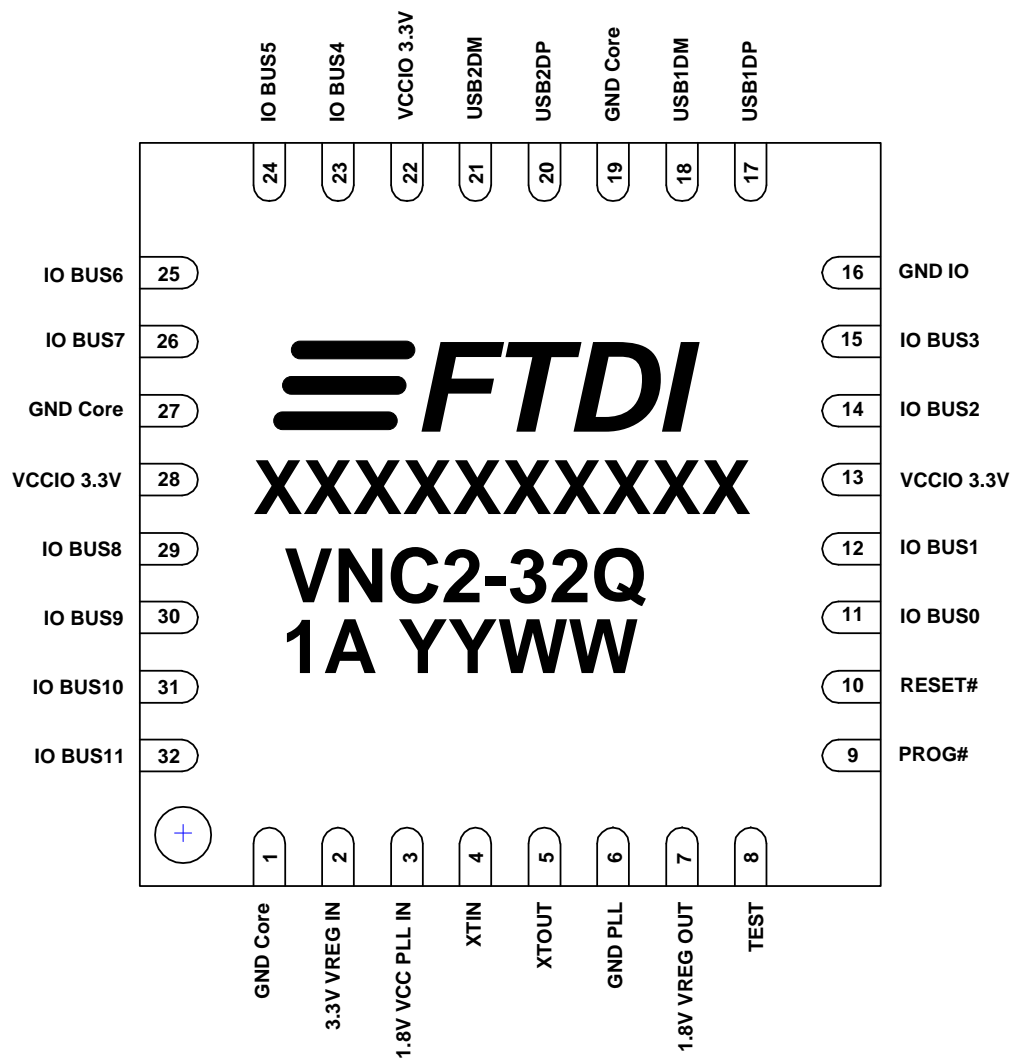
Figure 3-2 32 Pin QFN – Top Down View
