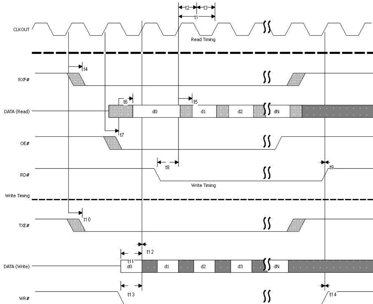
Figure 6-23 Synchronous FIFO mode Read / Write Cycle
