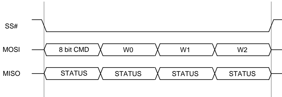
Figure 6-8 Half Duplex Data Master Write
