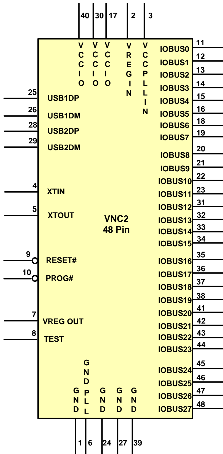
Figure 3-8 Schematic symbol 48 Pin
