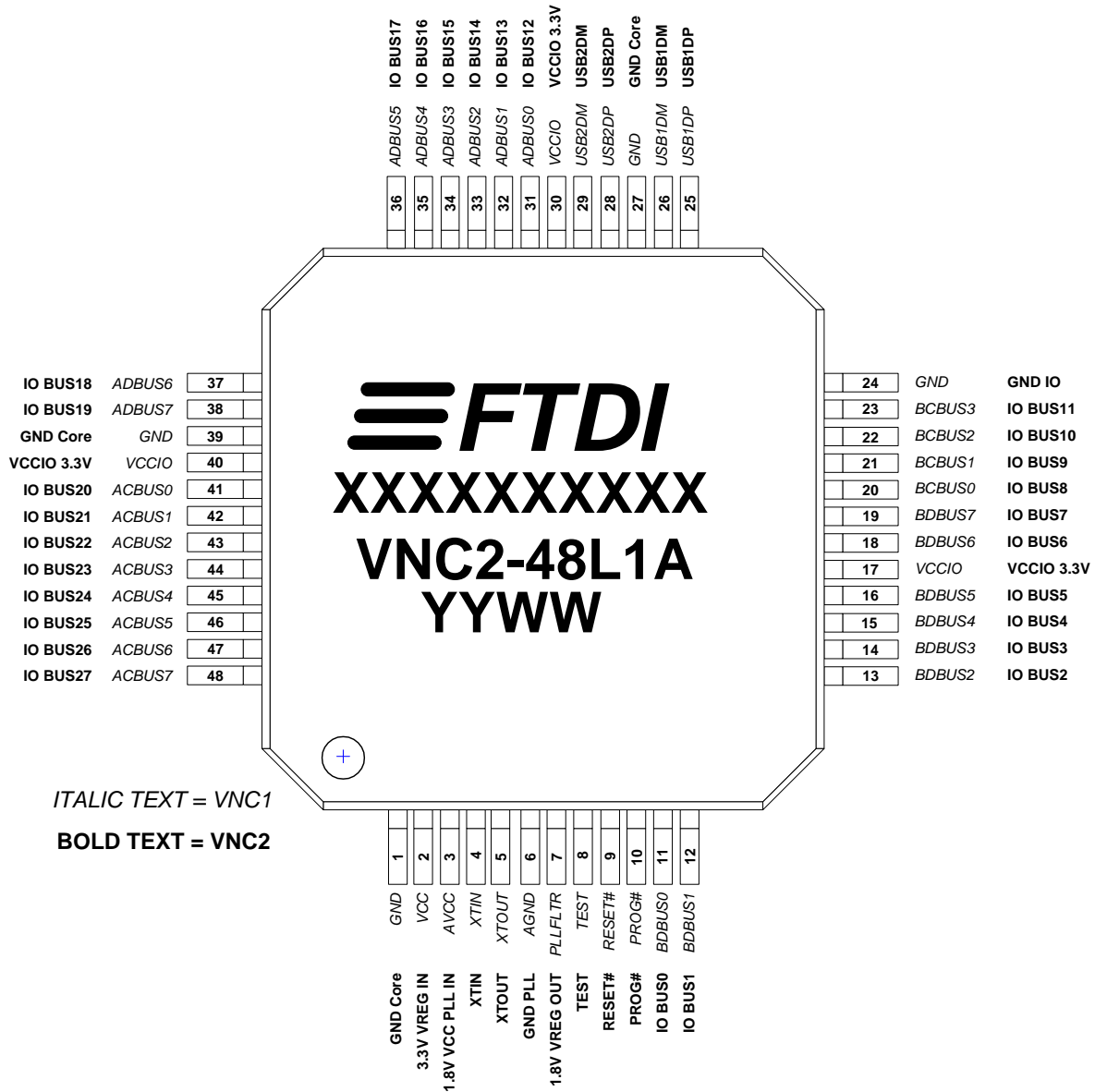
Figure 3-3 48 Pin LQFP – Top Down View
