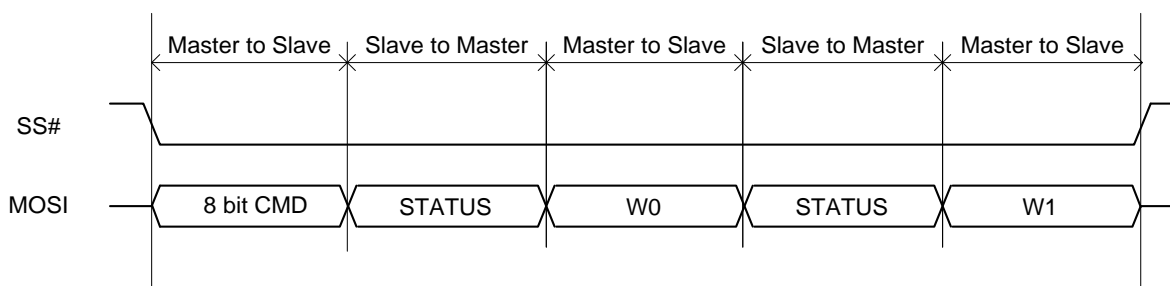
Figure 6-10 Half Duplex 3-pin Data Master Write
