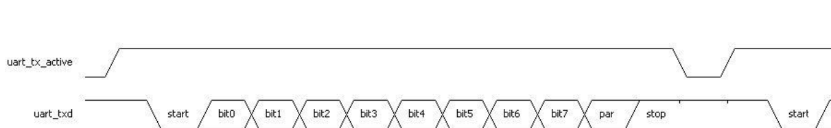
Figure 6-2 UART Transmit Waveform
