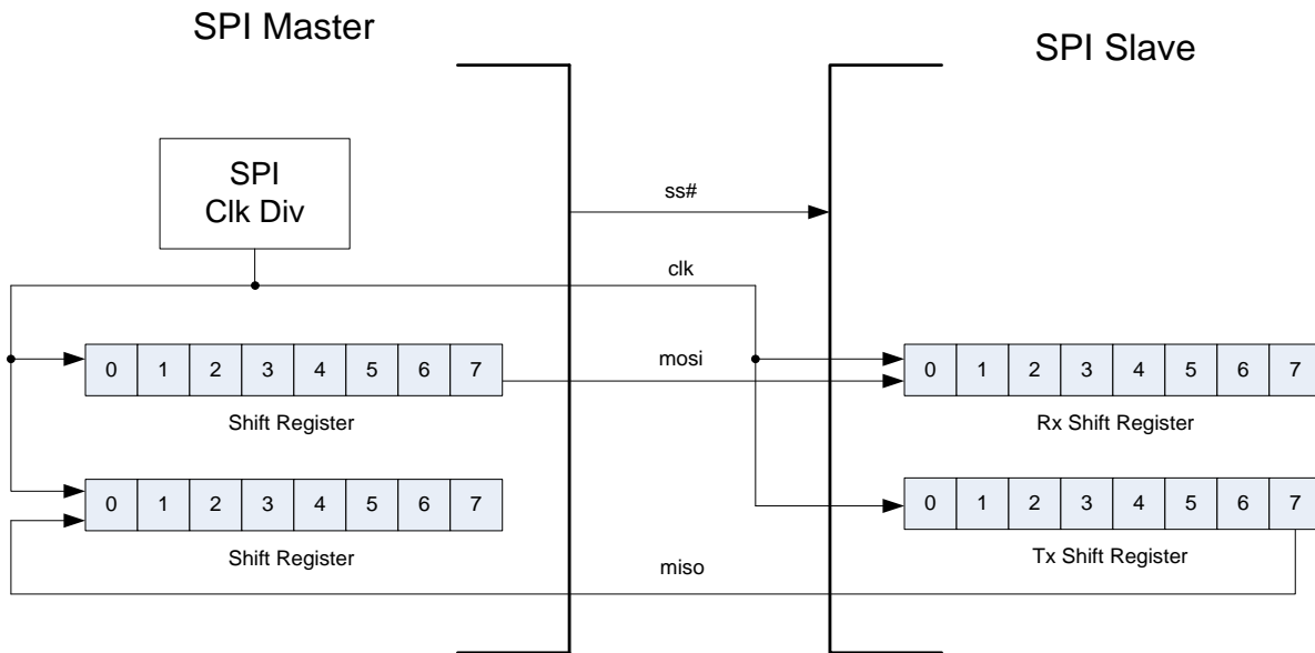
Figure 6-12 Unmanaged Mode Transfer Diagram
