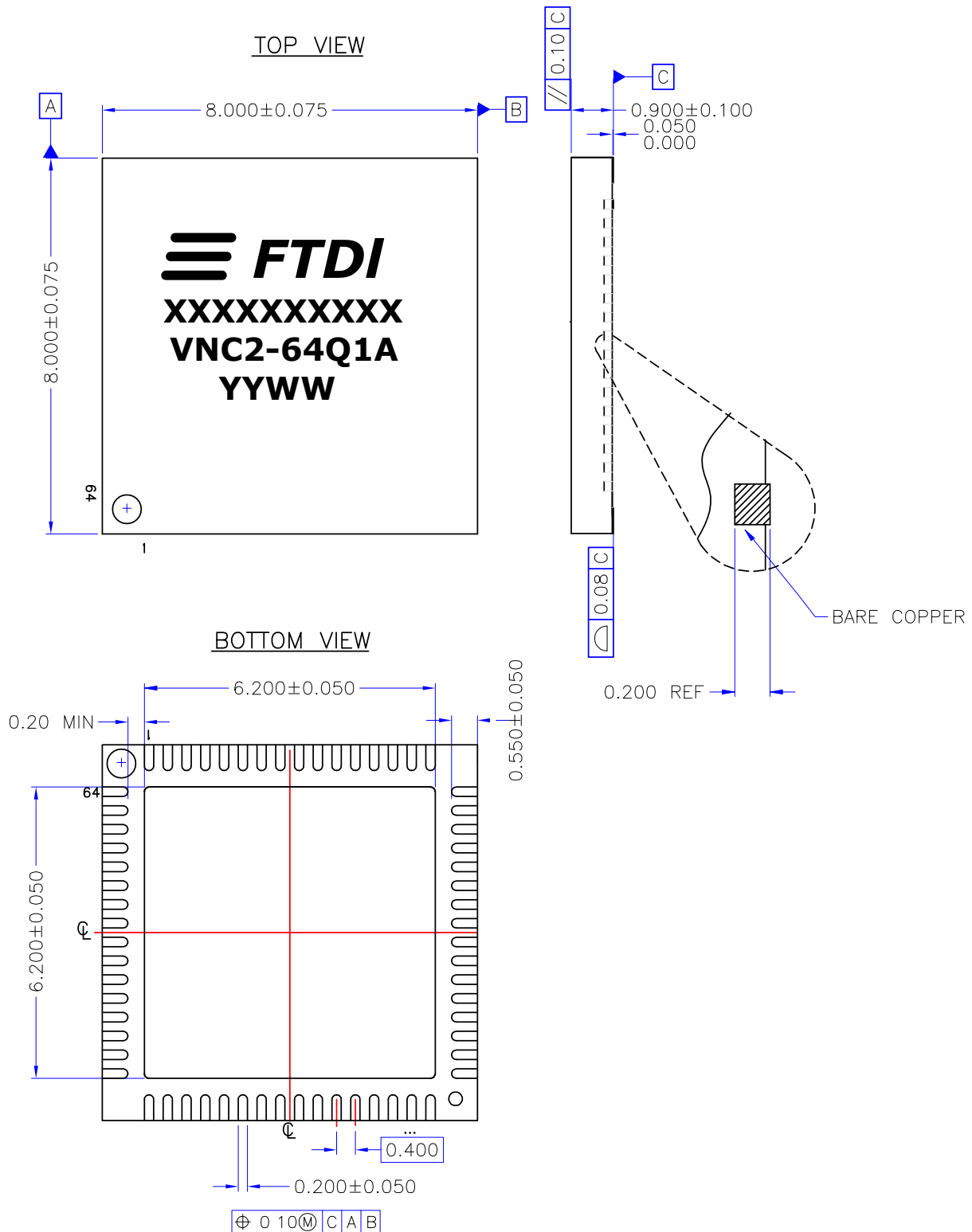
Figure 11-7 64 pin QFN Package Details
