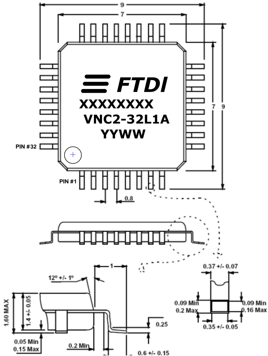
Figure 11-3 LQFP-32 Package Dimensions
