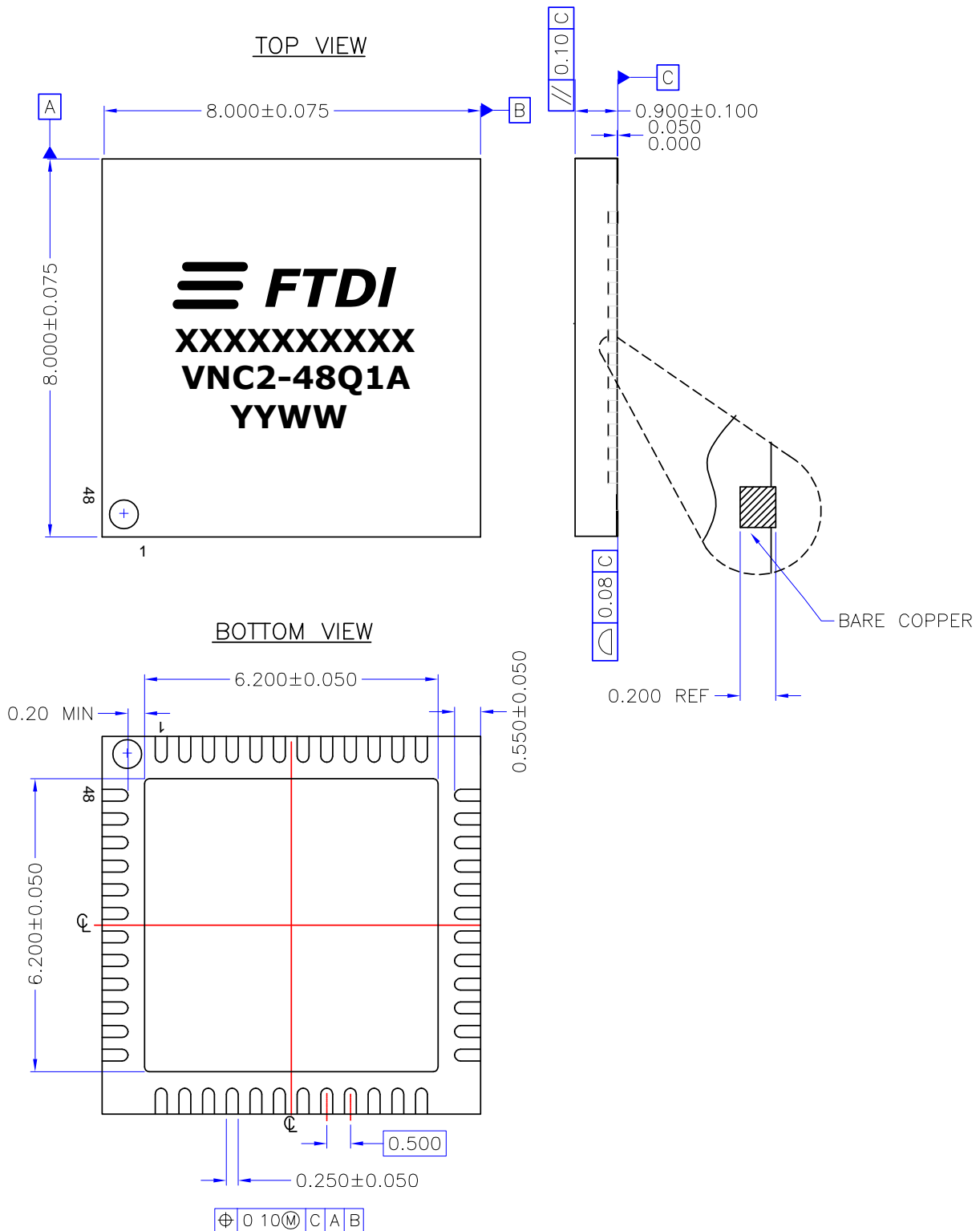
Figure 11.2 QFN-48 Package Dimensions
