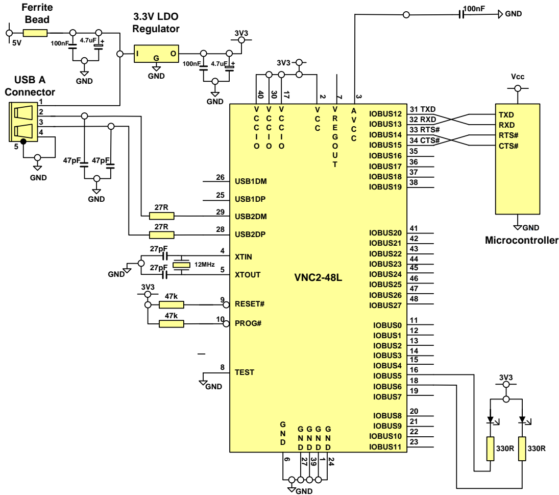
Figure 10-1 VNC2 Schematic (MCU - UART Interface)
