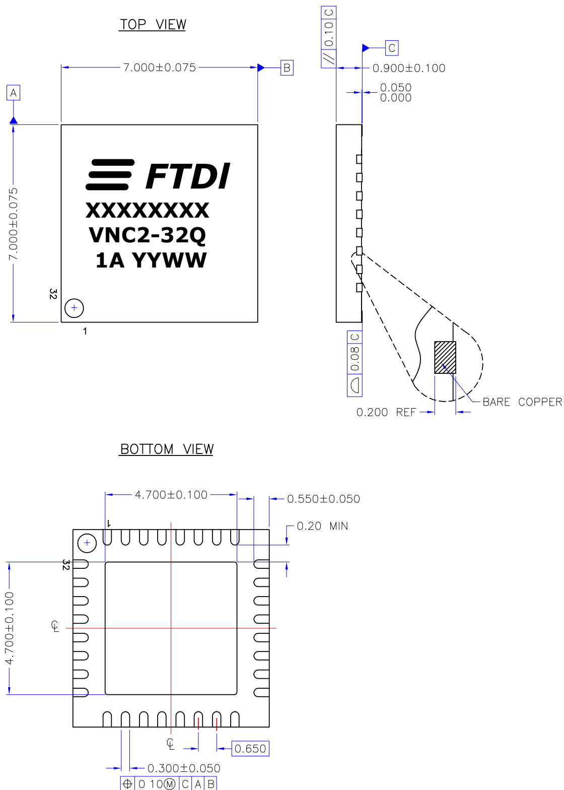
Figure 11-4 QFN-32 Package Dimensions
