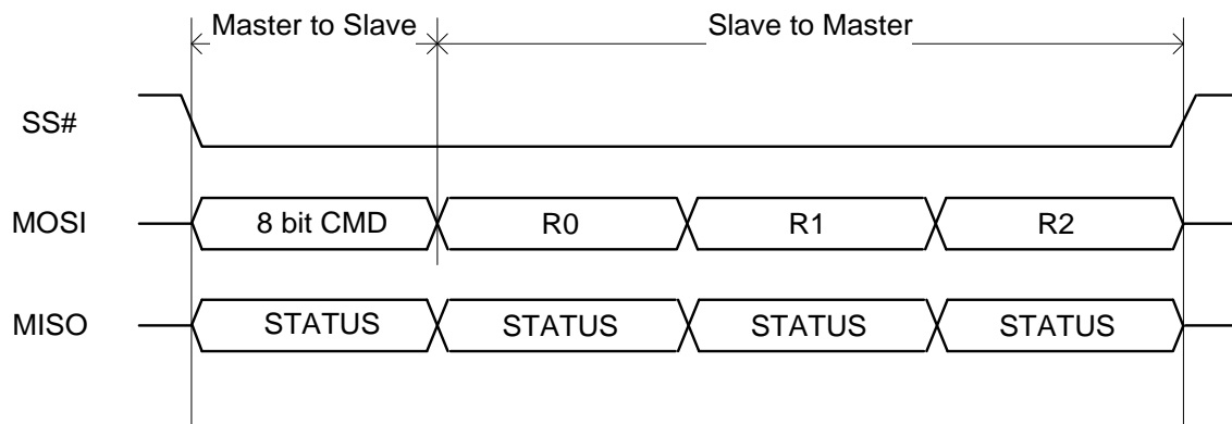
Figure 6-9 Half Duplex Data Master Read
