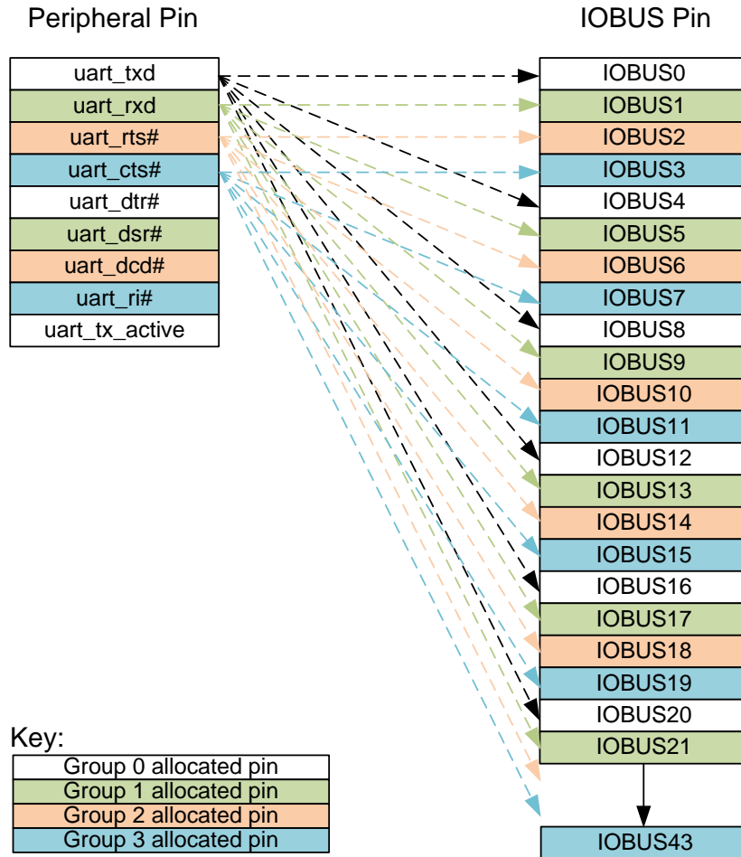
Figure 5-1 IOBUS to Group Relationship-64 Pin
