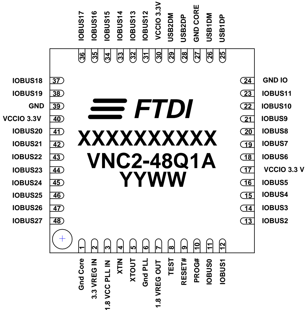
Figure 3-4 48 Pin QFN – Top Down View
