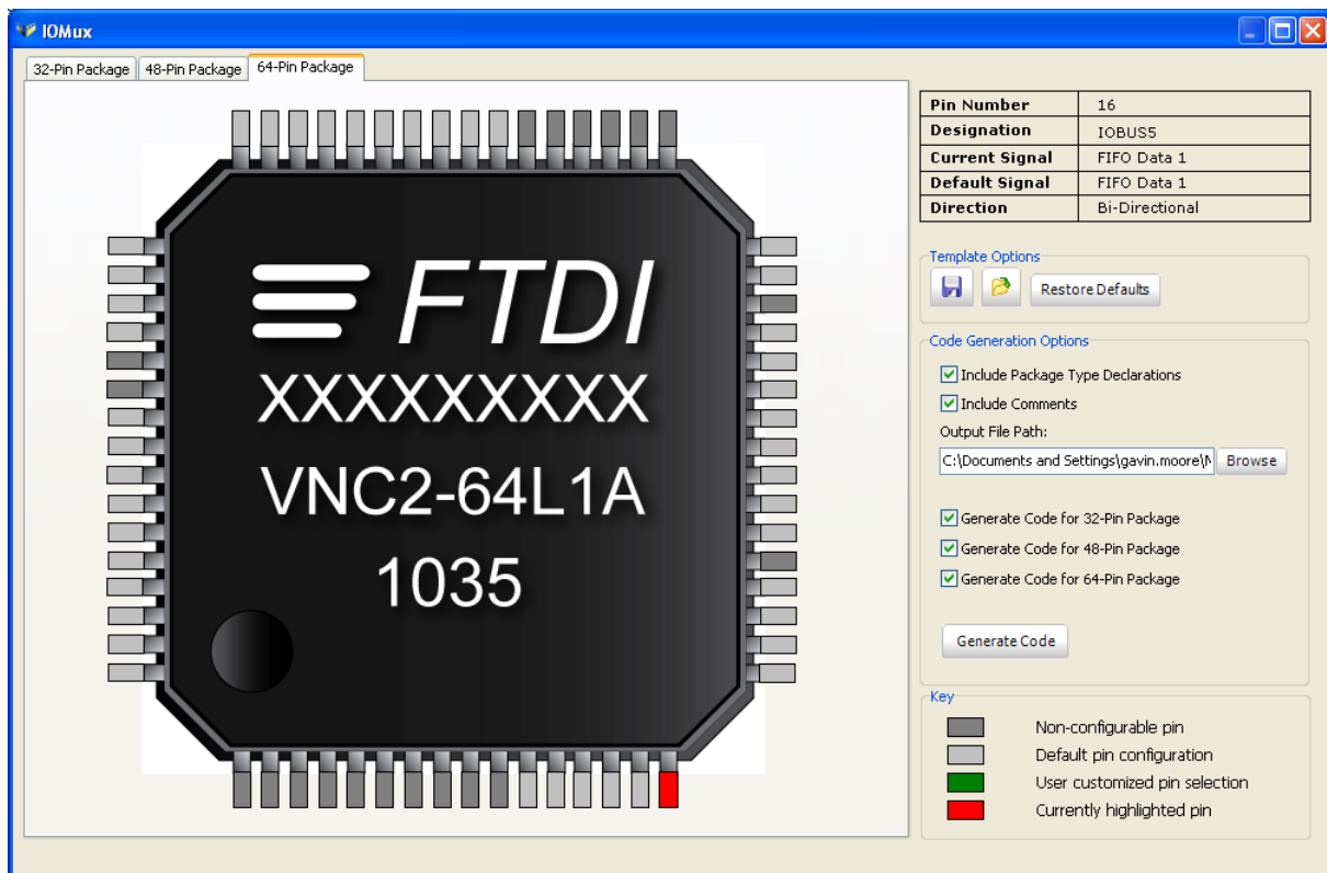
Figure 5-5 IOMux Utility screenshot
