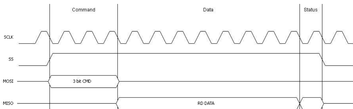
Figure 6-19 SPI Slave Mode Status Read
