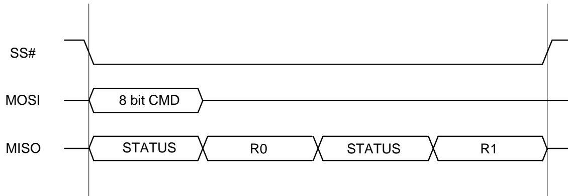
Figure 6-6 Full Duplex Data Master Read
