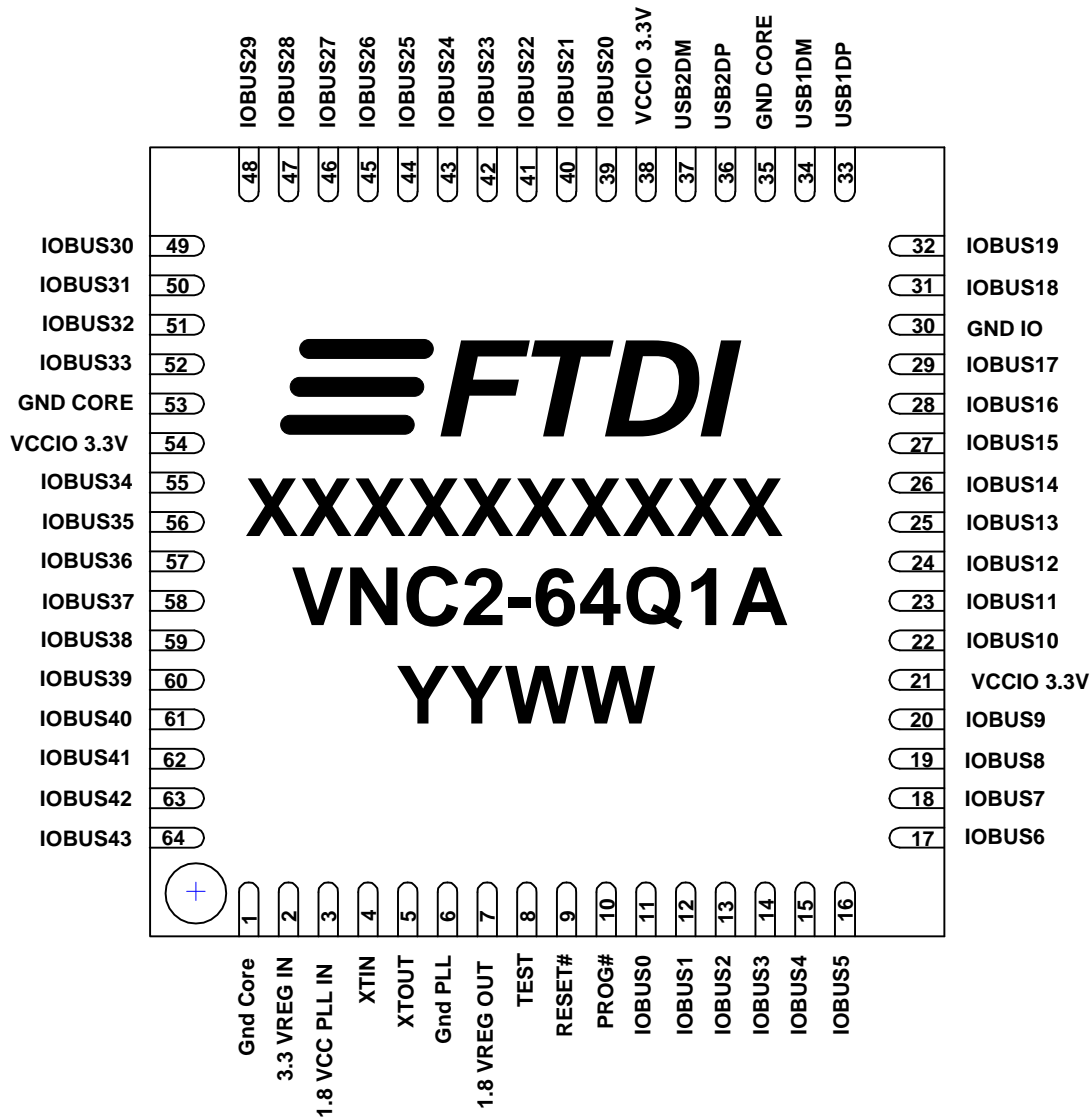
Figure 3-6 64 Pin QFN – Top Down View
