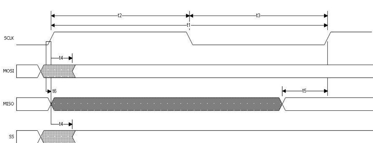
Figure 6-21 Typical SPI Master Timing
