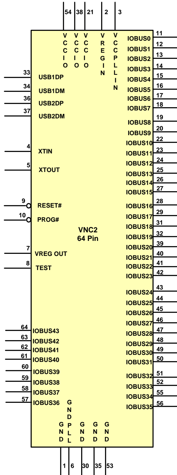
Figure 3-9 Schematic symbol 64 Pin
