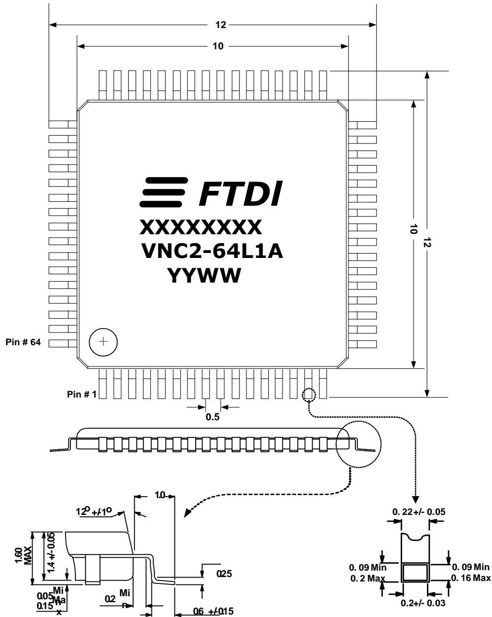
Figure 11-6 64 pin LQFP Package Details
