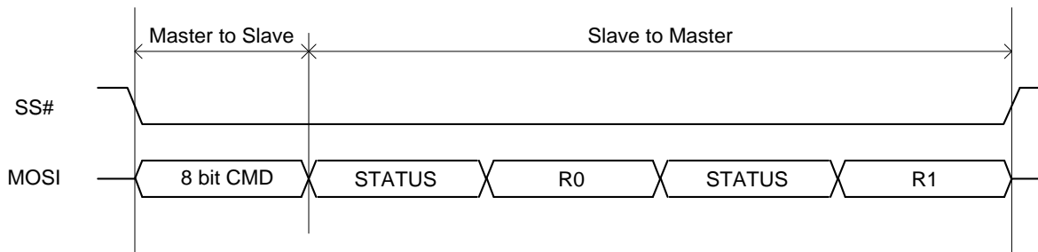
Figure 6-11 Half Duplex 3-pin Data Master Read
