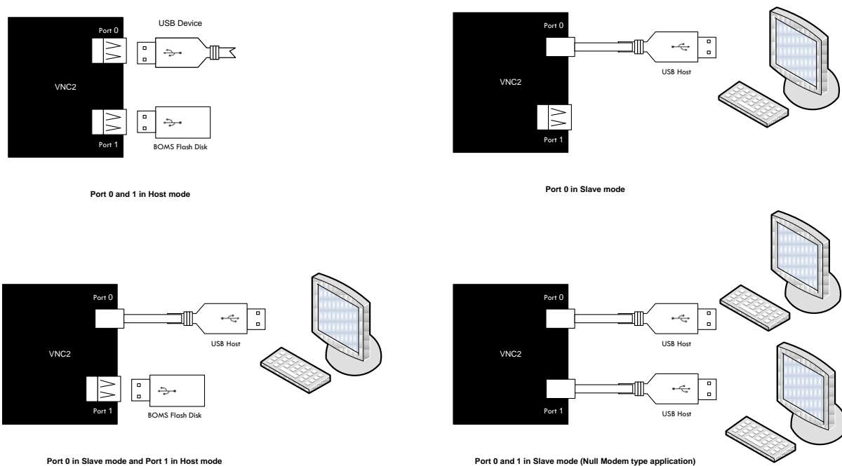
Figure 7-1 USB Modes
