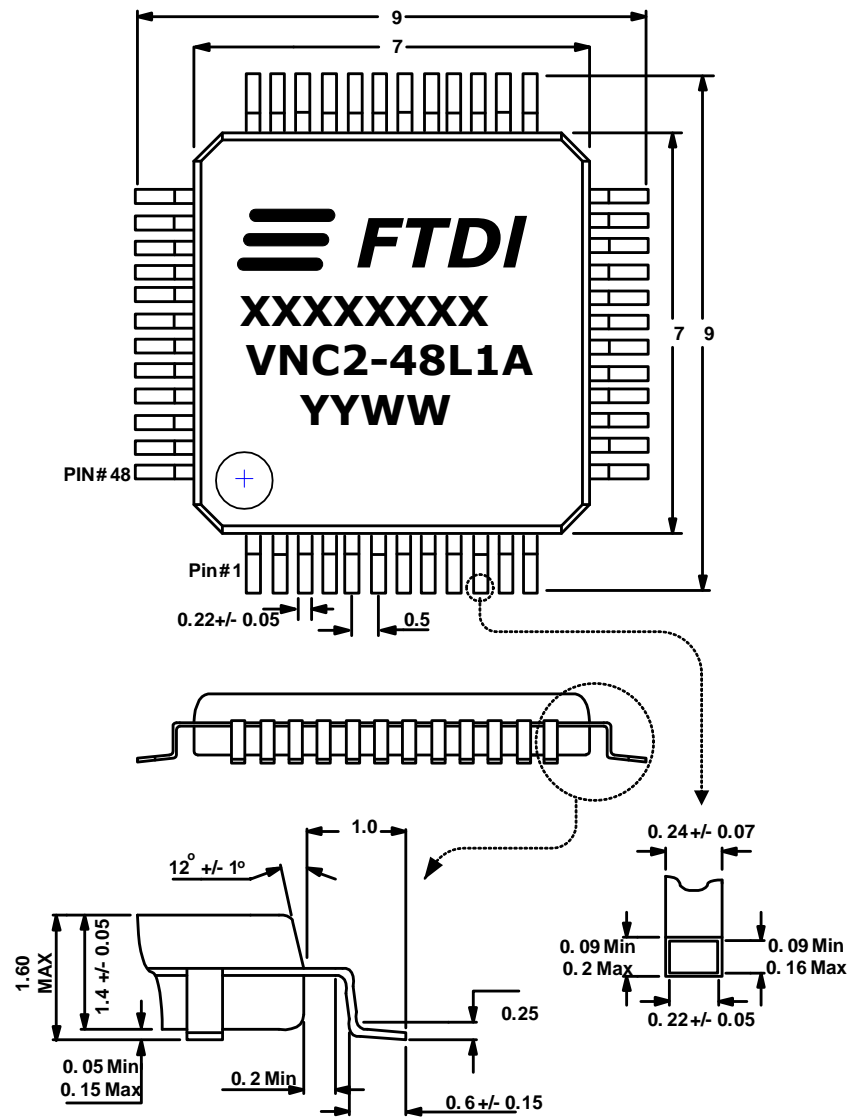
Figure 11-5 LQFP-48 Package Dimensions
