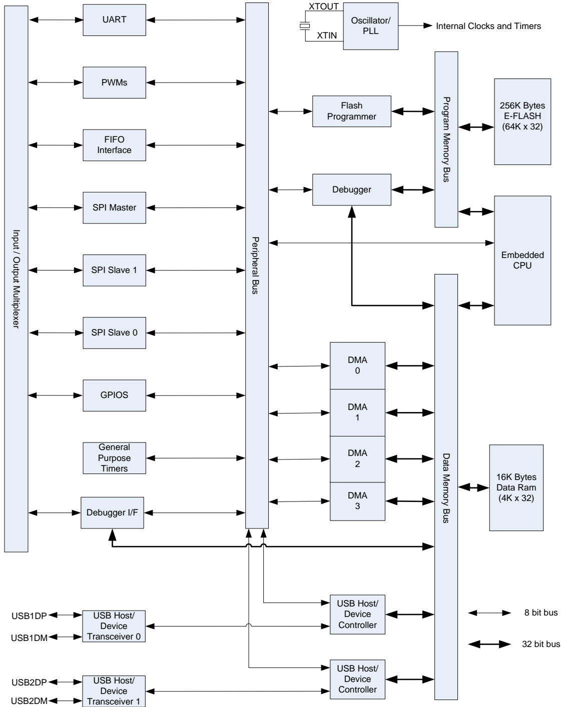
Figure 2-1 Simplified VNC2 Block Diagram
