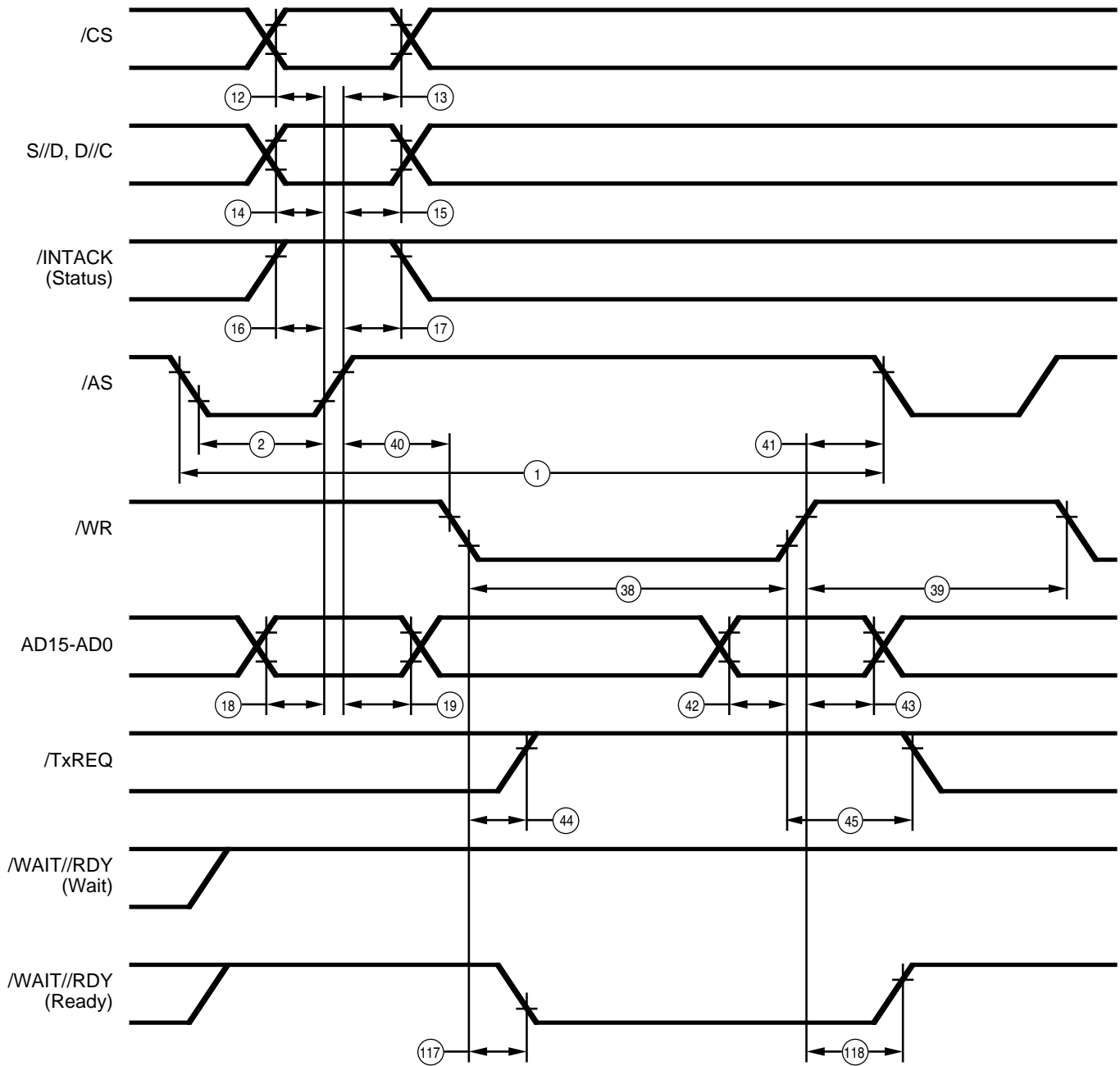
Figure 88. Multiplexed \overline{WR} Write Cycle
