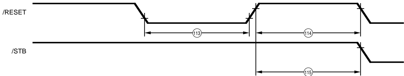
Figure 83. Reset Timing
