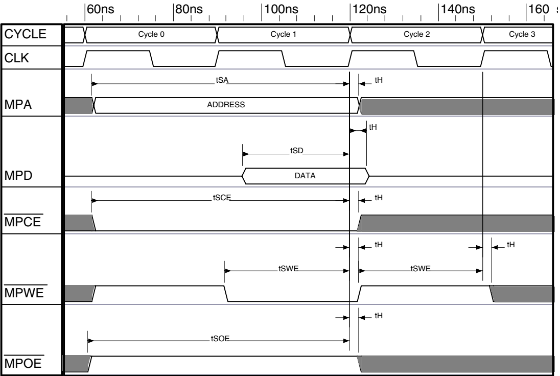
Figure 10: Single WORD Write to an ACE Register
