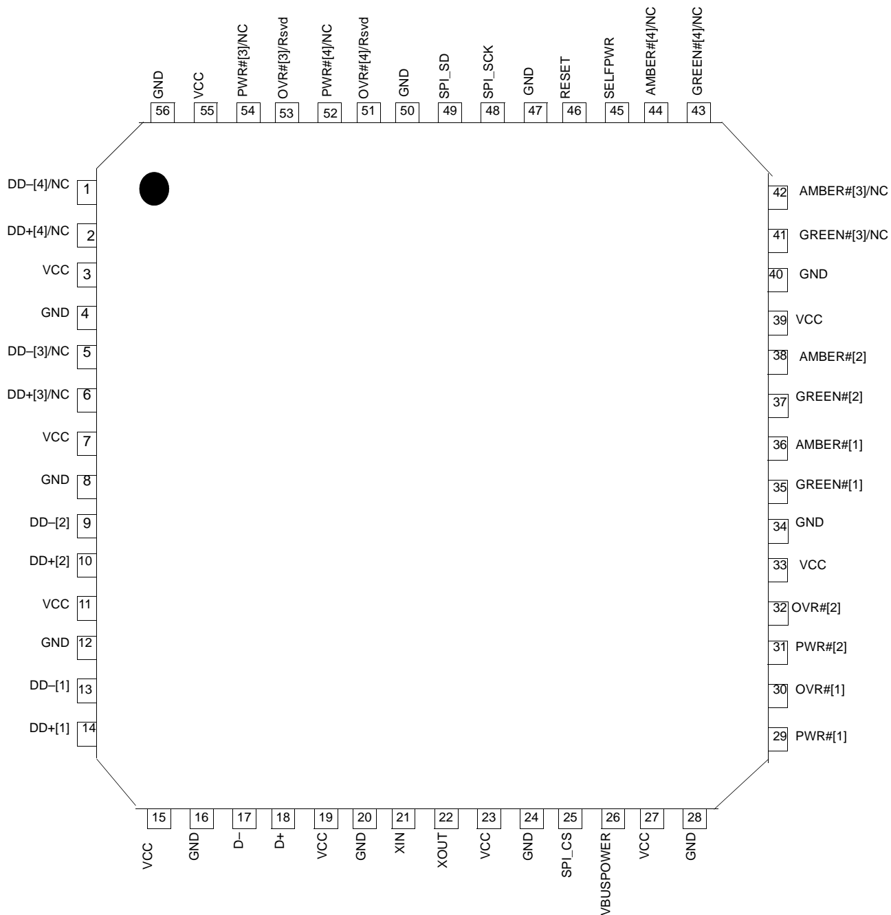
Figure 1. 56-Pin Quad Flat Pack No Leads (8 mm x 8 mm) [2]
