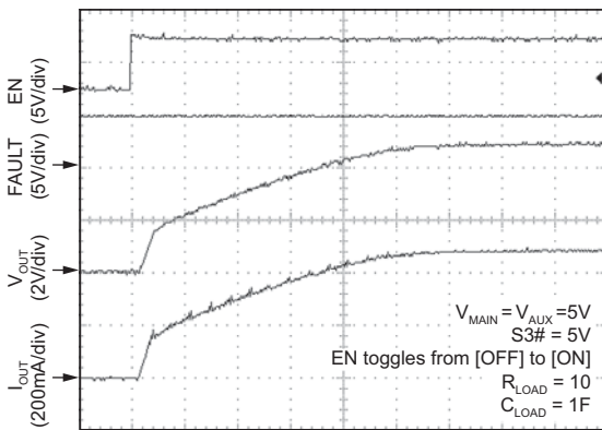
TIME (250s/div)
