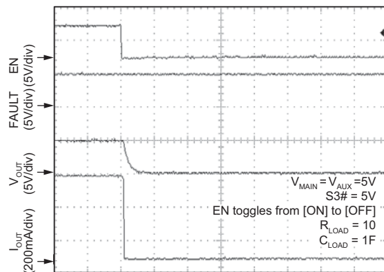
TIME (100s/div)
