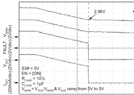
TIME (10ms/div)
