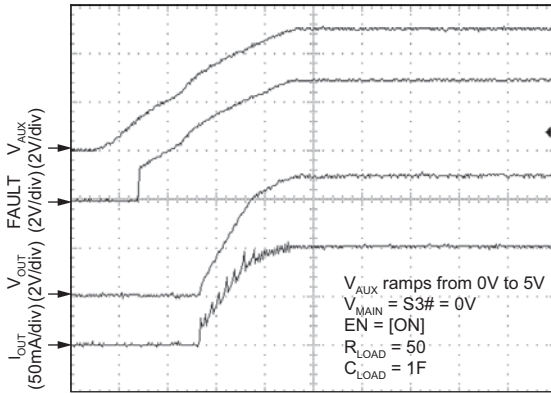
TIME (500s/div)
