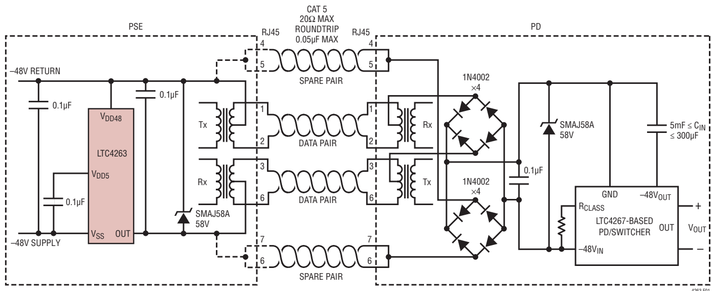
Figure 1. System Diagram
