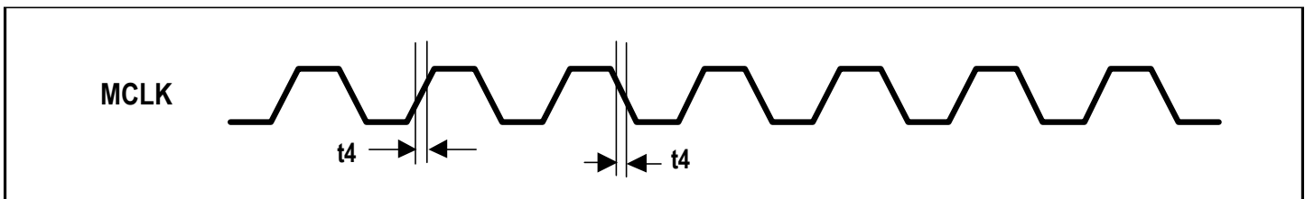
Figure 6. MCLK Timing
