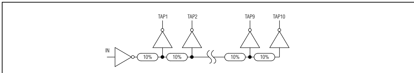
Figure 1. Logic Diagram
