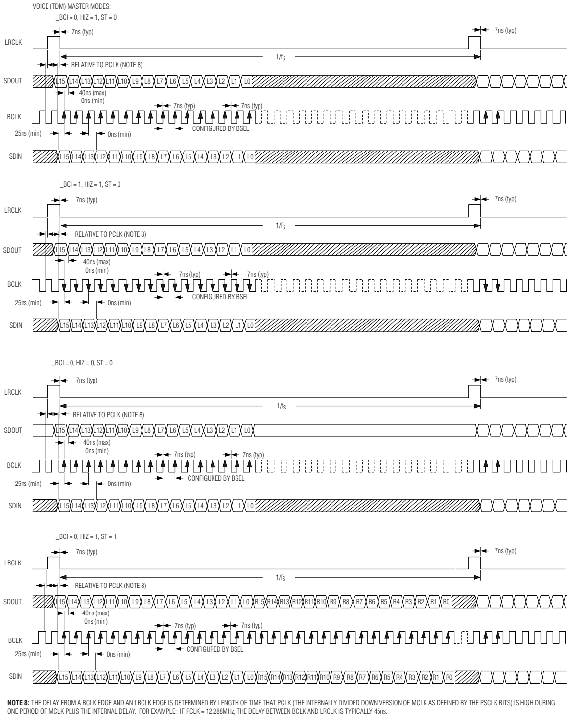
Figure 2. Digital Audio Interface Voice Master Mode Examples
