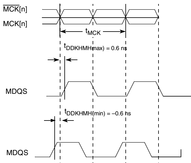
Figure 5. Timing Diagram for t_{DDKMHM}
