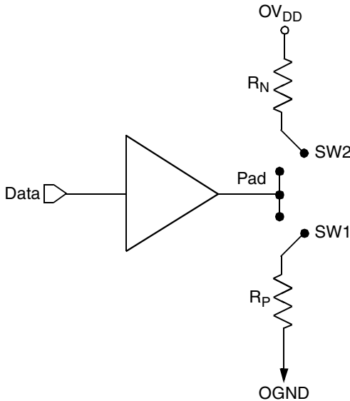
Figure 20. Driver Impedance Measurement
