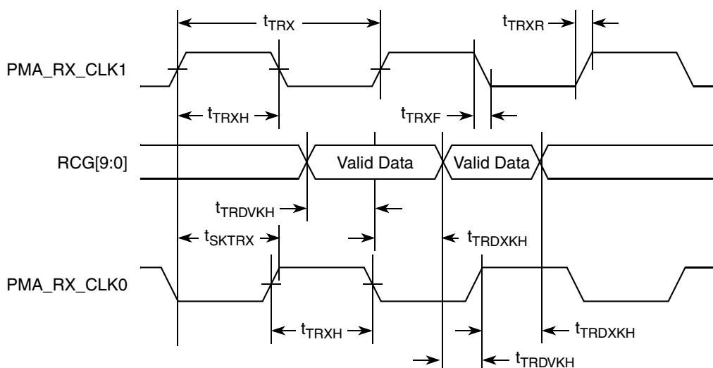
Figure 16. TBI Receive AC Timing Diagram
