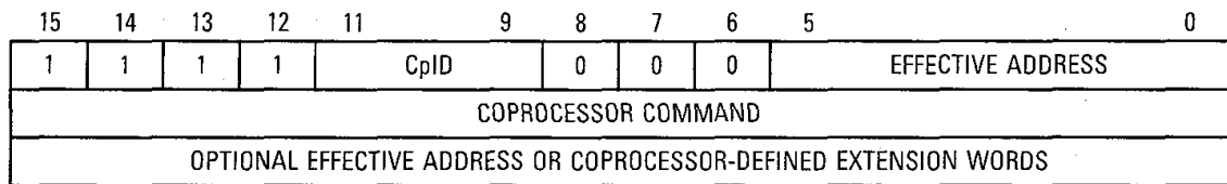
Figure 10-6. Coprocessor General Instruction Format (cpGEN)
