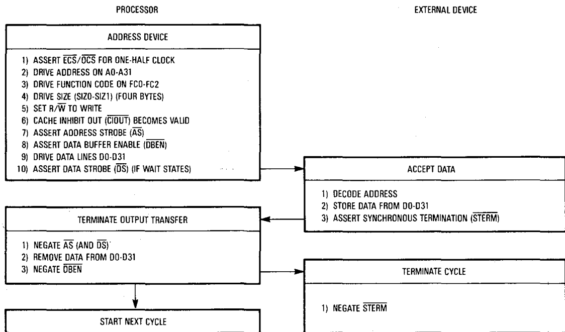
Figure 7-33. Synchronous Write Cycle Flowchart
