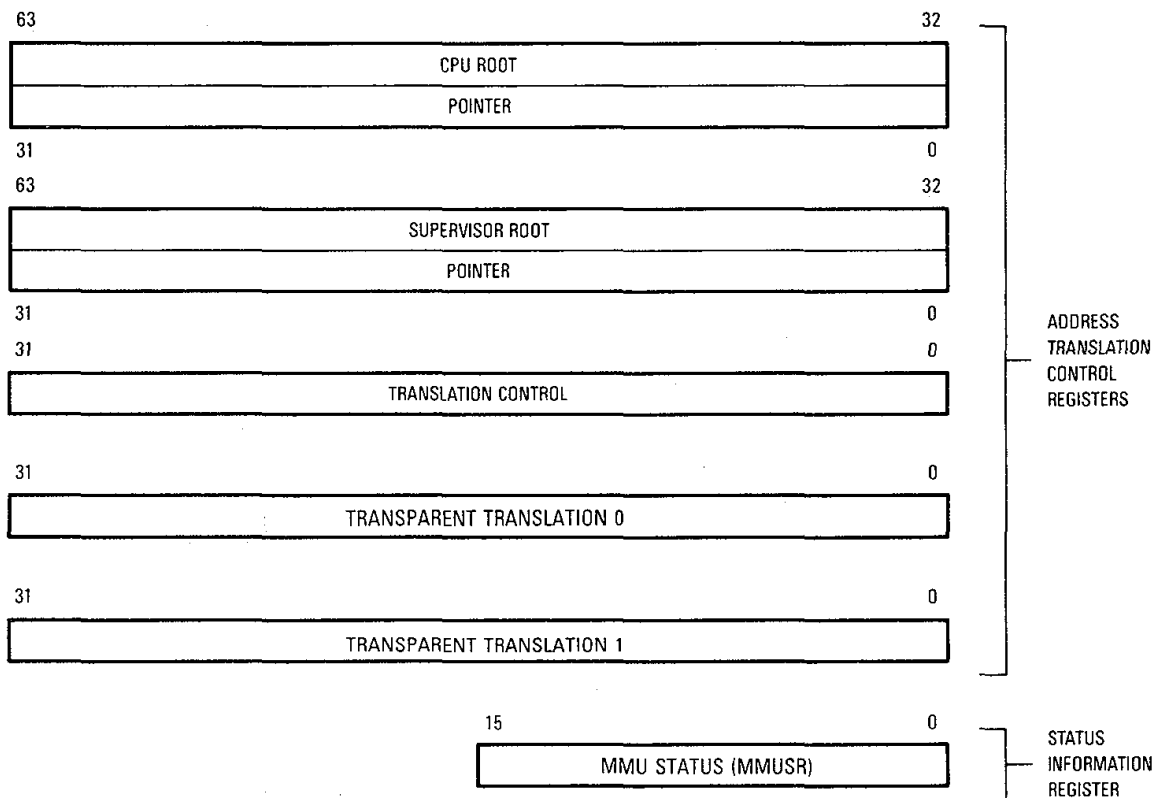
Figure 9-2. MMU Programming Model
