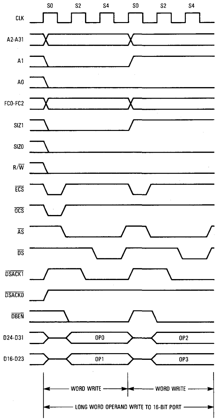
Figure 7-6. Long-Word Operand Write Timing (16-Bit Data Port)
