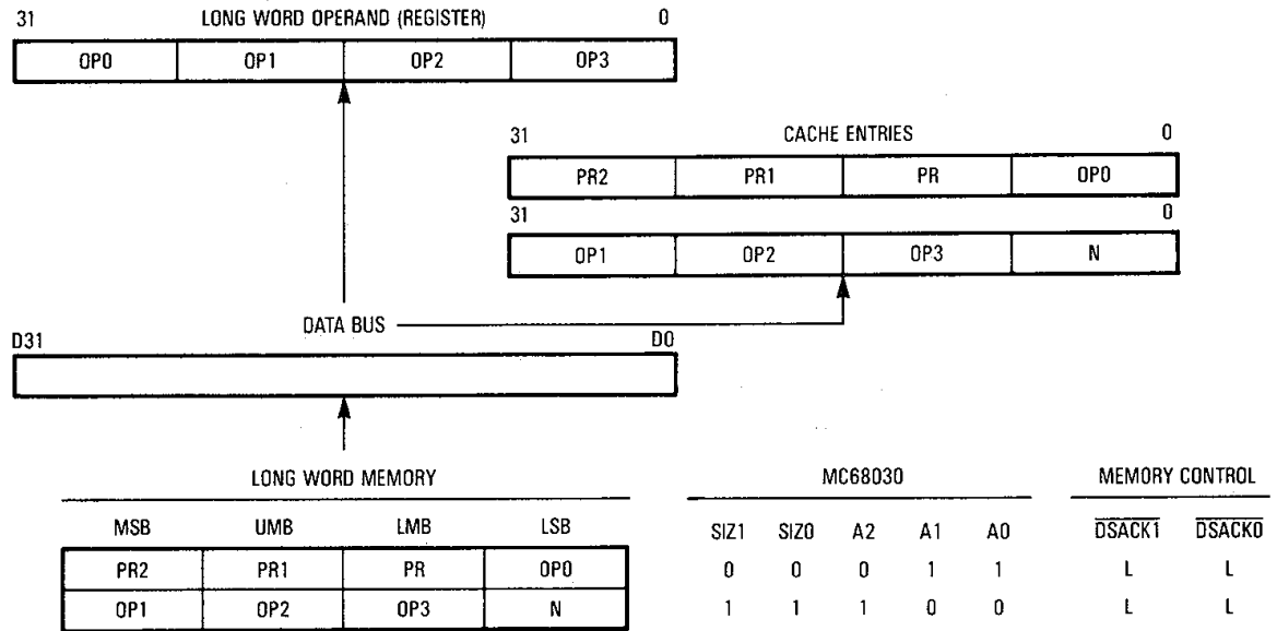
Figure 7-17. Misaligned Cachable Long-Word Transfer from Long-Word Bus
