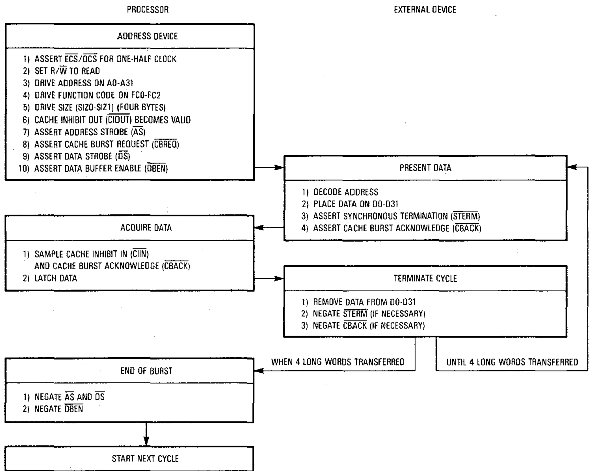
Figure 7-37. Burst Operation Flowchart — Four Long Words Transferred
