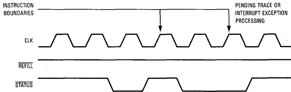
Figure 12-20. Trace or Interrupt Exception
