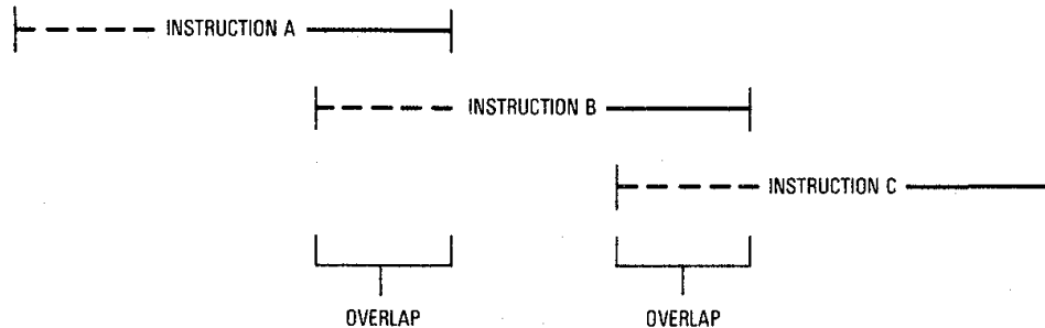
Figure 11-2. Simultaneous Instruction Execution
