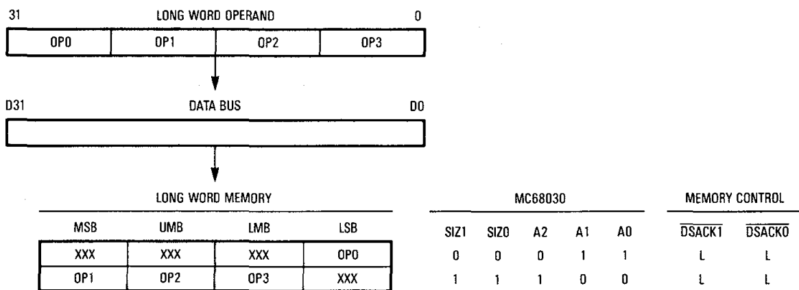
Figure 7-15. Misaligned Long-Word Transfer to Long-Word Port
