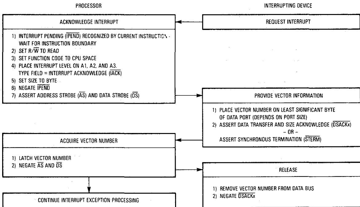
Figure 7-43. Interrupt Acknowledge Cycle Flowchart
