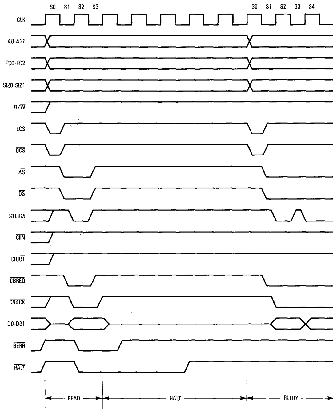
Figure 7-56. Late Retry Operation for a Burst
