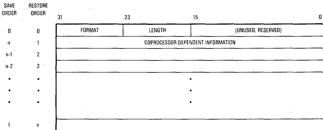
Figure 10-14. Coprocessor State Frame Format in Memory
