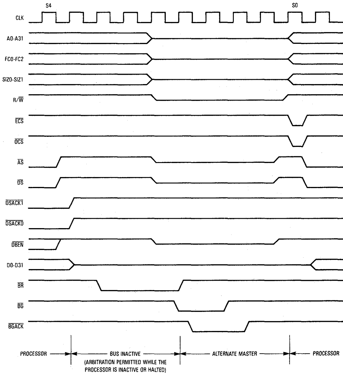
Figure 7-63. Bus Arbitration Operation (Bus Inactive)
