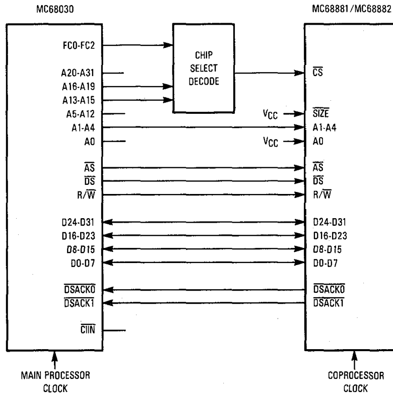
Figure 12-2. 32-Bit Data Bus Coprocessor Connection
