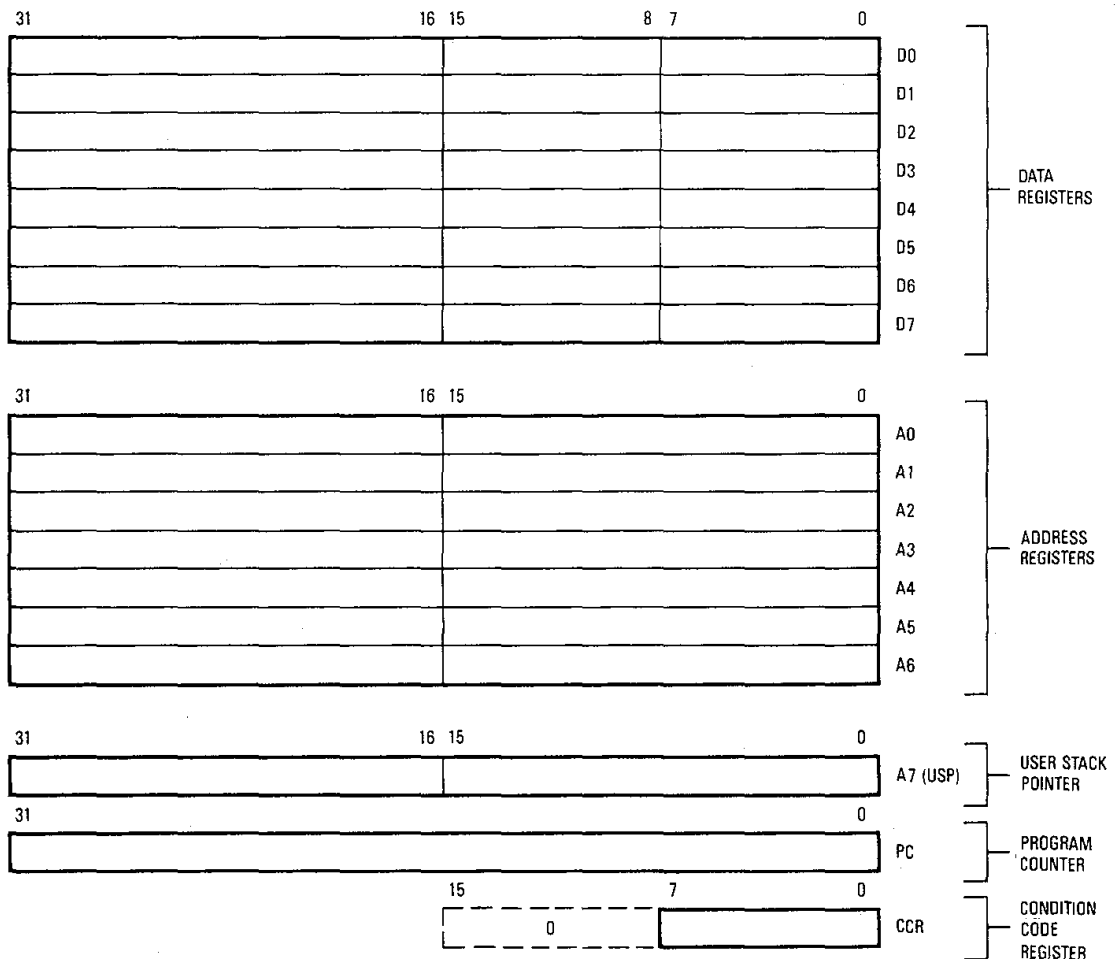
Figure 1-2. User Programming Model
