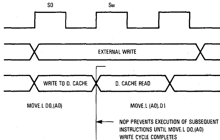
Figure 7-58. Bus Synchronization Example
