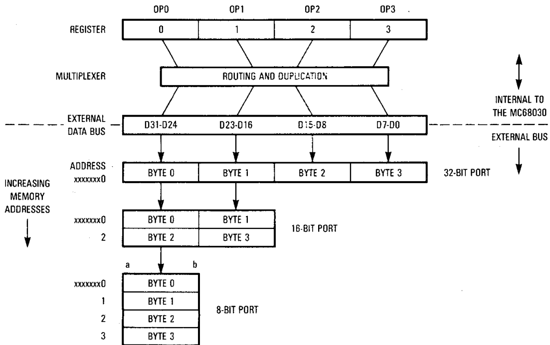
Figure 7-4. MC68030 Interface to Various Port Sizes
