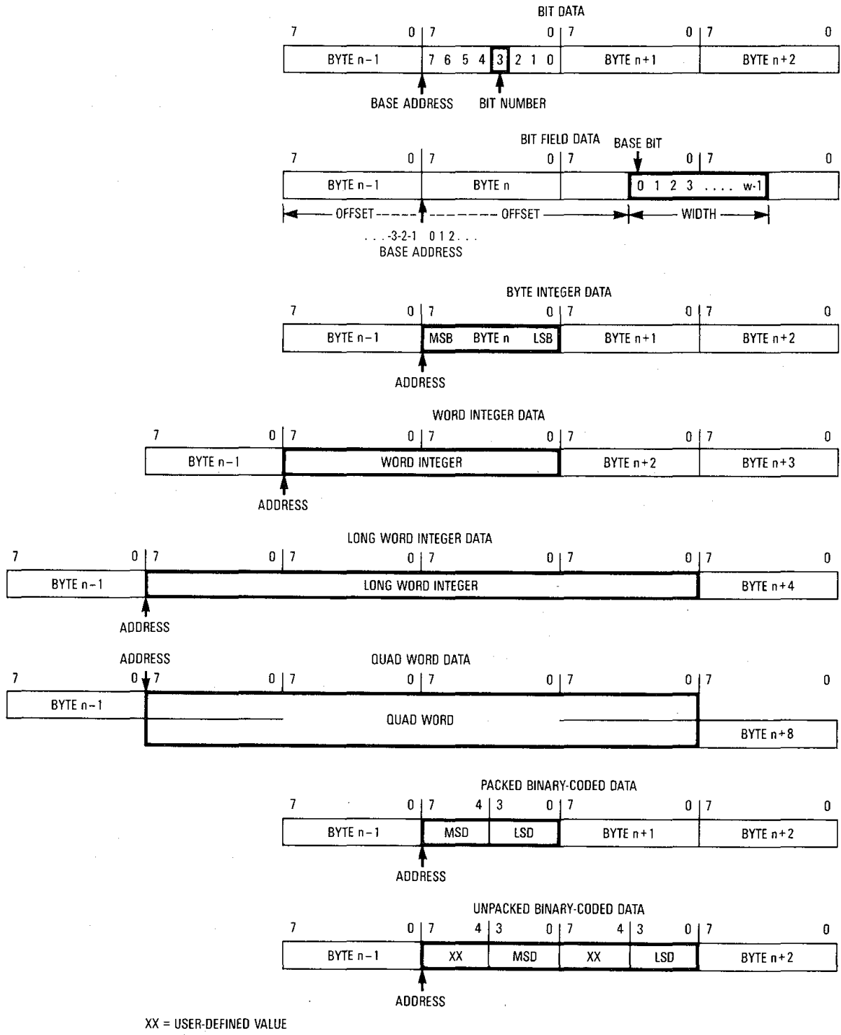
Figure 2-2. Memory Data Organization
