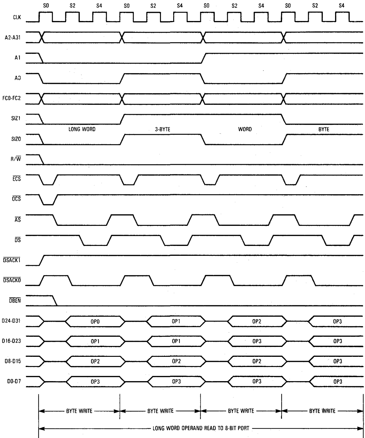
Figure 7-27. Long-Word Operand Write — 8-Bit Port
