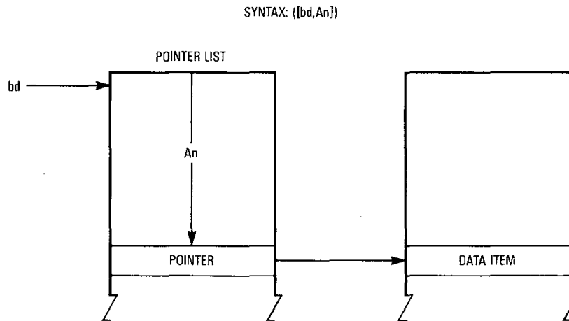
Figure 2-10. Indirect Addressing, Suppressed Index Register
