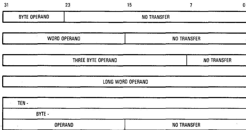
Figure 10-21. Operand Alignment for Operand CIR Accesses
