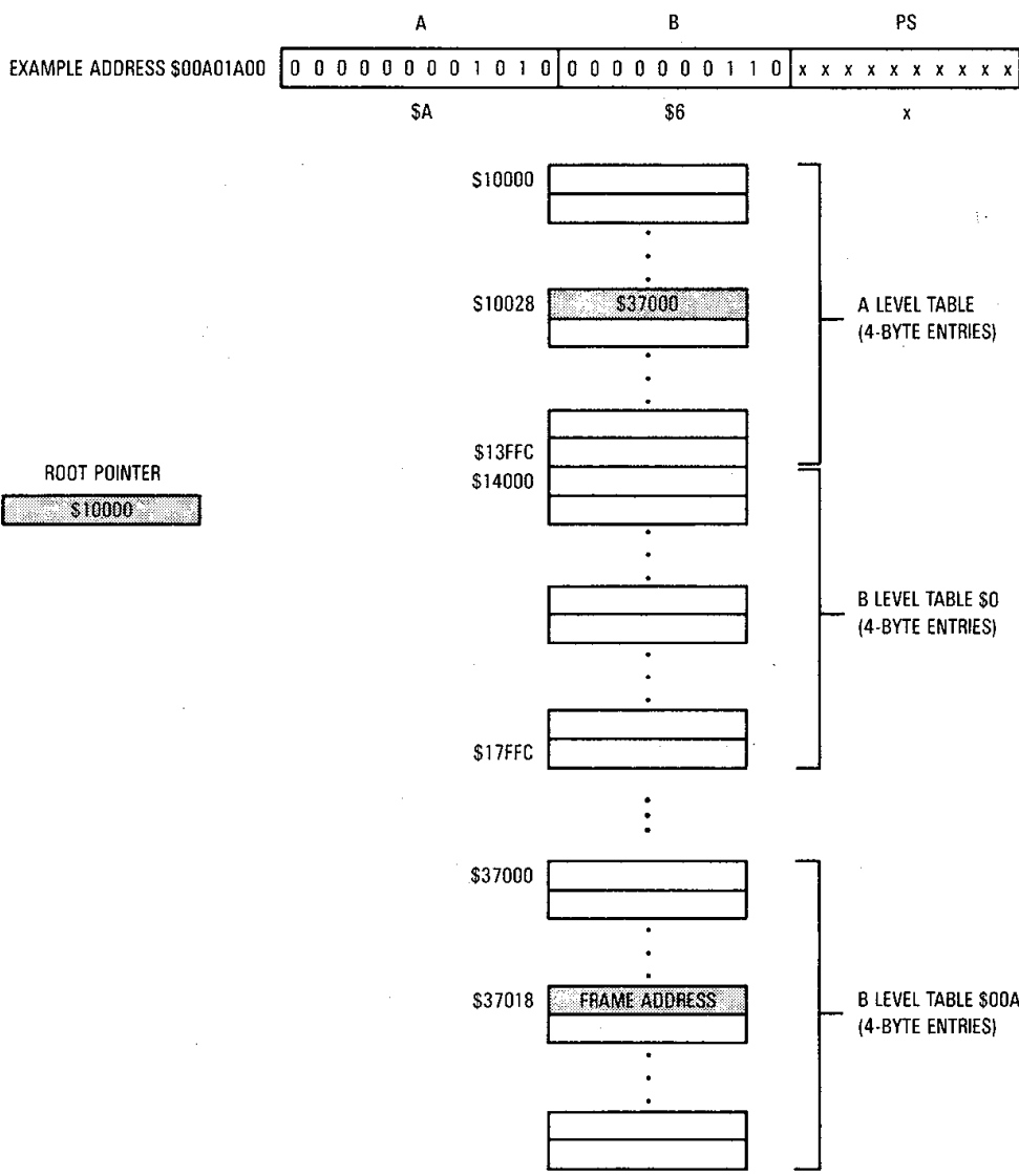
Figure 9-5. Example Translation Tree Layout in Memory
