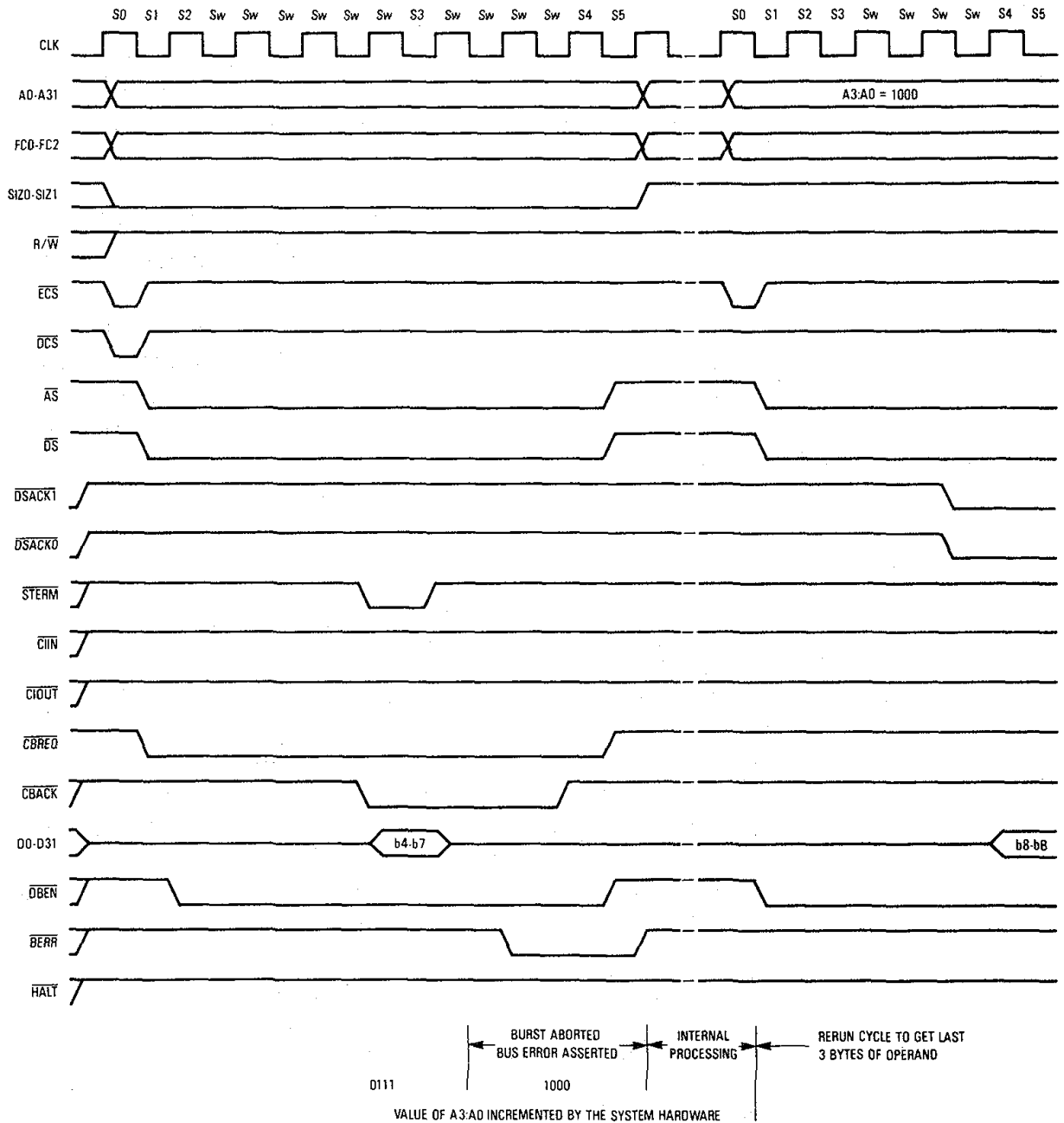
Figure 7-53. Long-Word Operand Request — \overline{\text{BERR}} on Second Access
