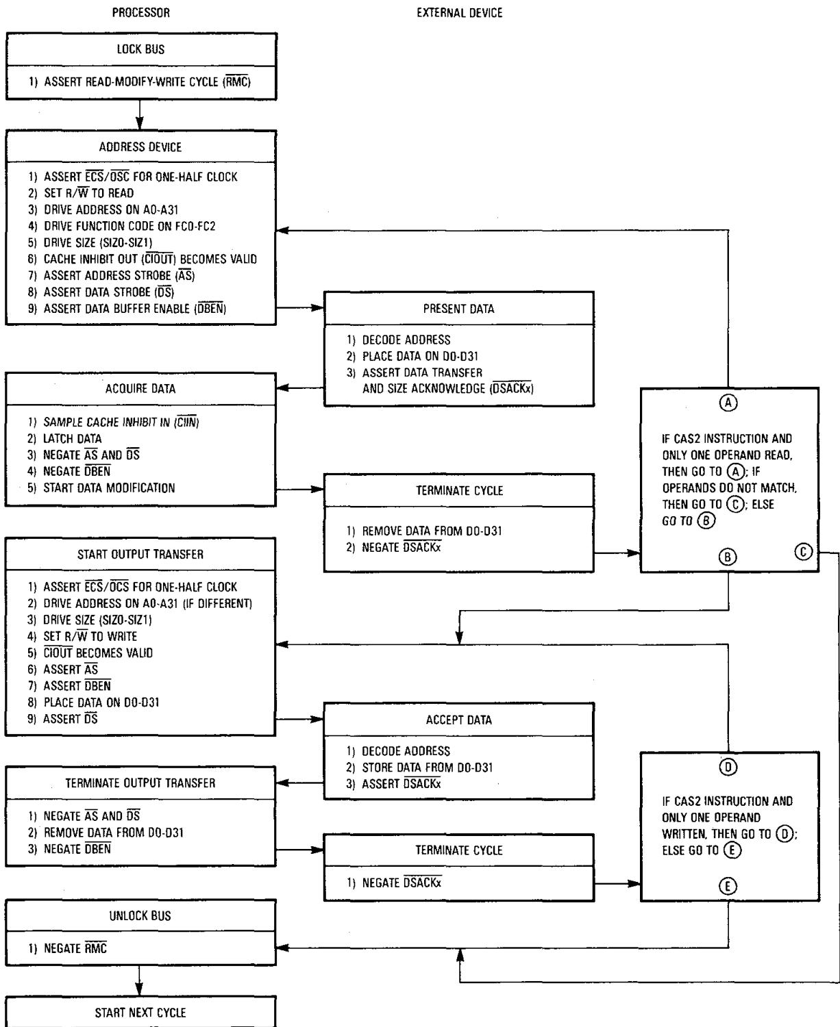
Figure 7-29. Asynchronous Read-Modify-Write Cycle Flowchart
