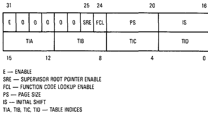
Figure 9-36. Translation Control Register (TC) Format
