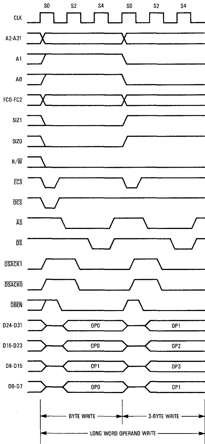
Figure 7-16. Misaligned Write Cycles to Long-Word Port
