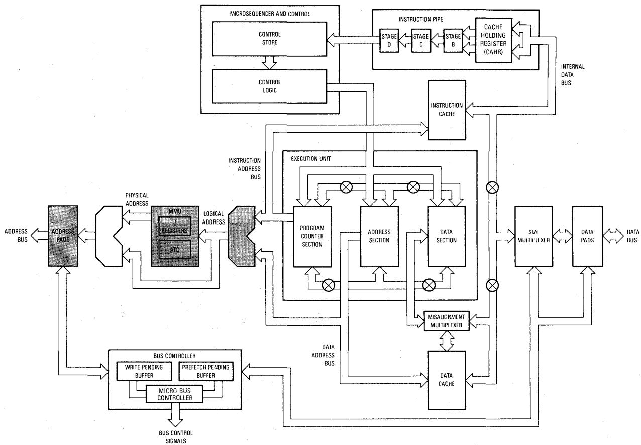
Figure 9-1. MMU Block Diagram
