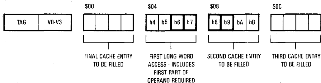
Figure 6-12. Burst Filling Wraparound Example
