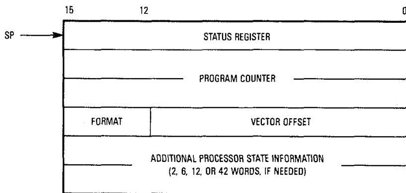
Figure 4-1. General Exception Stack Frame
