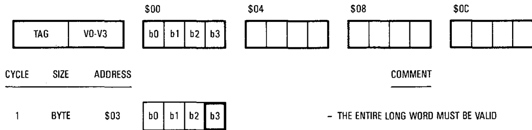
Figure 6-7. Single Entry Mode Operation — 32-Bit Port
