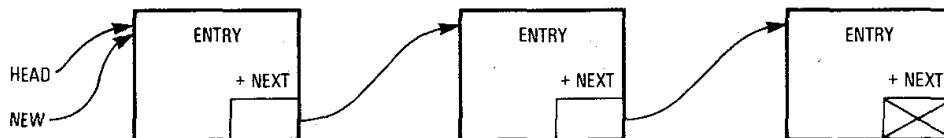
Figure 3-2. Linked List Insertion
