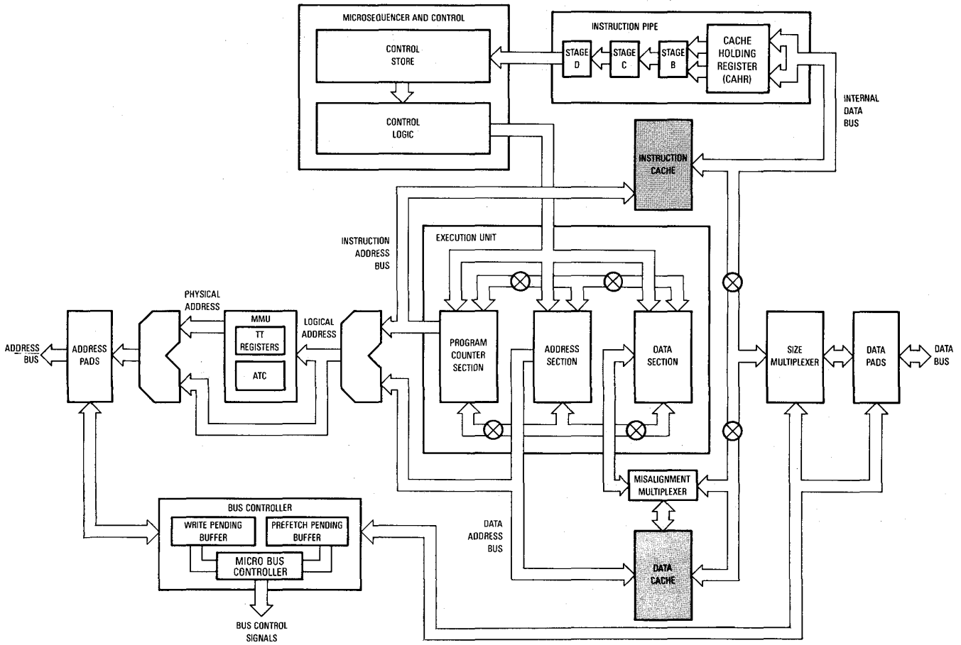
Figure 6-1. Internal Caches and the MC68030
