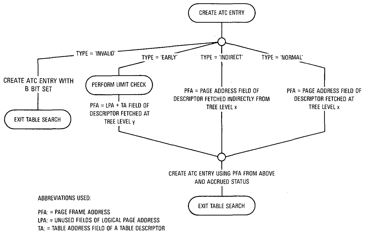
Figure 9-27. ATC Entry Creation Flowchart
