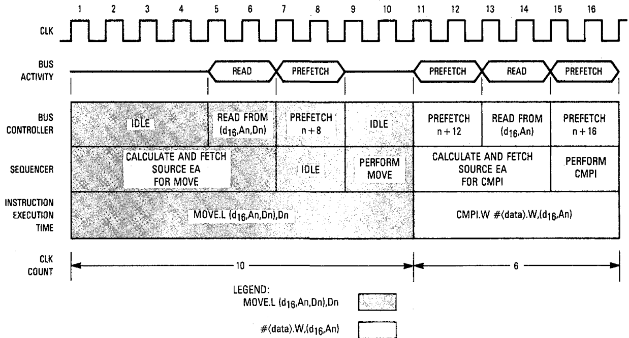
Figure 11-5. Processor Activity — Odd Alignment
