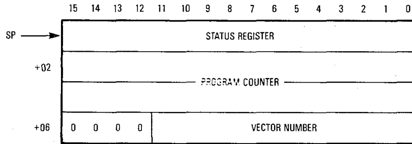
Figure 10-41. MC68030 Pre-Instruction Stack Frame
