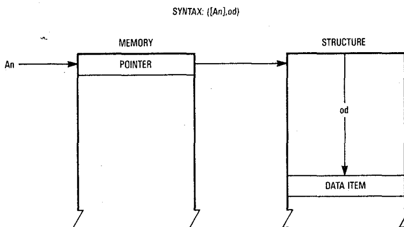
Figure 2-9. Accessing an Item in a Structure Using Pointer
