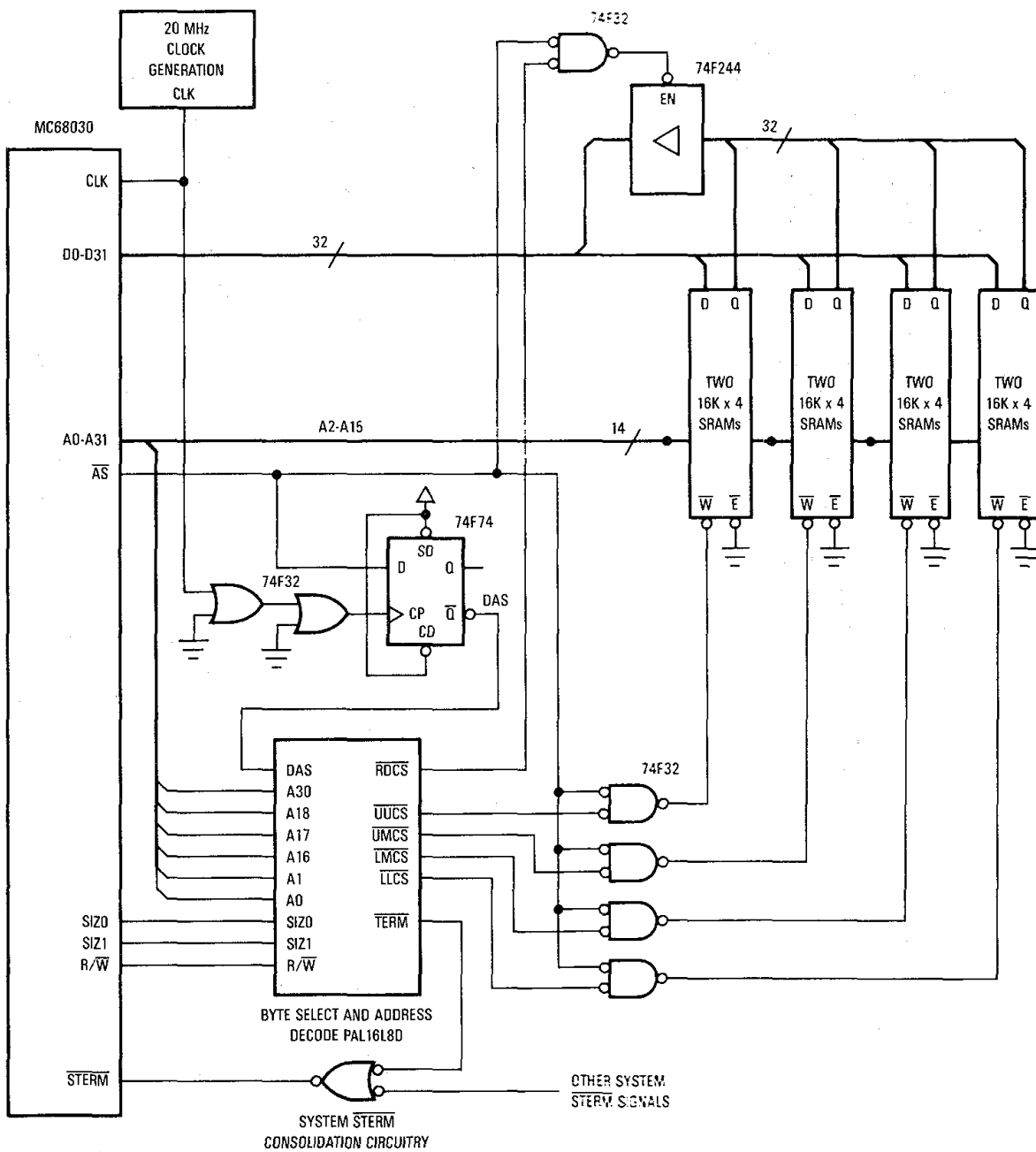
Figure 12-9. Example Two-Clock Read, Three-Clock Write Memory Bank
