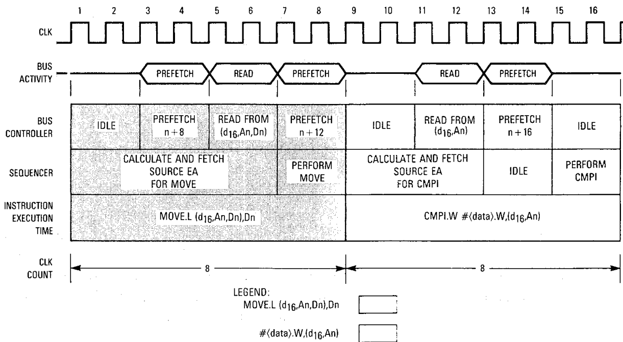
Figure 11-4. Processor Activity — Even Alignment
