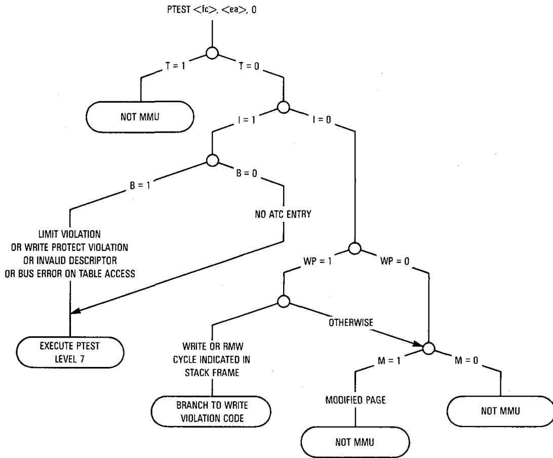
Figure 9-39. MMU Status Interpretation PTEST Level 0
