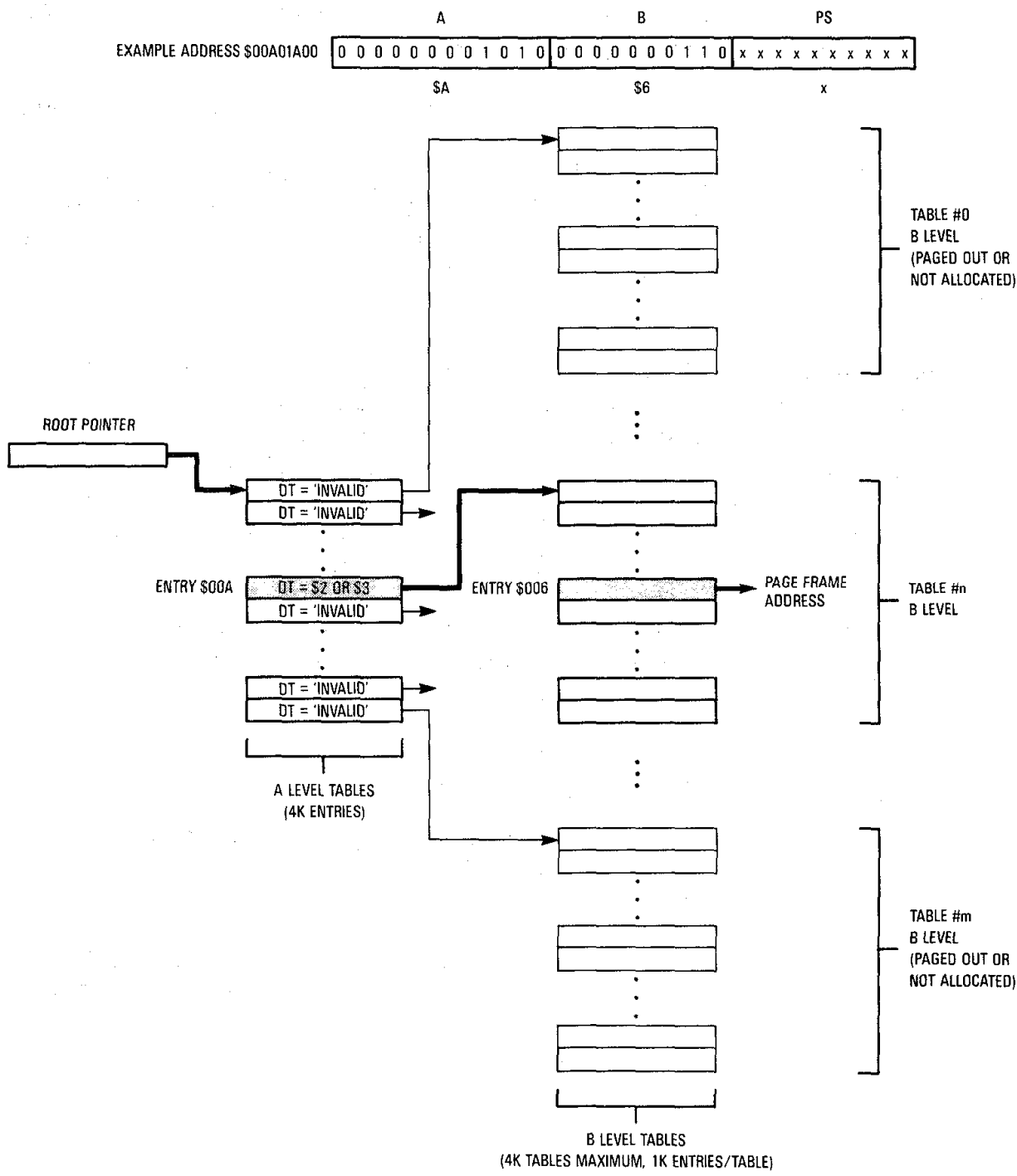
Figure 9-24. Example Translation Tree with Nonresident Tables
