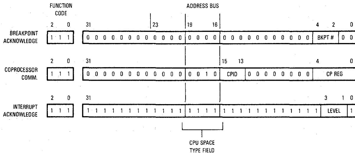
Figure 7-42. MC68030 CPU Space Address Encoding
