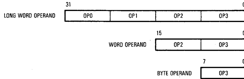
Figure 7-3. Internal Operand Representation
