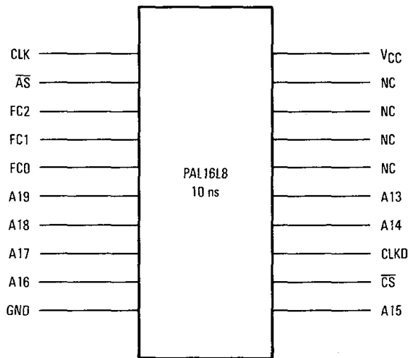
Figure 12-3. Chip-Select Generation PAL
