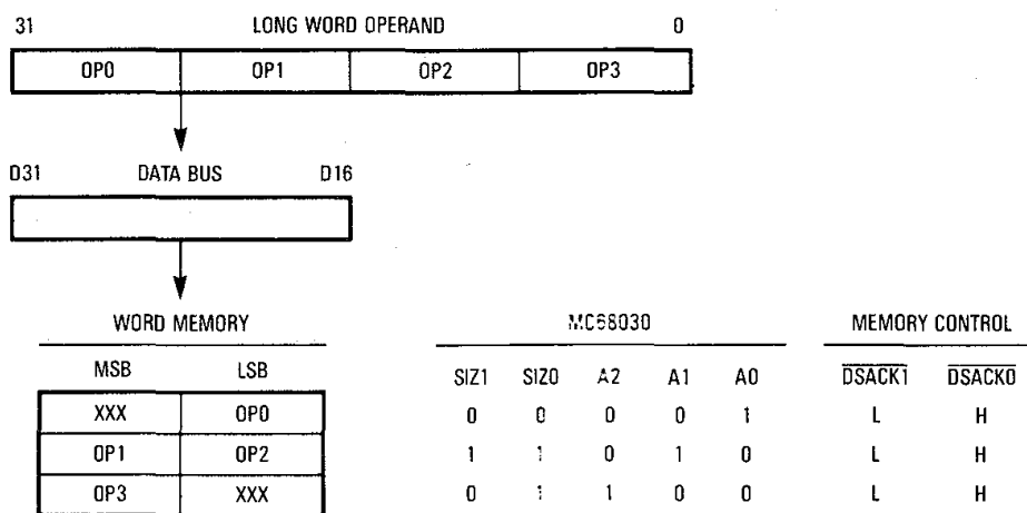
Figure 7-9. Misaligned Long-Word Transfer to Word Port Example
