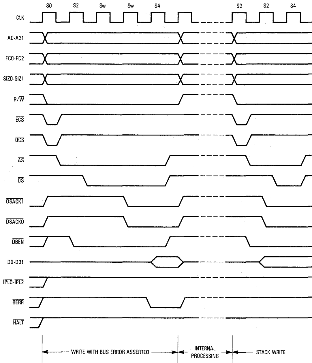
Figure 7-50. Late Bus Error with DSACKx
