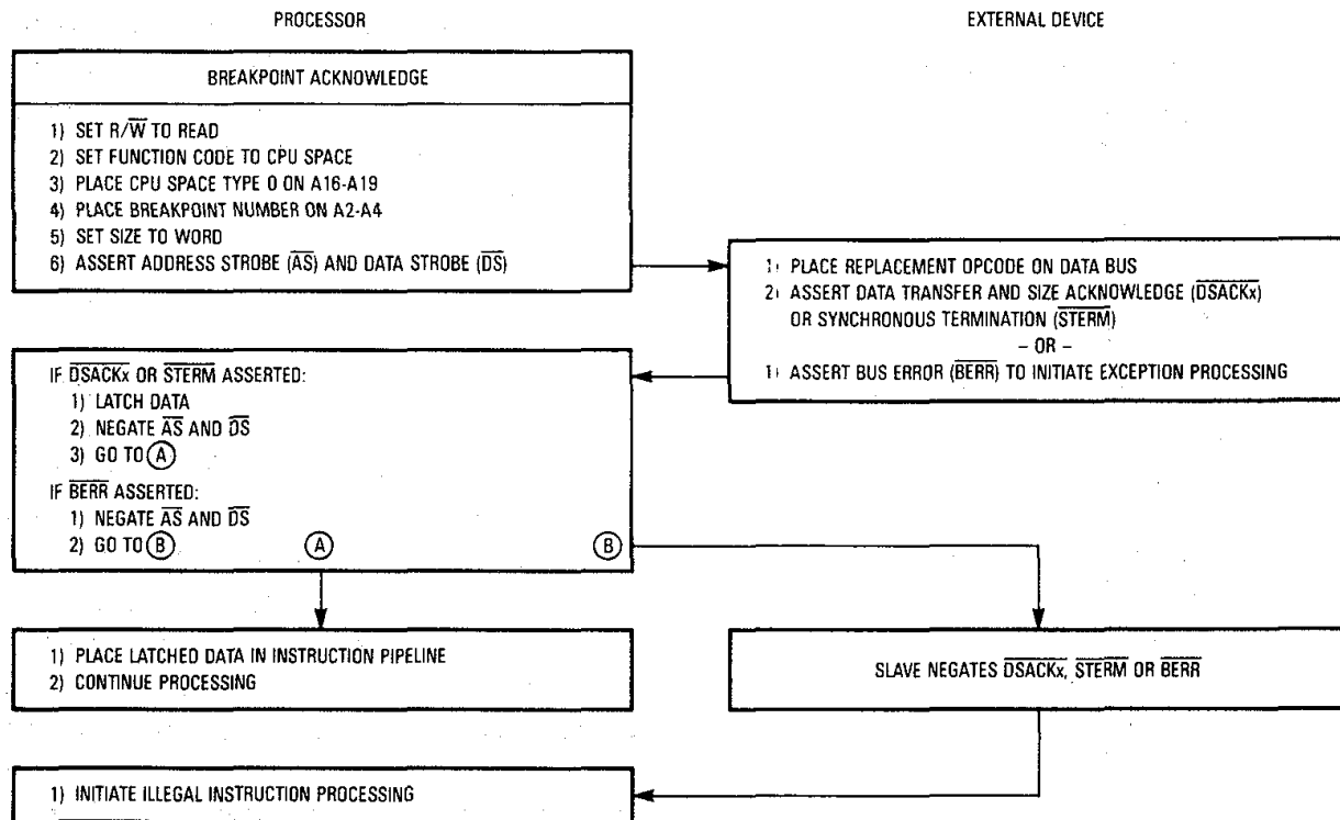
Figure 7-46. Breakpoint Operation Flow
