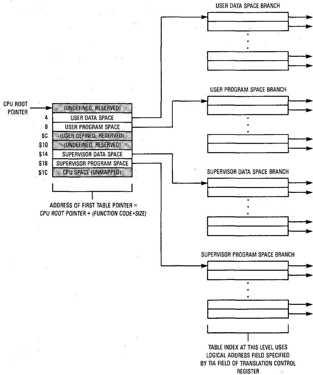
Figure 9-31. Example Translation Tree Using Function Code Lookup
