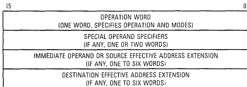
Figure 3-1. Instruction Word General Format
