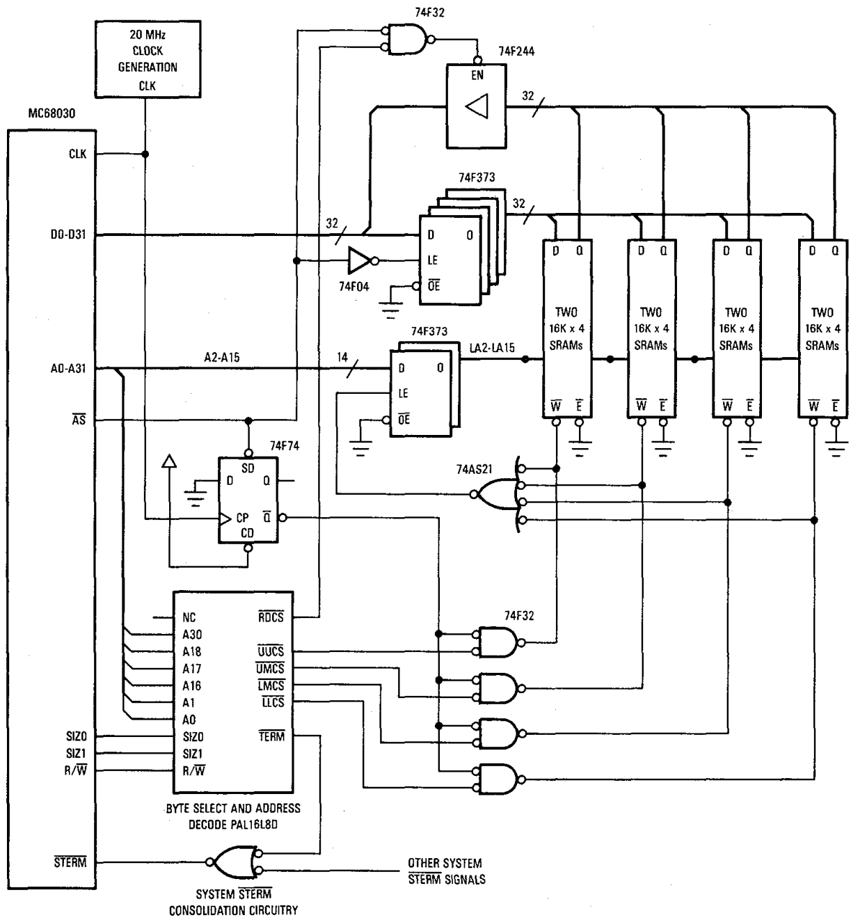
Figure 12-12. Example Two-Clock Read and Write Memory Bank
