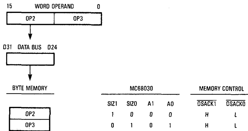
Figure 7-7. Example of Word Transfer to Byte Port
