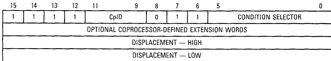
Figure 10-10. Branch On Coprocessor Condition Instruction (cpBcc.L)
