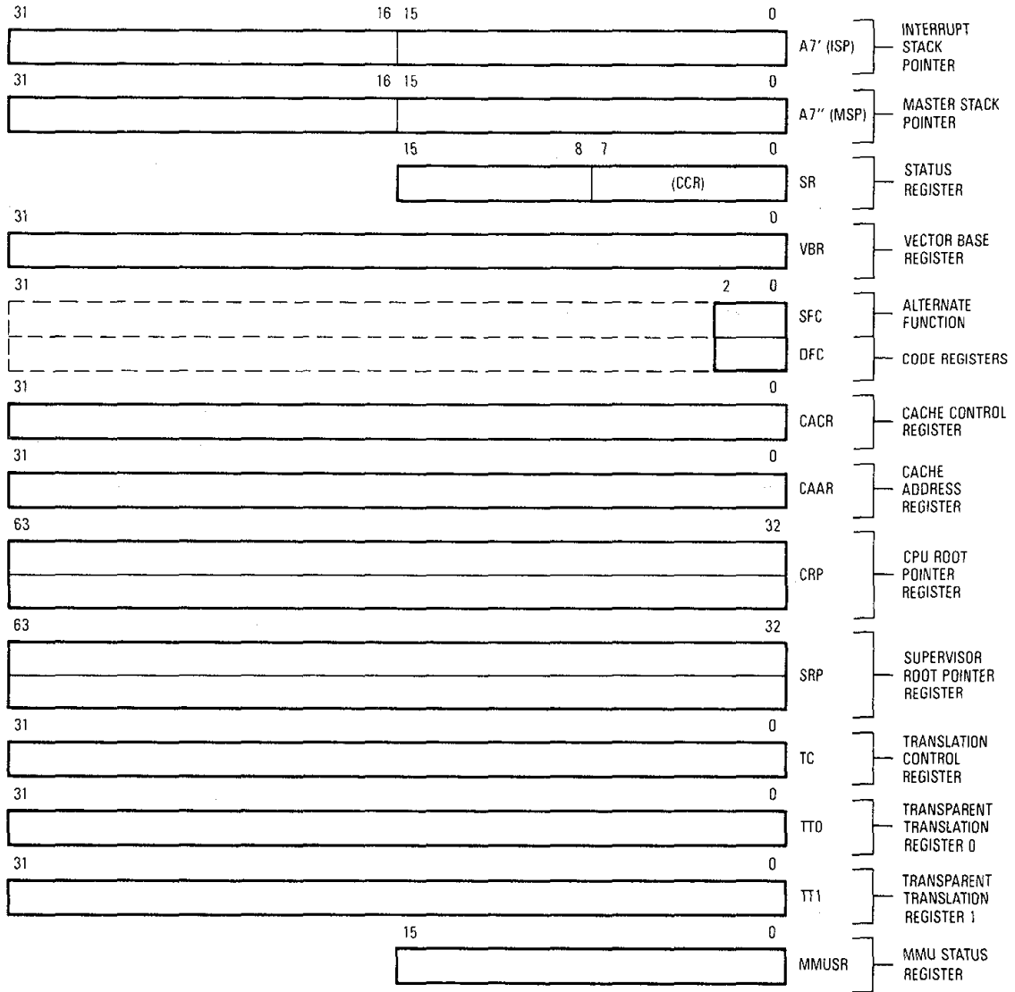
Figure 1-3. Supervisor Programming Model Supplement
