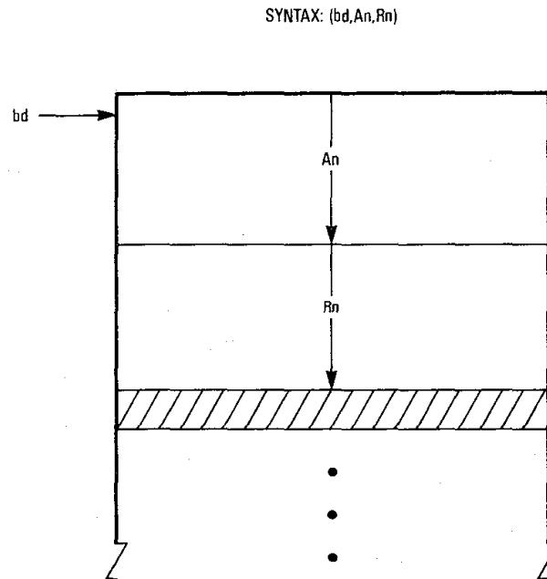
Figure 2-6. Using Absolute Address with Indexes
