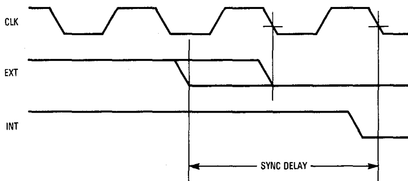
Figure 7-1. Relationship between External and Internal Signals
