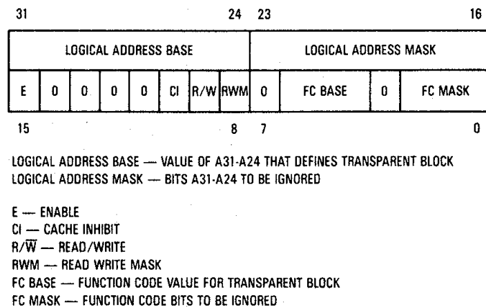
Figure 9-37. Transparent Translation Register (TT0 and TT1) Format
