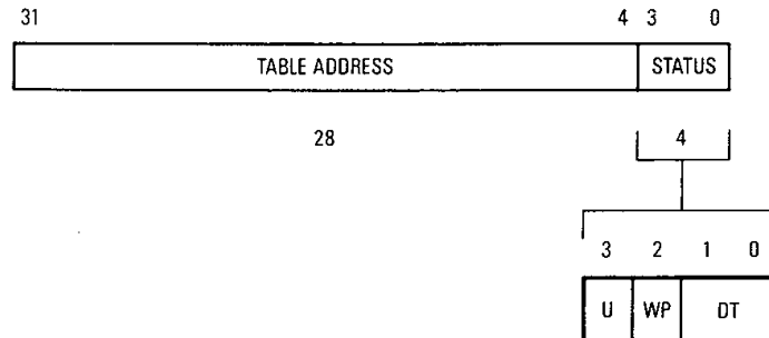
Figure 9-10. Short-Format Table Descriptor
