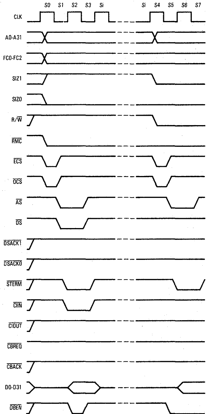
Figure 7-36. Synchronous Read-Modify-Write Cycle Timing — \overline{CIIN} Asserted
