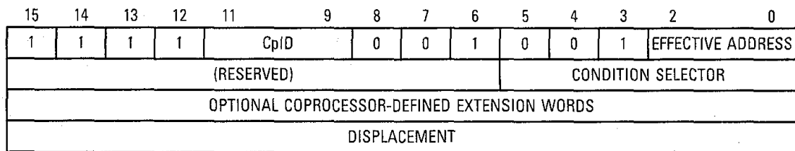
Figure 10-12. Test Coprocessor Condition, Decrement and Branch Instruction Format (cpDBcc)
