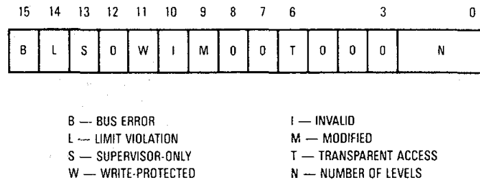
Figure 9-38. MMU Status Register (MMUSR) Format
