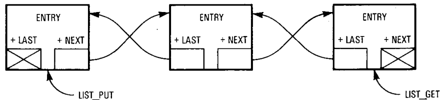
Figure 3-4. Doubly Linked List Insertion
