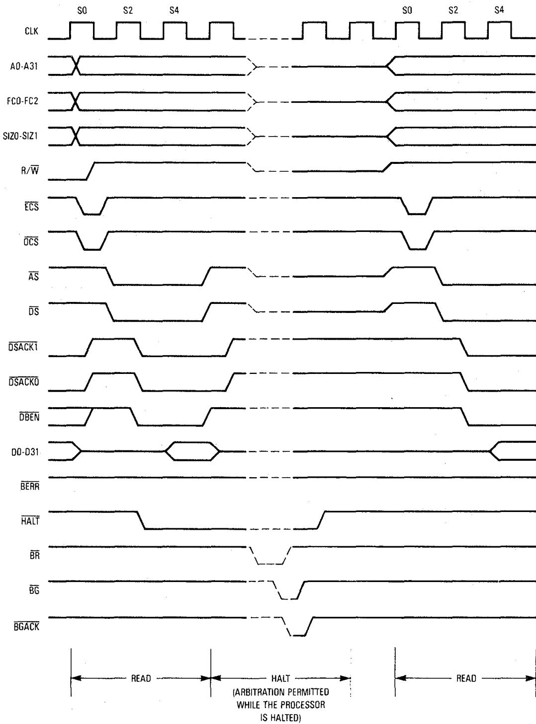
Figure 7-57. Halt Operation Timing
