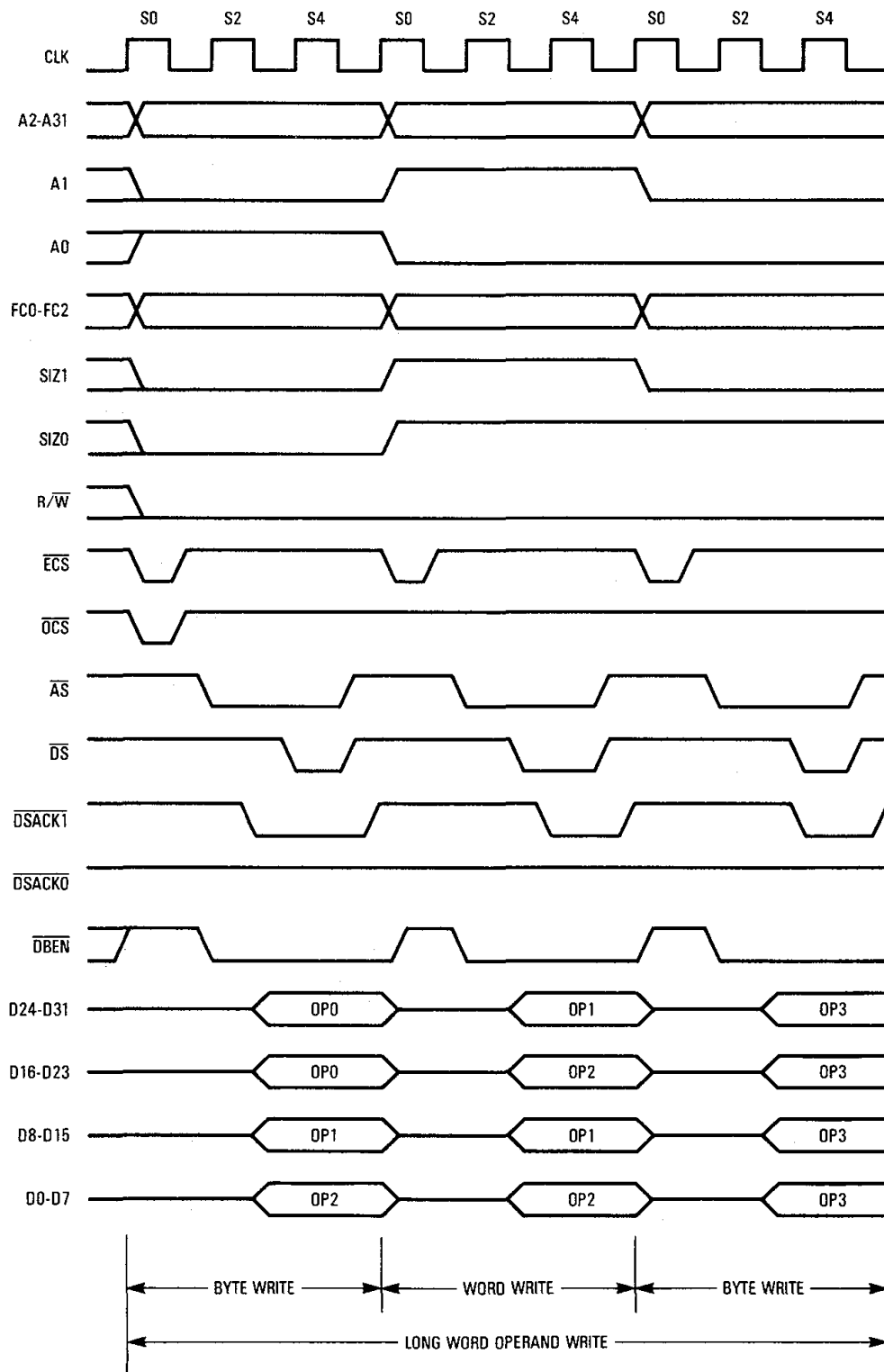
Figure 7-10. Misaligned Long-Word Transfer to Word Port
