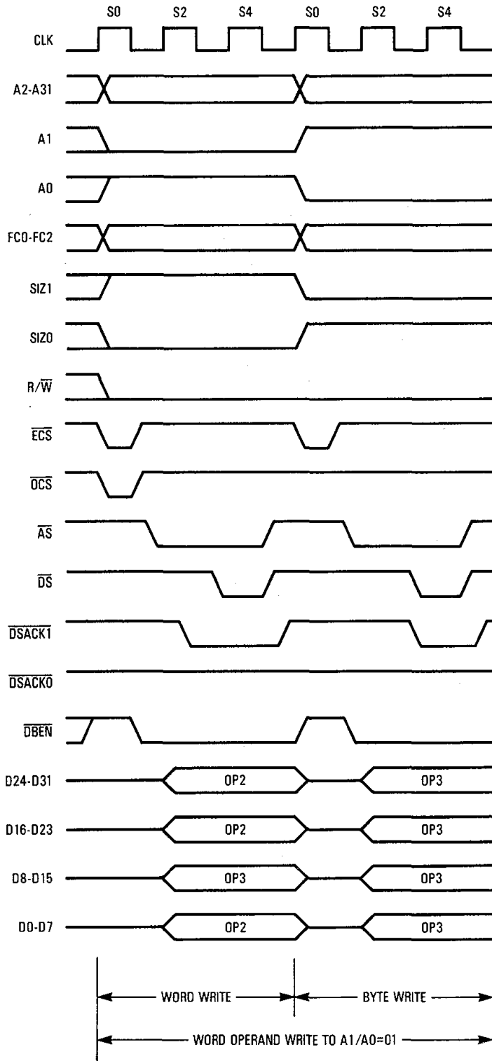
Figure 7-13. Misaligned Word Transfer to Word Port
