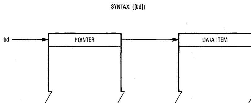
Figure 2-8. Using Indirect Absolute Memory Addressing
