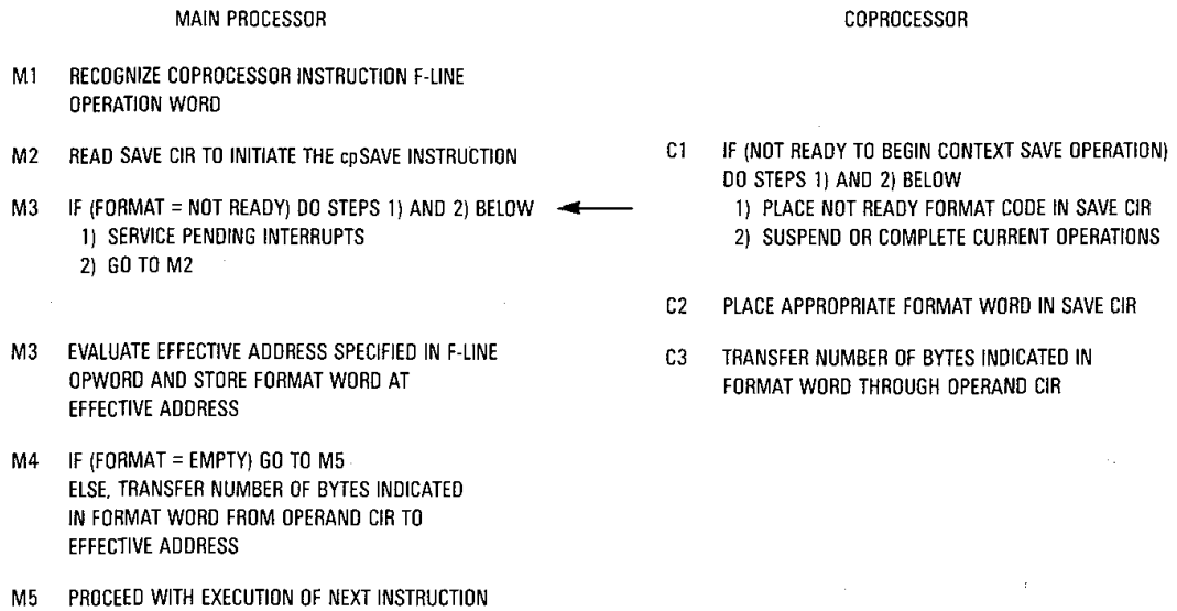
Figure 10-16. Coprocessor Context Save Instruction Protocol
