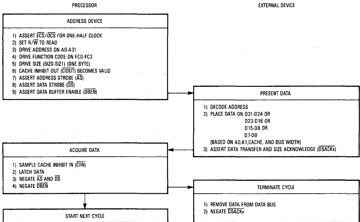
Figure 7-20. Asynchronous Byte Read Cycle Flowchart
