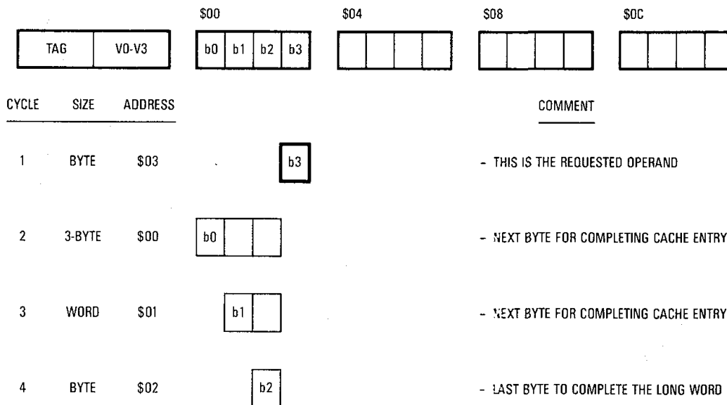
Figure 6-5. Single Entry Mode Operation — 8-Bit Port
