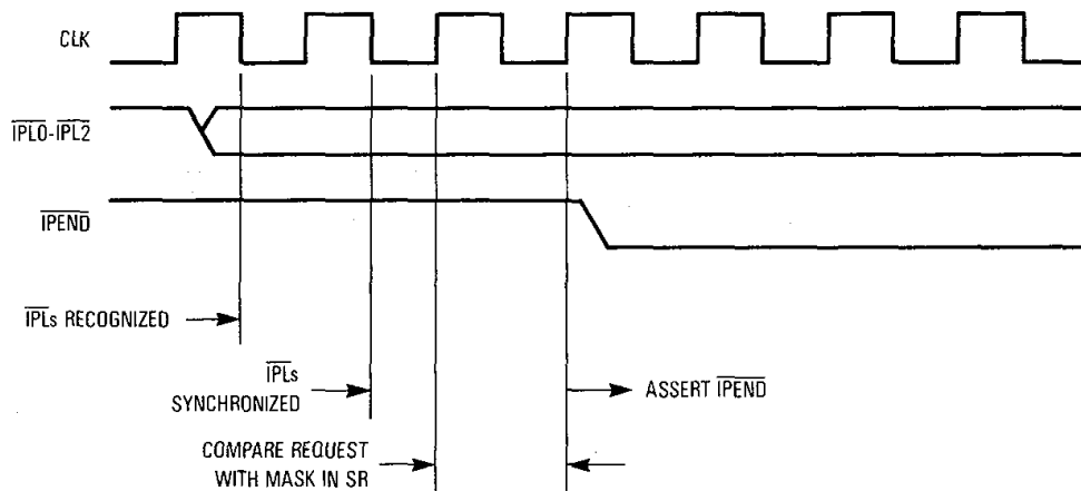
Figure 8-4. Assertion of \overline{IPEND}
