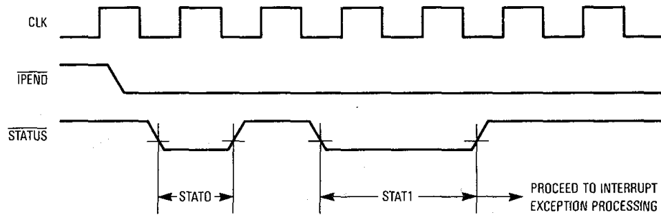
EXAMPLE 1: INTERRUPT EXCEPTION SIGNALLED DURING STAT1
