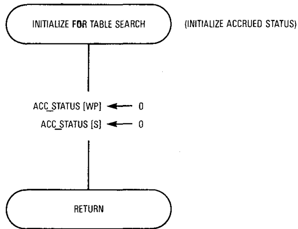
Figure 9-26. Table Search Initialization Flowchart
