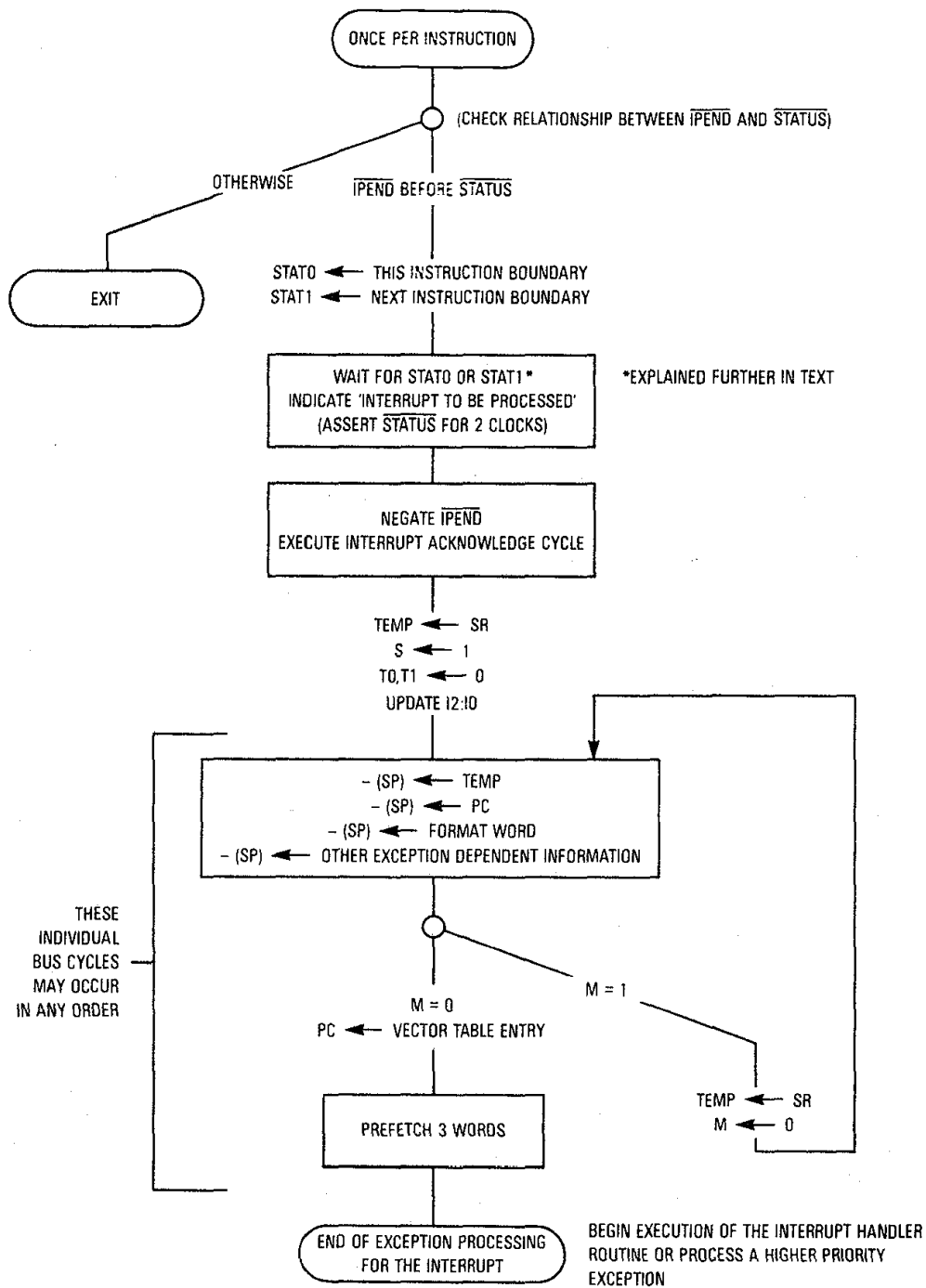
Figure 8-5. Interrupt Exception Processing Flowchart
