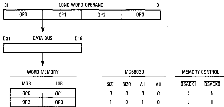
Figure 7-5. Example of Long-Word Transfer to Word Port
