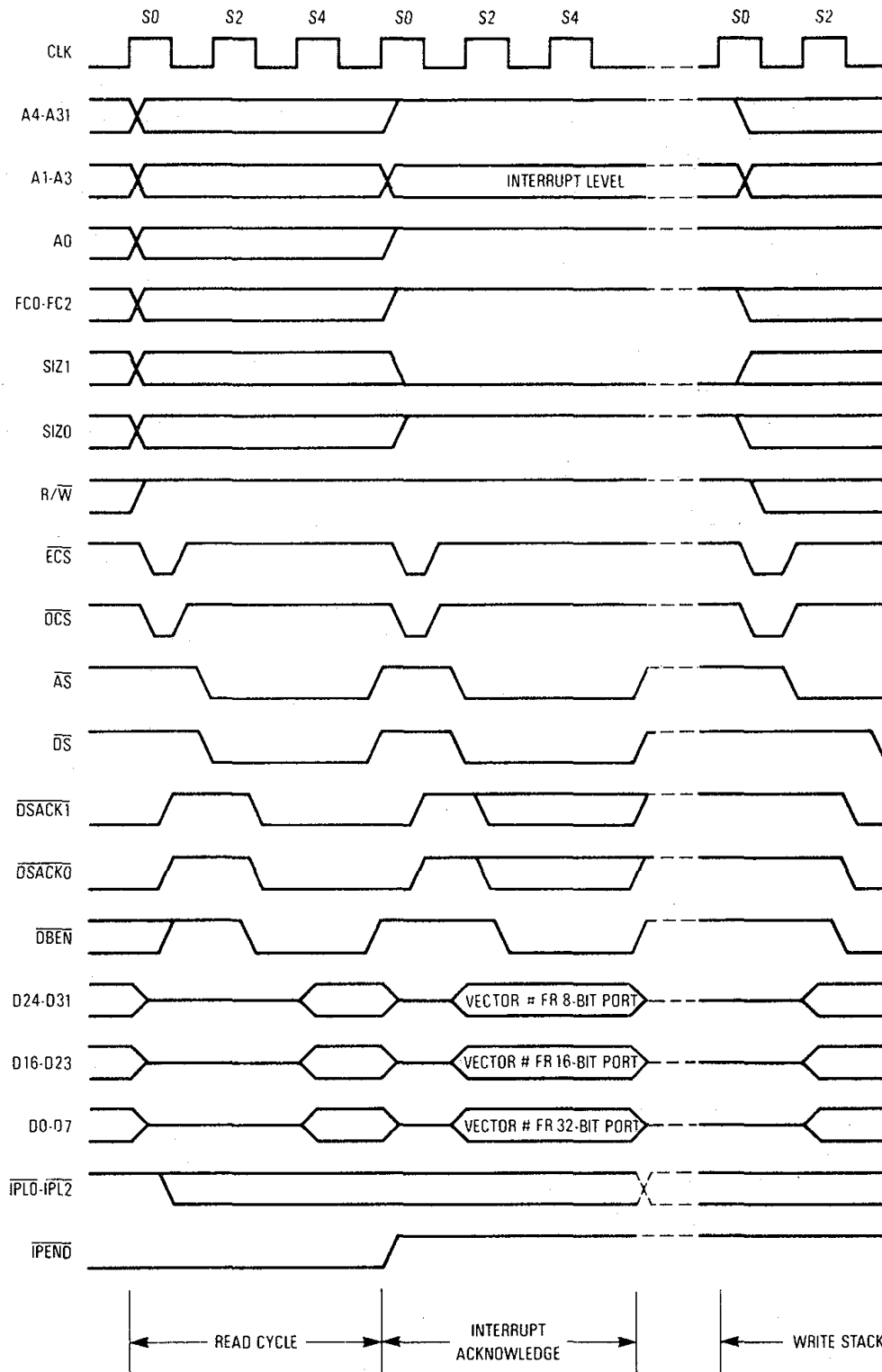
Figure 7-44. Interrupt Acknowledge Cycle Timing
