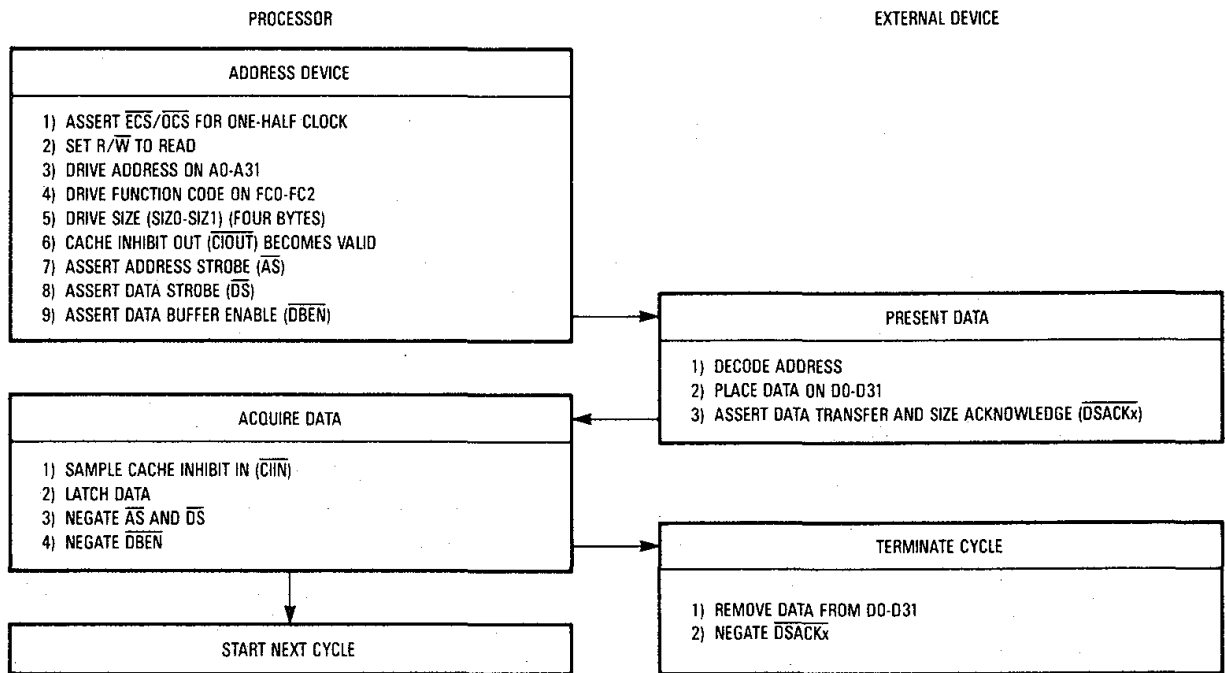
Figure 7-19. Asynchronous Long-Word Read Cycle Flowchart
