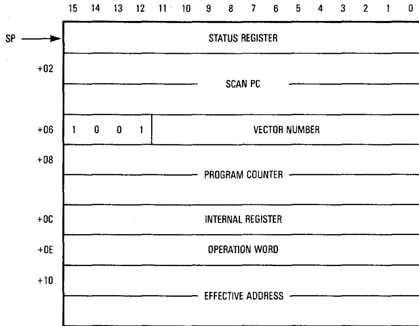
Figure 10-43. MC68030 Mid-Instruction Stack Frame
