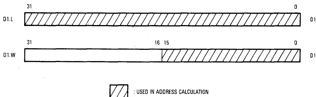
Figure 2-5. Using SIZE in the Index Selection
