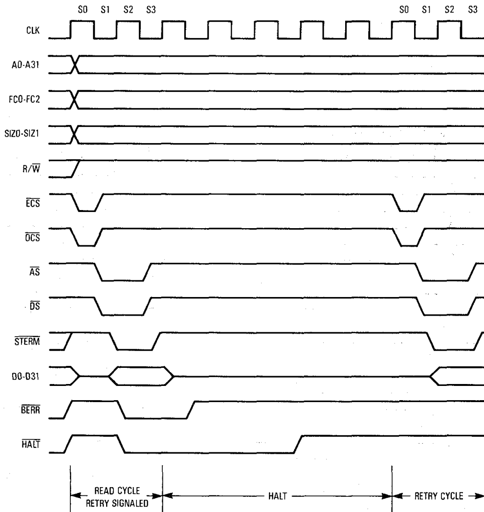
Figure 7-55. Synchronous Late Retry
