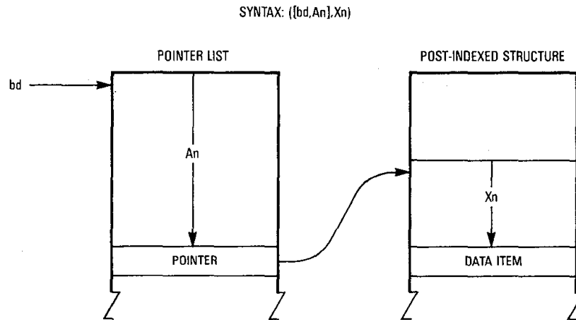
Figure 2-12. Postindexed Indirect Addressing
