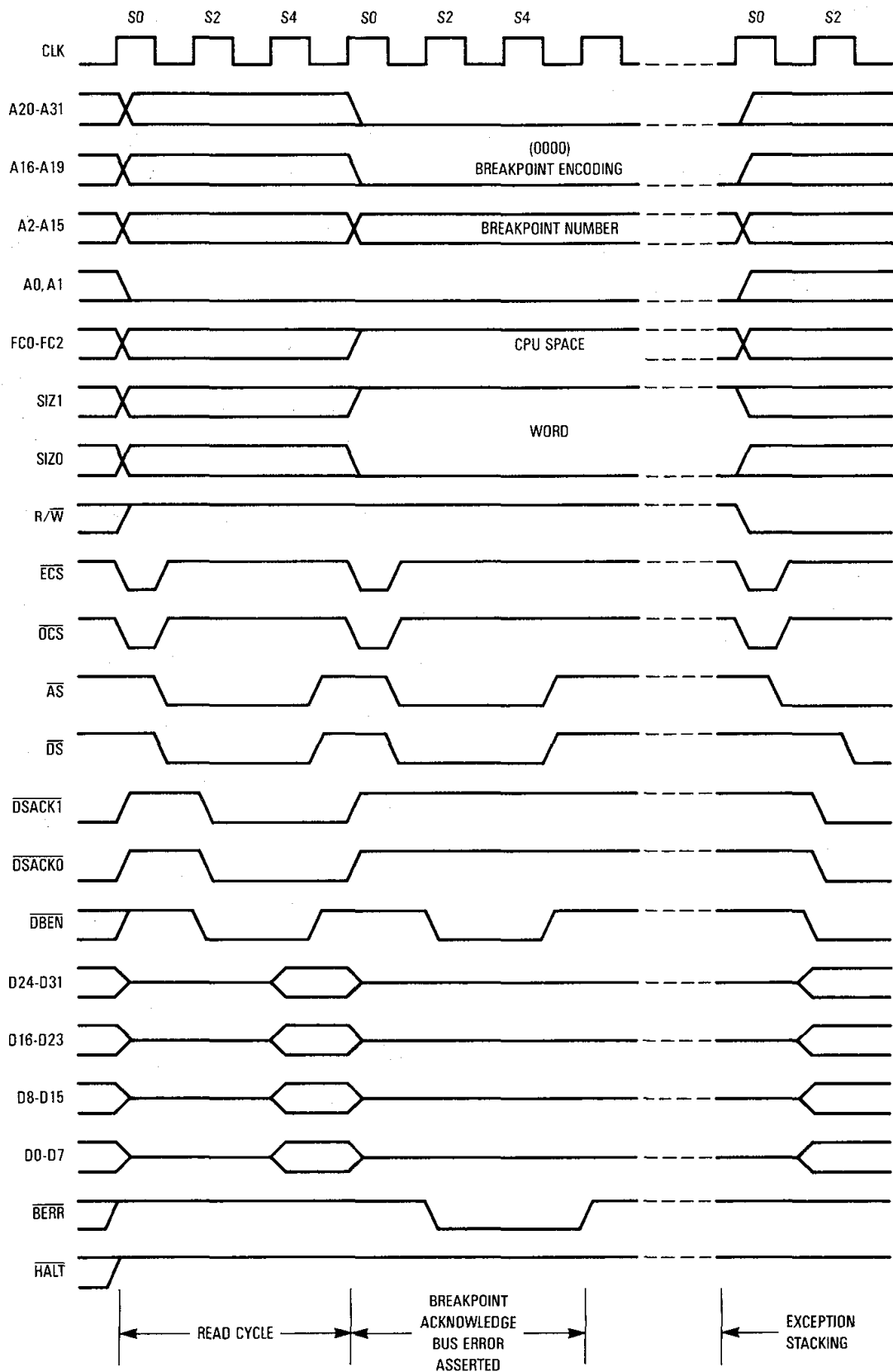
Figure 7-49. Bus Error without \overline{DSACKx}
