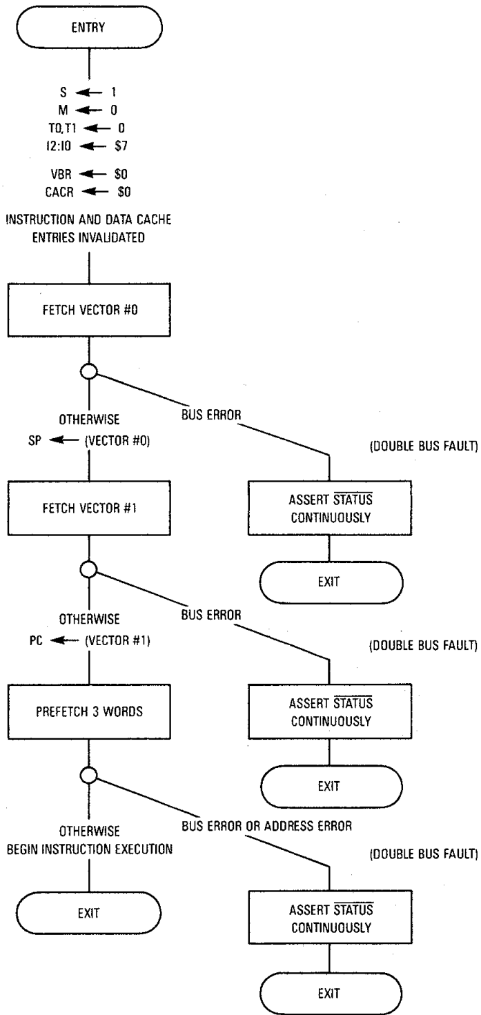
Figure 8-1. Reset Operation Flowchart
