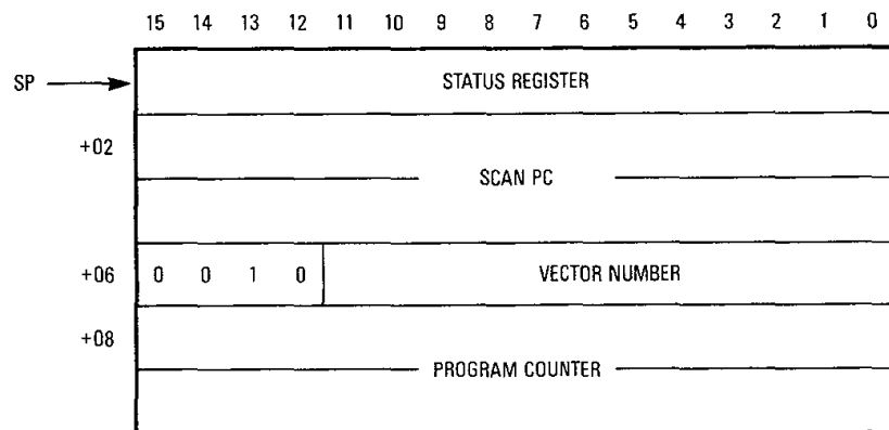
Figure 10-45. MC68030 Post-Instruction Stack Frame
