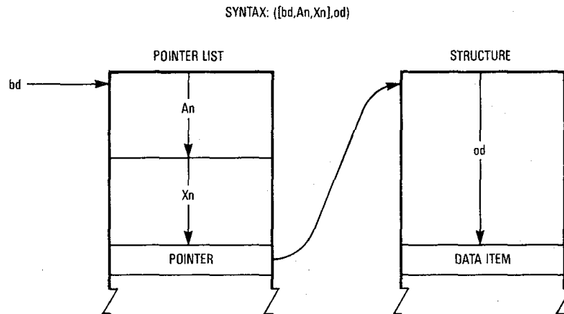
Figure 2-13. Preindexed Indirect Addressing with Outer Displacement
