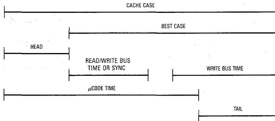
Figure 11-3. Derivation of Instruction Overlap Time
