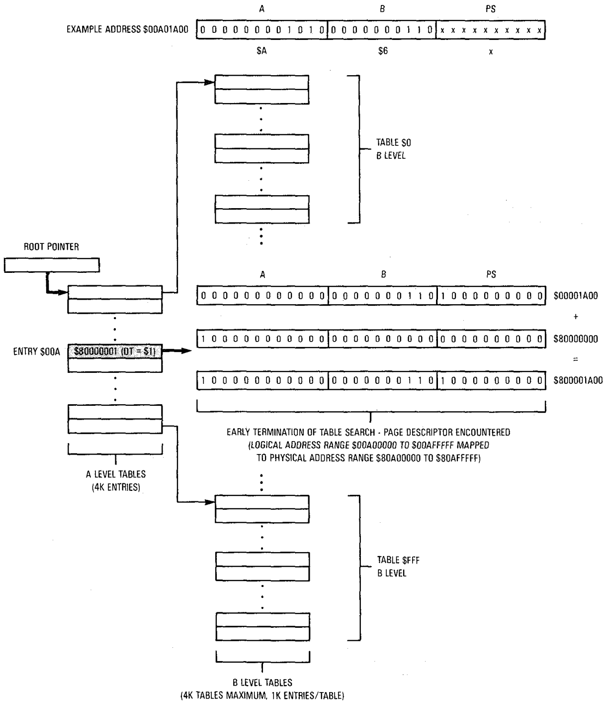
Figure 9-21. Example Translation Tree Using Contiguous Memory
