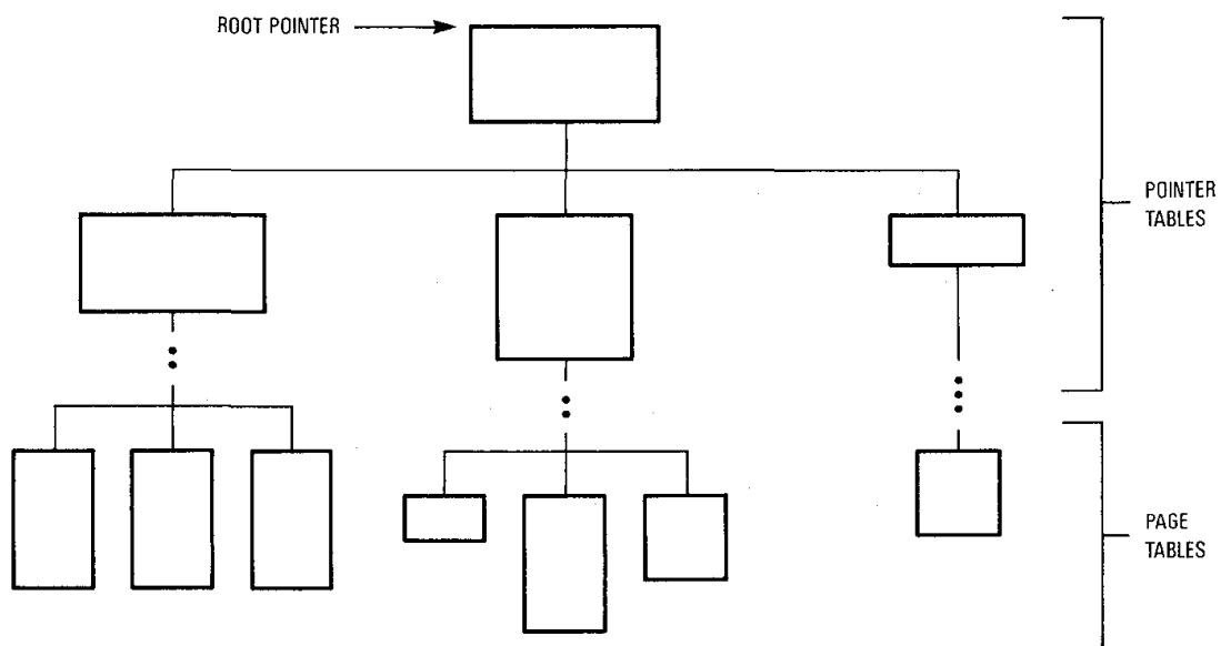
Figure 9-3. Translation Table Tree
