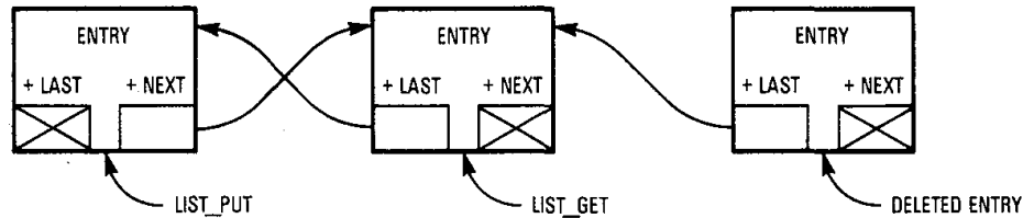
Figure 3-5. Doubly Linked List Deletion
