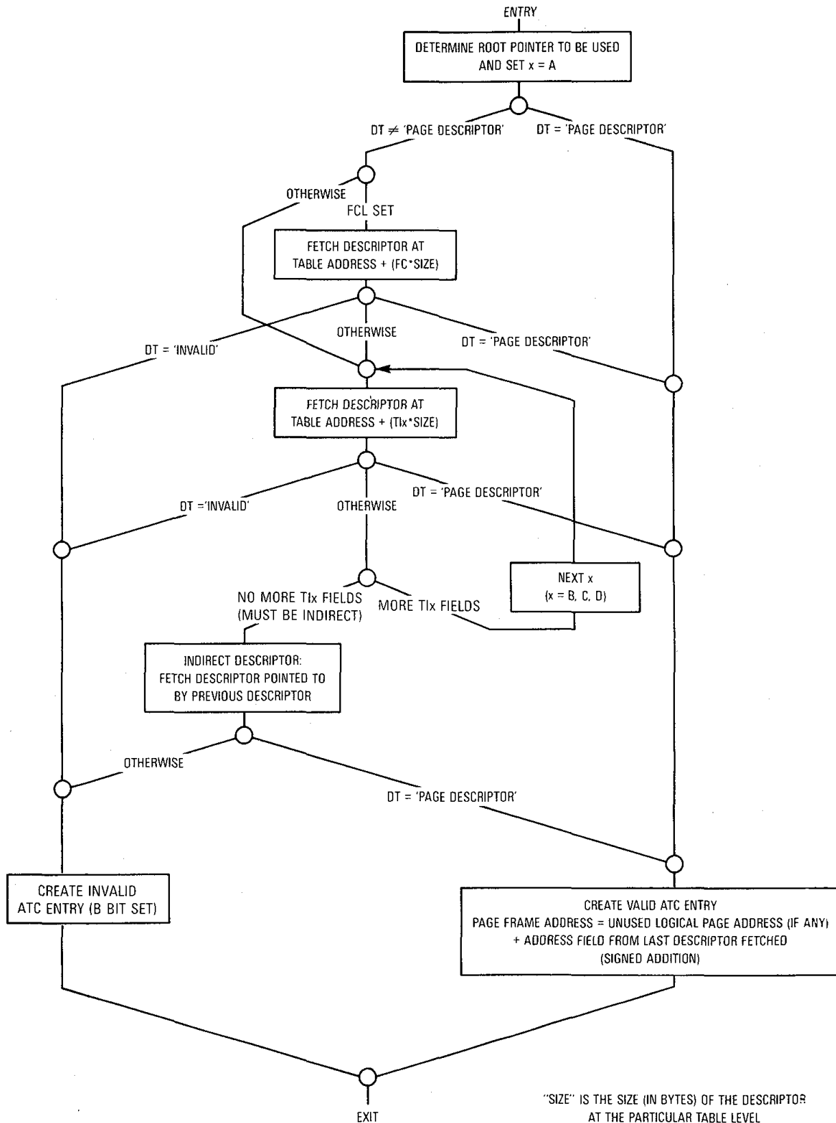
Figure 9-19. Simplified Table Search Flowchart
