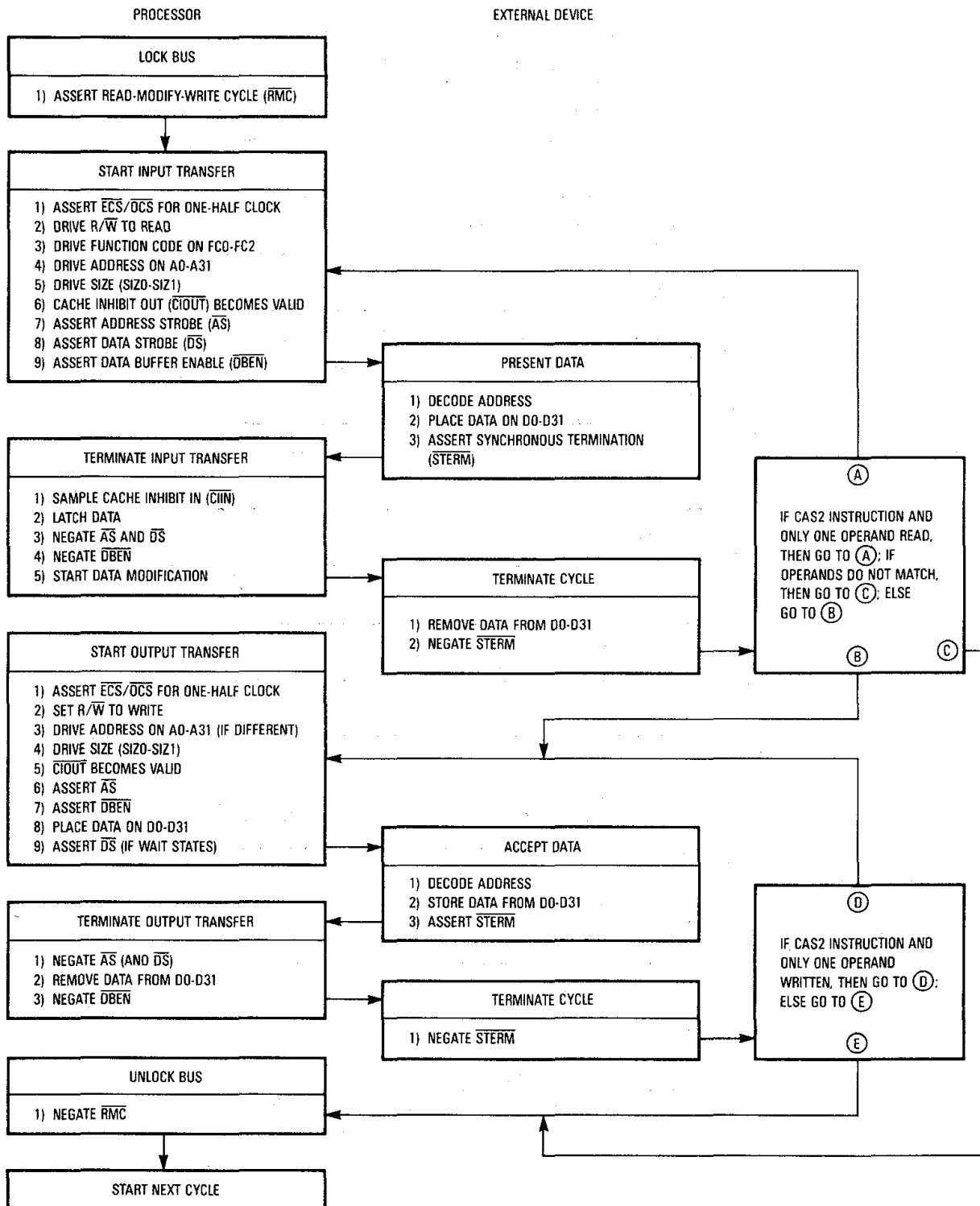
Figure 7-35. Synchronous Read-Modify-Write Cycle Flowchart
