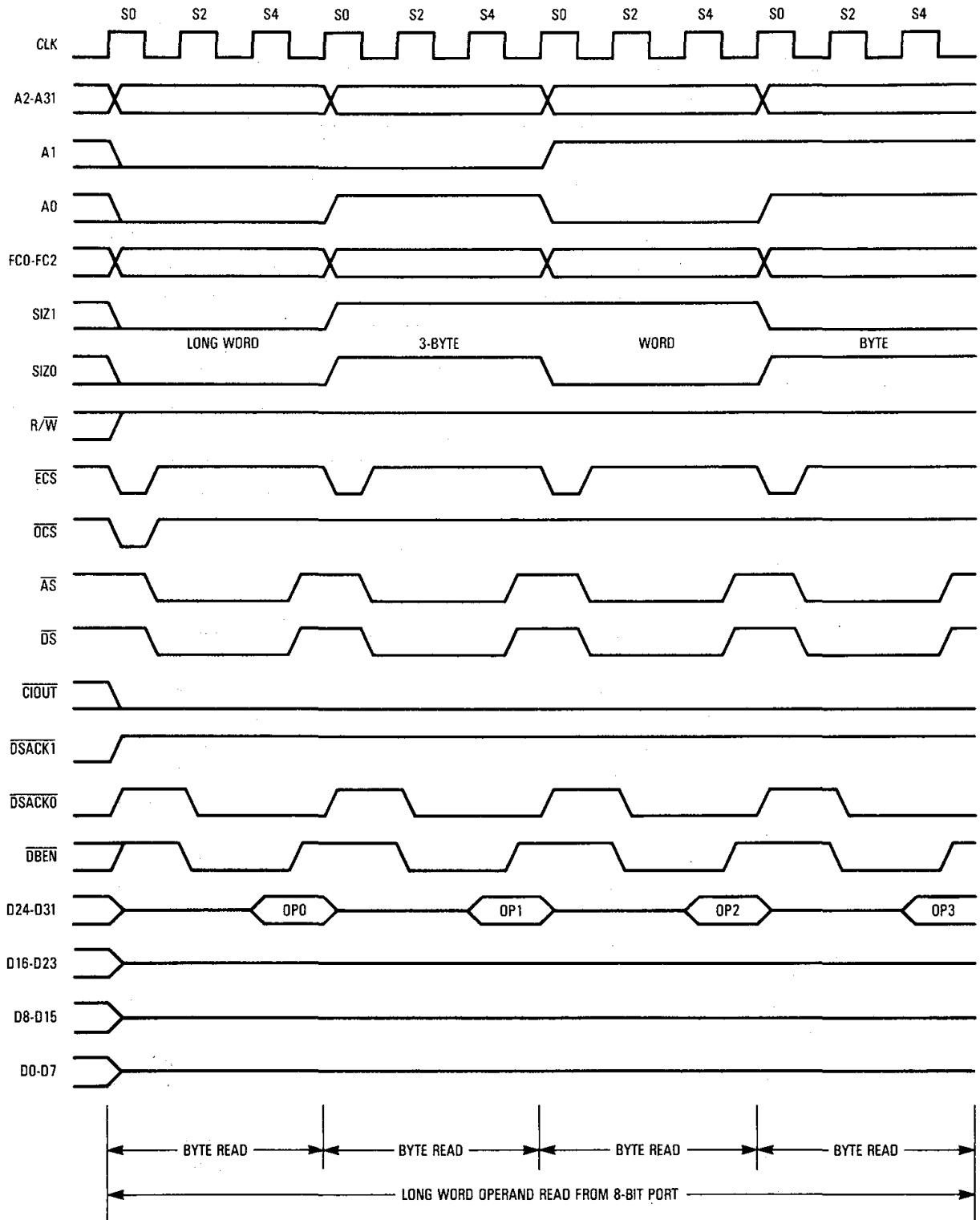
Figure 7-22. Long-Word Read — 8-Bit Port with \overline{CIOUT} Asserted
