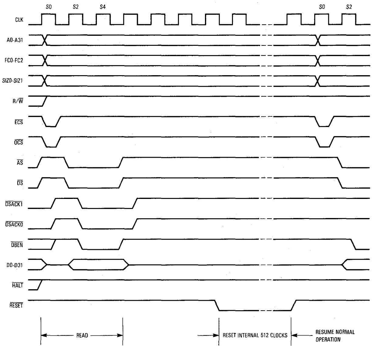
Figure 7-65. Processor-Generated Reset Operation
