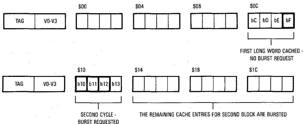
Figure 6-13. Deferred Burst Filling Example
