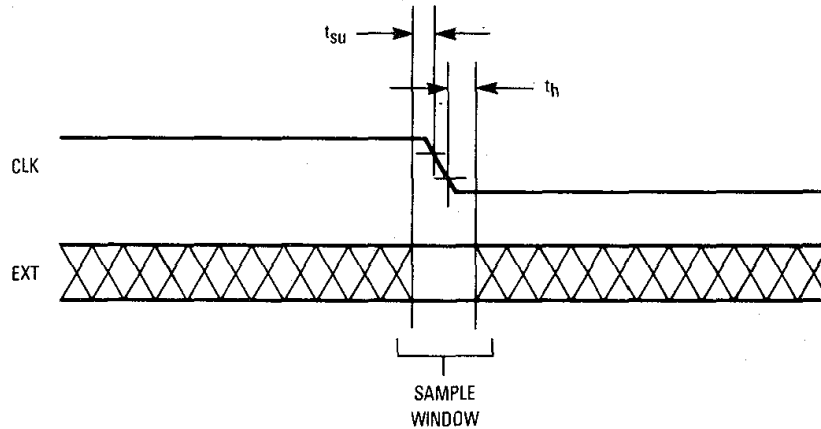
Figure 7-2. Asynchronous Input Sample Window
