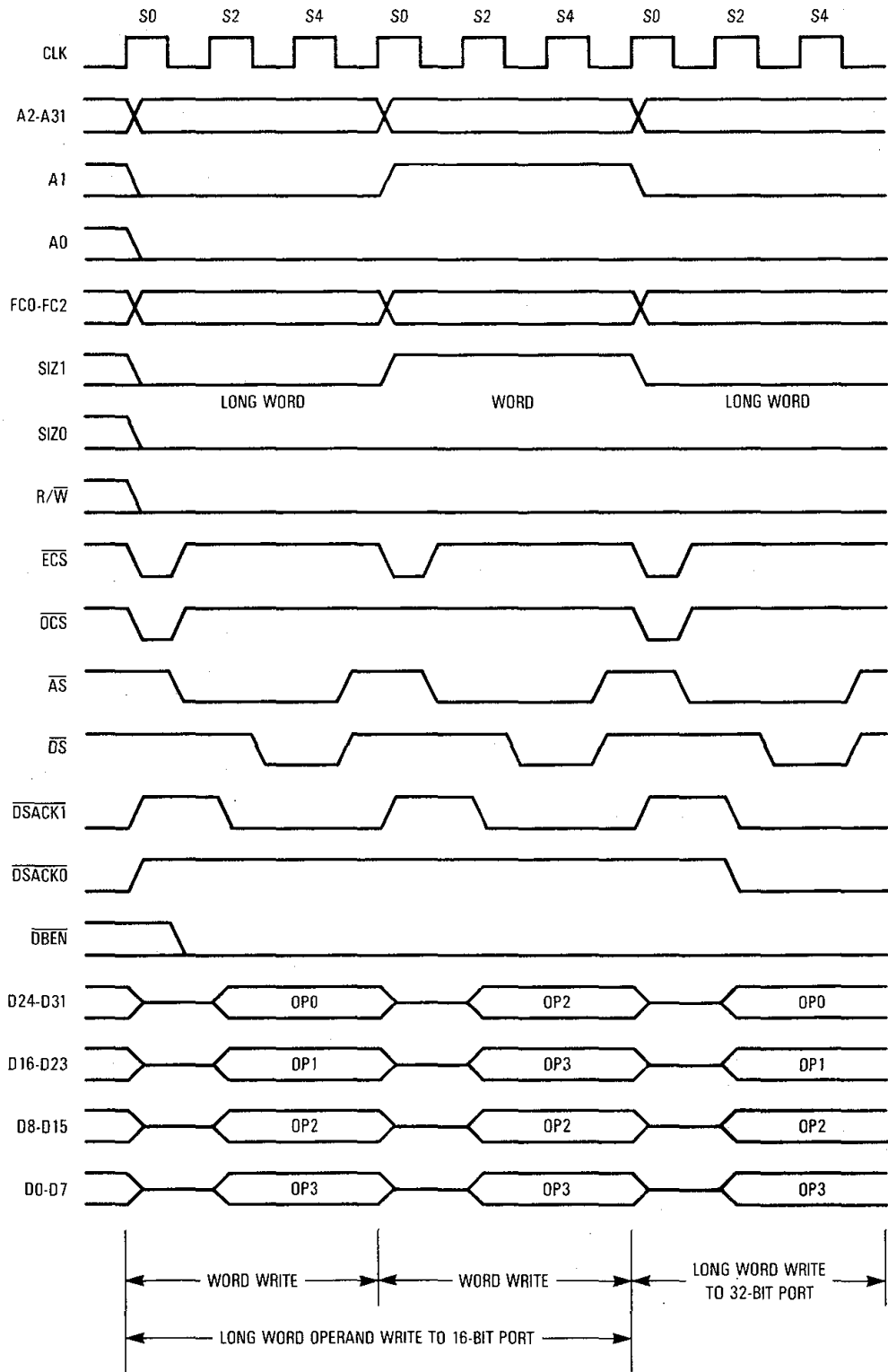
Figure 7-28. Long-Word Operand Write — 16-Bit Port
