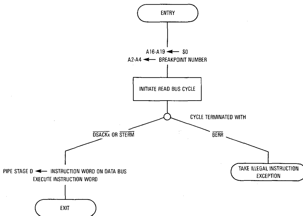
Figure 8-7. Breakpoint Instruction Flowchart
