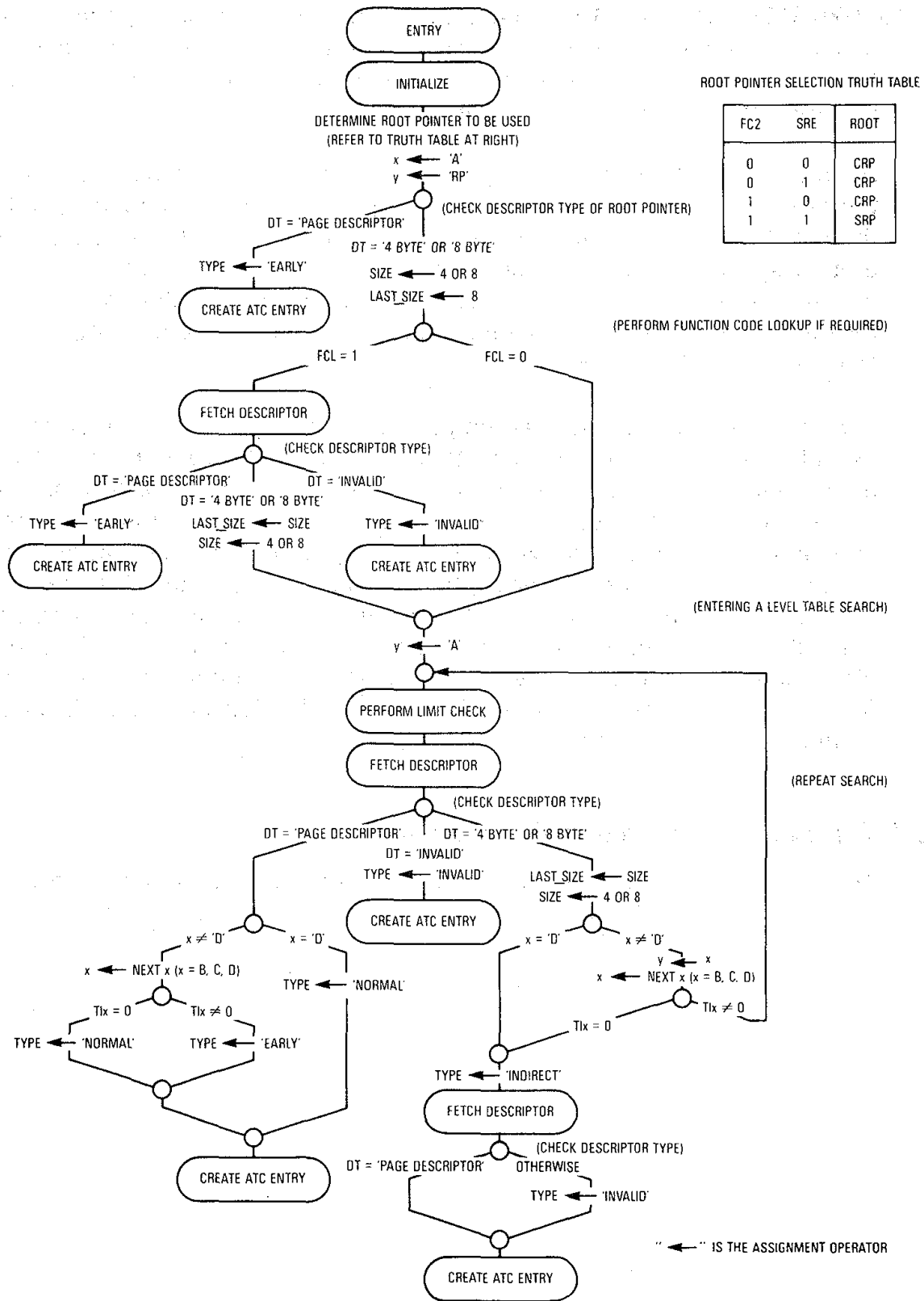
Figure 9-25. Detailed Flowchart of MMU Table Search Operation
