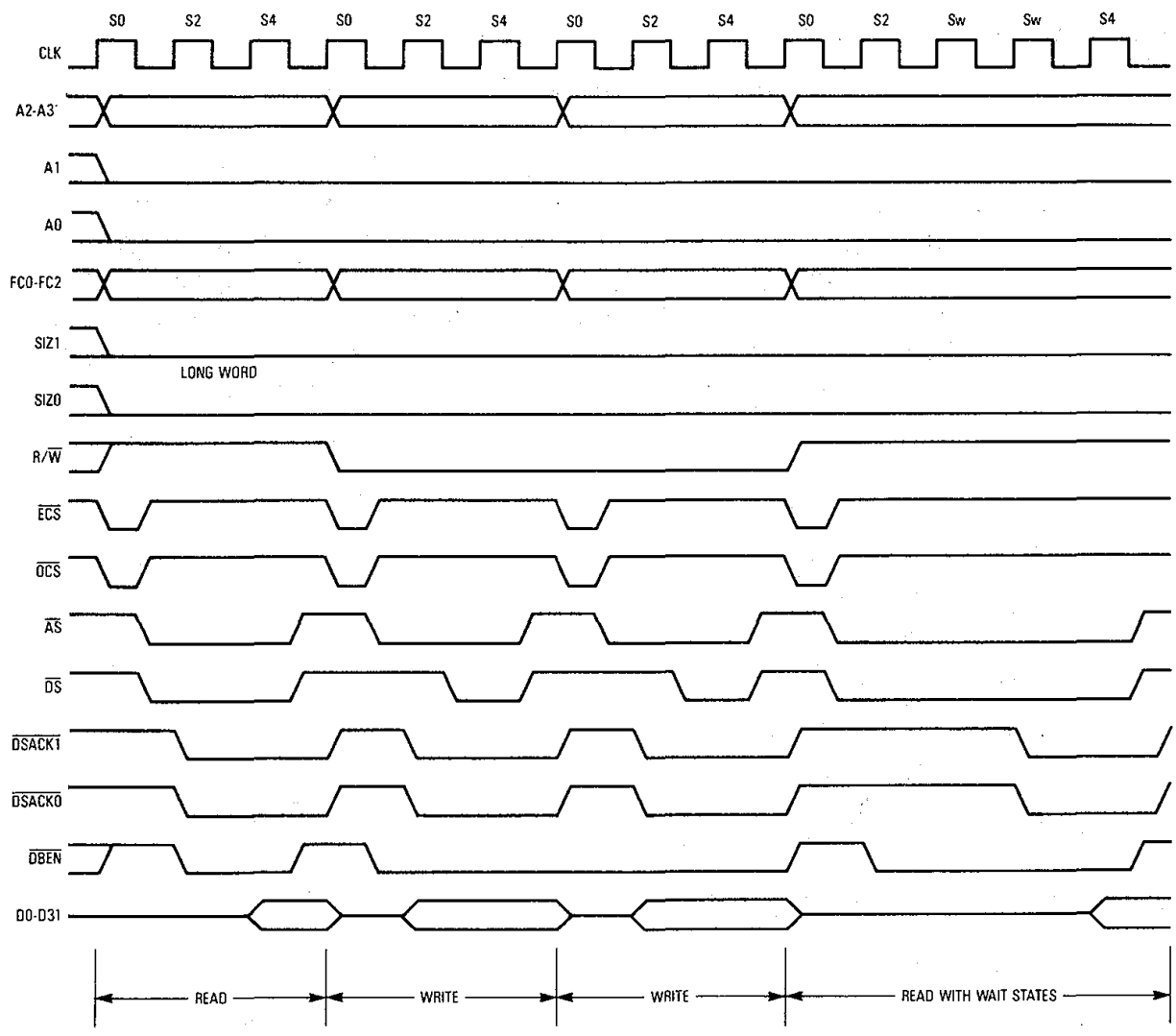
Figure 7-25. Asynchronous Read-Write-Read Cycles — 32-Bit Port
