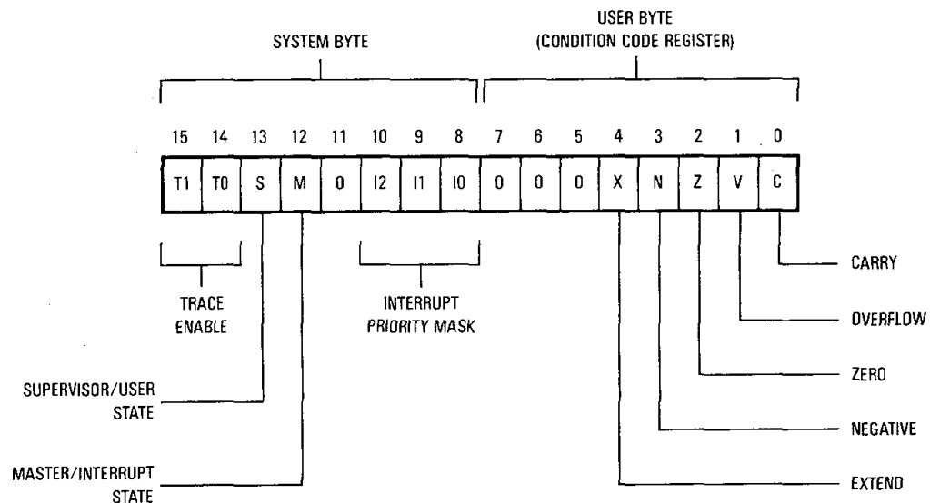
Figure 1-4. Status Register
