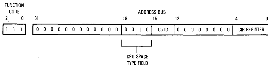
Figure 10-3. MC68030 CPU Space Address Encodings
