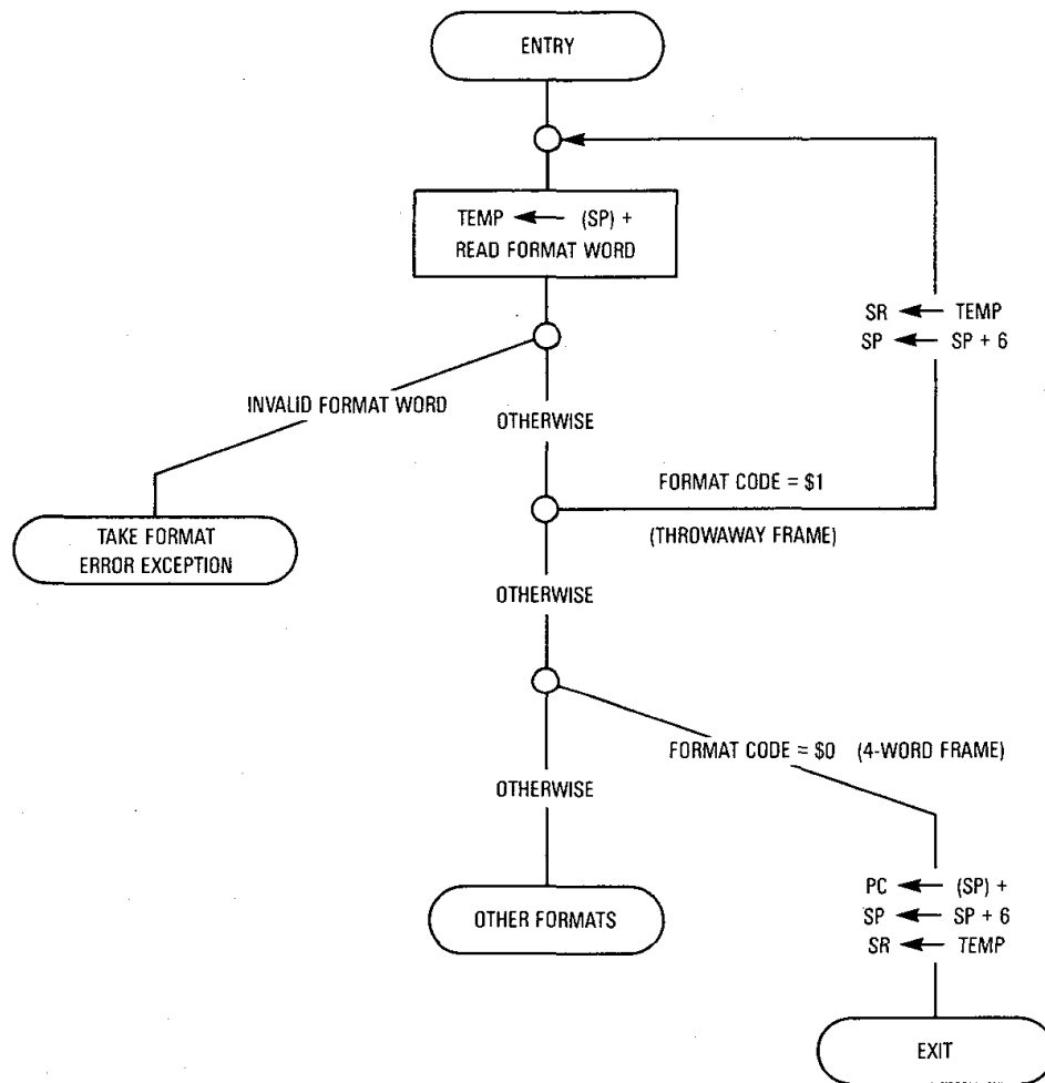
Figure 8-8. RTE Instruction for Throwing Four-Word Frame
