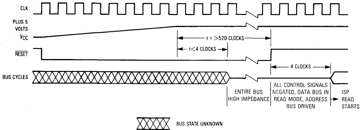
Figure 7-64. Initial Reset Operation Timing
