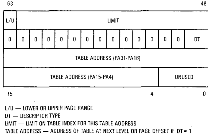
Figure 9-35. Root Pointer Register (CRP, SRP) Format
