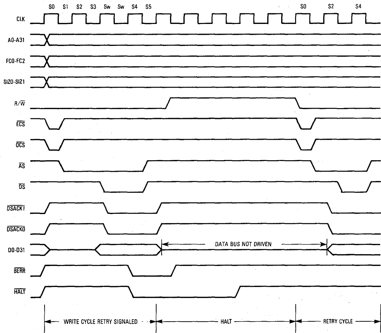
Figure 7-54. Asynchronous Late Retry
