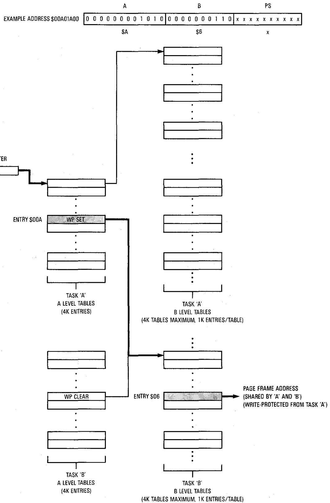
Figure 9-23. Example Translation Tree Using Shared Tables
