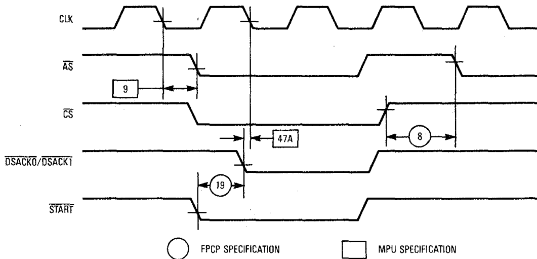
Figure 12-5. Bus Cycle Timing Diagram
