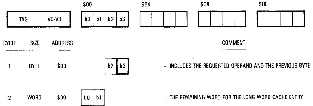
Figure 6-6. Single Entry Mode Operation — 16-Bit Port
