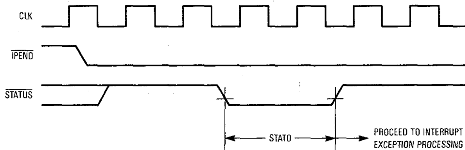
EXAMPLE 2: INTERRUPT EXCEPTION SIGNALLED DURING STAT0
