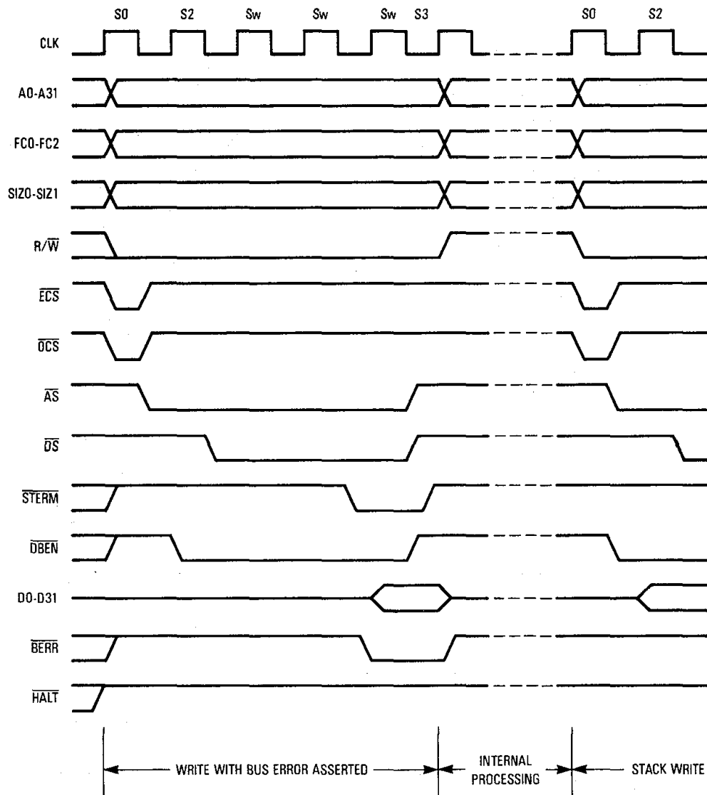
Figure 7-51. Late Bus Error with \overline{\text{STERM}} — Exception Taken
