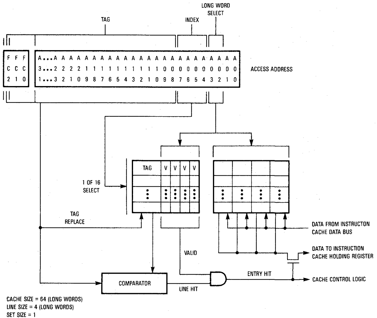
Figure 6-2. On-Chip Instruction Cache Organization
