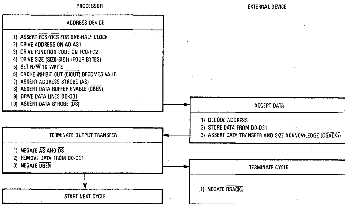
Figure 7-24. Asynchronous Write Cycle Flowchart
