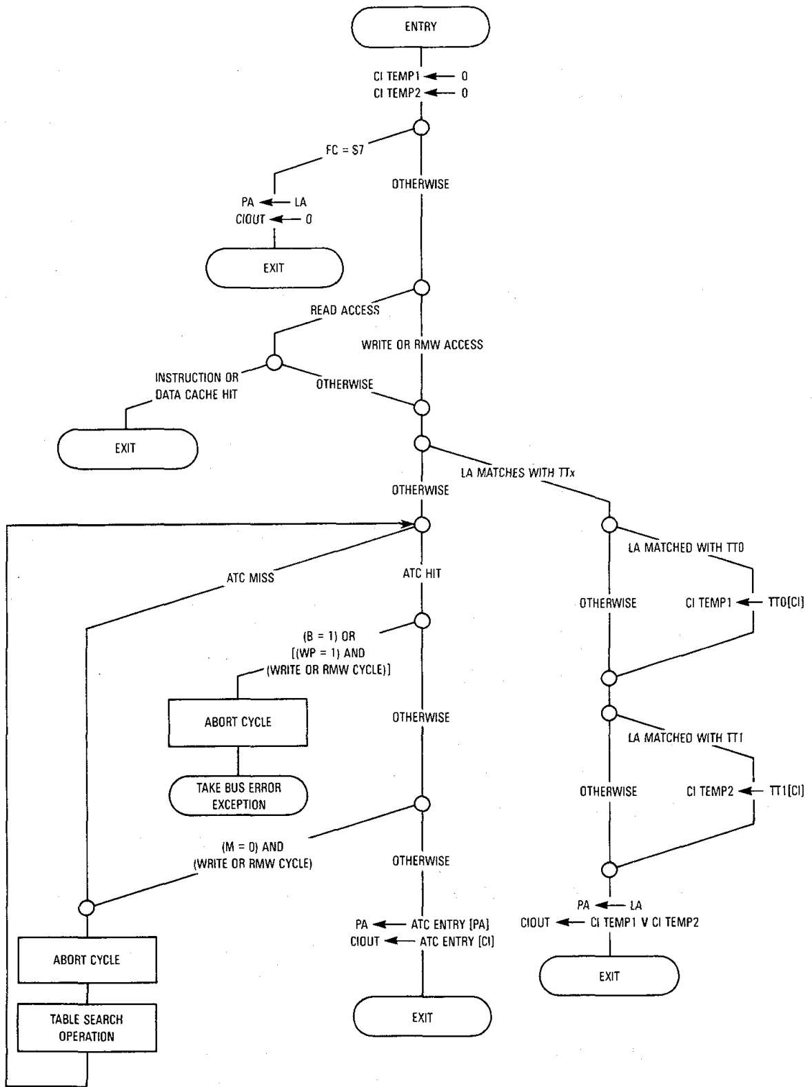
Figure 9-8. Address Translation General Flowchart
