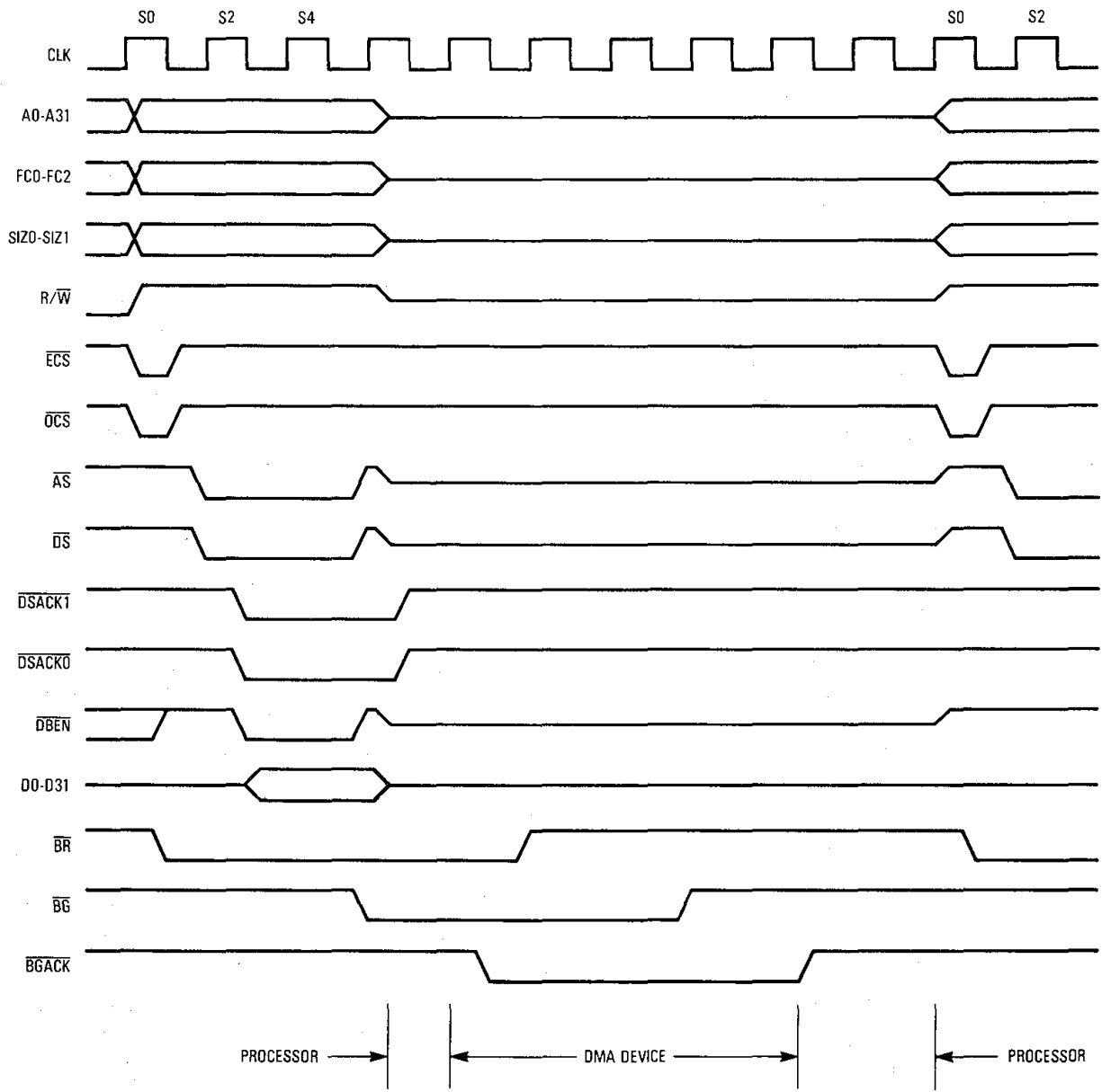
Figure 7-60. Bus Arbitration Operation Timing
