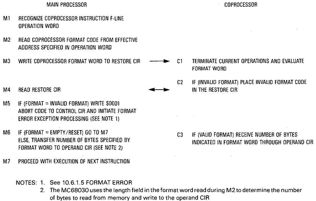
Figure 10-18. Coprocessor Context Restore Instruction Protocol
