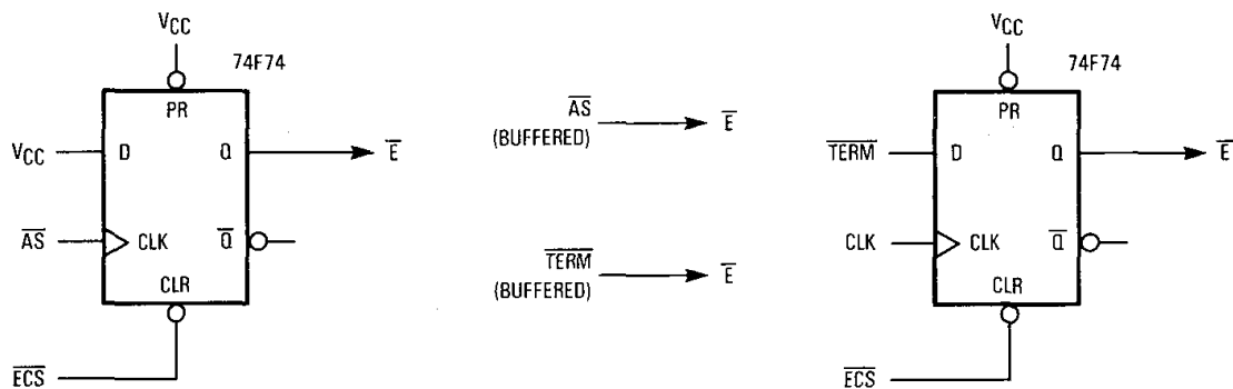
Figure 12-16. Additional Memory Enable Circuits
