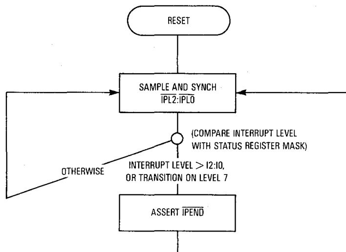
Figure 8-2. Interrupt Pending Procedure
