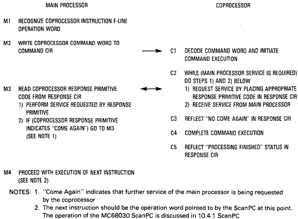
Figure 10-7. Coprocessor Interface Protocol for General Category Instructions
