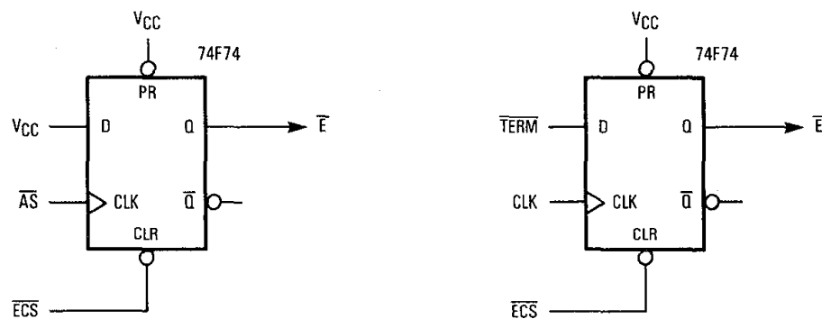
Figure 12-11. Additional Memory Enable Circuits
