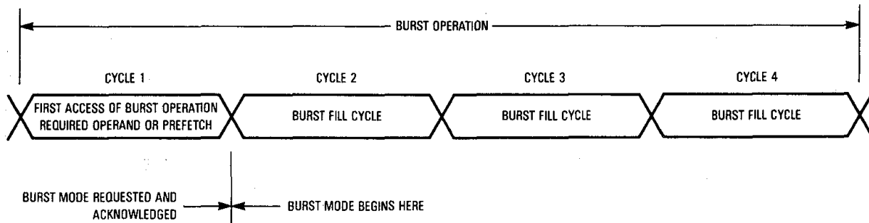
Figure 6-11. Burst Operation Cycles and Burst Mode
