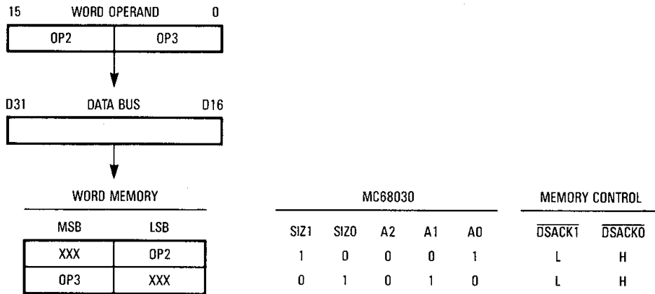
Figure 7-12. Misaligned Word Transfer to Word Port Example
