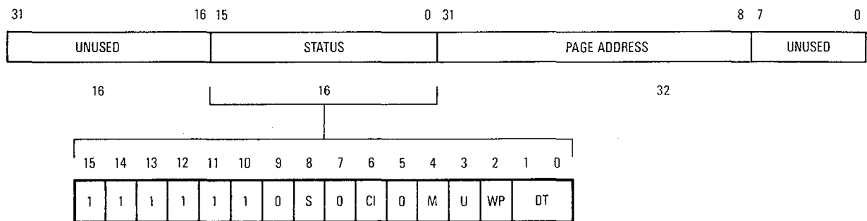
Figure 9-14. Long-Format Page Descriptor
