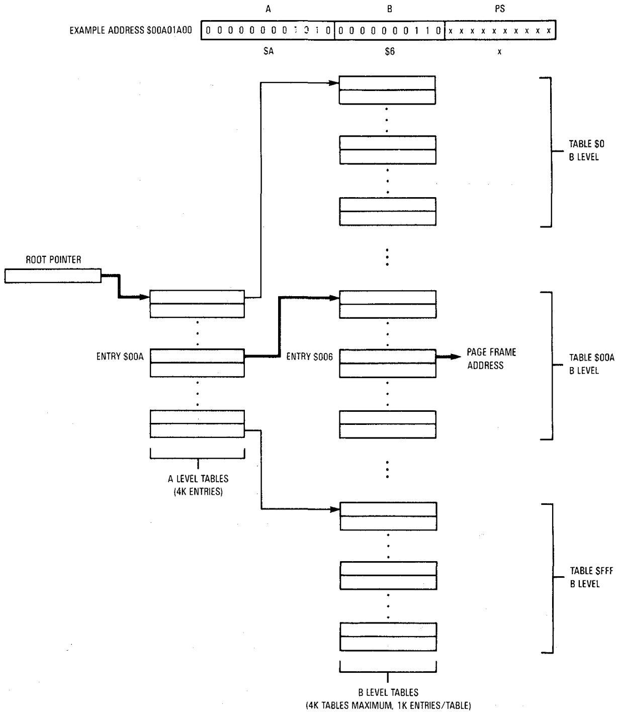
Figure 9-4. Example Translation Table Tree
