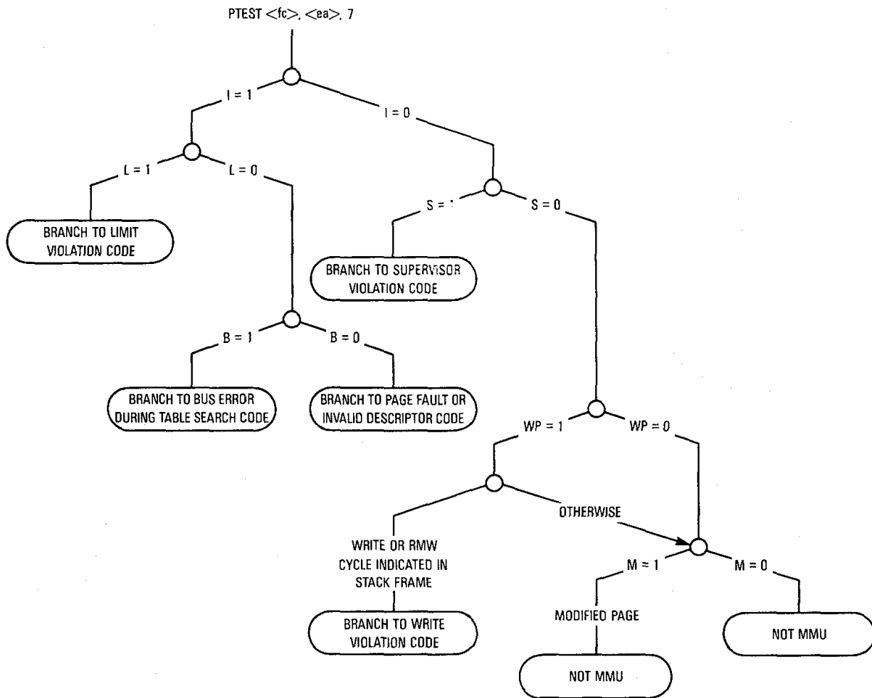
Figure 9-40. MMU Status Interpretation PTEST Level 7
