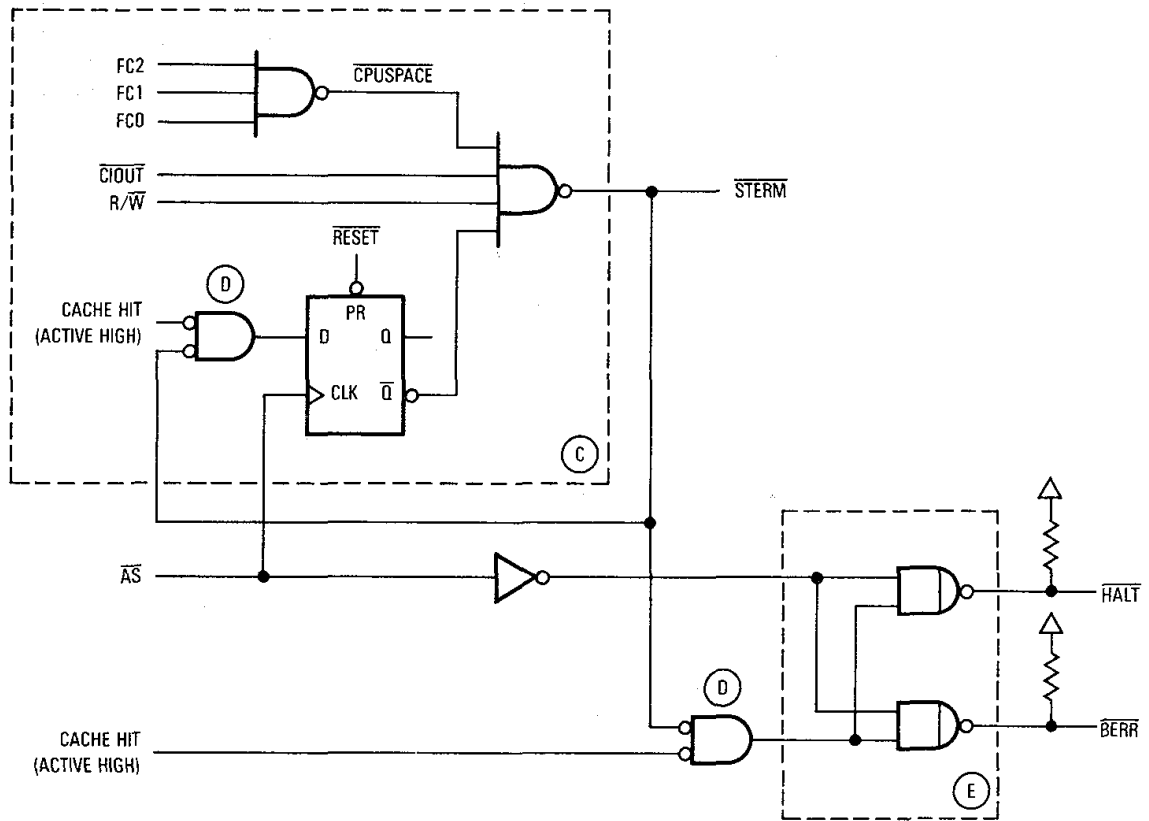
Figure 12-18. Example Early Termination Control Circuit
