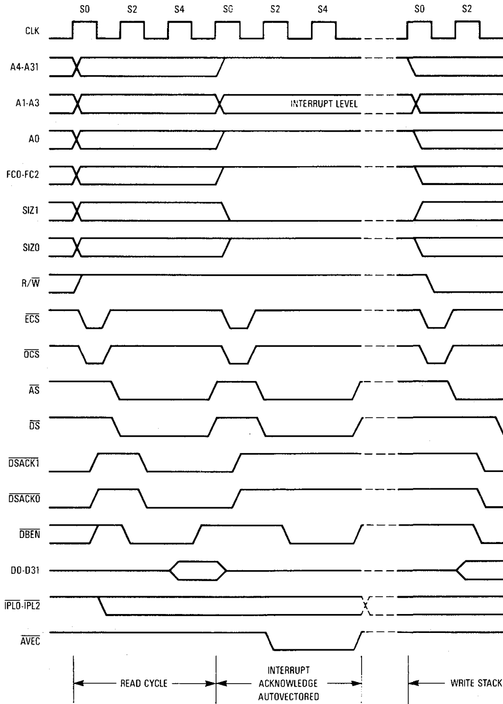
Figure 7-45. Autovector Operation Timing
