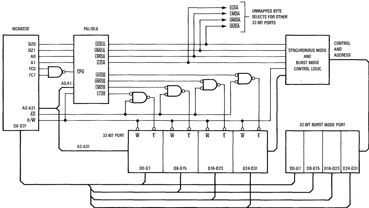
Figure 12-6. Example MC68030 Byte Select PAL System Configuration
