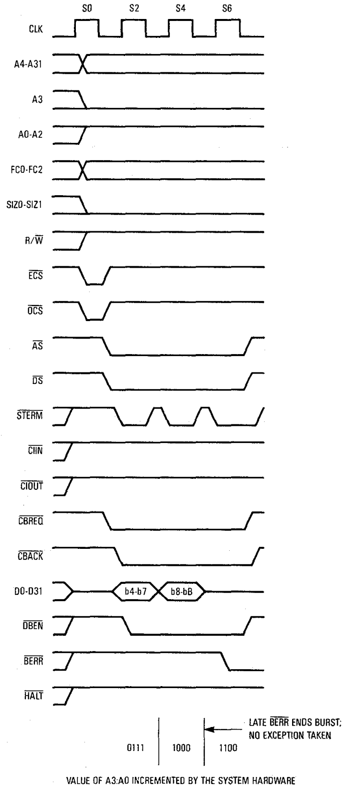
Figure 7-52. Long-Word Operand Request — Late \bar{BERR} on Third Access
