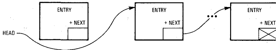
Figure 3-3. Linked List Deletion
