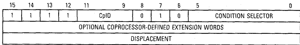
Figure 10-9. Branch on Coprocessor Condition Instruction (cpBcc.W)
