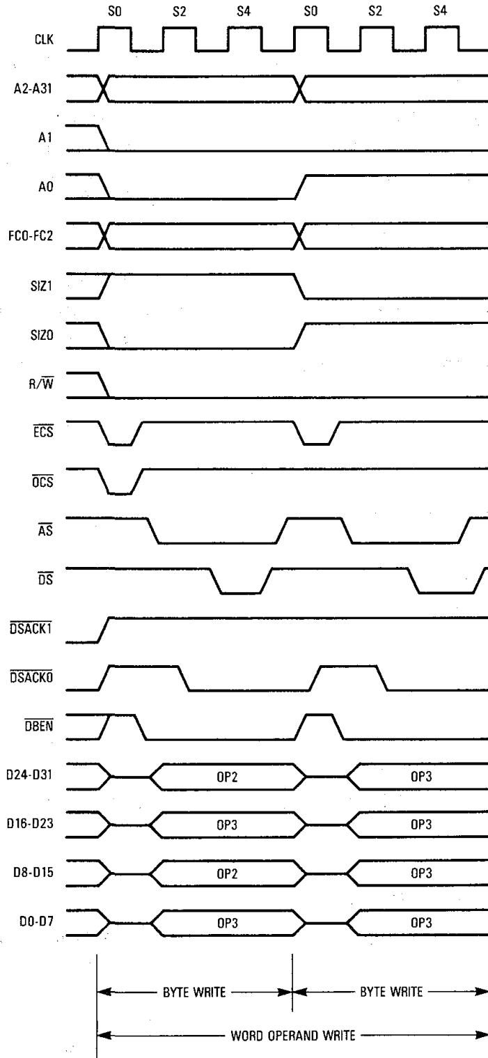
Figure 7-8. Word Operand Write Timing (8-Bit Data Port)
