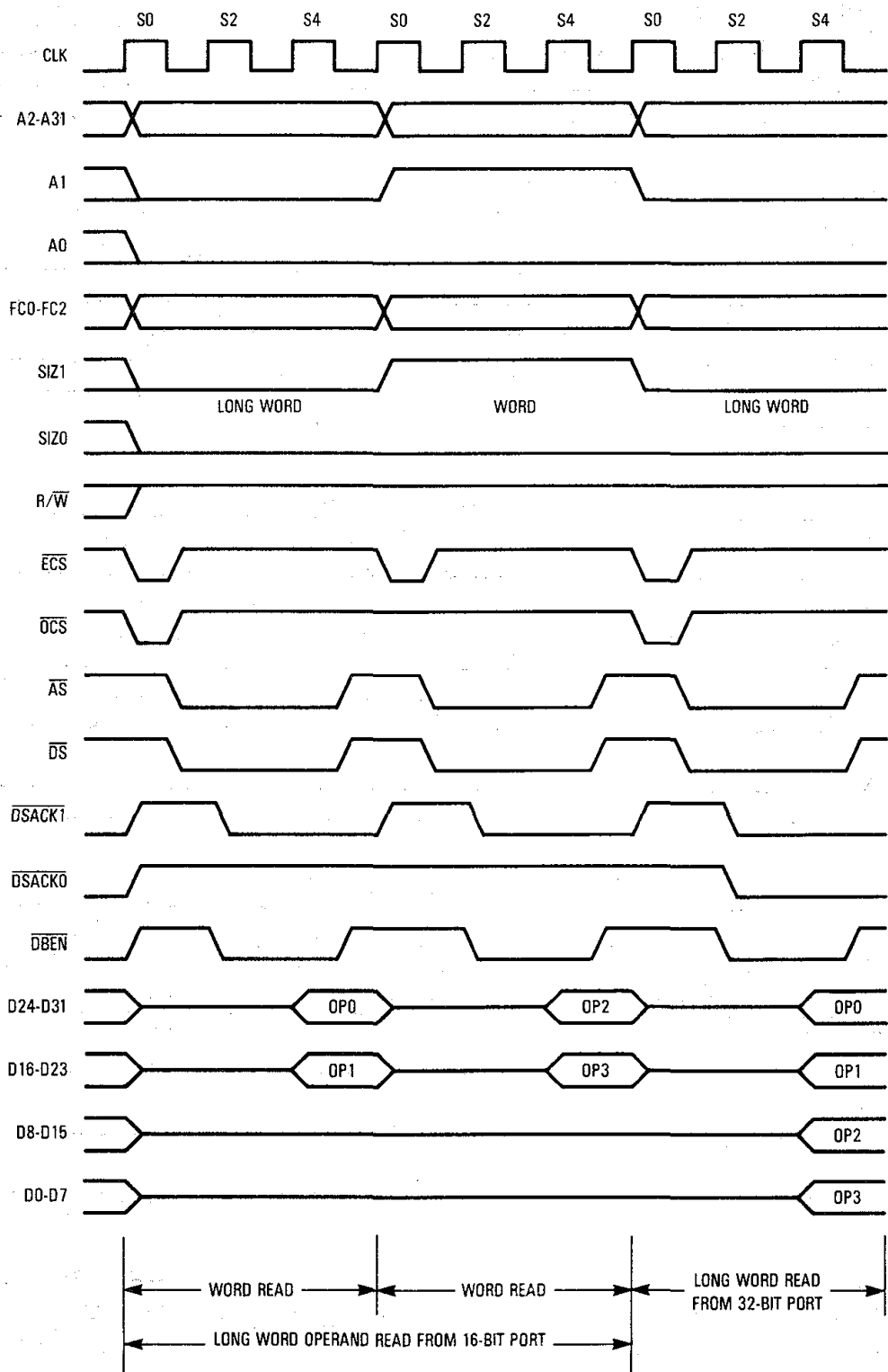
Figure 7-23. Long-Word Read — 16-Bit and 32-Bit Port
