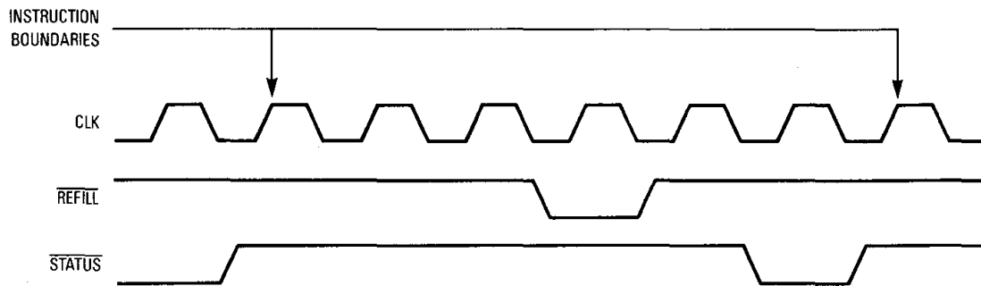
Figure 12-19. Normal Instruction Boundaries
