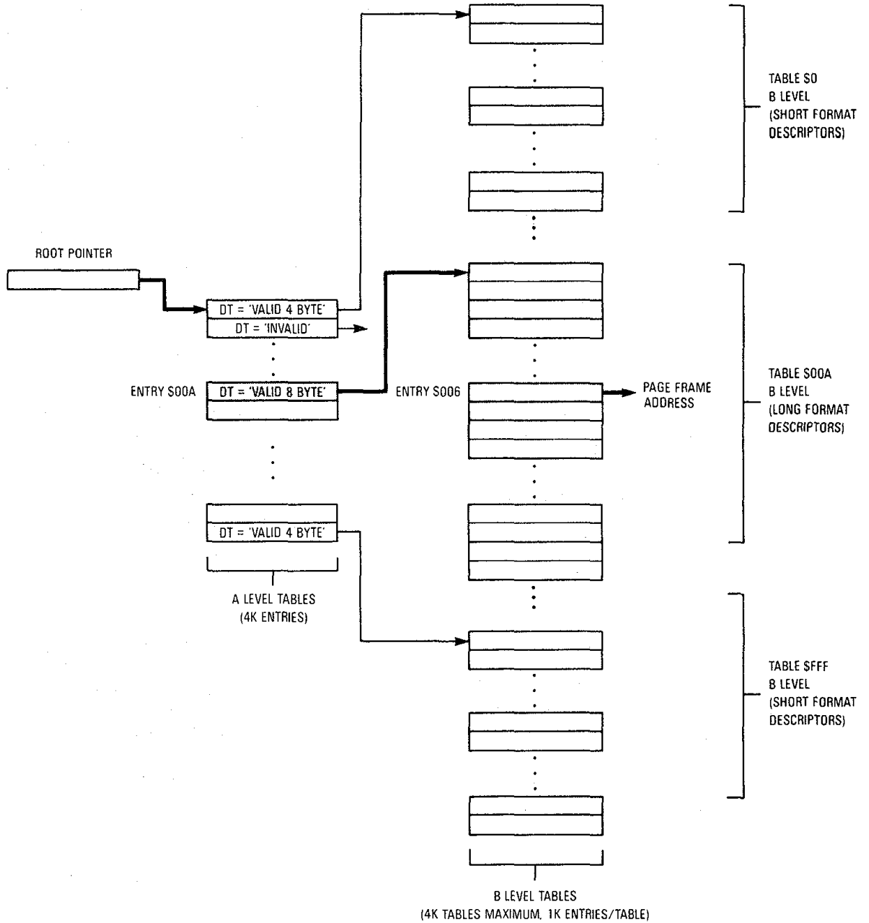
Figure 9-7. Example Translation Tree Using Different Format Descriptors
