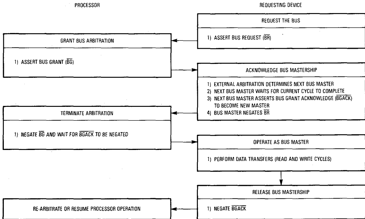
Figure 7-59. Bus Arbitration Flowchart for Single Request
