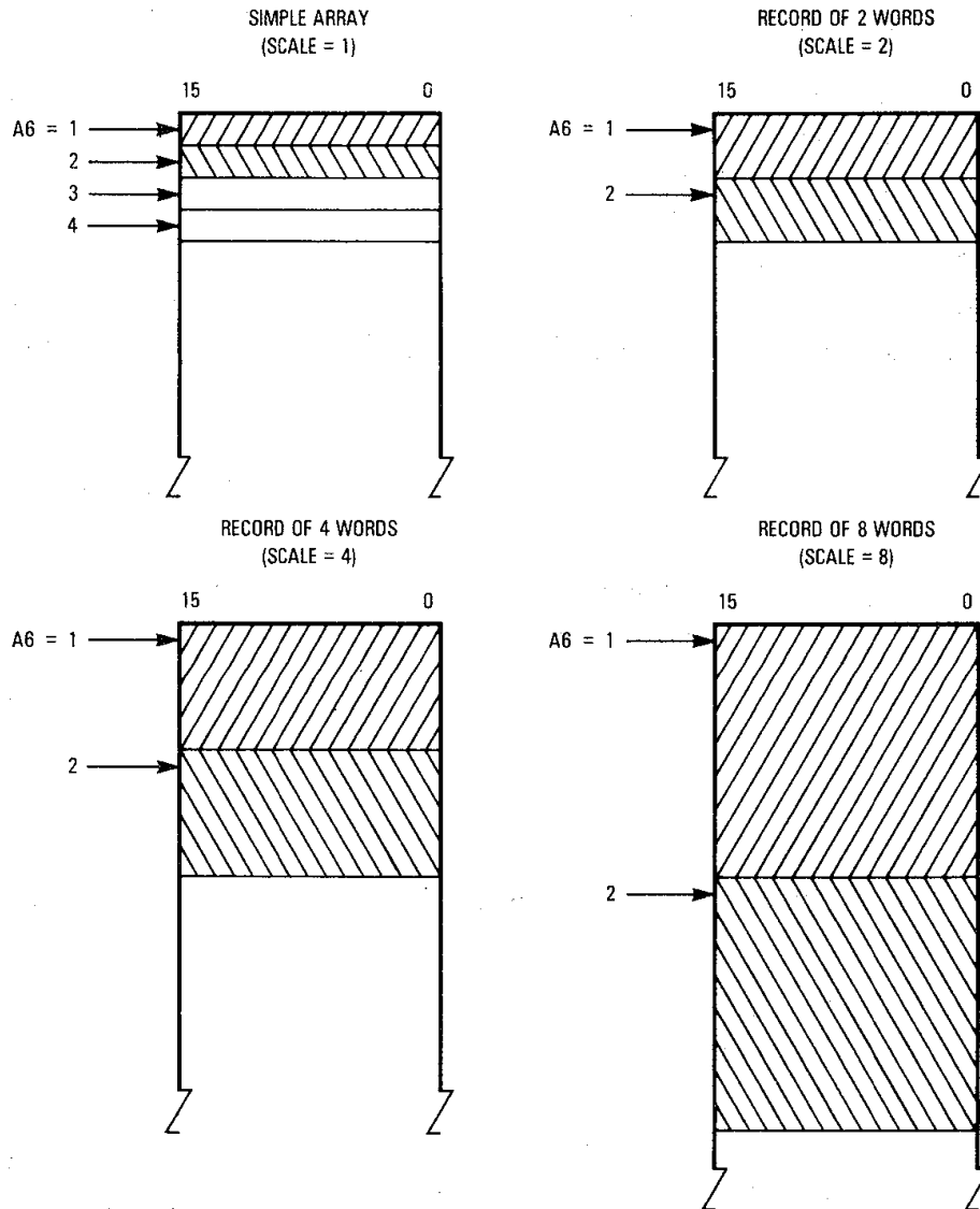
Figure 2-7. Addressing Array Items
