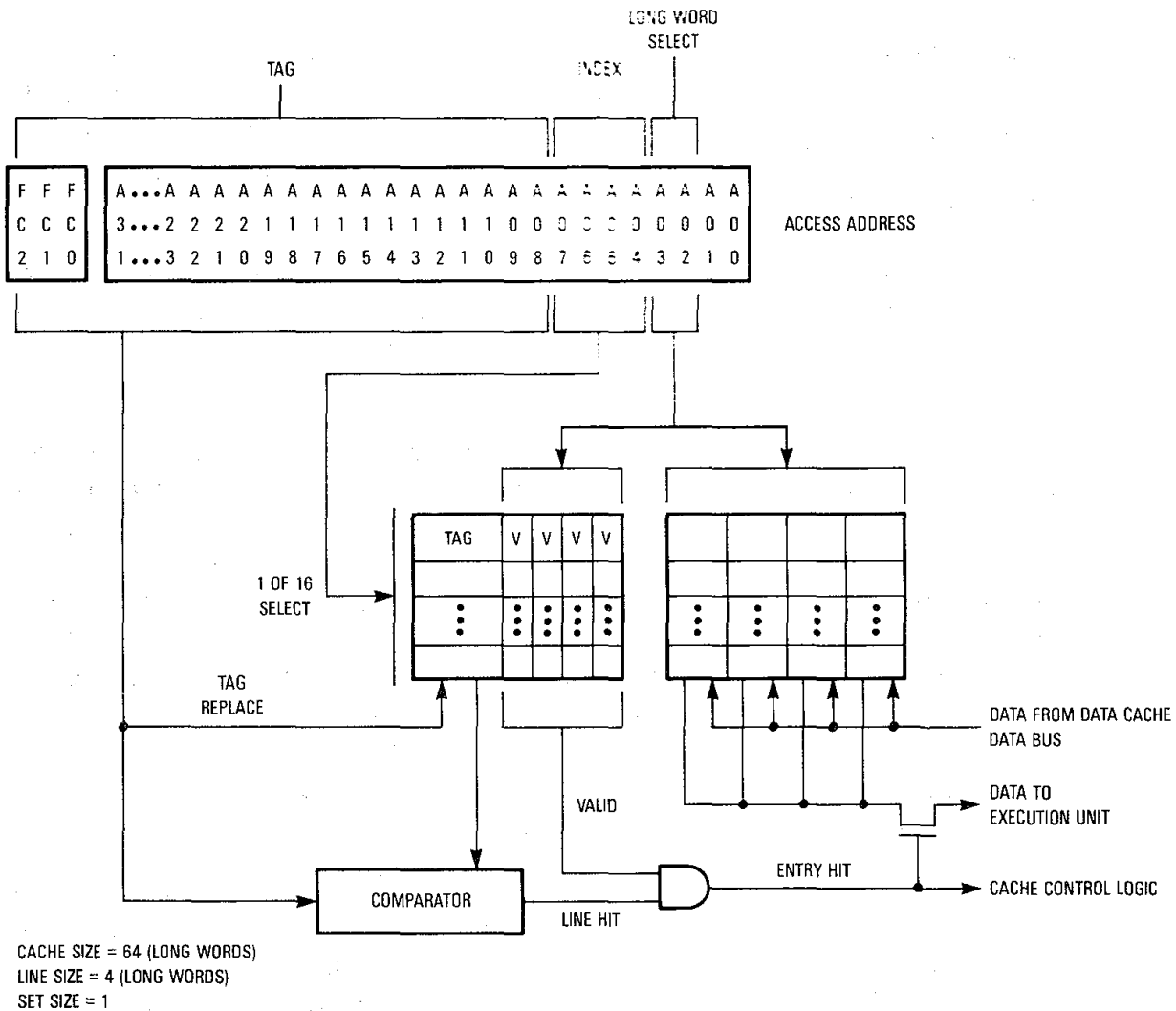
Figure 6-3. On-Chip Data Cache Organization
