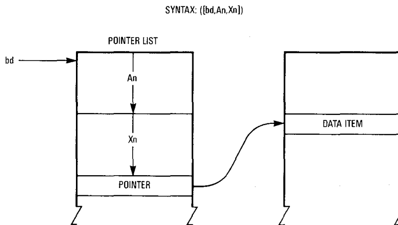
Figure 2-11. Preindexed Indirect Addressing
