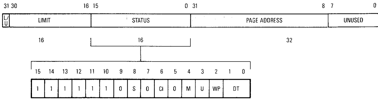
Figure 9-13. Long-Format Early Termination Page Descriptor
