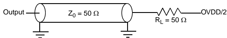
Figure 45. SPI AC Test Load
