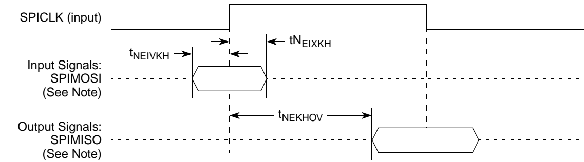
Figure 46. SPI AC Timing in Slave Mode (External Clock) Diagram
