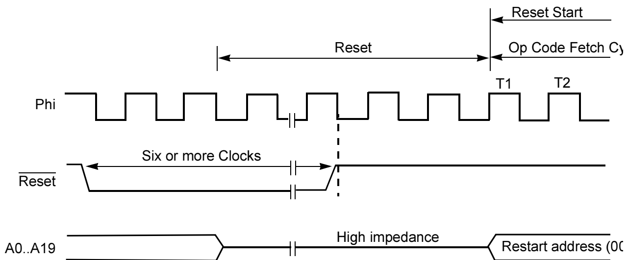
Figure 8. Reset Timing
