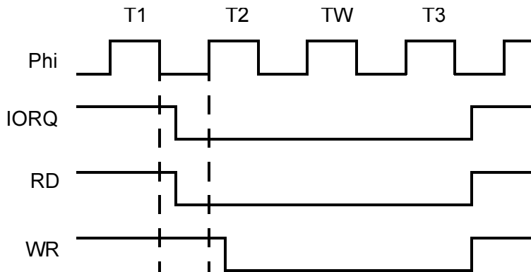
Figure 14. I/O Read and Write Cycles with \overline{IOCS} Set to 1
