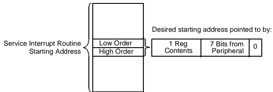
Figure 8. Mode 2 Interrupt Operation
