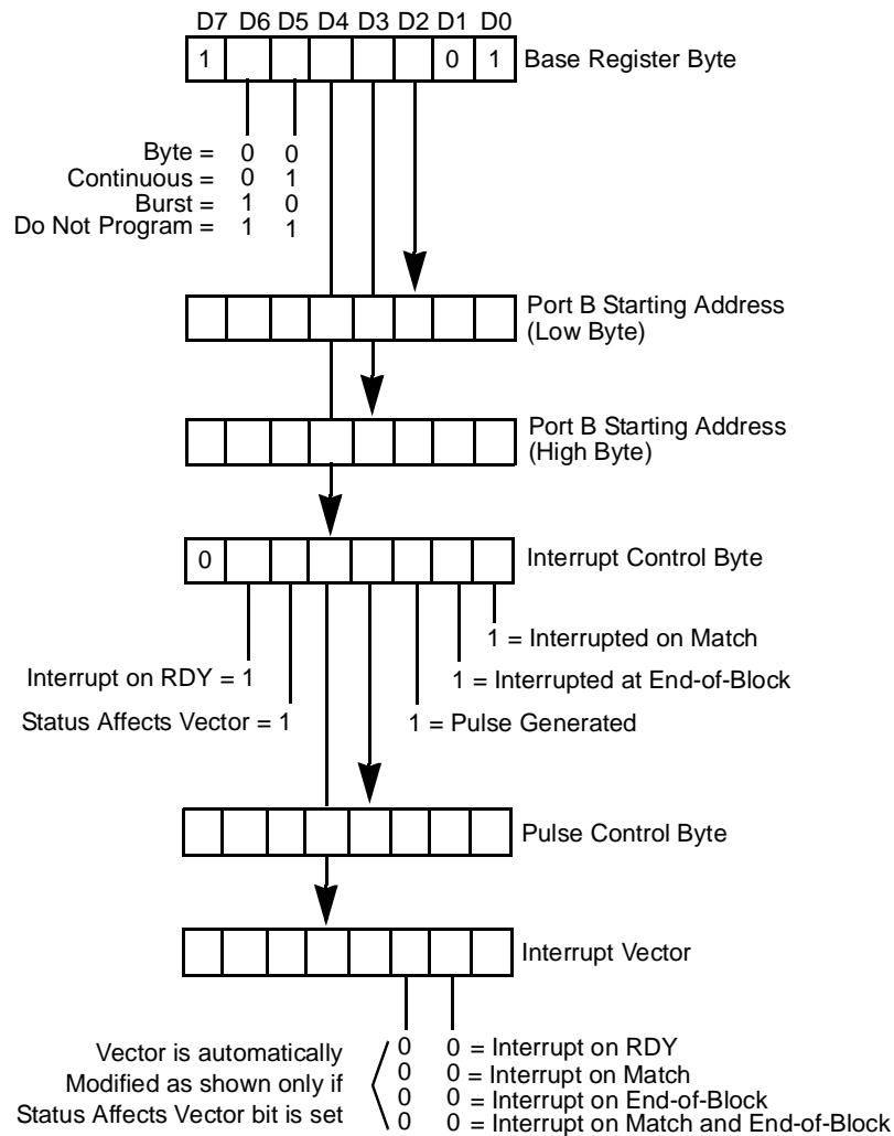
Figure 44. Write Register 4 Group
