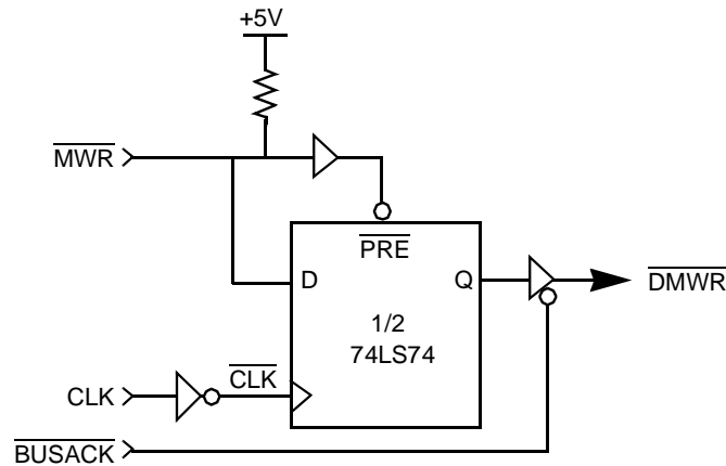
Figure 53. Delaying the Leading Edge of \overline{\text{MWR}}
