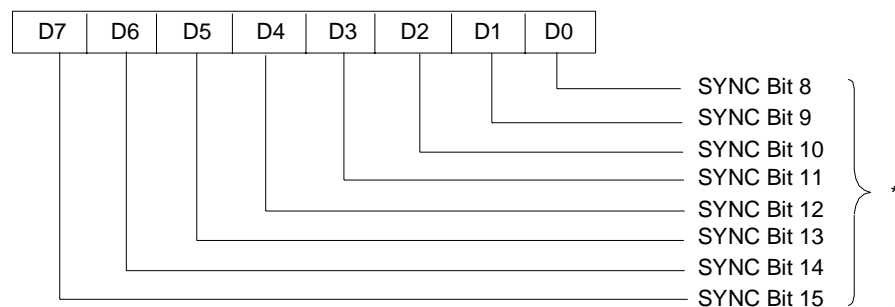
Figure 121. Write Register 7
