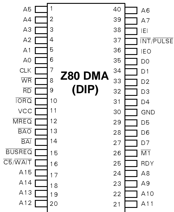
Figure 26. 40-Pin DIP Pin Assignments
