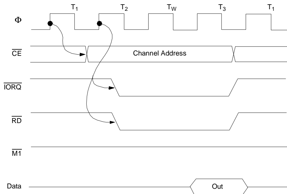
Figure 128. Read Cycle Timing
