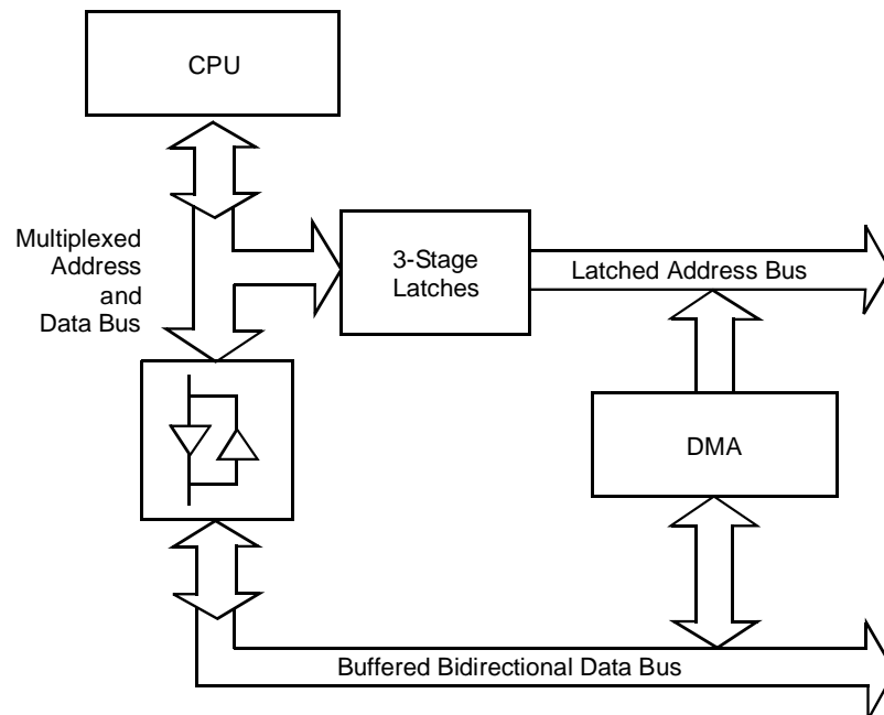
Figure 56. Connecting DMA to Demultiplexed Address/Data Buses
