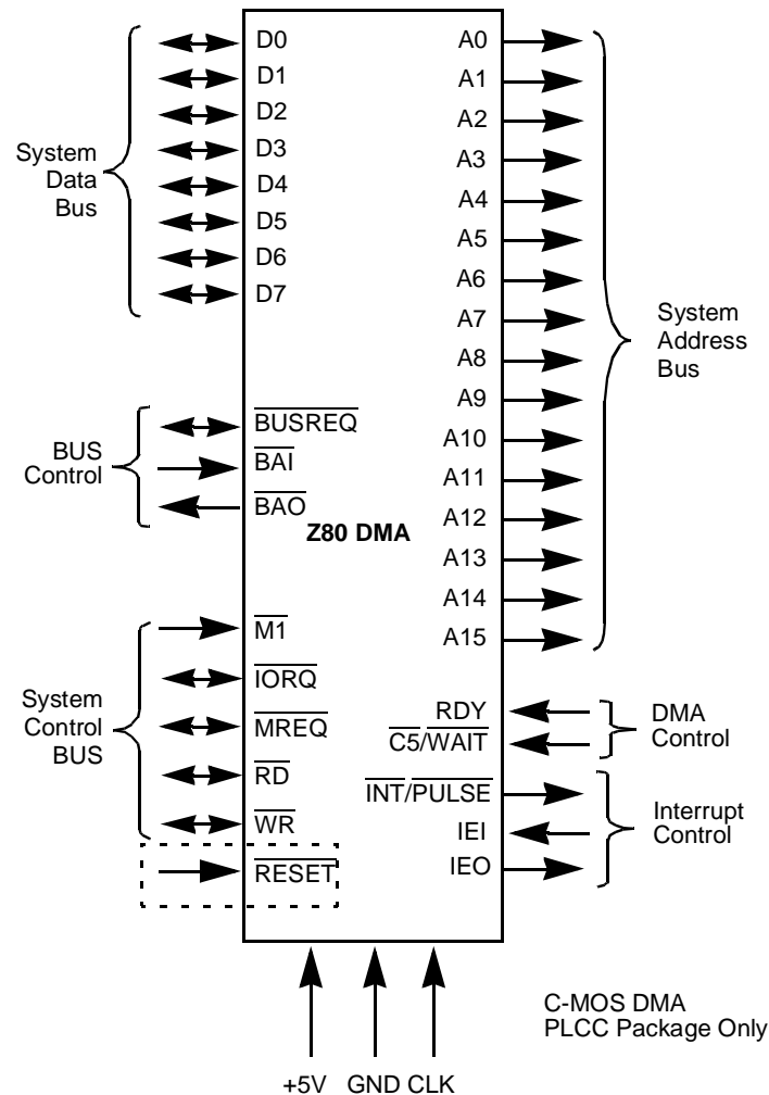
Figure 25. Pin Functions (CMOS PLCC Package Only)
