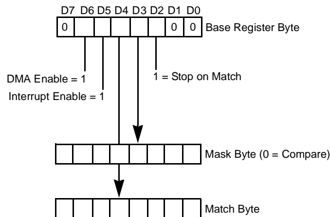
Figure 43. Write Register 3 Group
