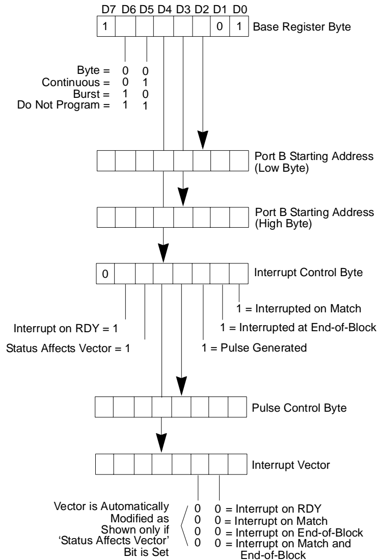
Figure 80. Write Register 4 Group
