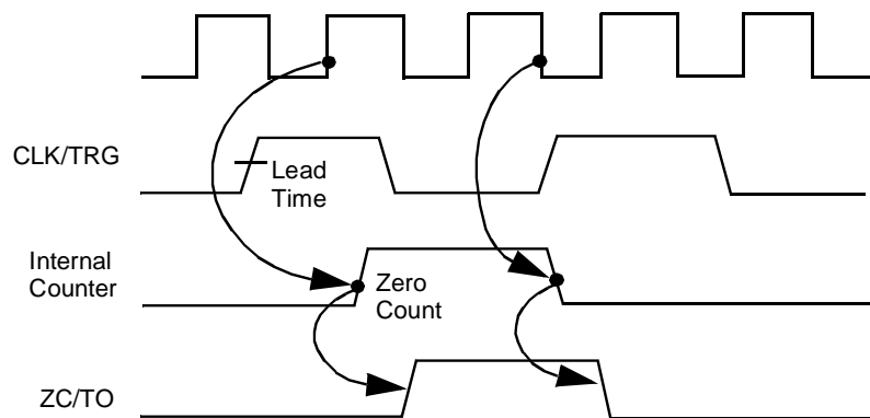
Figure 11. CTC Counting and Timing
