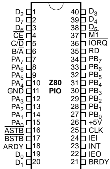
Figure 6. 40-Pin DIP Pin Assignments
