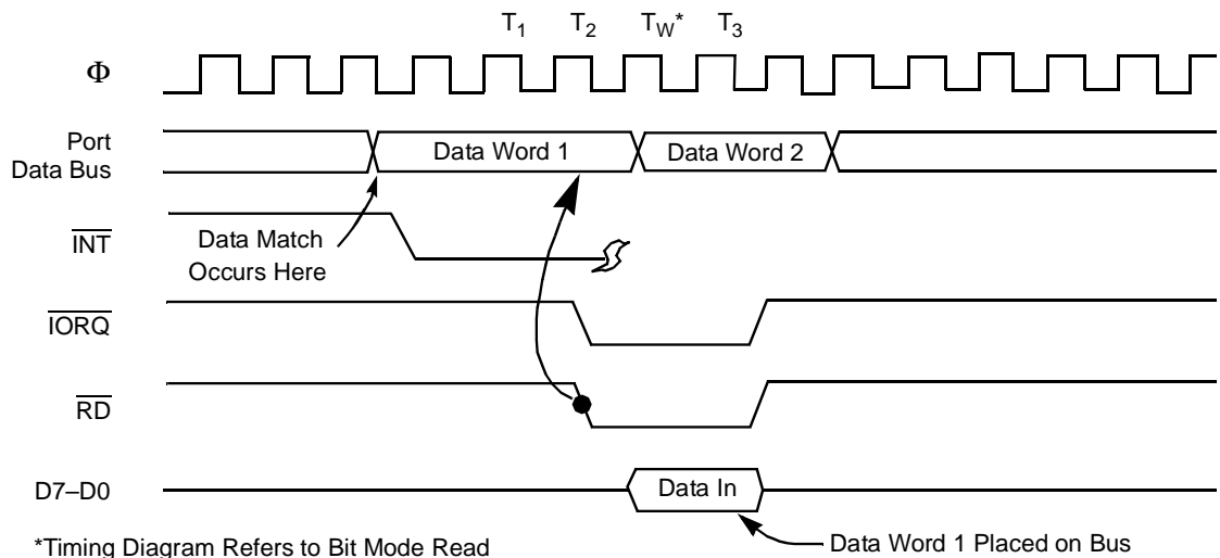
Figure 10. Control Mode (Mode 3) Timing
