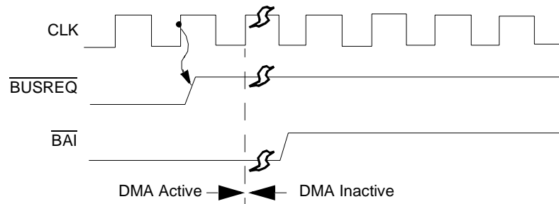
Figure 66. Bus Release in Byte Mode
