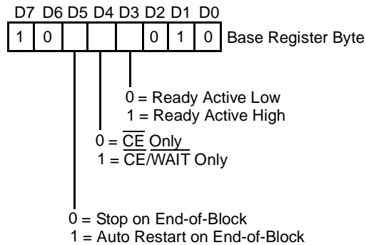
Figure 45. Write Register 5 Group
