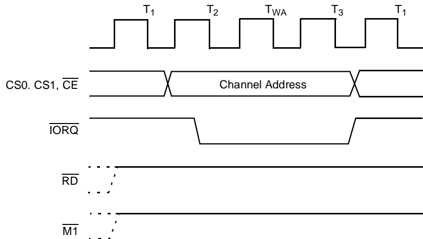
Figure 9. CTC Write Cycle
