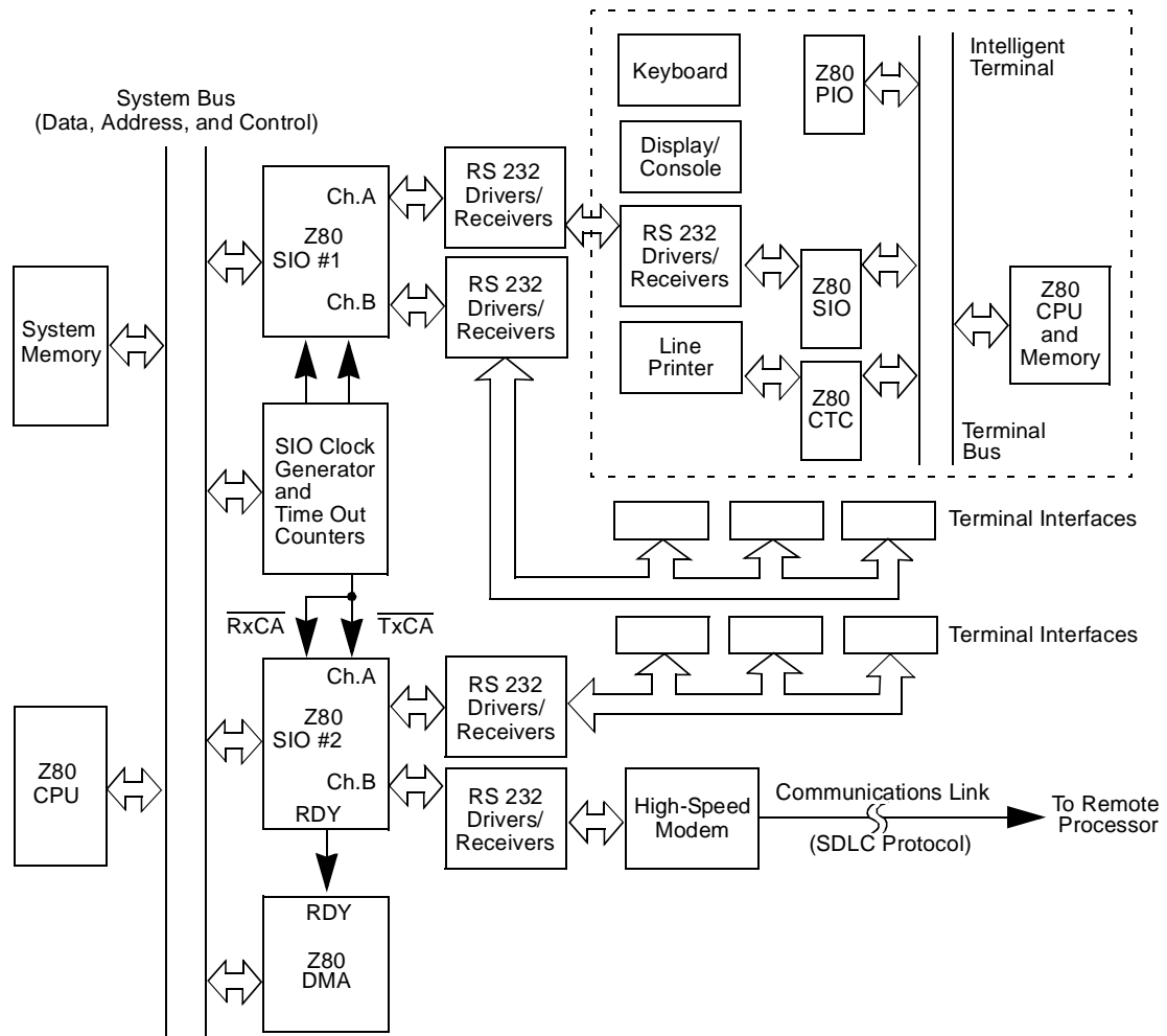
Figure 127. Data Concentrator
