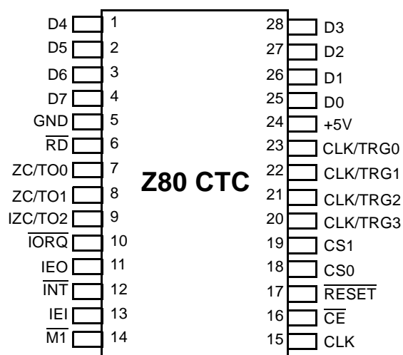
Figure 5. Package Configuration
