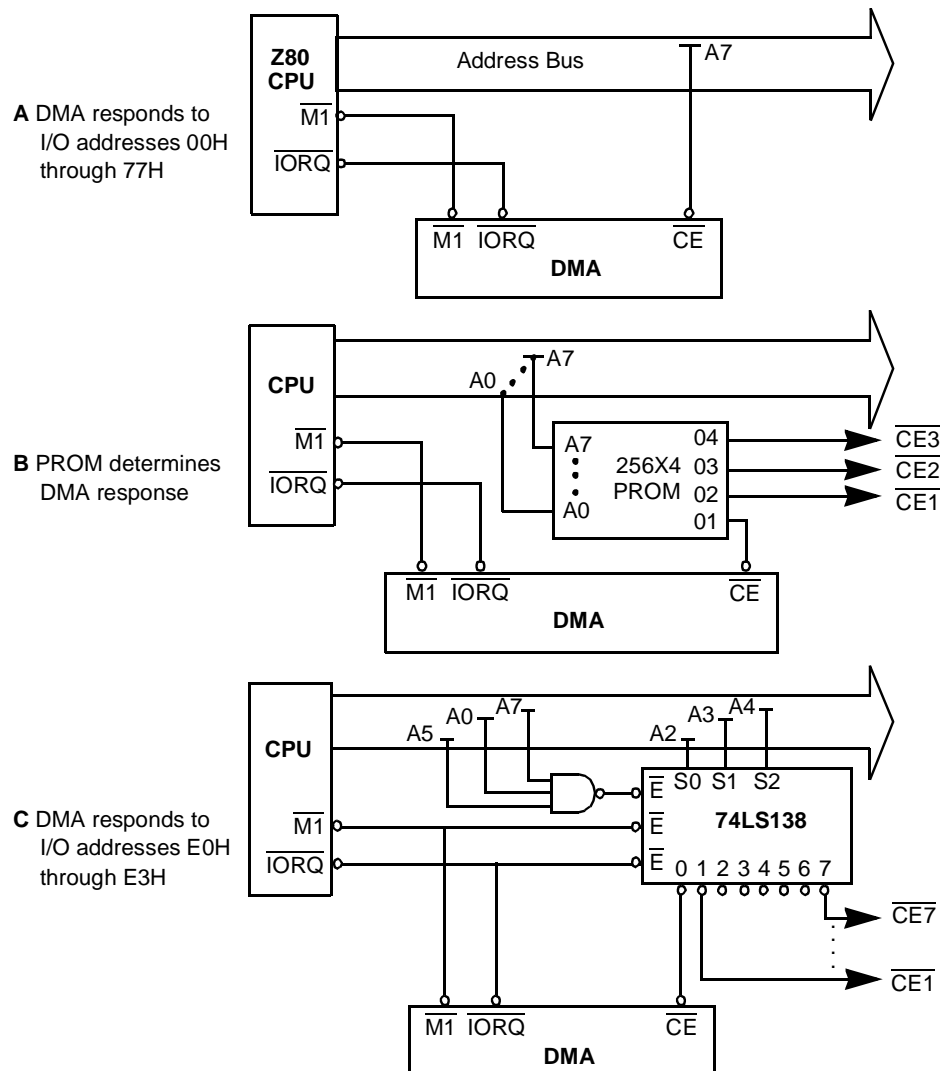
Figure 49. Chip Enable Decoding with Z80 CPU
