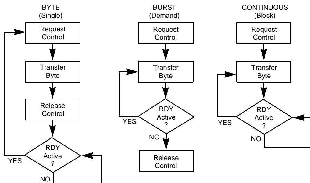
Figure 17. Modes of Operation
