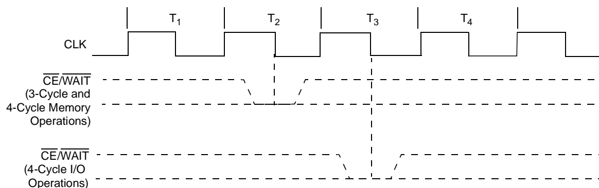
Figure 74. \overline{\text{WAIT}} Line Sampling in Variable-Cycle Timing
