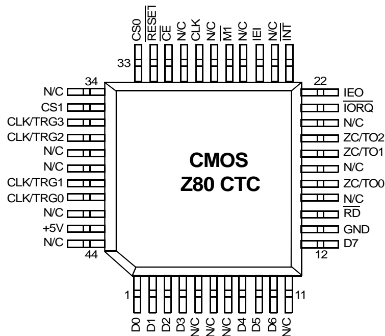
Figure 7. 44-Pin Quad Flat Pack Pin Assignments
