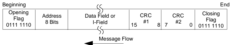
Figure 113. Transmit/Receive SDLC/HDLC Message Format
