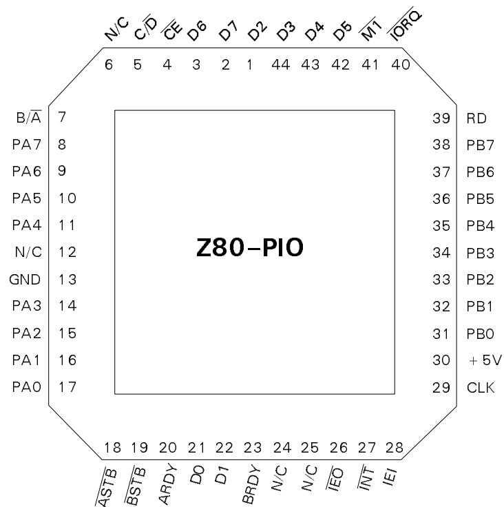
Figure 4. 44-Pin PLCC Pin Assignments
