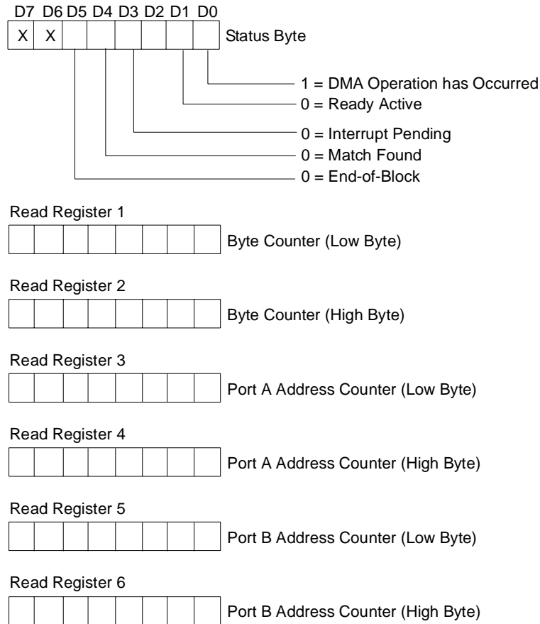
Figure 83. Read Register 0 through 6 Bit Functions
