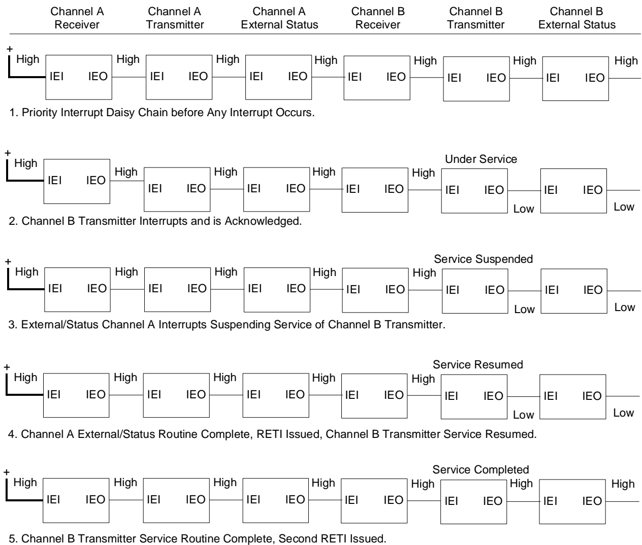
Figure 132. Typical Interrupt Service
