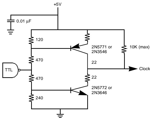
Figure 48. Z80/Z8000 Clock Driver
