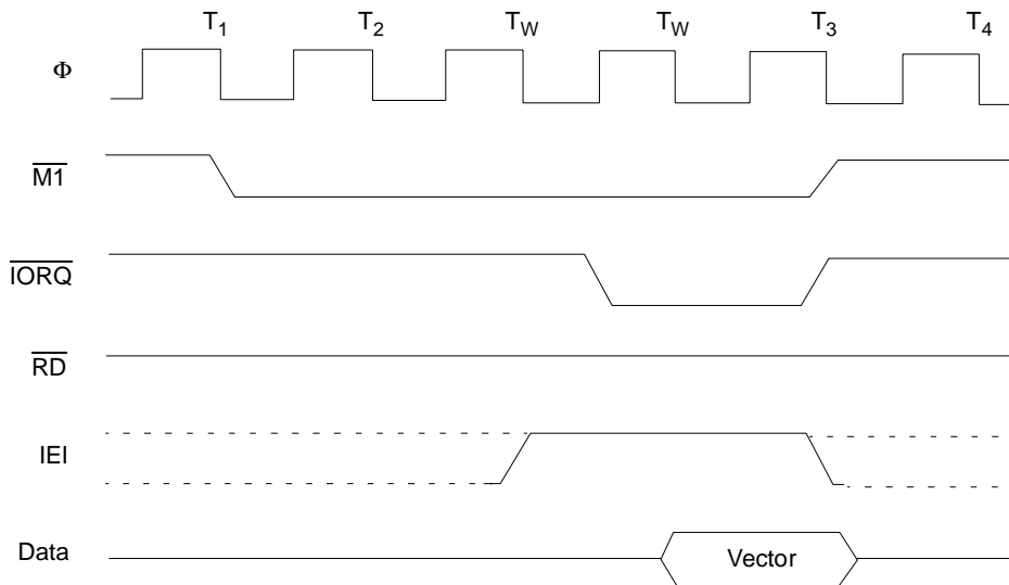
Figure 130. Interrupt Acknowledge Cycle Timing
