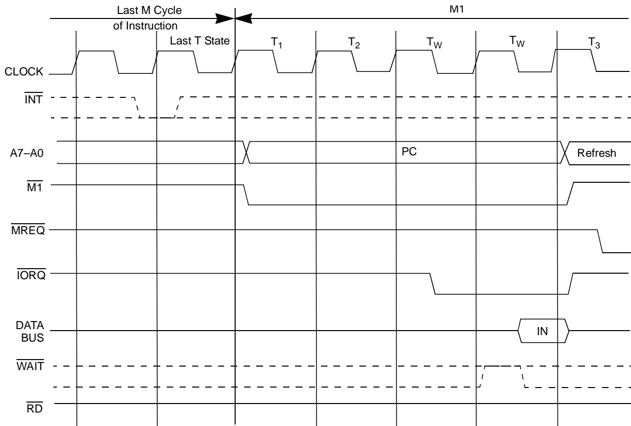
Figure 75. Interrupt Acknowledge
