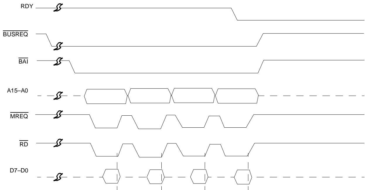
Figure 71. RDY Line in Burst Mode
