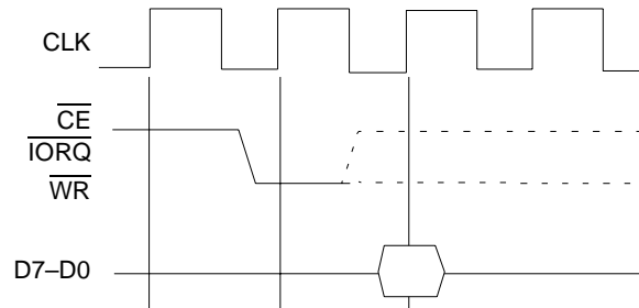
Figure 59. CPU-to-DMA Write Cycle Requirements
