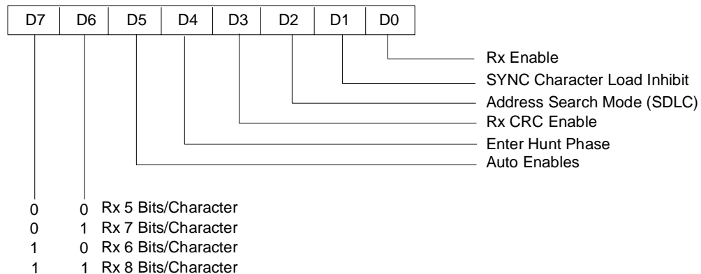
Figure 117. Write Register 3
