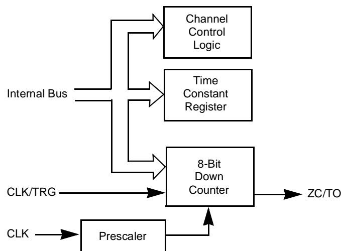
Figure 2. Channel Block Diagram
