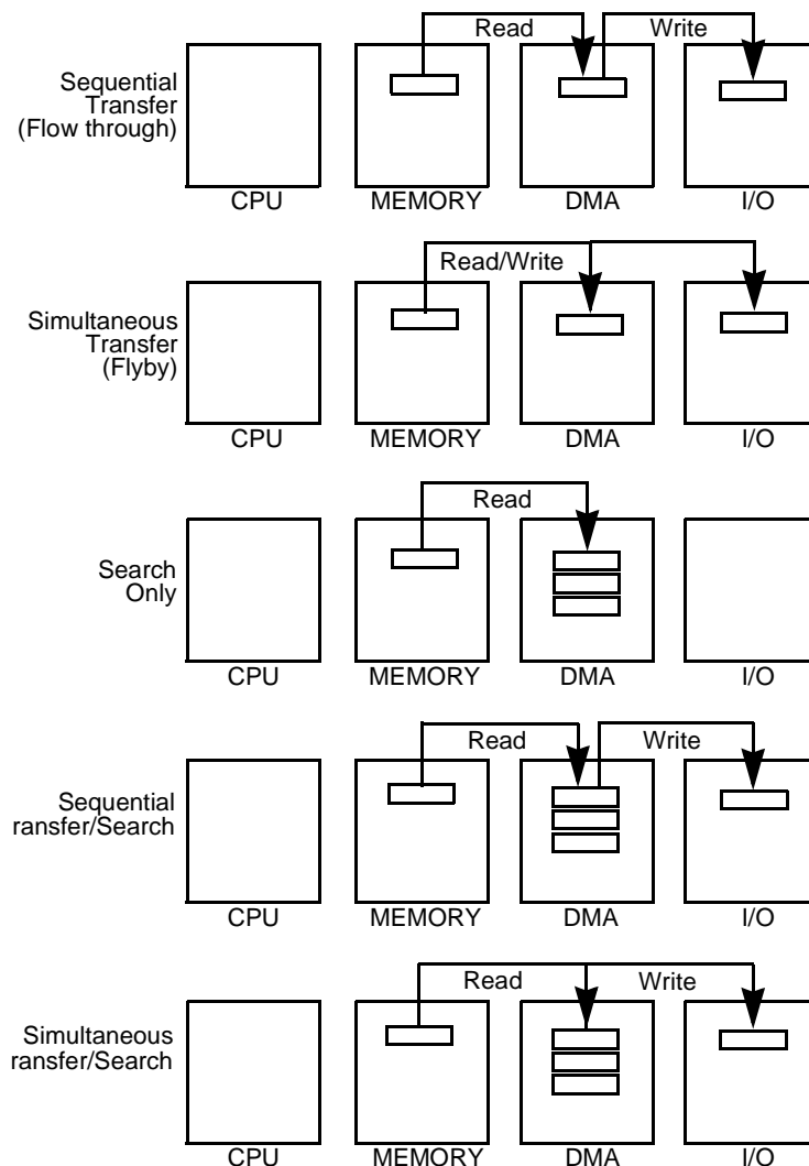
Figure 18. Class of Operation
