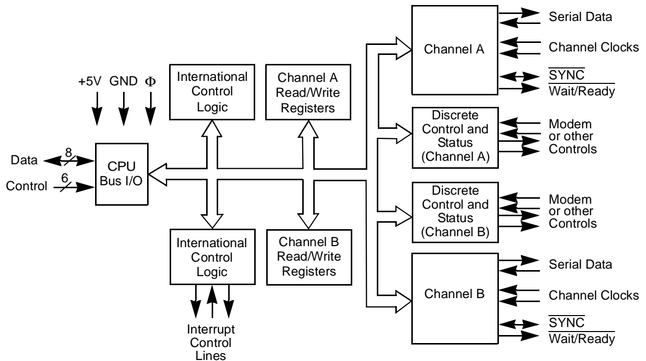
Figure 100. Z80 SIO Block Diagram
