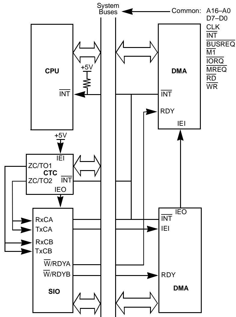
Figure 55. DMA-SIO Environment
