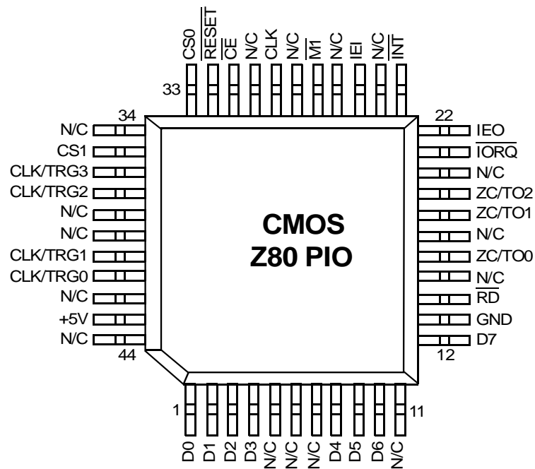
Figure 5. 44-Pin QFP Pin Assignments
