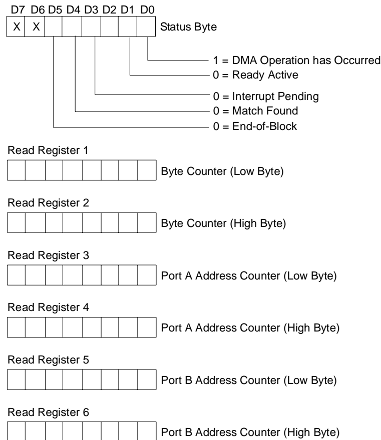
Figure 47. Read Register 0 through Read Register 6
