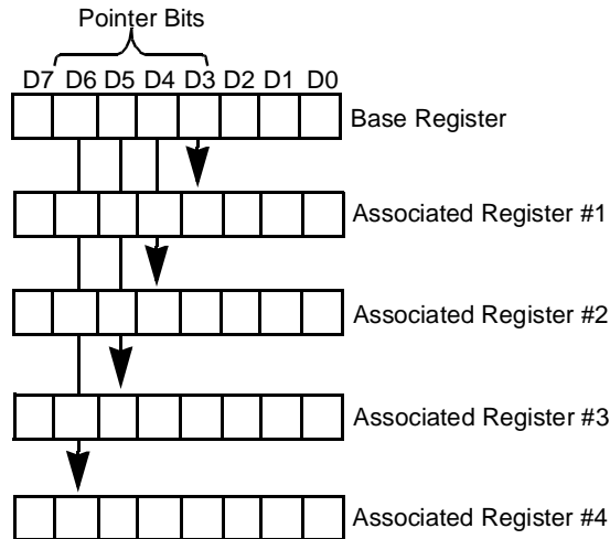
Figure 39. Write-Register Pointing Methods
