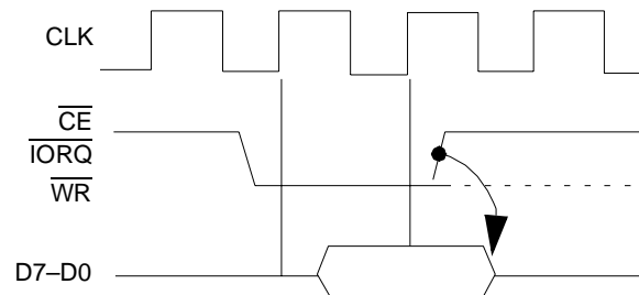
Figure 60. CPU-to-DMA Read Cycle Requirements
