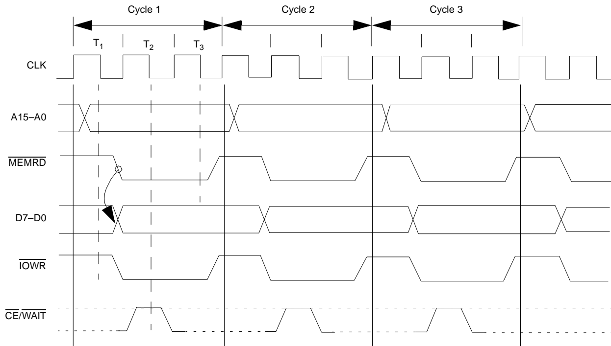
Figure 63. Simultaneous Memory-to-I/O Transfer (Burst and Continuous Mode)
