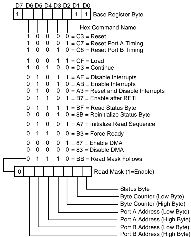
Figure 46. Write Register 6 Group
