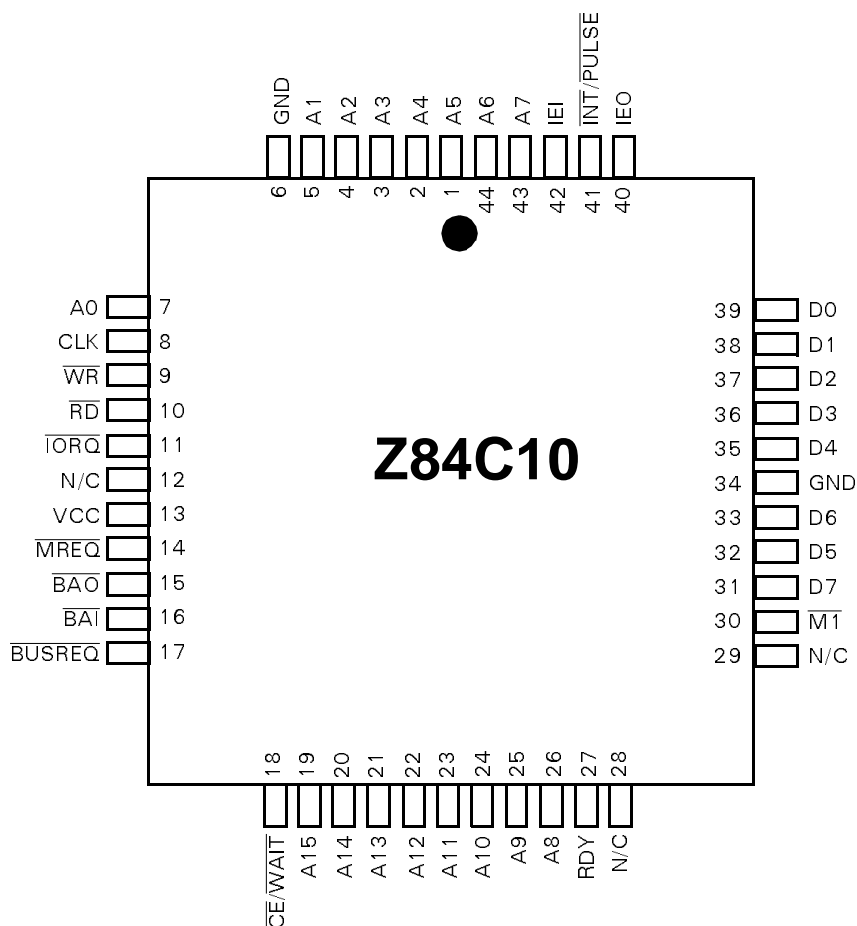
Figure 28. 44-Pin PLCC Pin Assignments (Z84C10 NMOS)
