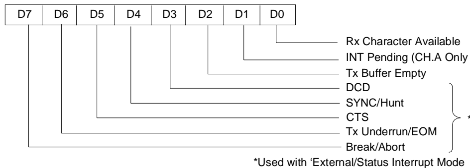
Figure 122. Read Register 0
