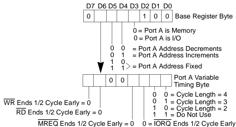
Figure 77. Write Register 1 Group
