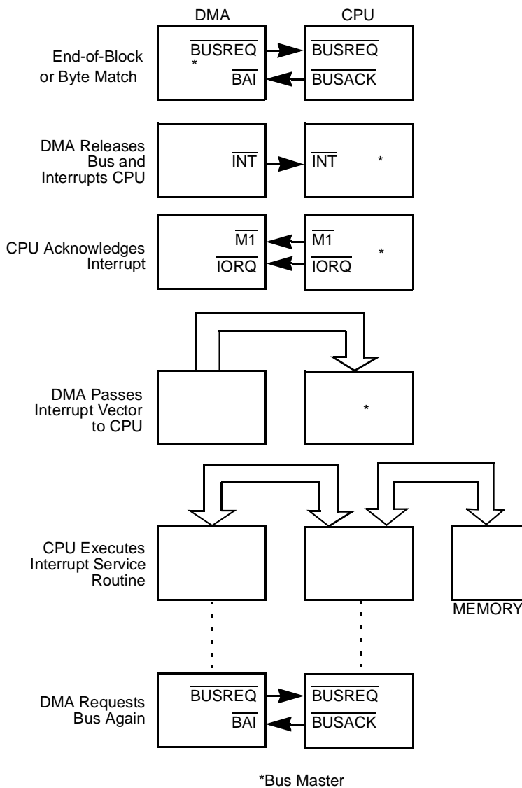
Figure 32. Z80 Interrupt Sequence
