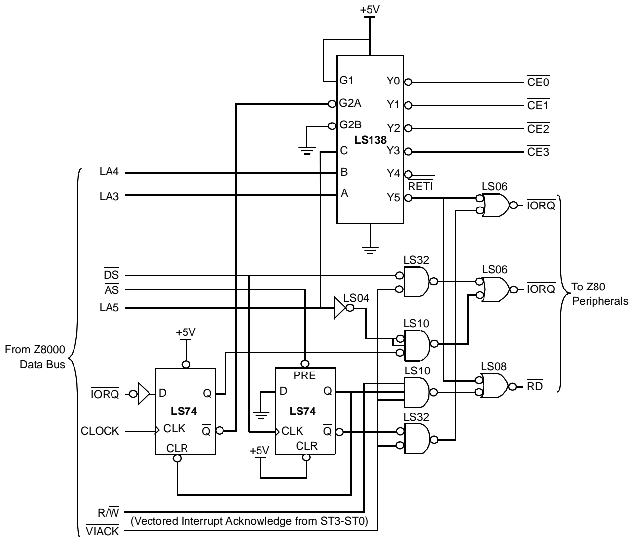
Figure 57. Z8000/Z80 Peripheral Interface
