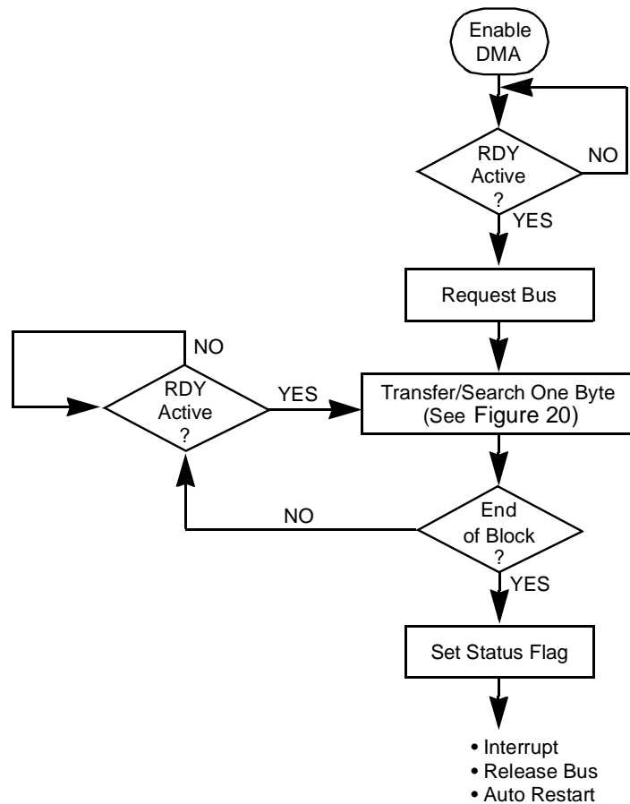
Figure 23. Continuous Mode
