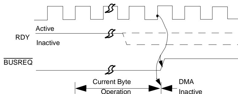
Figure 67. Bus Release on End-of-Block (Burst and Continuous Modes)
