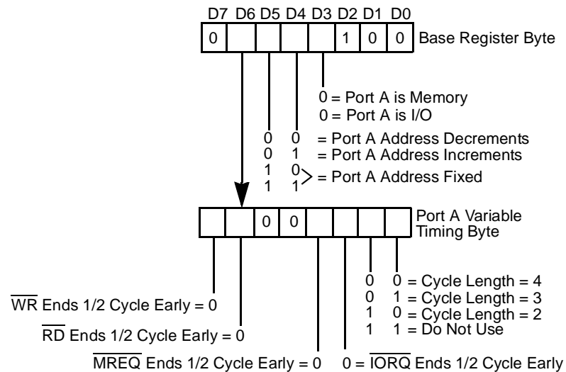
Figure 41. Write Register 1 Group
