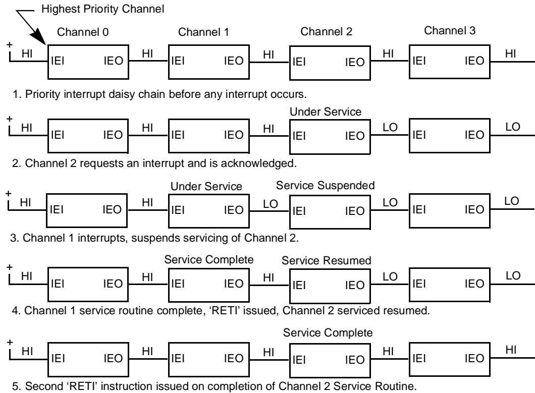
Figure 14. Daisy-Chain Interrupt Servicing
