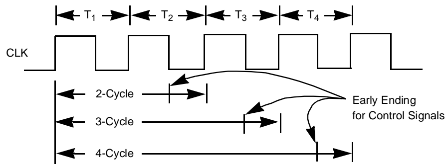
Figure 24. Variable Cycle Length
