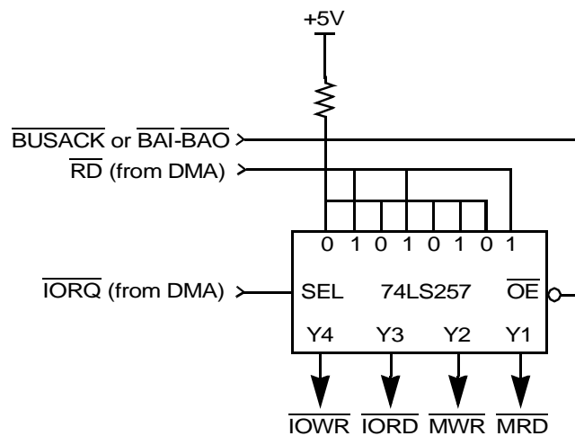
Figure 51. Simultaneous Transfer Multiplexer
