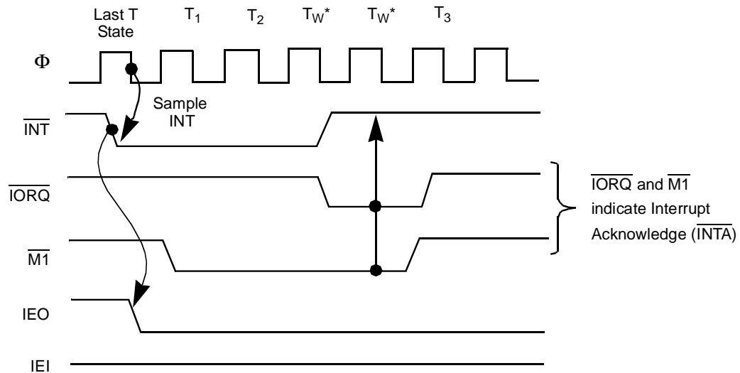
Figure 11. Interrupt Acknowledge Timing
