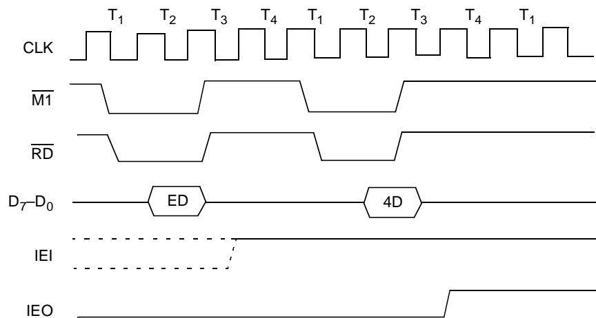
Figure 12. Return from Interrupt Cycle
