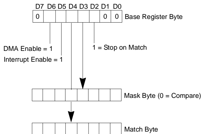
Figure 79. Write Register 3 Group
