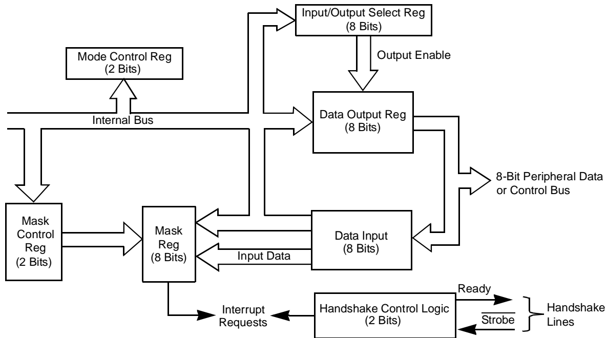
Figure 2. Port I/O Block Diagram
