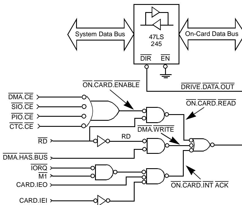
Figure 54. Data Bus Buffer Control Example
