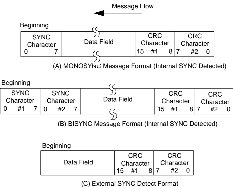
Figure 112. Synchronous Formats
