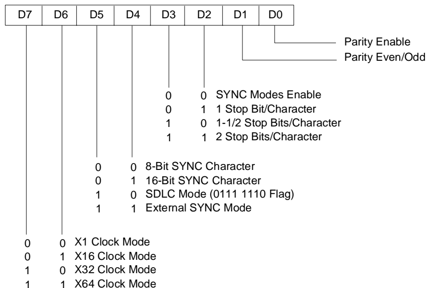
Figure 118. Write Register 4
