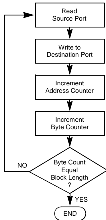
Figure 15. Typical CPU I/O Sequence
