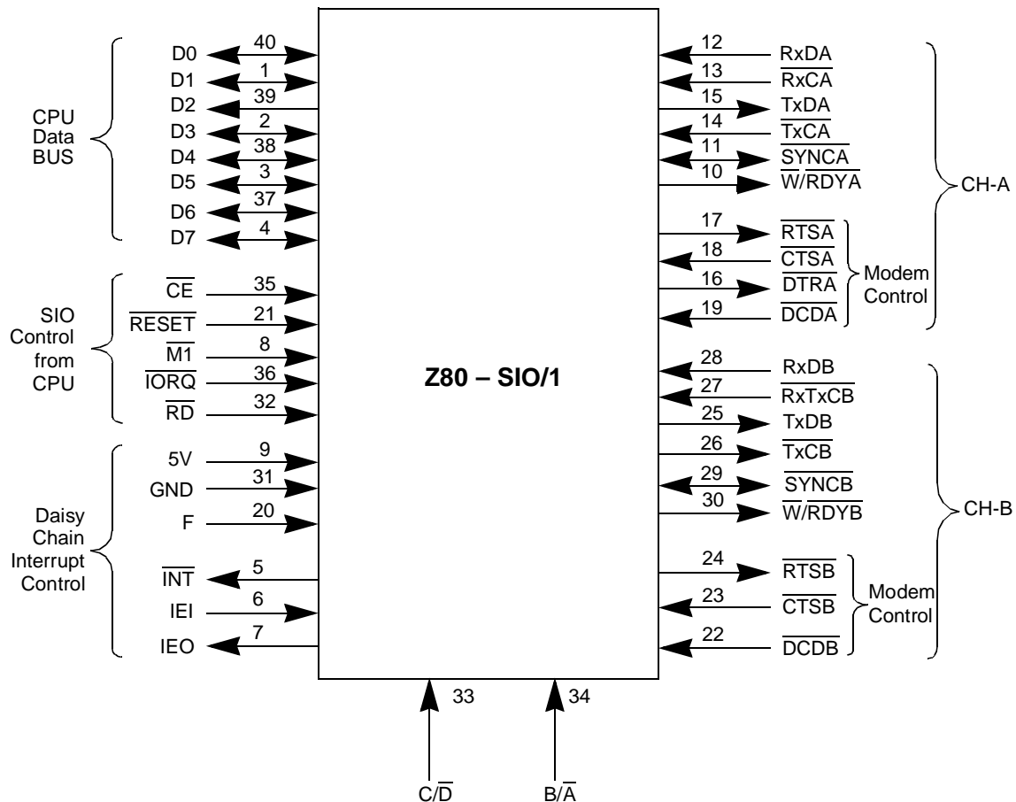
Figure 104. Z80 SIO/1 Pin Assignments
