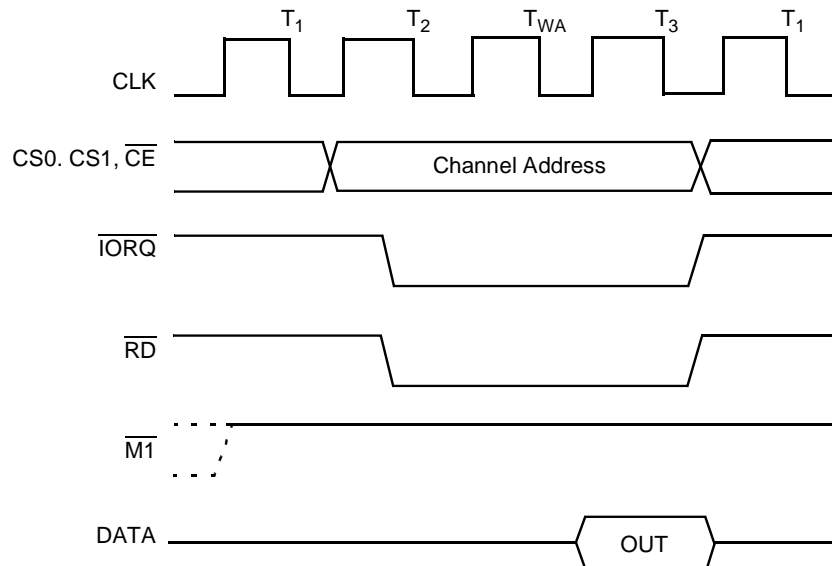
Figure 10. CTC Read Cycle
