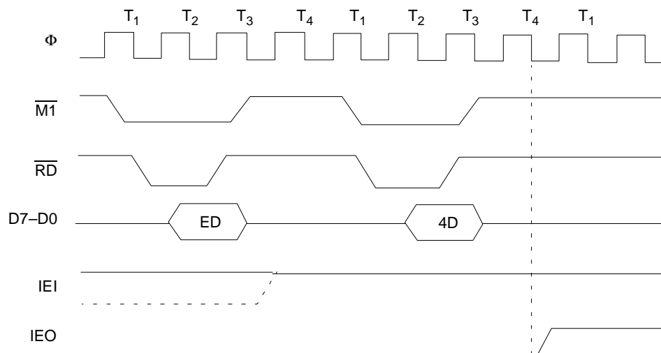
Figure 131. Return from Interrupt Cycle Timing
