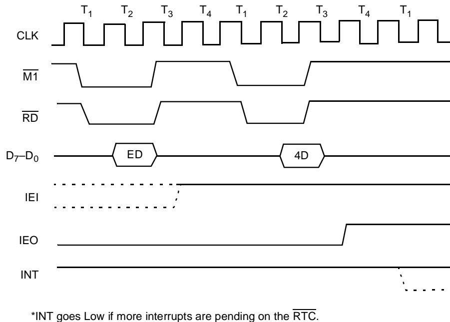
Figure 13. Return from Interrupt Cycle
