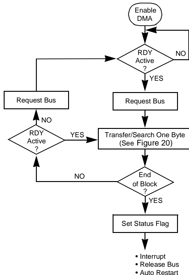
Figure 22. Burst Mode
