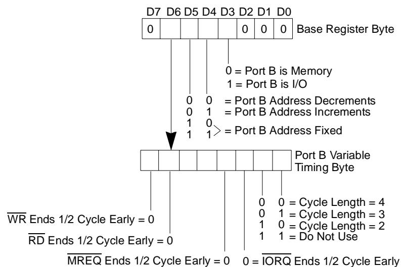
Figure 78. Write Register 2 Group
