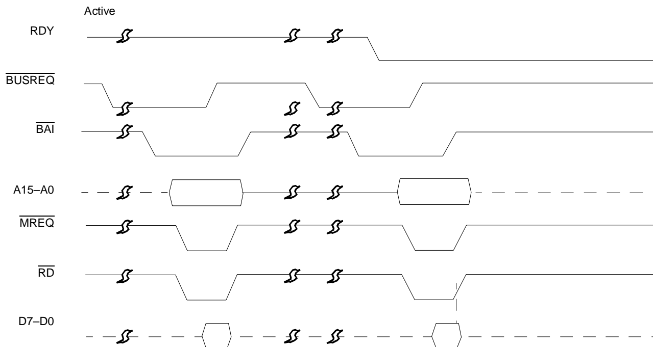
Figure 70. RDY Line in Byte Mode
