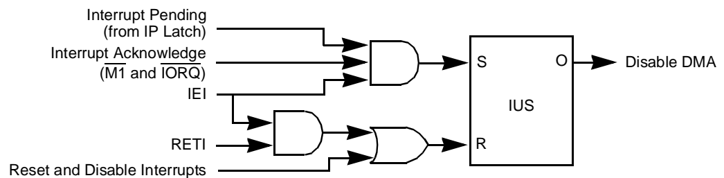
Figure 35. Interrupt Under Service (IUS) Latch
