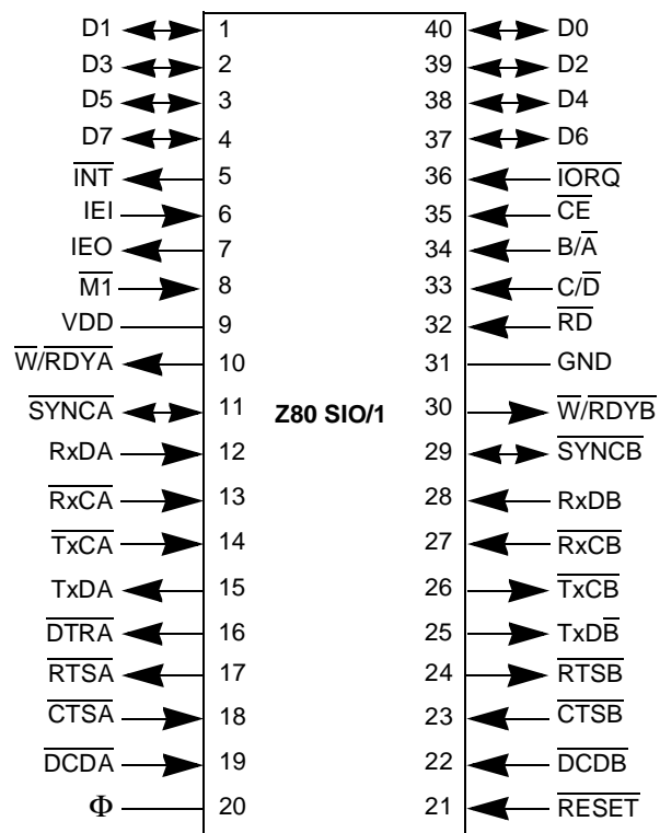
Figure 103. Z80 SIO/1 Pin Functions
