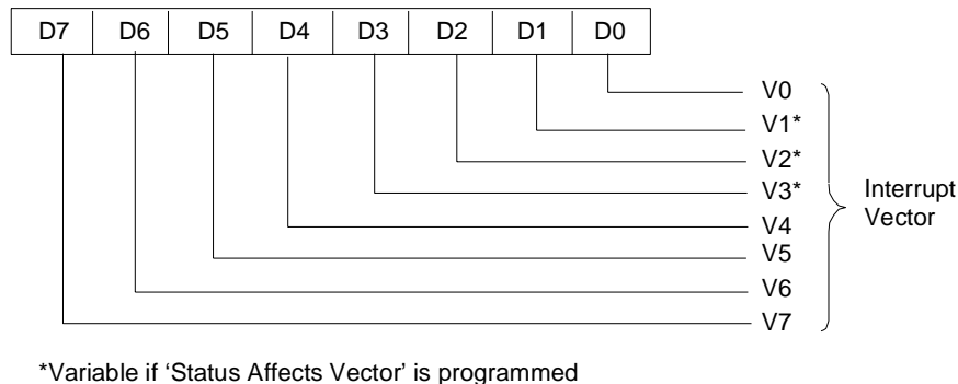
Figure 124. Read Register 2 (Channel B Only)
