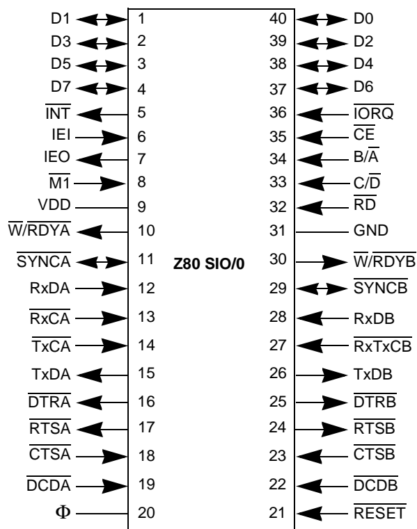
Figure 101. Z80 SIO/0 Functions
