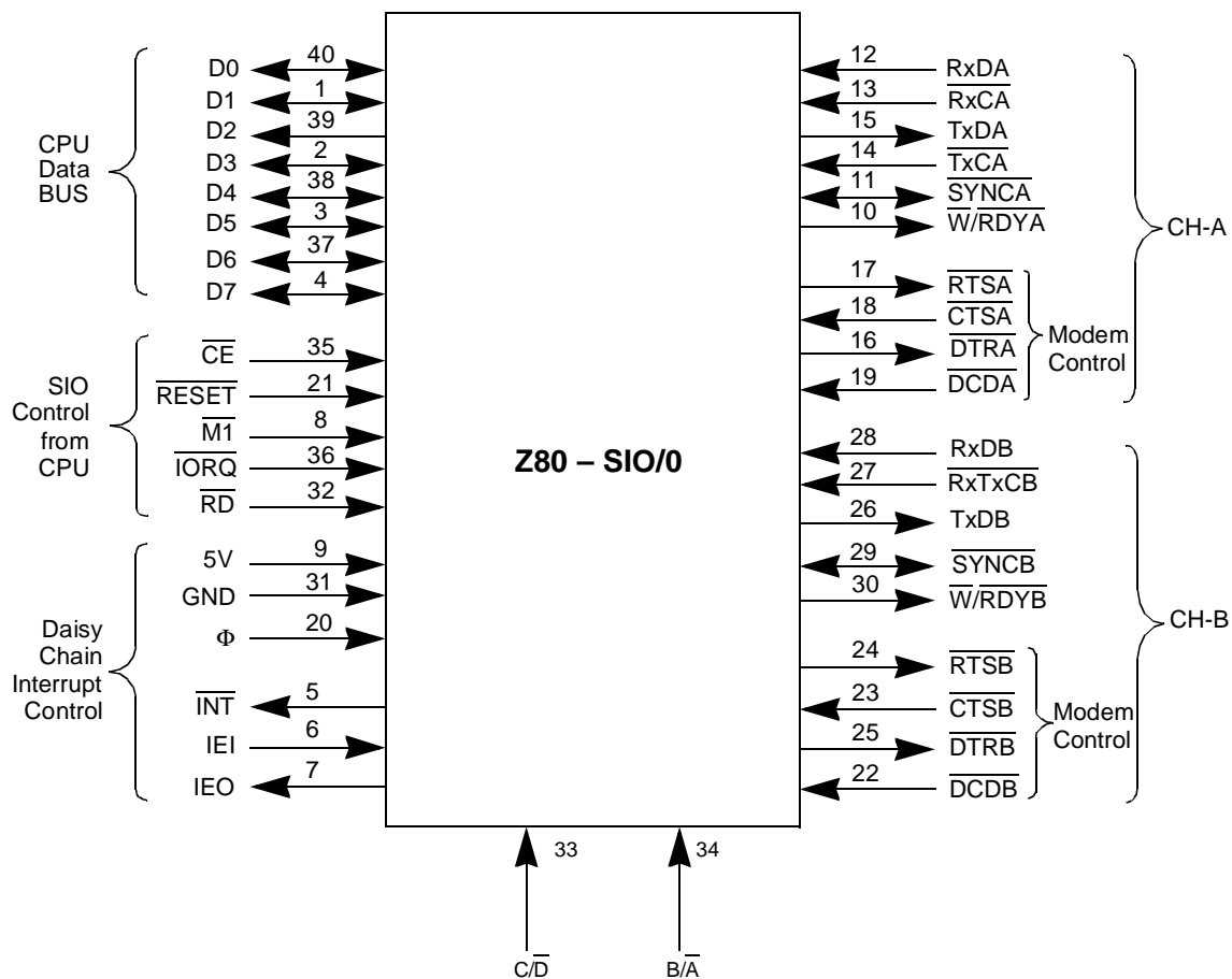
Figure 102. Z80 SIO/0 Pin Assignments
