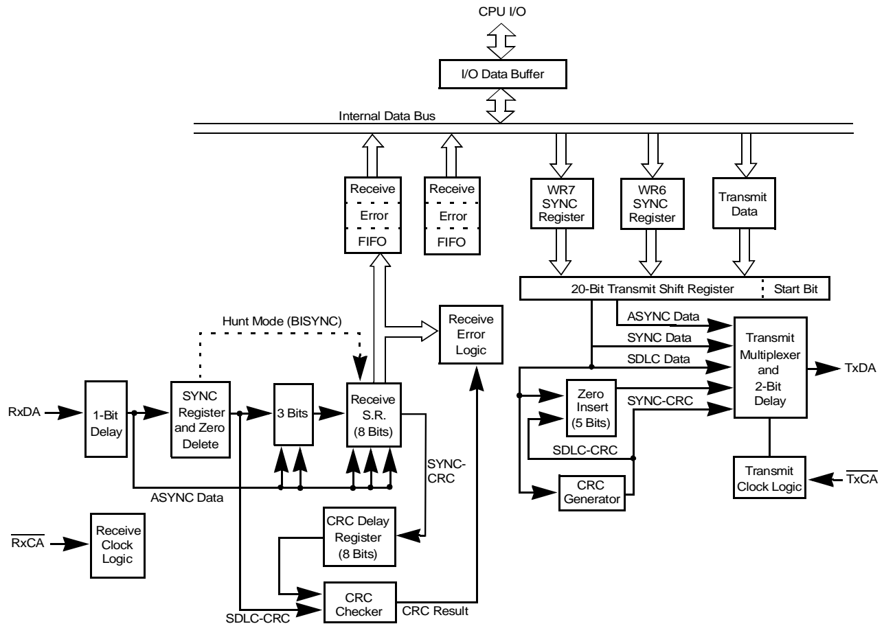
Figure 109. Transmit and Receive Data Path
