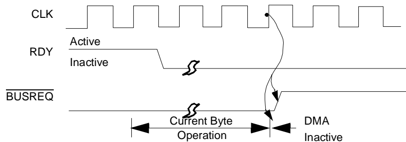
Figure 69. Bus Release on Not Ready (Burst Mode)
