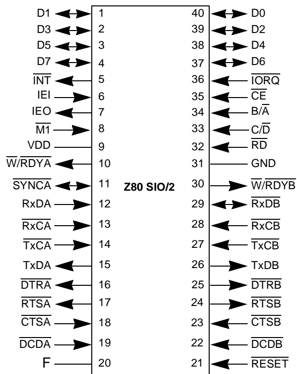
Figure 105. Z80 SIO/2 Pin Functions
