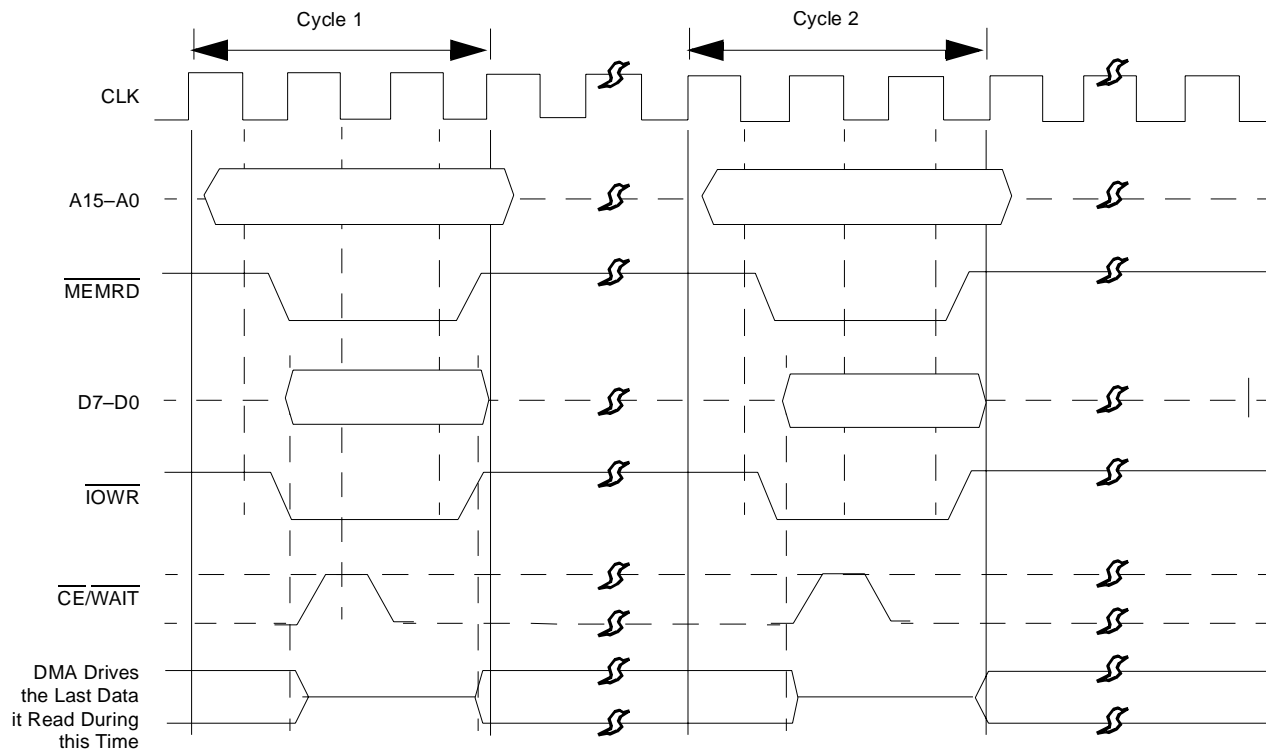
Figure 64. Simultaneous Memory-to-I/O Transfer (Byte Mode)
