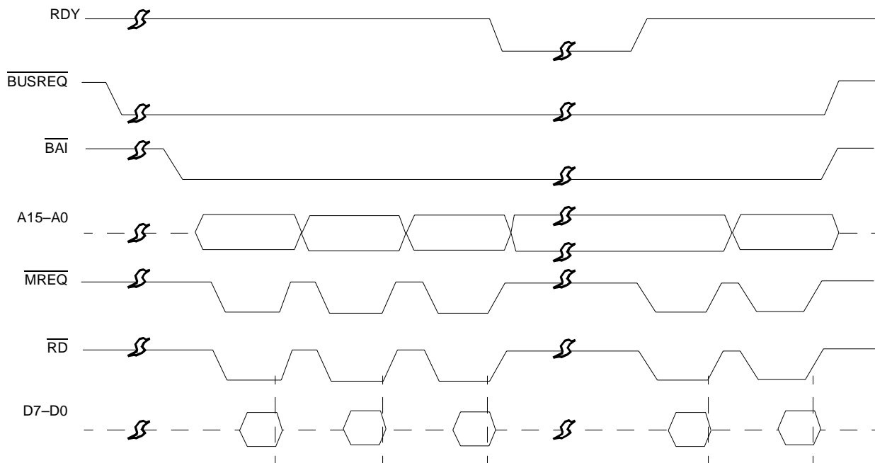
Figure 72. RDY Line in Continuous Mode
