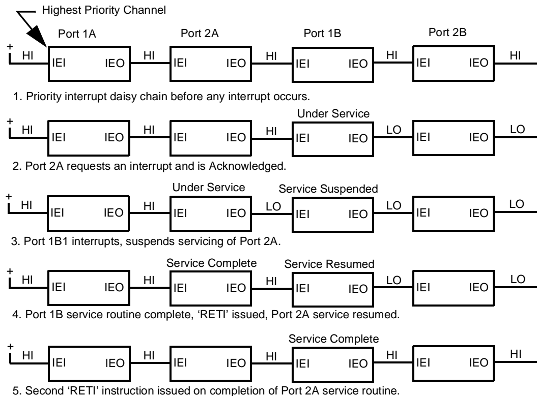
Figure 13. Daisy-Chain Interrupt Servicing
