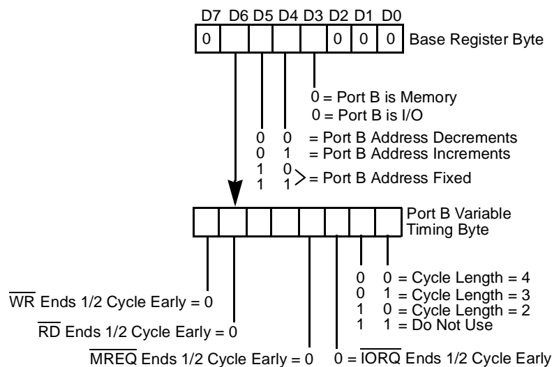
Figure 42. Write Register 2 Group
