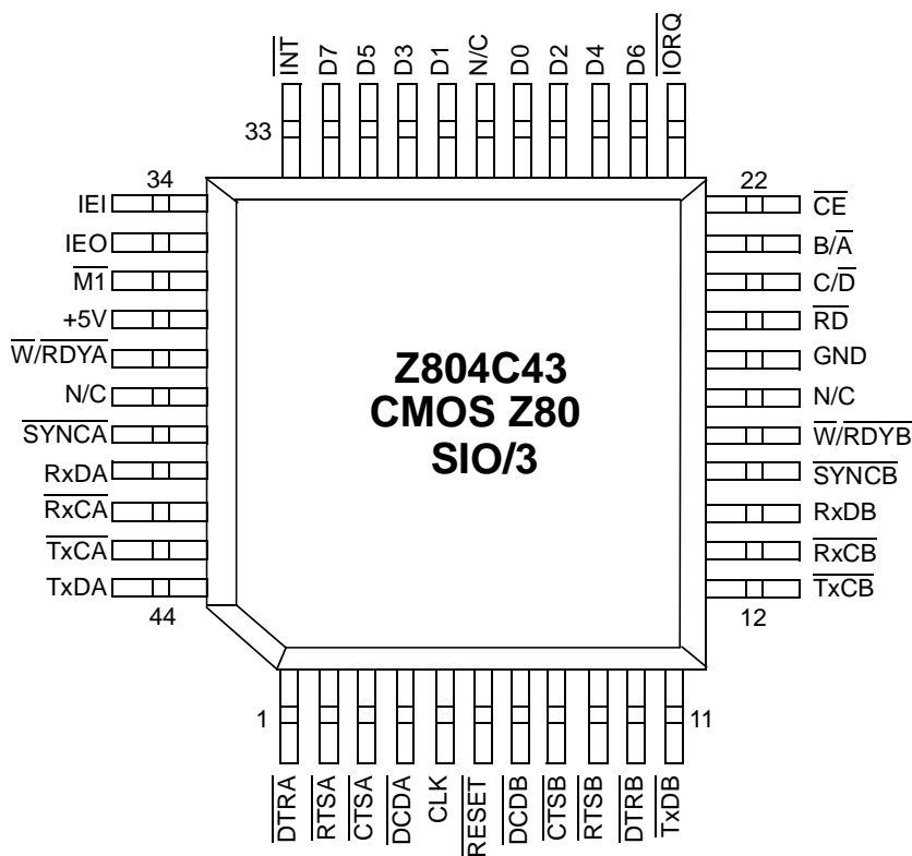
Figure 107. Z80 SIO/3 Pin Assignments
