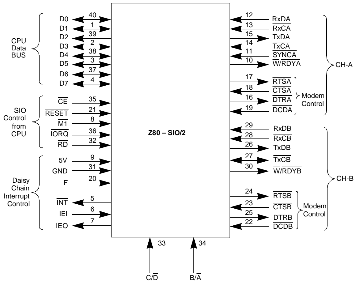
Figure 106. Z80 SIO/2 Pin Assignments
