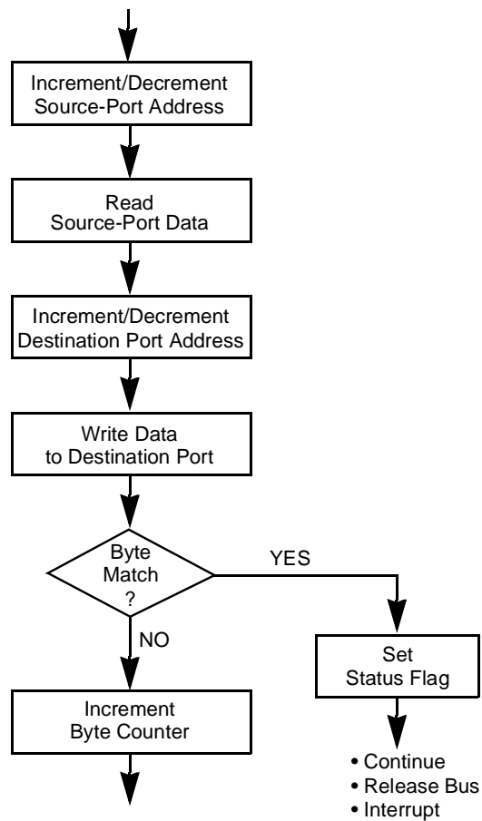
Figure 20. Transfer/Search One Byte
