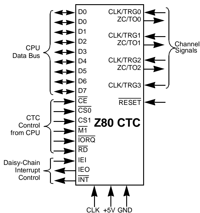
Figure 4. CTC Pin Configuration
