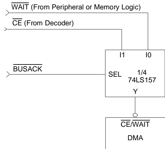
Figure 50. \overline{\text{CE}}/\overline{\text{WAIT}} Multiplexer
