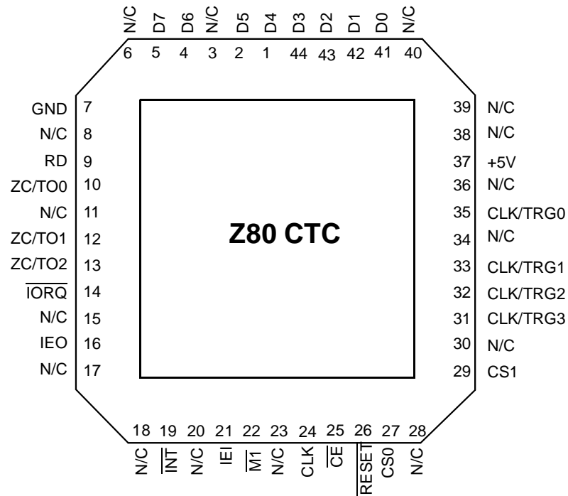
Figure 6. 44-Pin Chip Carrier Pin Assignments
