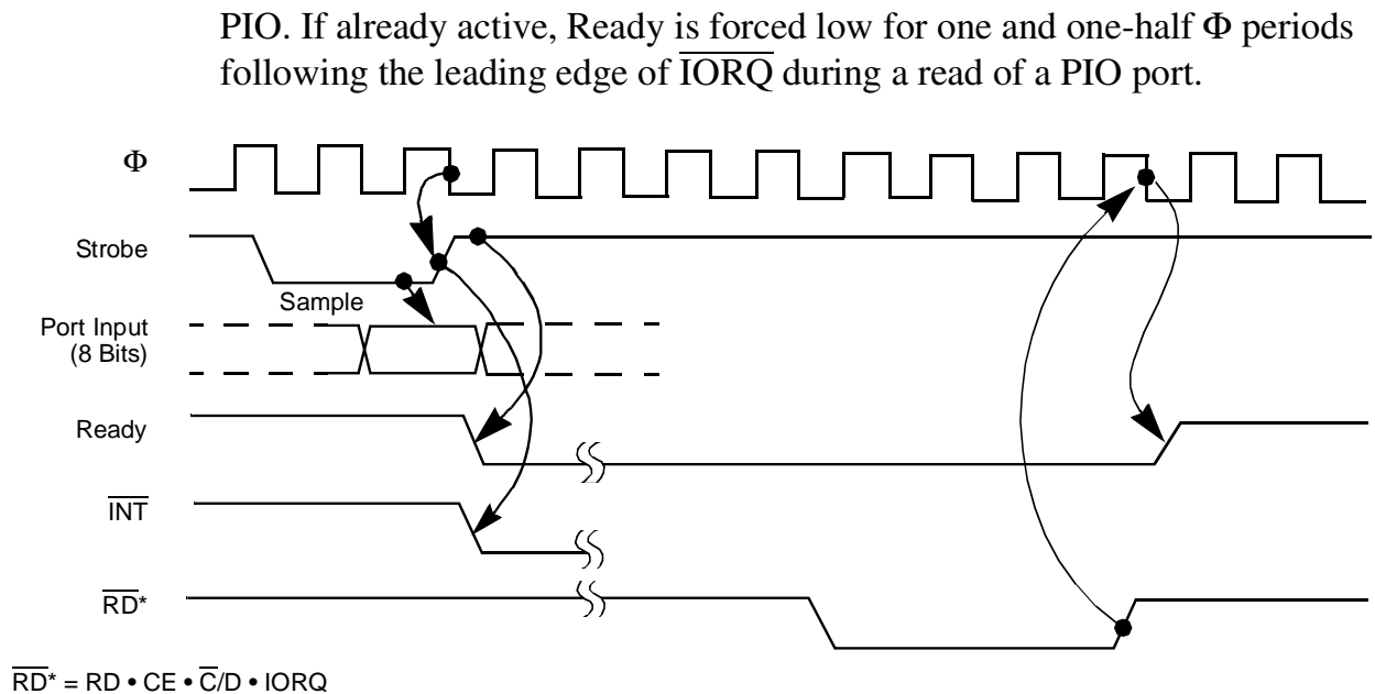
Figure 8. Mode 1 (Input) Timing
