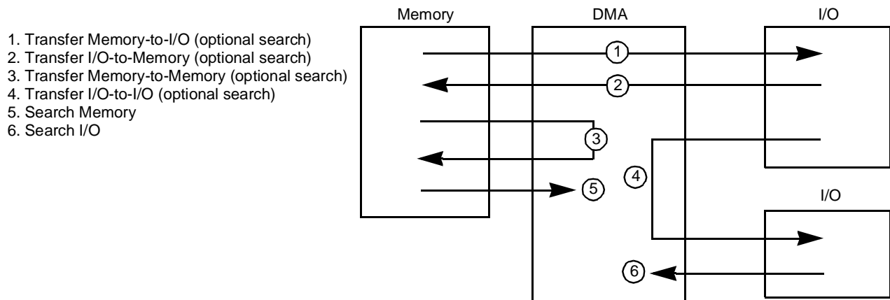
Figure 19. Basic Functions of the Z80 DMA
