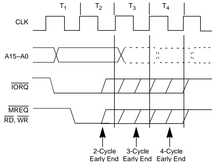
Figure 73. Variable-Cycle and Edge Timing
