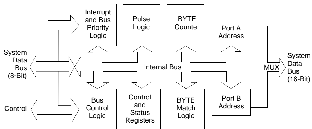
Figure 29. Z80 DMA Block Diagram
