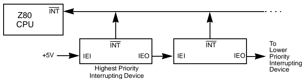
Figure 37. Interrupt Daisy-Chain
