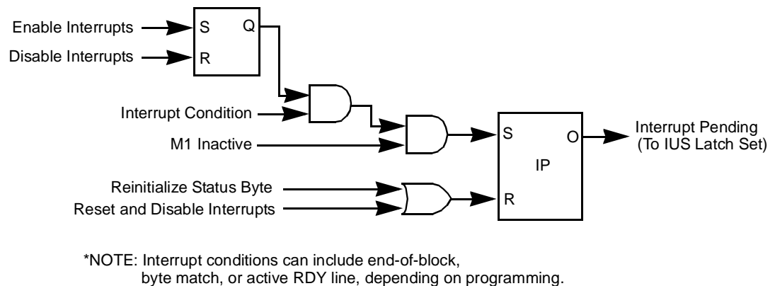
Figure 34. Interrupt Pending (IP) Latch
