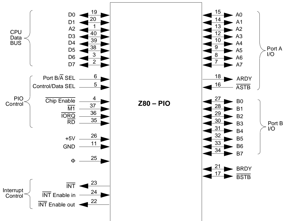
Figure 3. PIO Pin Functions
