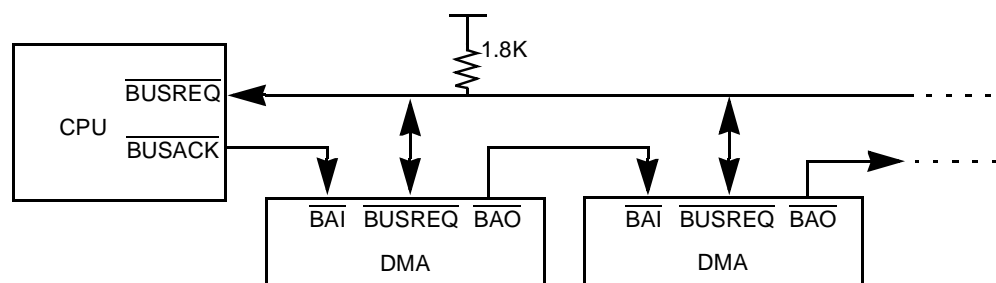
Figure 31. Bus-Requesting Daisy-Chain
