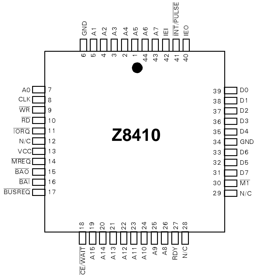
Figure 27. 44-Pin PLCC Pin Assignments (Z8410 NMOS)
