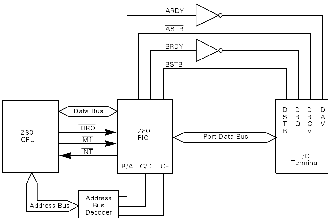
Figure 15. Example of I/O Interface
