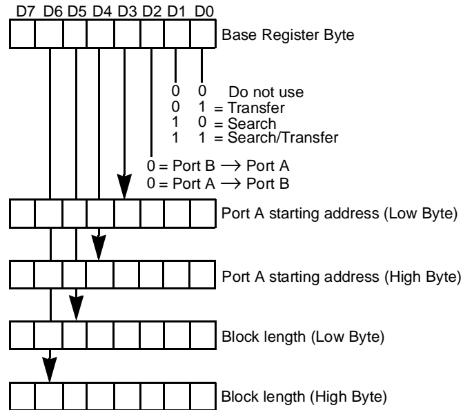
Figure 40. Write Register 0 Group
