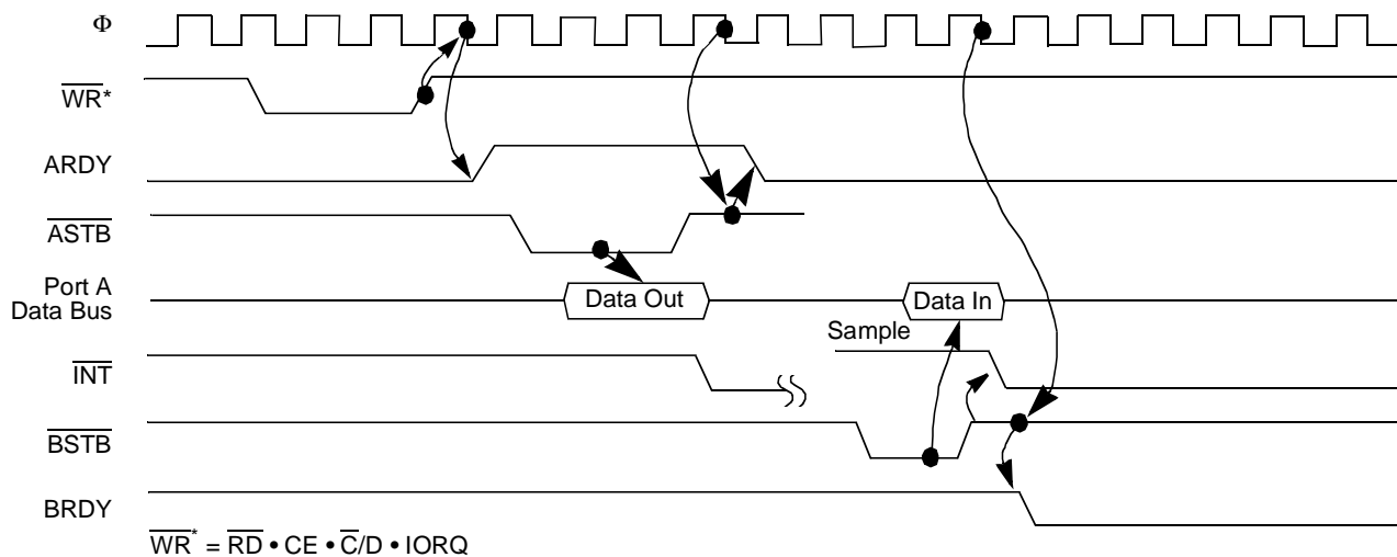
Figure 9. Port A, Mode 2 (Bidirectional) Timing
