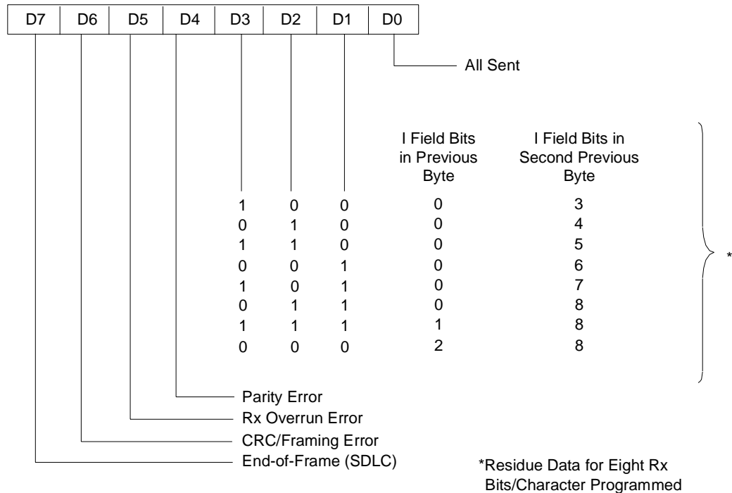
Figure 123. Read Register 1
