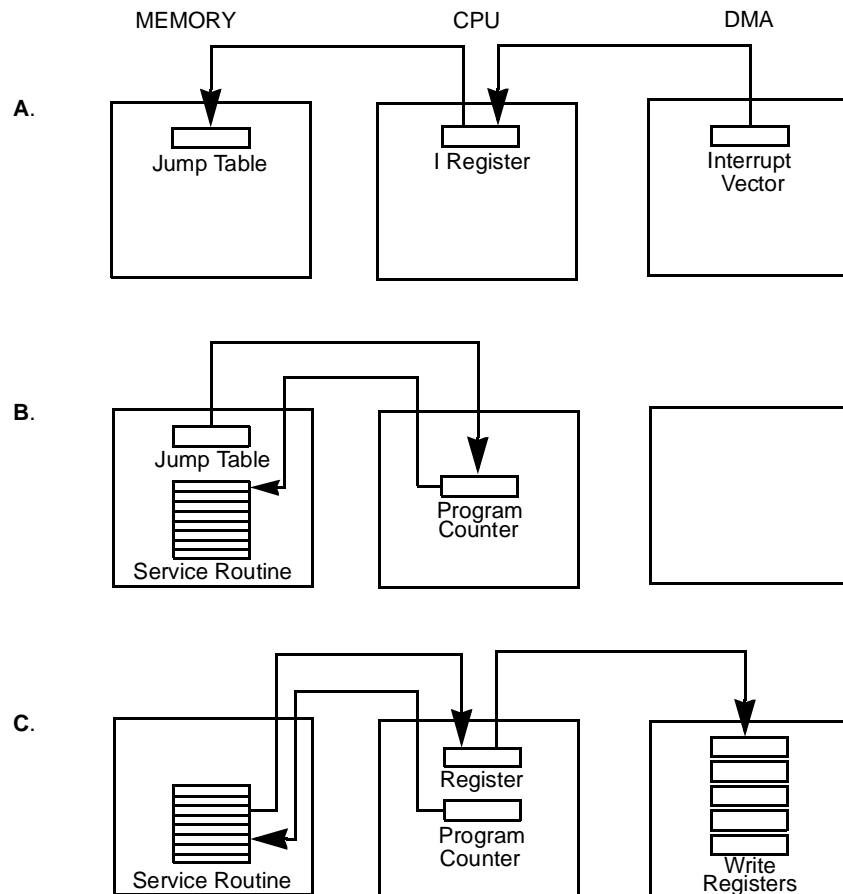
Figure 33. Interrupt Service Routine
