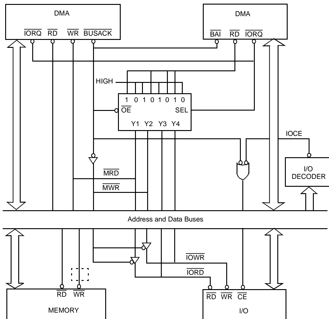
Figure 52. Simultaneous Transfer
