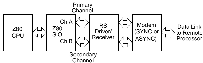
Figure 126. Synchronous/Asynchronous Processor-to-Processor Communication (Using Telephone Line)
