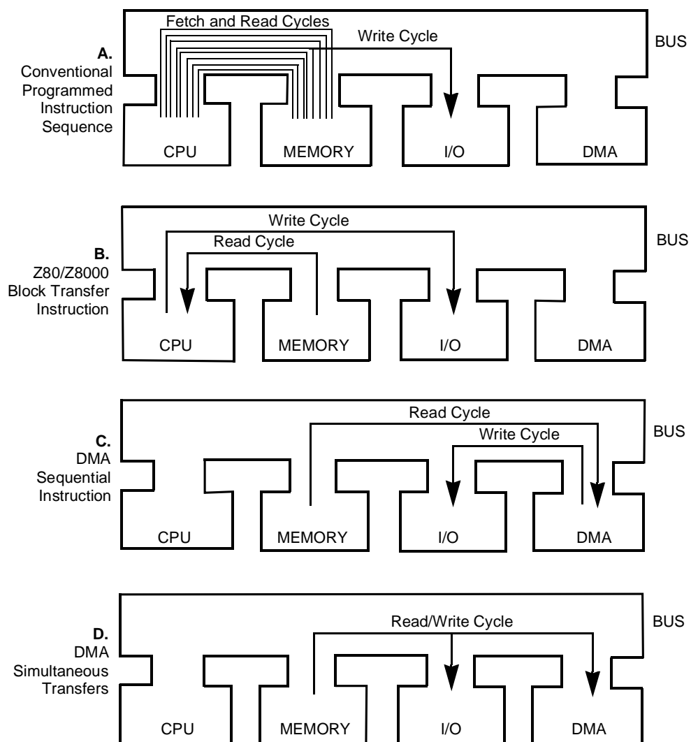
Figure 16. Conceptual Comparison of Various I/O Transfer Methods
