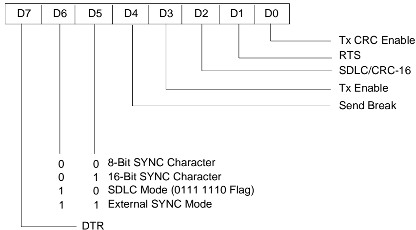
Figure 119. Write Register 5
