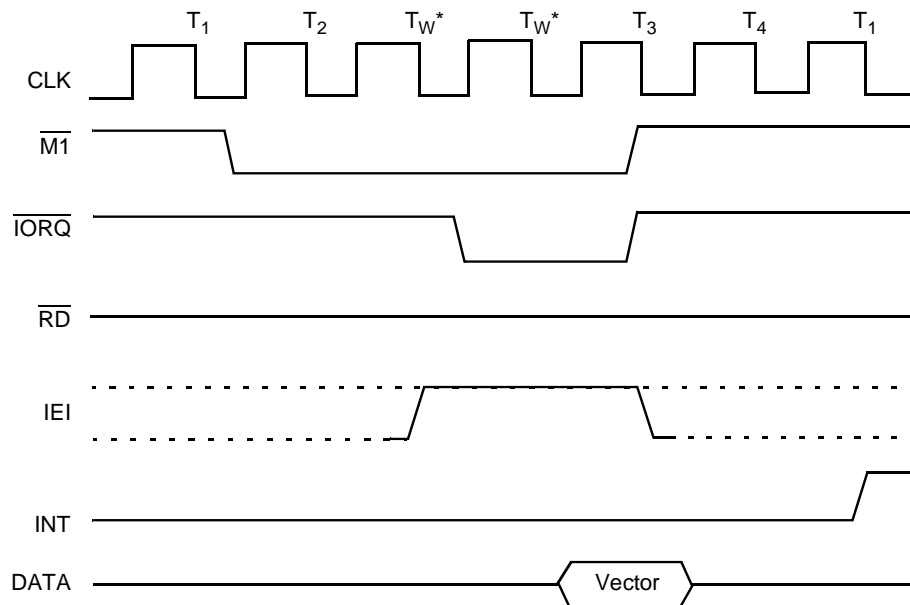
Figure 12. Interrupt Acknowledge Cycle
