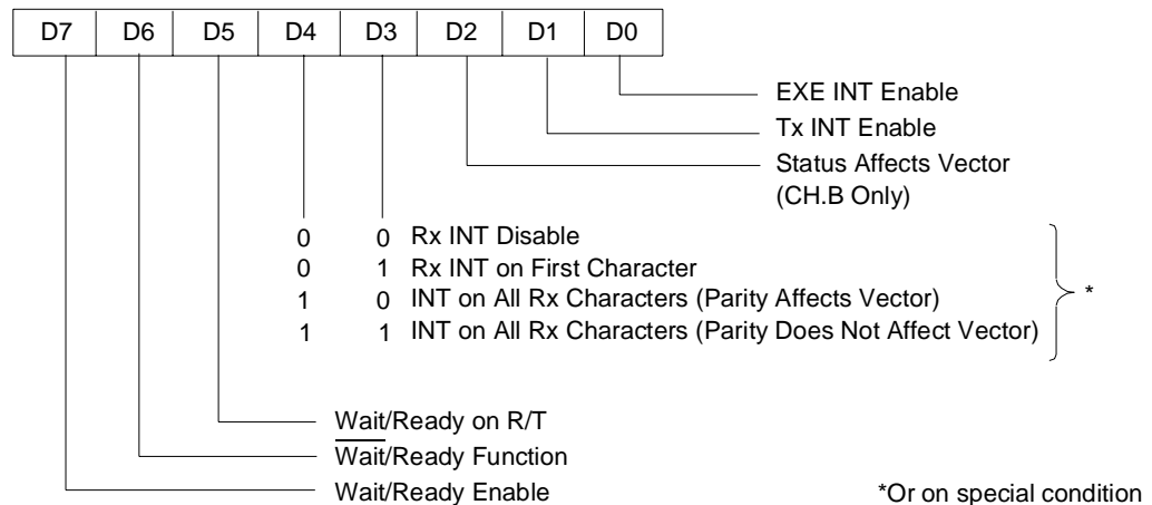
Figure 115. Write Register 1
