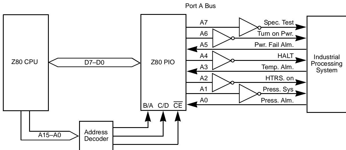
Figure 16. Control Mode Application
