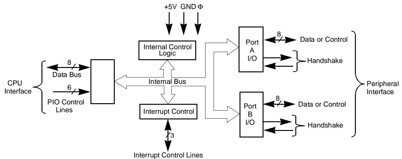
Figure 1. PIO Block Diagram
