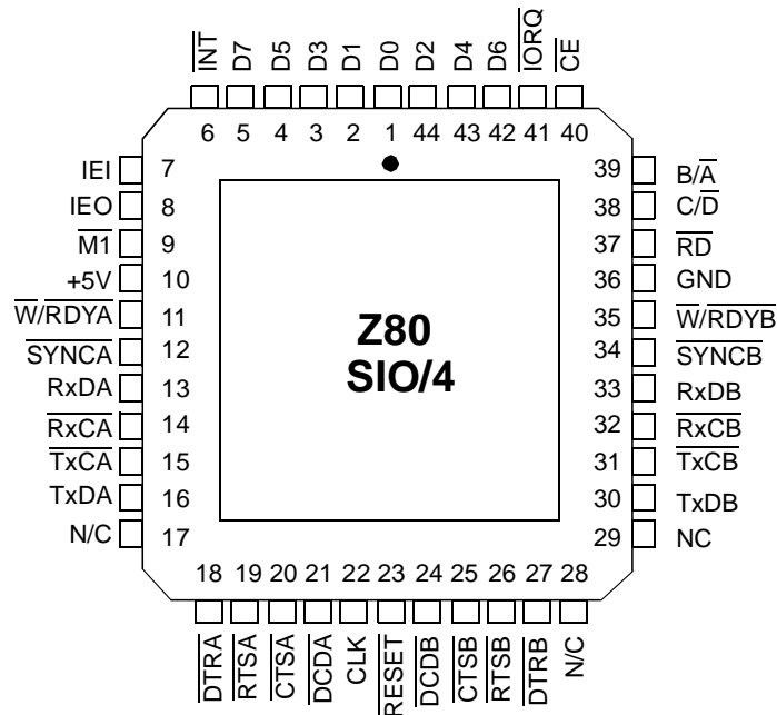
Figure 108. Z80 SIO/4 Pin Assignments
