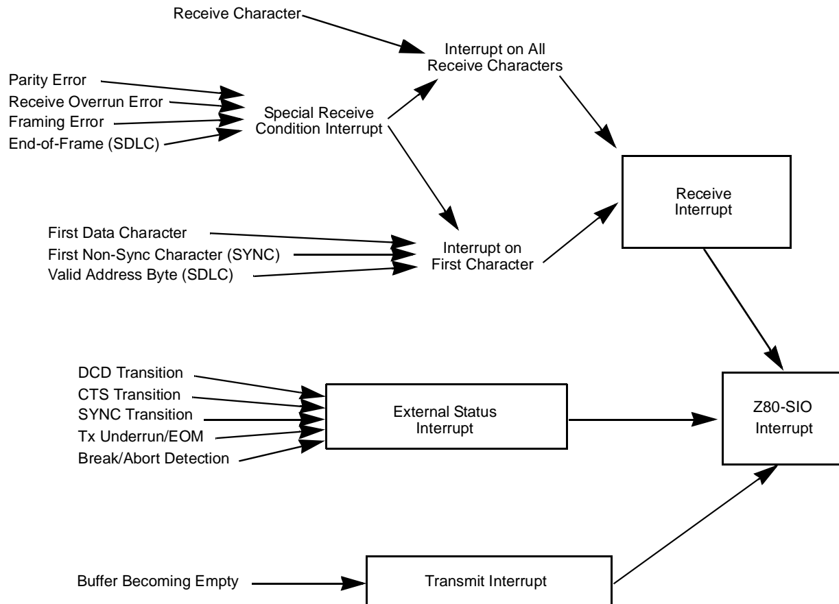
Figure 110. Interrupt Structure
