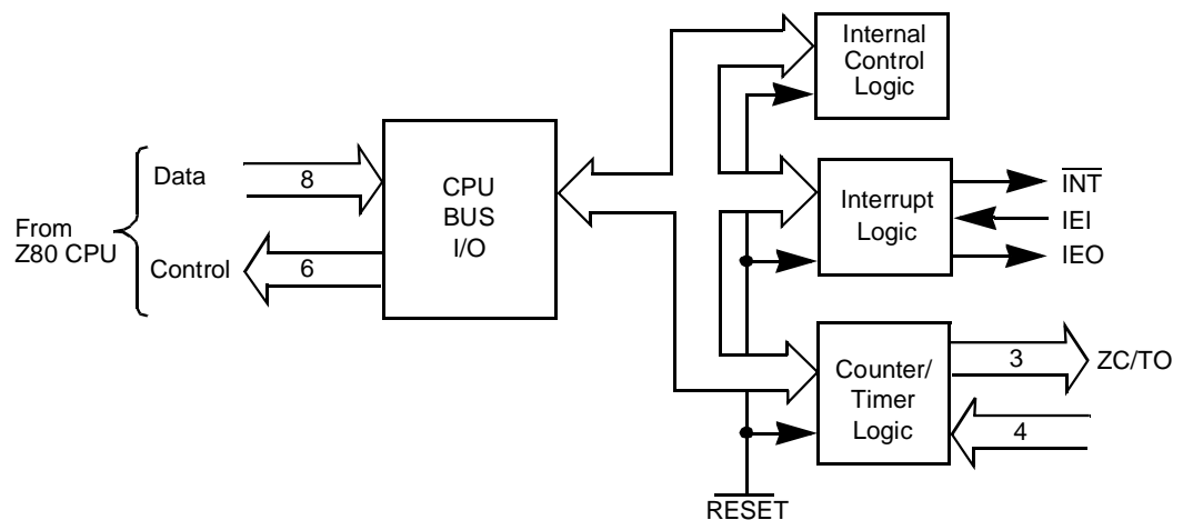
Figure 1. CTC Block Diagram
