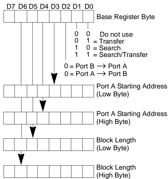
Figure 76. Write Register 0 Group
