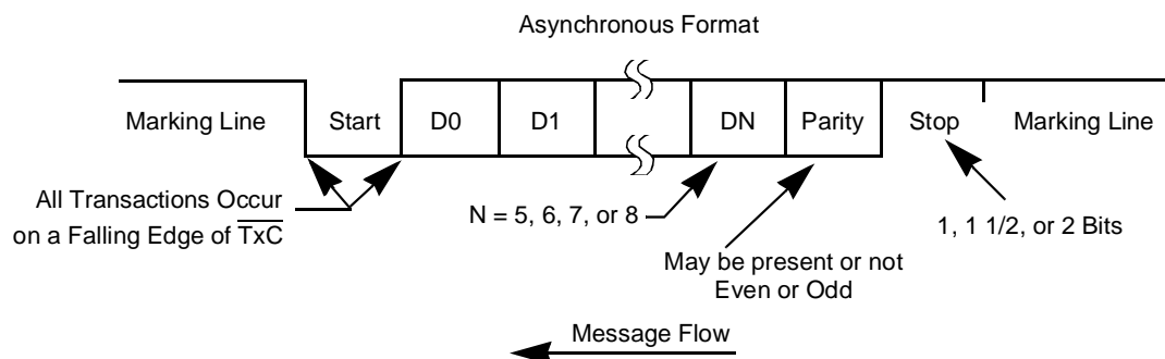
Figure 111. Asynchronous Message Format
