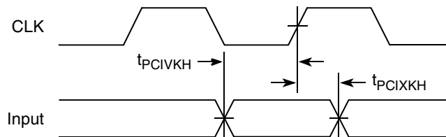
Figure 36. PCI Input AC Timing Measurement Conditions
