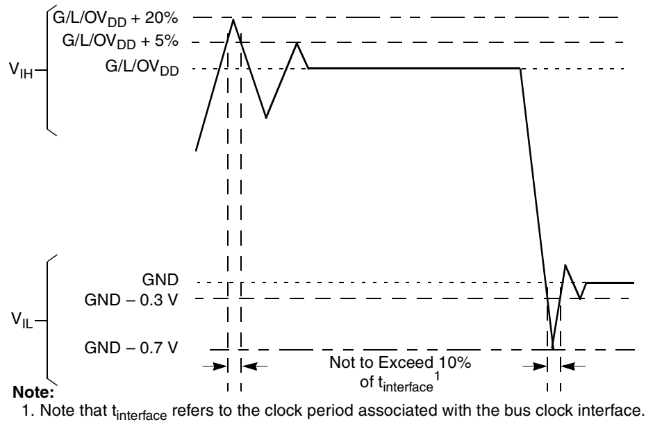
Figure 3. Overshoot/Undershoot Voltage for GV_{DD}/OV_{DD}/LV_{DD}
