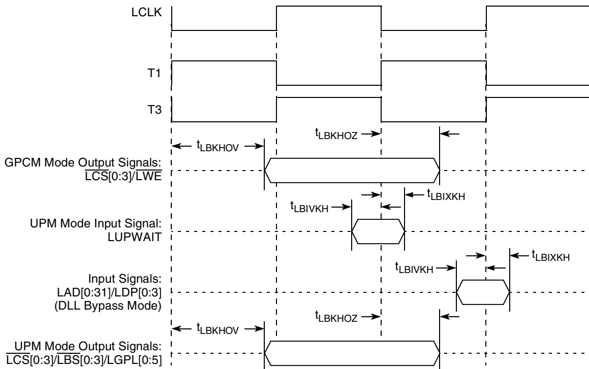
Figure 26. Local Bus Signals, GPCM/UPM Signals for \text{LCRR}[\text{CLKDIV}] = 2 (DLL Bypass Mode)
