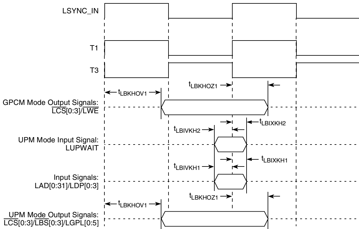
Figure 25. Local Bus Signals, GPCM/UPM Signals for \text{LCRR}[\text{CLKDIV}] = 2 (DLL Enabled)
