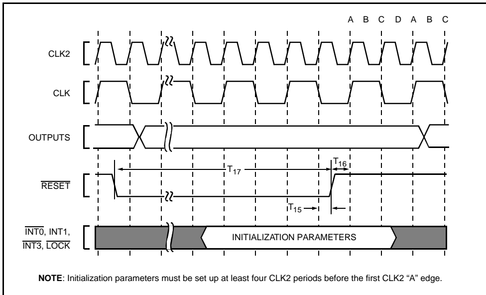
Figure 13. RESET Signal Timing
