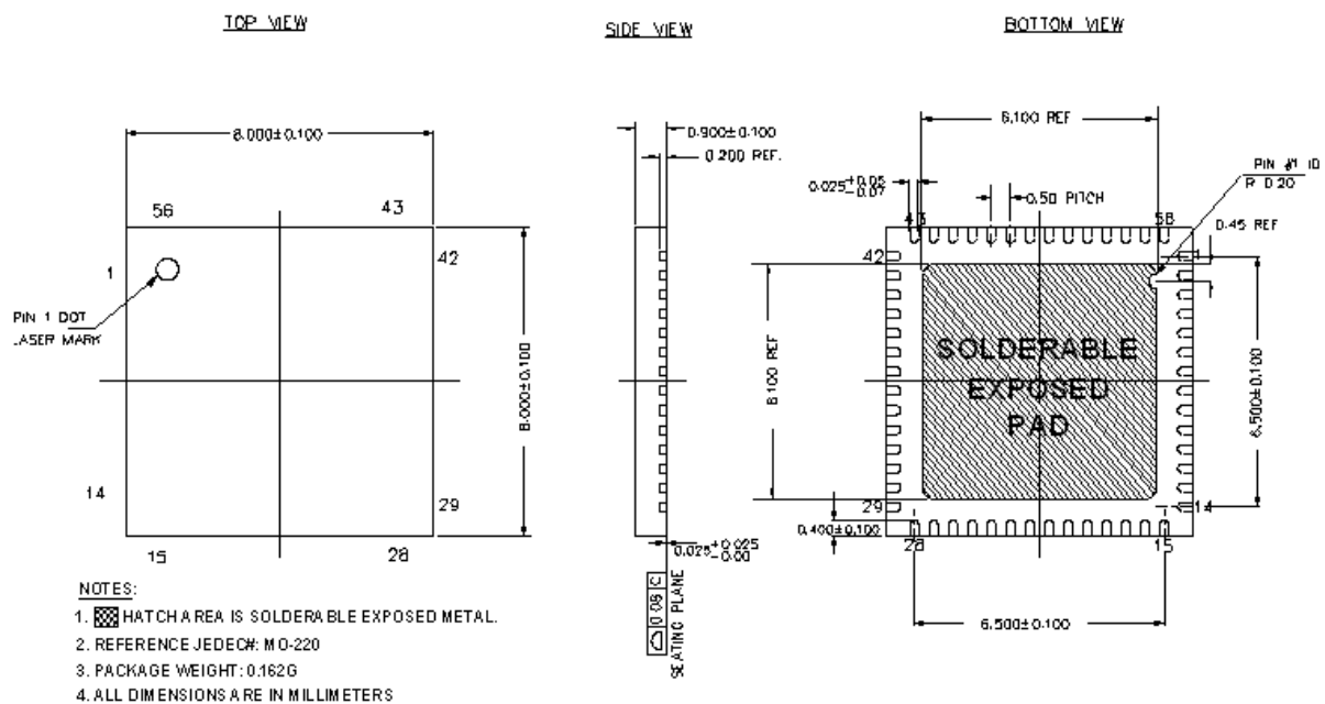
Figure 38. 56-Pin QFN 8 x 8 mm (Sawn Version)
