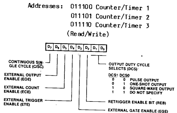
Figure 2-15. Counter/Timer Mode Specification Registers
