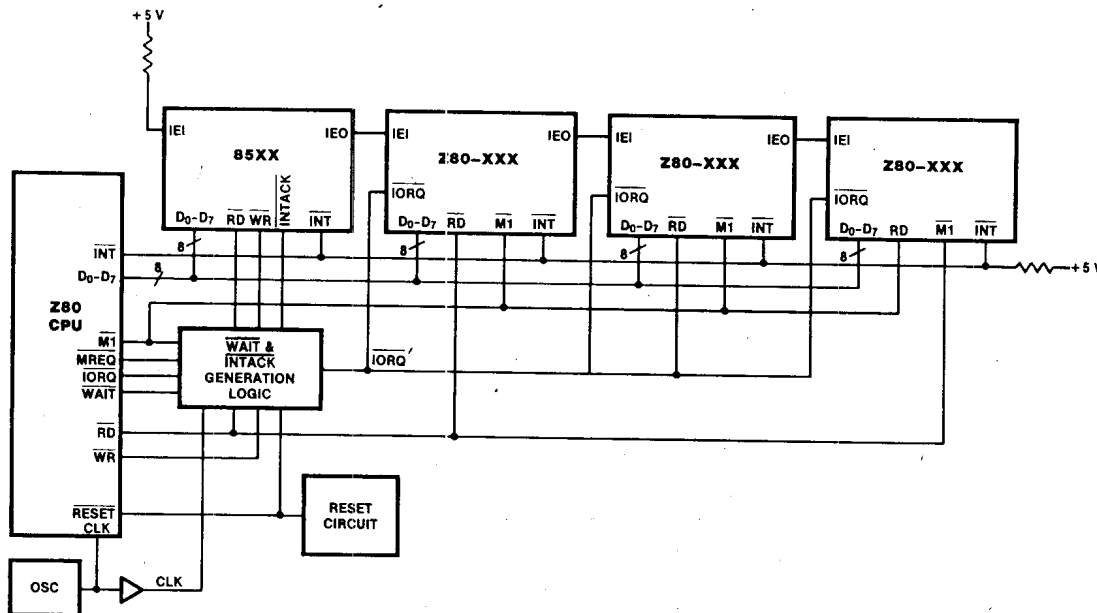
Figure 5-3. Non Z-Bus Interrupt Arbitration
