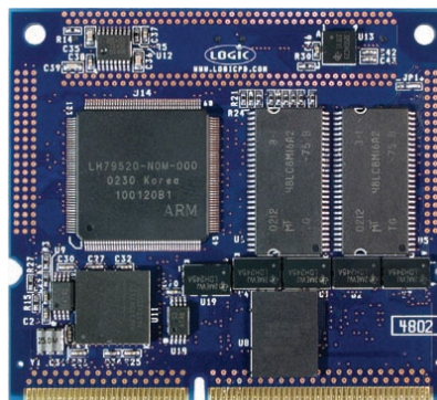
LH79520 CARD ENGINE
