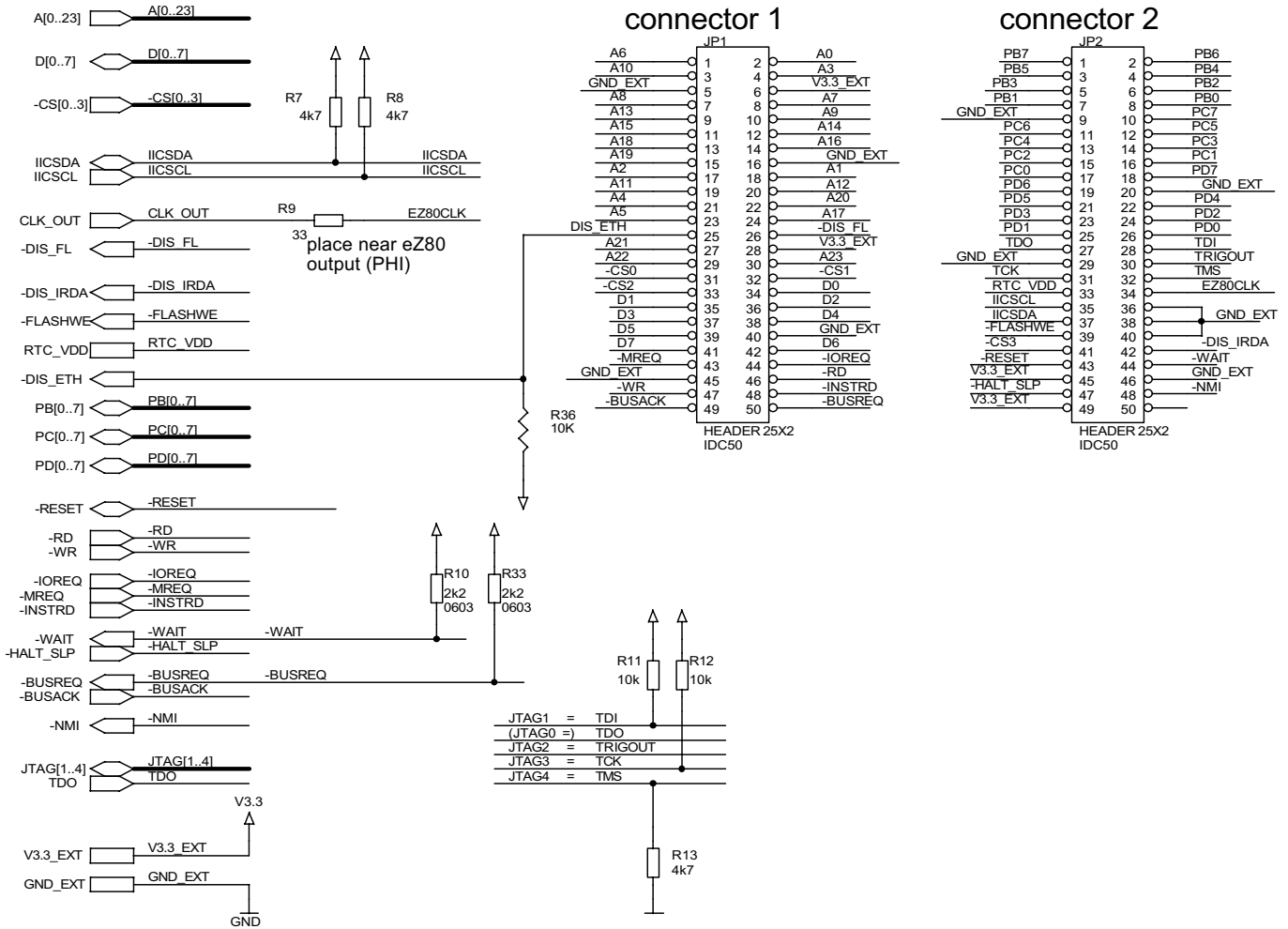
Figure 15. eZ80L92 Module Schematic Diagram, #7 of 9—Headers
