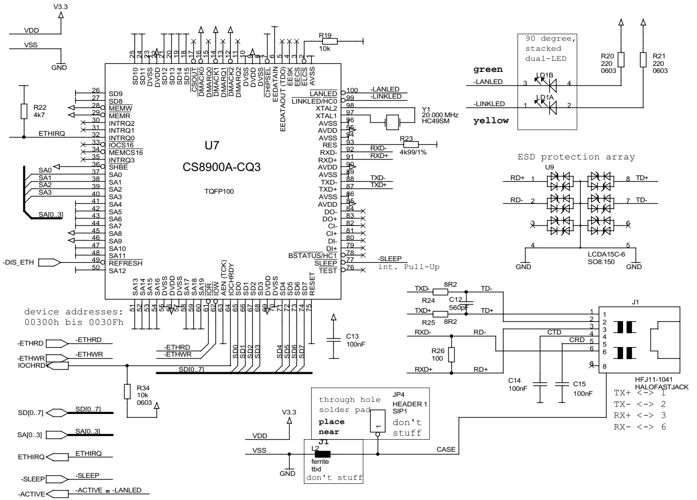
Figure 13. eZ80L92 Module Schematic Diagram, #5 of 9—E-NET Module
