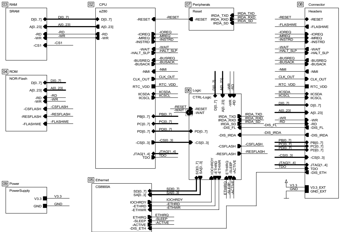
Figure 9. eZ80L92 Module Schematic Diagram, #1 of 9—Top Level
