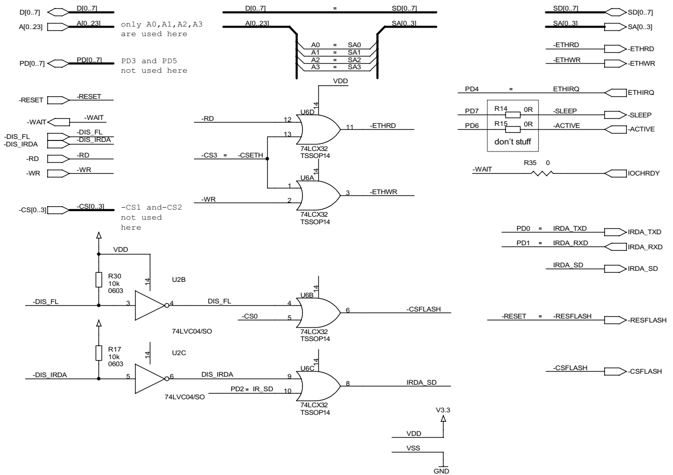
Figure 17. eZ80L92 Module Schematic Diagram, #9 of 9—Control Logic
