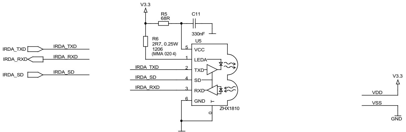
Figure 14. eZ80L92 Module Schematic Diagram, #6 of 9—IrDA Reset
