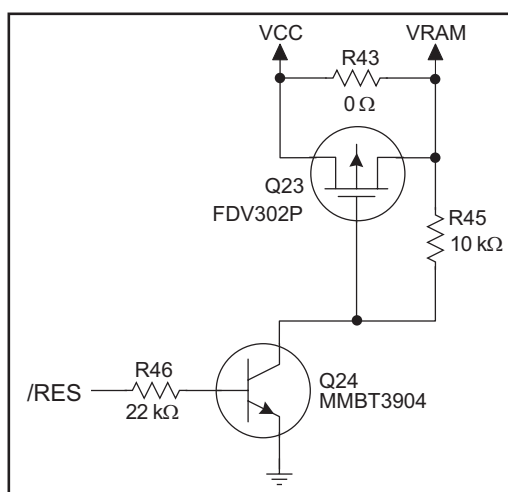
Figure C-6. VRAM Switch
