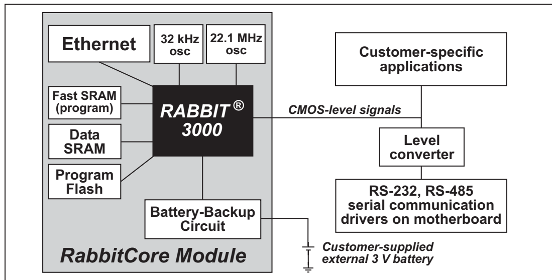
Figure 5. RCM3200 Subsystems
