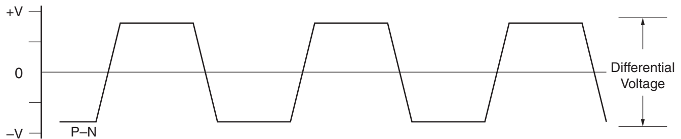
Figure 12: Differential Peak-to-Peak Voltage
