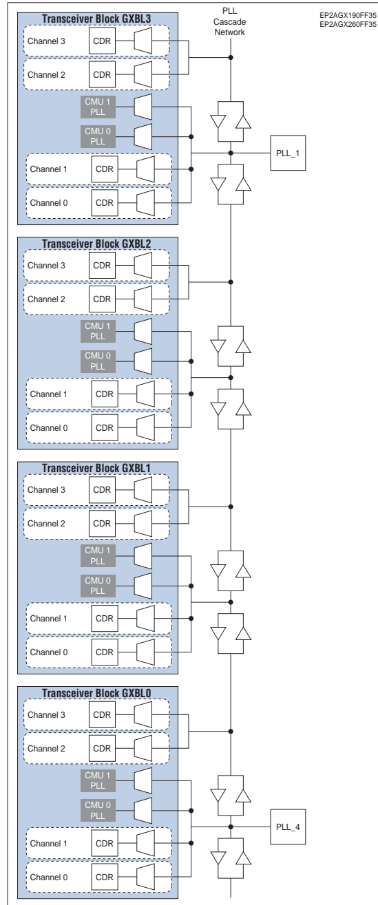
Figure 2-34. FPGA Fabric PLLs-Transceiver PLL's Cascading Option Allowed in the EP2AGX190FF35 and EP2AGX260FF35 Devices
