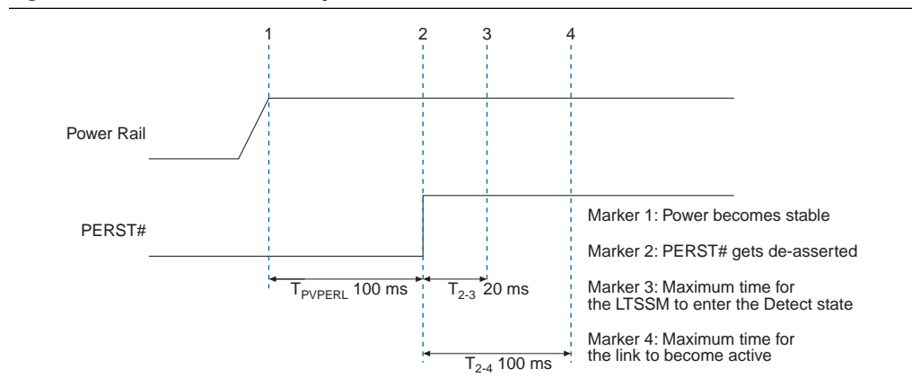
Figure 1-69. PCIe Cold Reset Requirements
