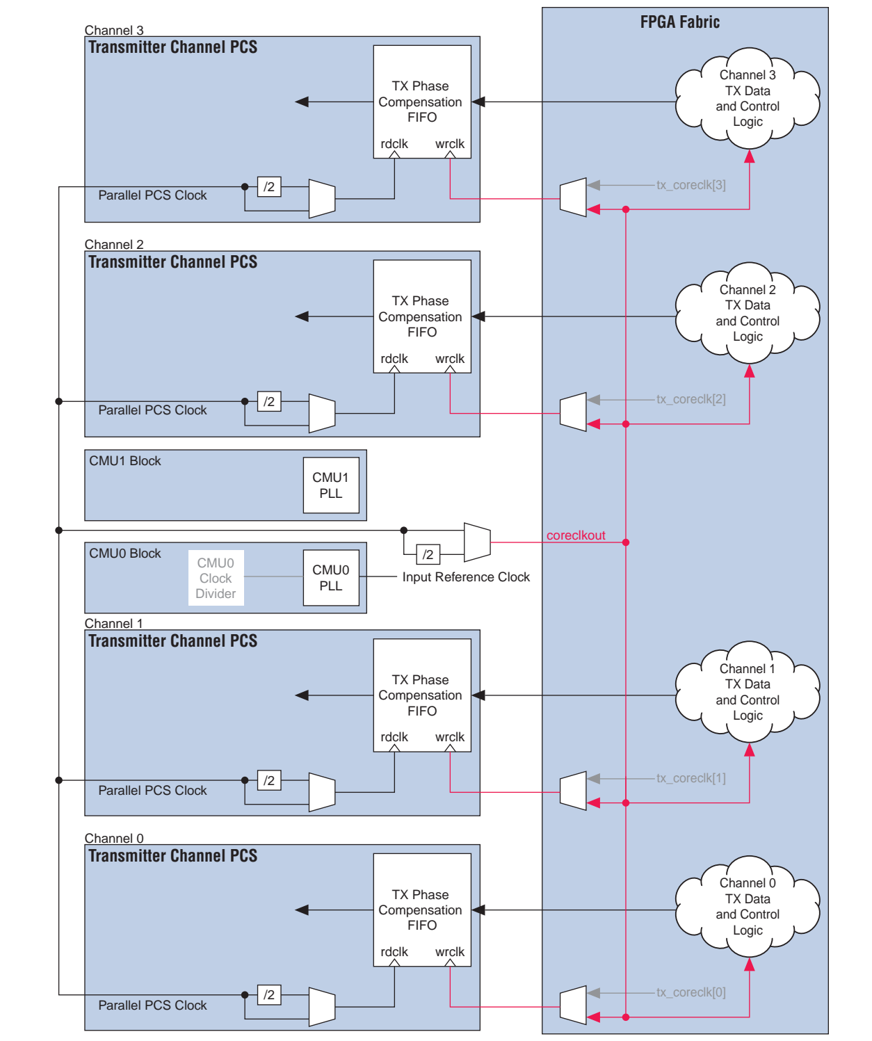
Figure 2-20. FPGA Fabric-Transmitter Interface Clocking in an ×4 Bonded Channel Configuration
