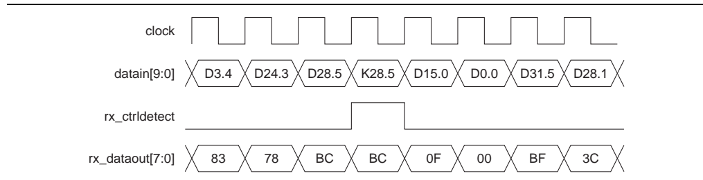
Figure 1-42. 8B/10B Decoder in Control Code Group Detection
