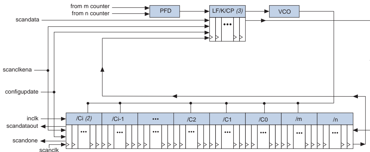
Figure 5-35. PLL Reconfiguration Scan Chain for Arria II Devices (Note 1)
