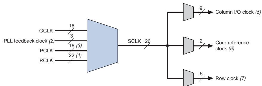
Figure 5-5. Hierarchical Clock Networks per Spine Clock in Arria II Devices (Note 1)
