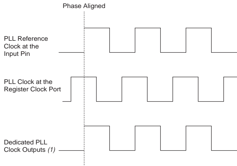
Figure 5-25. Phase Relationship Between PLL Clocks in Zero Delay Buffer Mode for Arria II Devices
