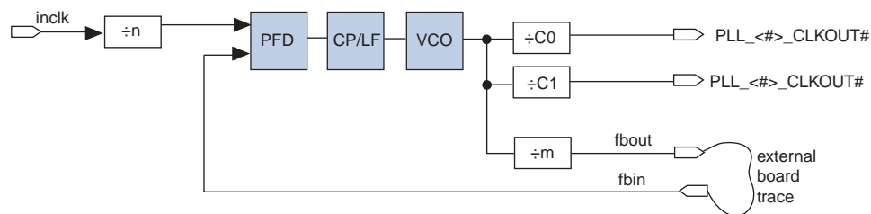
Figure 5-27. External Feedback Mode in Arria II GZ Devices
