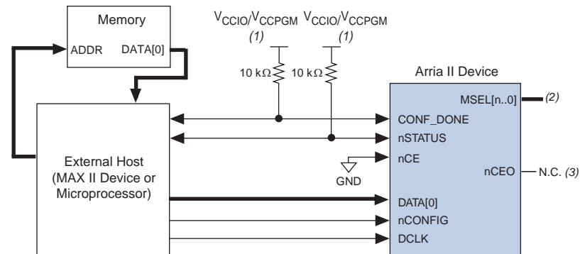
Figure 9-10. Single Device PS Configuration Using an External Host
