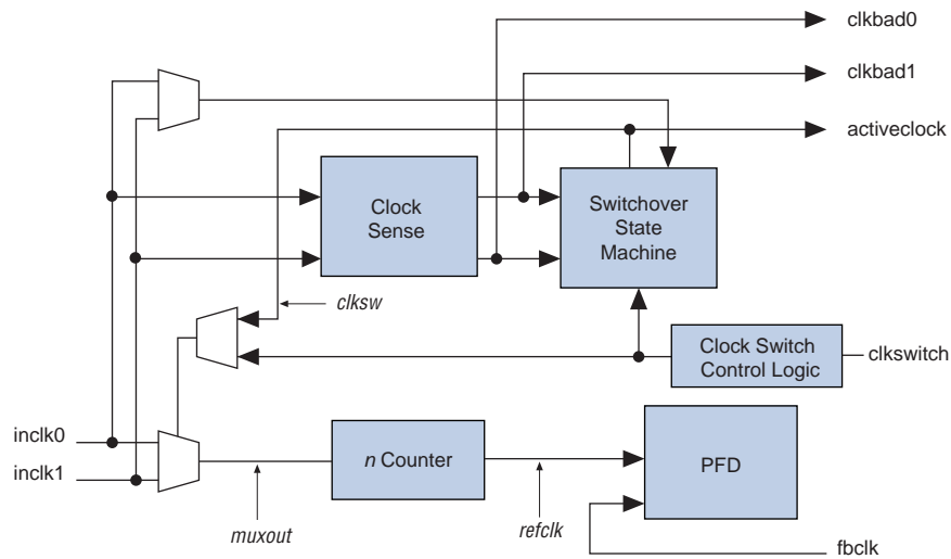
Figure 5-30. Automatic Clock Switchover Circuit Block Diagram for Arria II Devices
