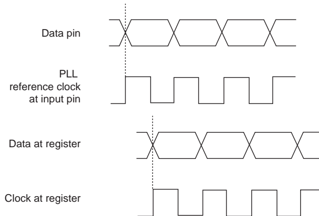
Figure 5-20. Phase Relationship Between Clock and Data in Source-Synchronous Mode in Arria II Devices
