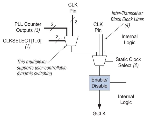
Figure 5-8. GCLK Control Block for Arria II Devices
