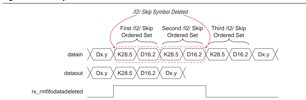
Figure 1-60. Example of Rate Match Deletion in GIGE Mode
