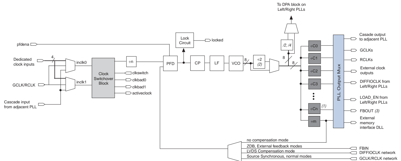
Figure 5-16. PLL Block Diagram for Arria II Devices
