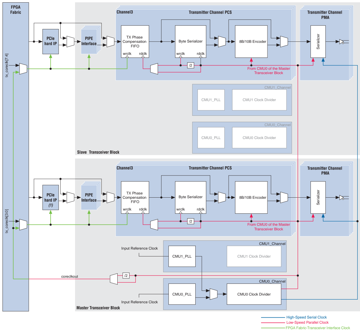
Figure 2-7. Transmitter Datapath Clcking in a \times 8 Bonded Configuration
