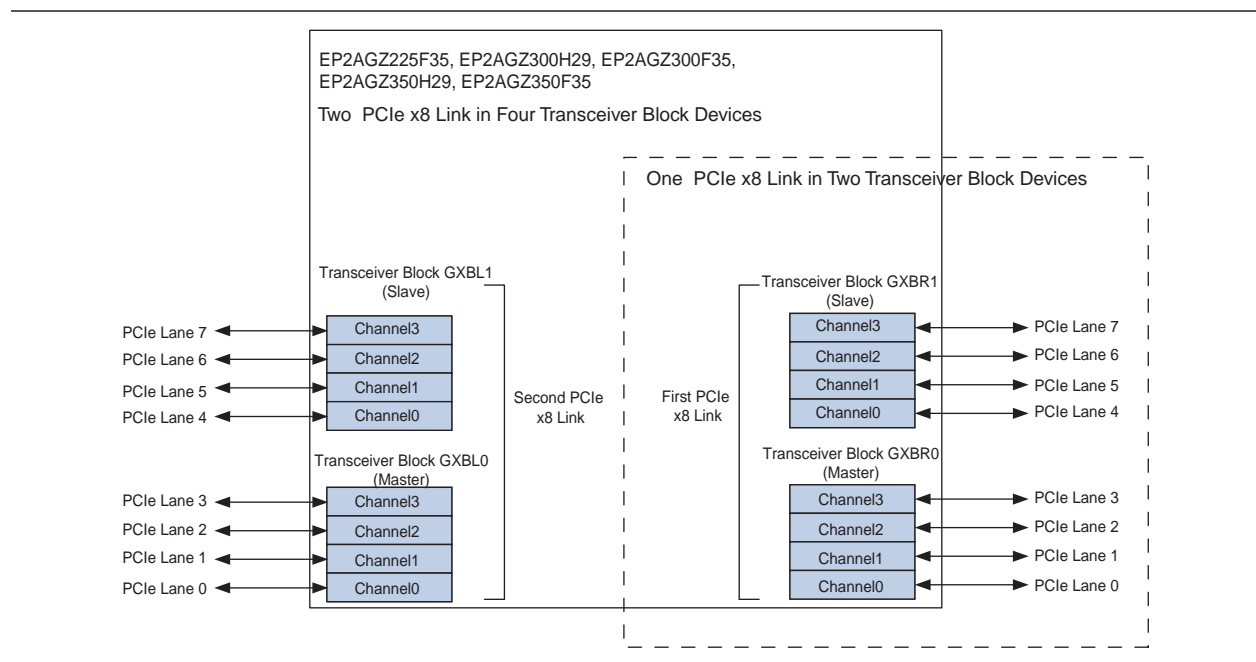
Figure 2-11. One PCIe x8 Link in Two Transceiver Block Devices and Two PCIe x8 Links in Four Transceiver Block Arria II GZ Devices
