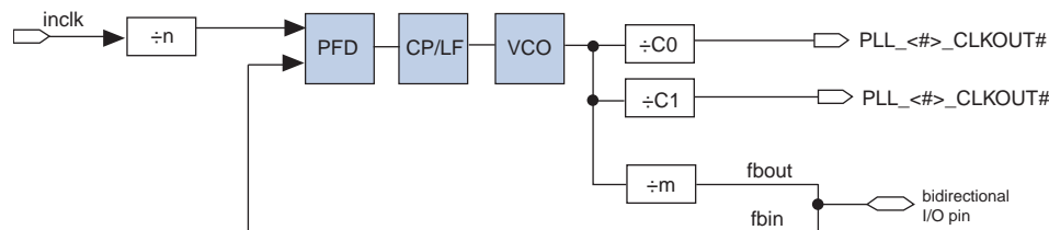
Figure 5–24. ZDB Mode in PLLs for Arria II GZ Devices
