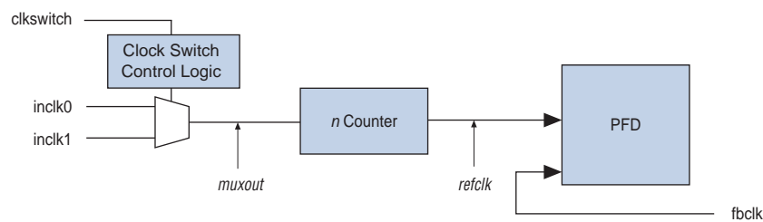
Figure 5-33. Manual Clock Switchover Circuitry in PLLs for Arria II Devices
