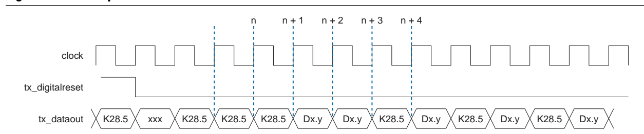
Figure 1-59. Example of Reset Condition in GIGE Mode
