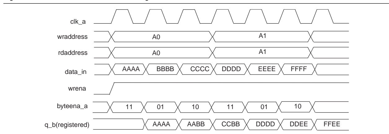
Figure 3–24. MLABs Mixed-Port Read-During-Write: Don't Care Mode
