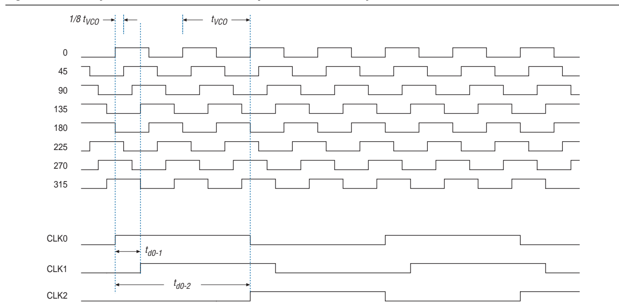
Figure 5-29. Delay Insertion with VCO Phase Output and Counter Delay Time for Arria II Devices
