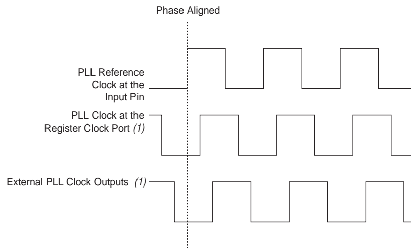
Figure 5-22. Phase Relationship Between PLL Clocks in No-Compensation Mode for Arria II Devices
