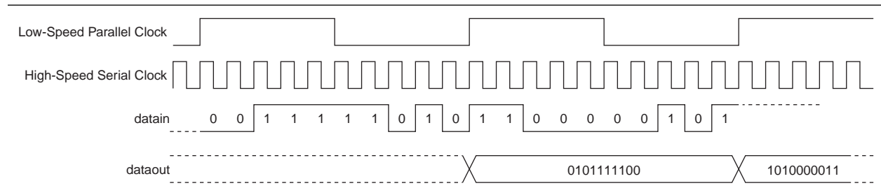
Figure 1-30. 10-Bit Deserializer Bit Order
