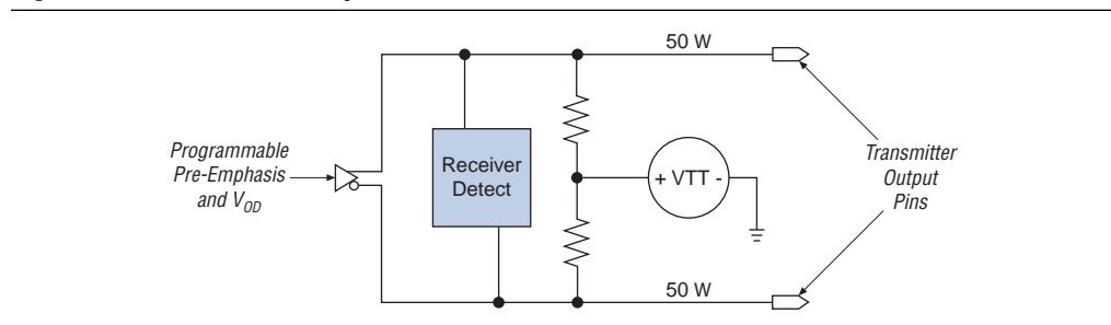
Figure 1-22. Transmitter Output Buffer
