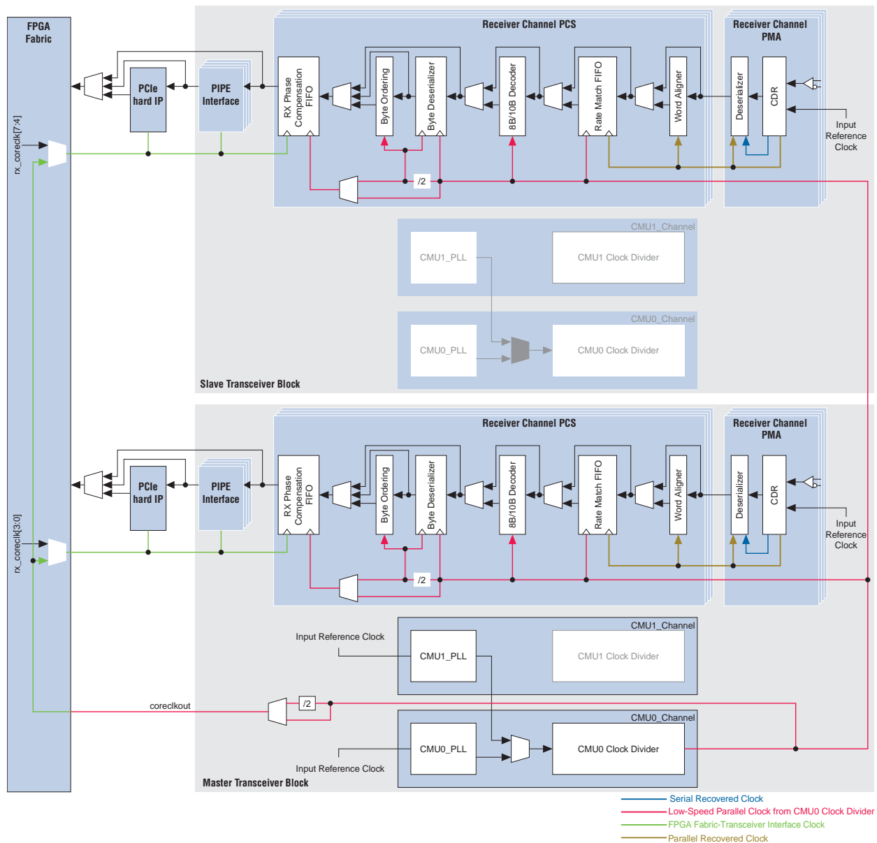
Figure 2-17. Receiver Datapath Clocking in \times 8 Bonded Channel Configuration
