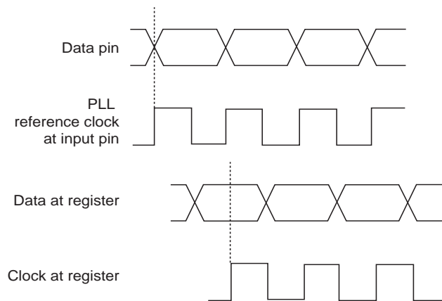
Figure 5-21. Source-Synchronous Mode for LVDS Compensation for Arria II Devices
