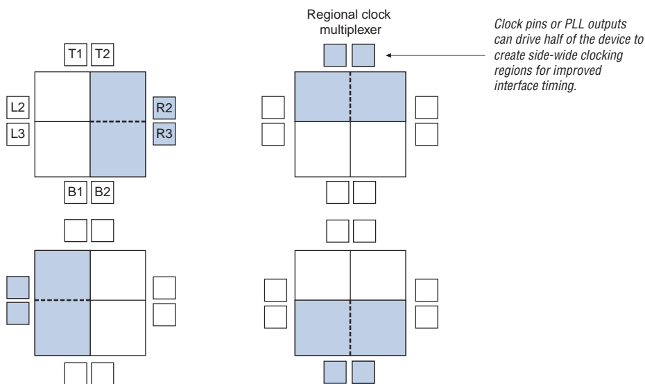
Figure 5-7. Device Dual-Regional Clock Region for Arria II GZ Devices
