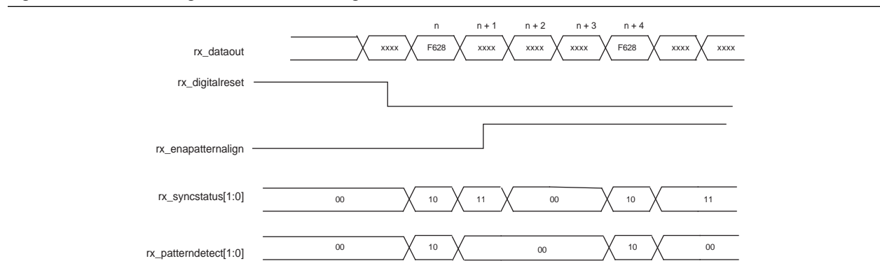
Figure 1–36. Manual Alignment Mode Word Aligner in 16-Bit PMA-PCS Interface Modes
