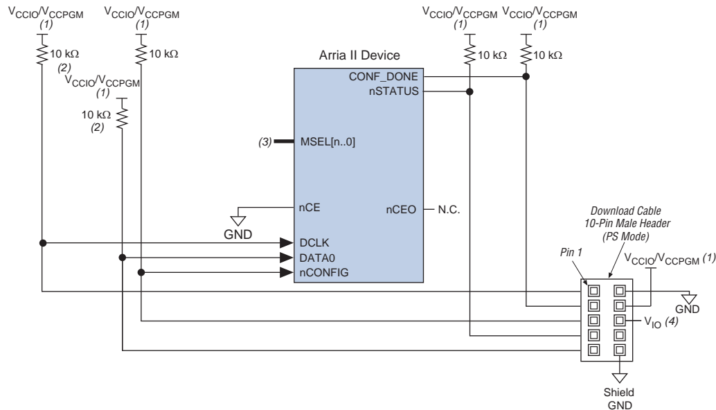
Figure 9-14. PS Configuration Using a USB-Blaster, EthernetBlaster, EthernetBlaster II, MasterBlaster, ByteBlaster II, or ByteBlasterMV Cable
