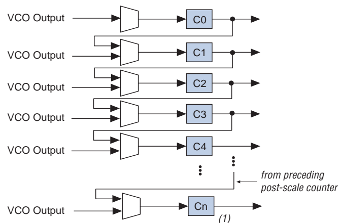
Figure 5-28. Counter Cascading for Arria II Devices
