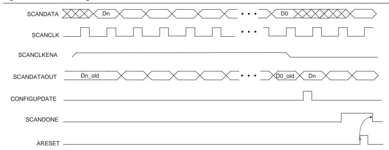
Figure 5-36. PLL Reconfiguration Waveform for Arria II Devices
