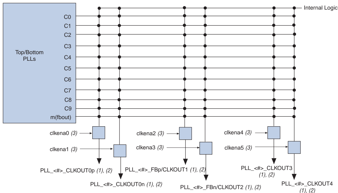
Figure 5-18. External Clock Outputs for Top and Bottom PLLs in Arria II GZ Devices
