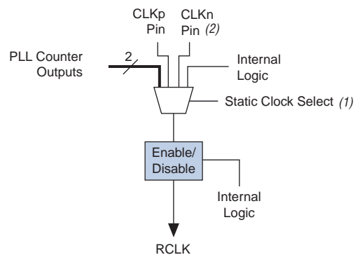
Figure 5-10. RCLK Control Block for Arria II GZ Devices
