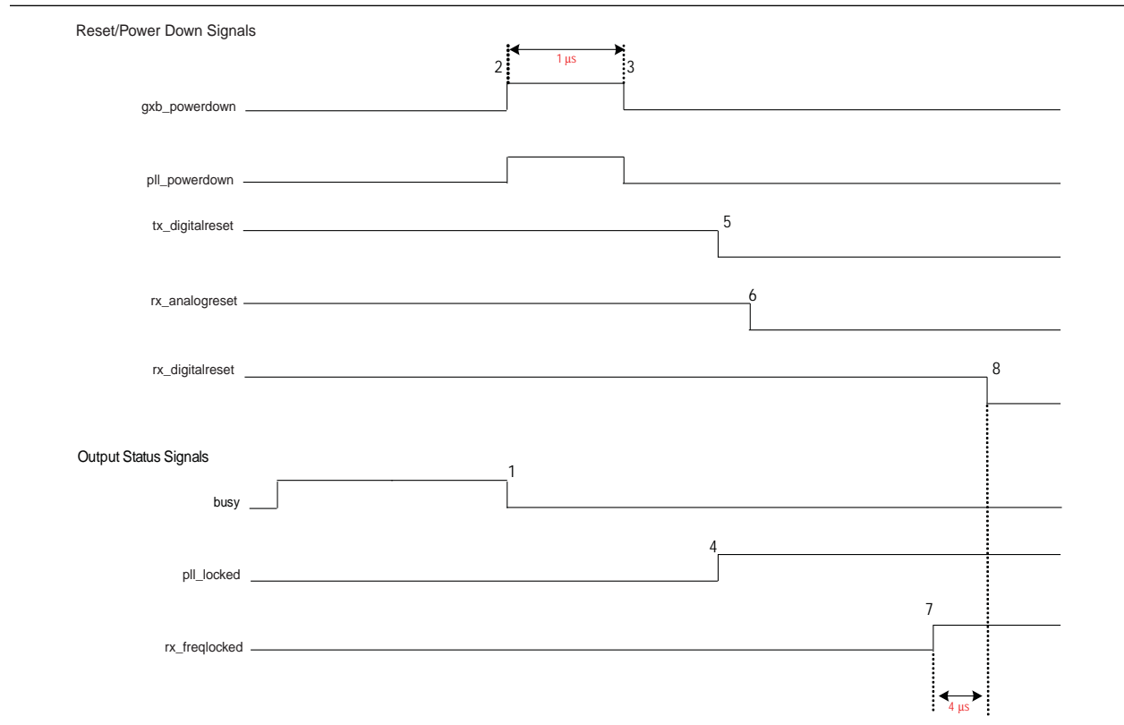
Figure 4-13. Sample Reset Sequence of Four Receiver and Transmitter Channels—Receiver CDR in Automatic Lock Mode with Optional gxb_powerdown Signal
