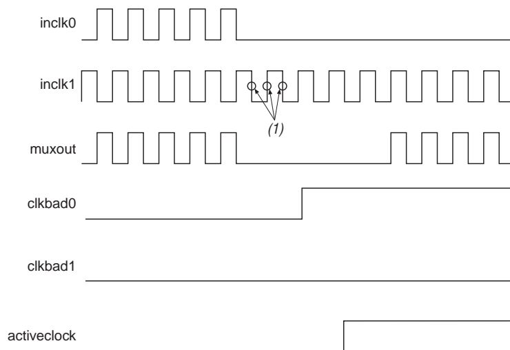
Figure 5-31. Automatic Switchover Upon Loss of Clock Detection for Arria II Devices
