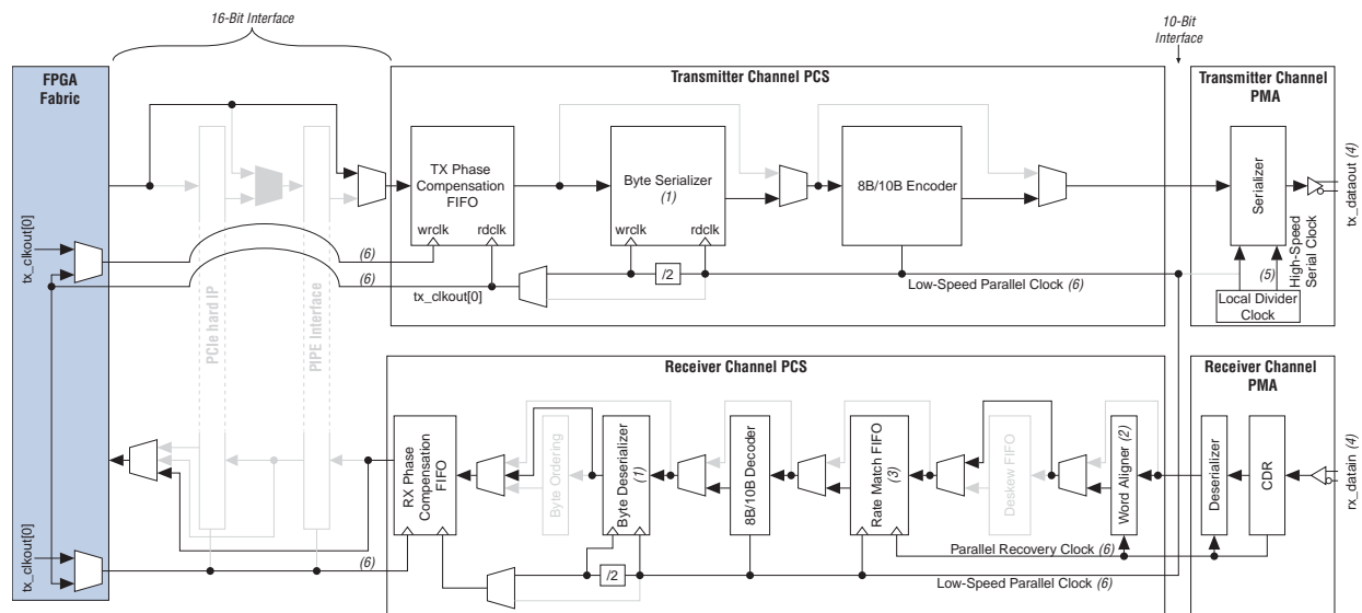
Figure 1-71. Serial RapidIO Mode Datapath
