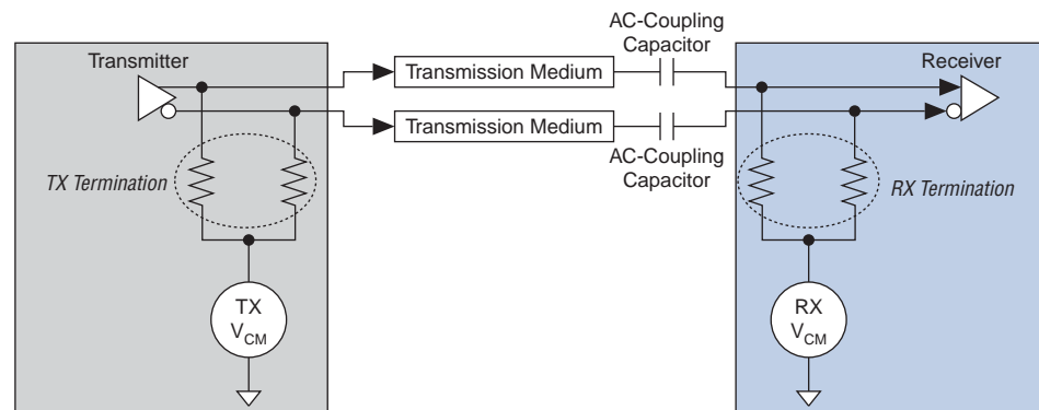
Figure 1-25. AC-Coupled Link
