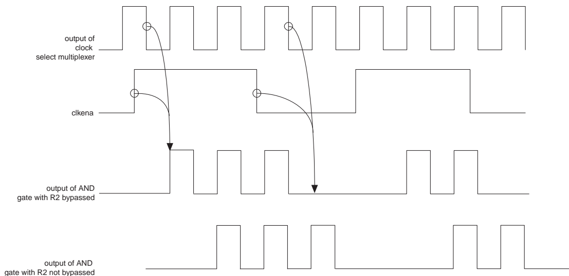
Figure 5-13. clkena Signals for Arria II Devices
