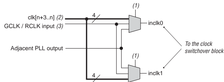
Figure 5-15. Clock Input Multiplexer Logic for Arria II GZ devices
