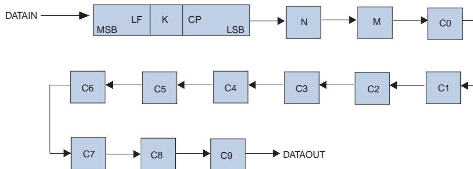
Figure 5-38. Scan Chain Order of PLL Components for Top and Bottom of Arria II GZ PLLs (Note 1)
