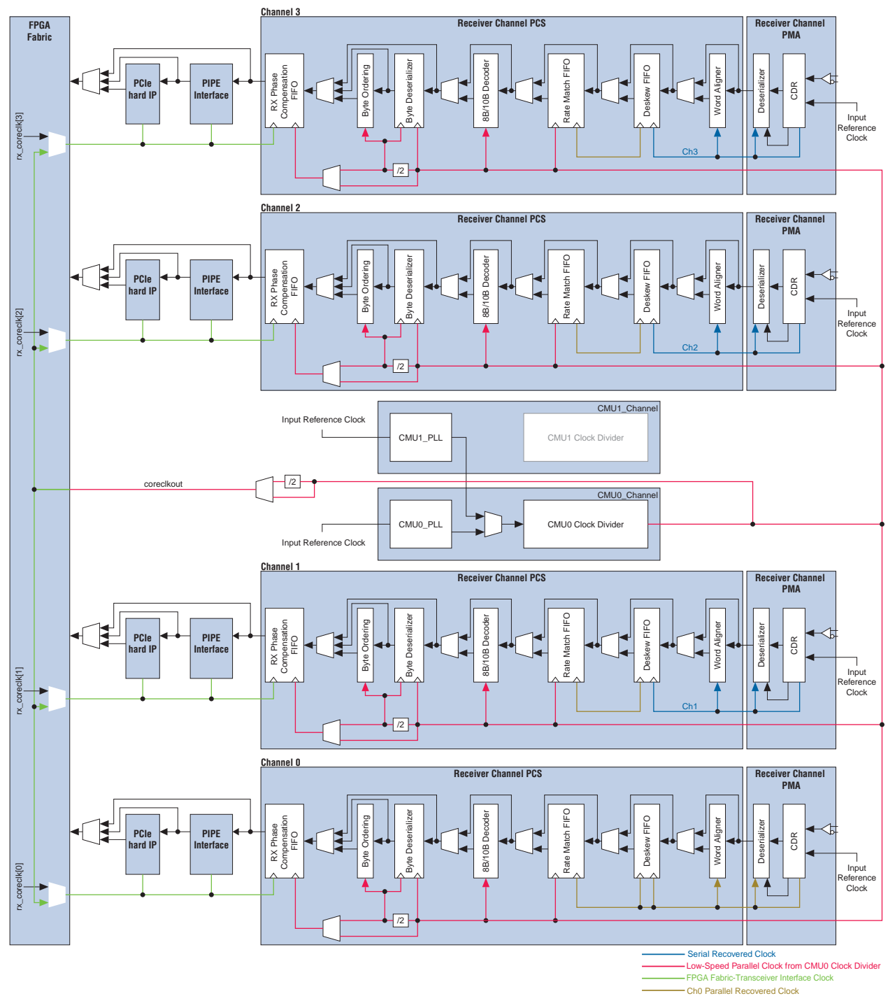
Figure 2-15. Receiver Datapath Clocking in ×4 Bonded Channel Configuration with Deskew FIFO
