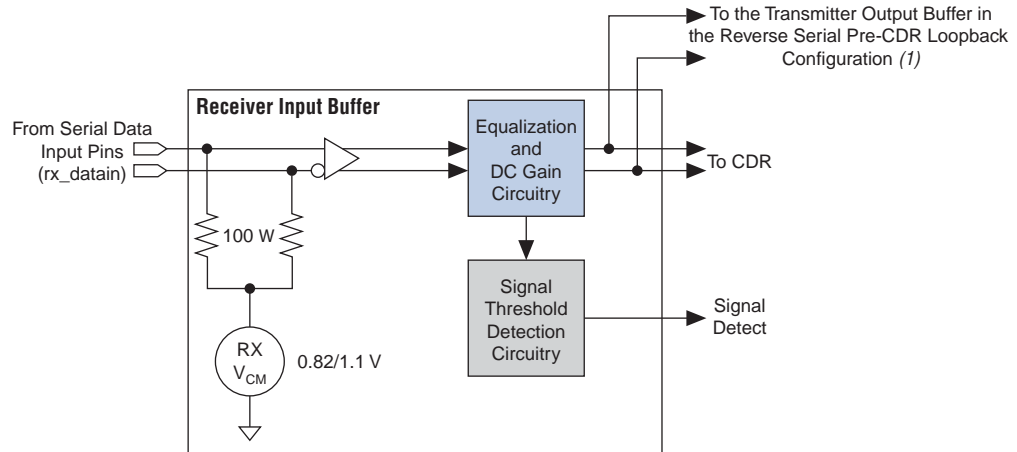
Figure 1-24. Receiver Input Buffer
