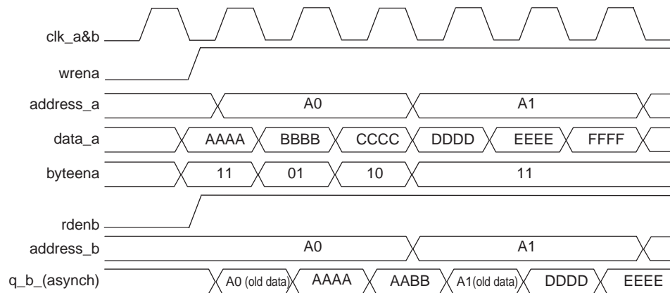
Figure 3–25. M9K and M144K Mixed Port Read During Write: Old Data Mode
