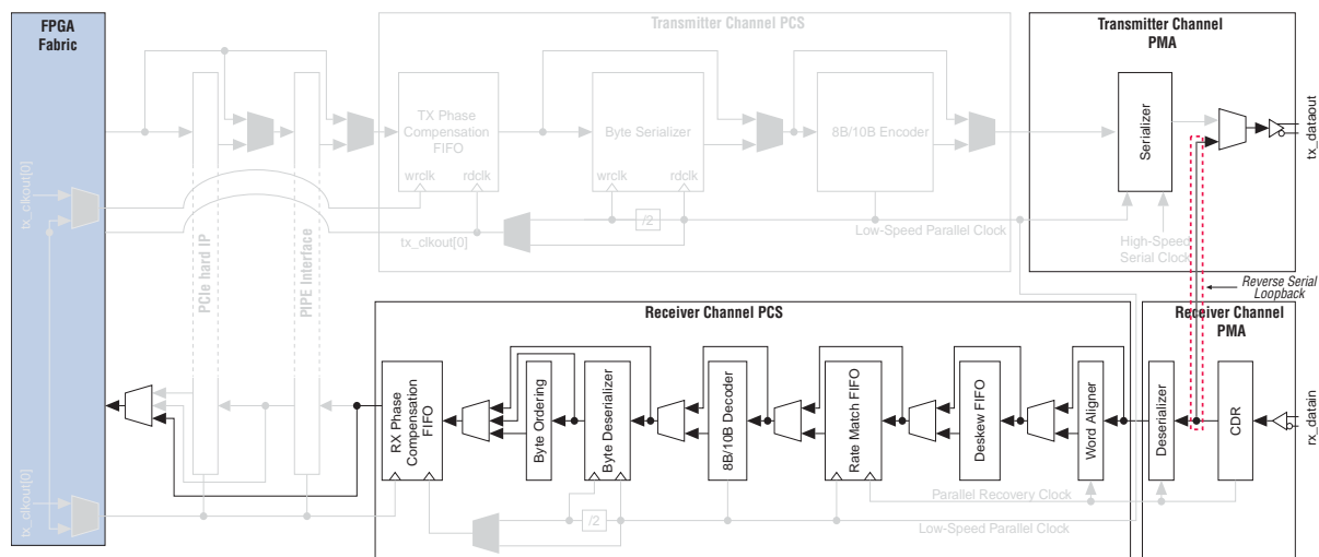
Figure 1-82. Reverse Serial Loopback Datapath (Note 1)
