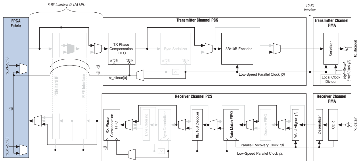
Figure 1-57. GIGE Functional Mode
