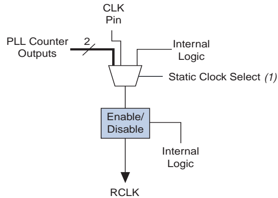
Figure 5-9. RCLK Control Block for Arria II GX Devices
