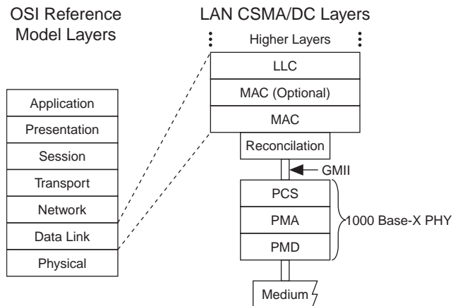
Figure 1-56. 1000 Base-X PHY in a GIGE OSI Reference Model
