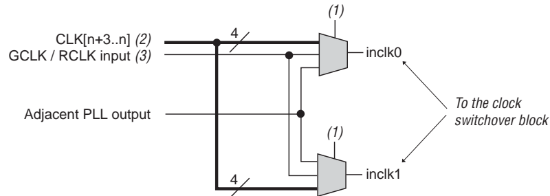
Figure 5-14. Clock Input Multiplexer Logic for Arria II GX PLLs
