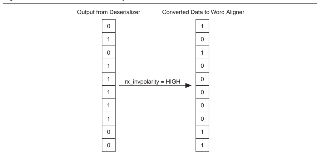
Figure 1-32. 10-Bit Receiver Polarity Inversion
