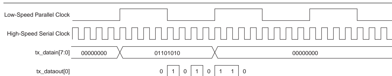
Figure 1-21. Serializer Bit Order (Note 1)
