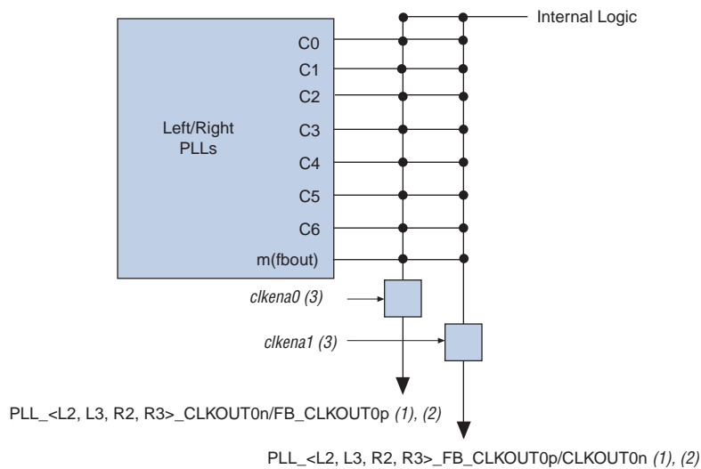
Figure 5–19. External Clock Outputs for Left and Right PLLs in Arria II GZ Devices
