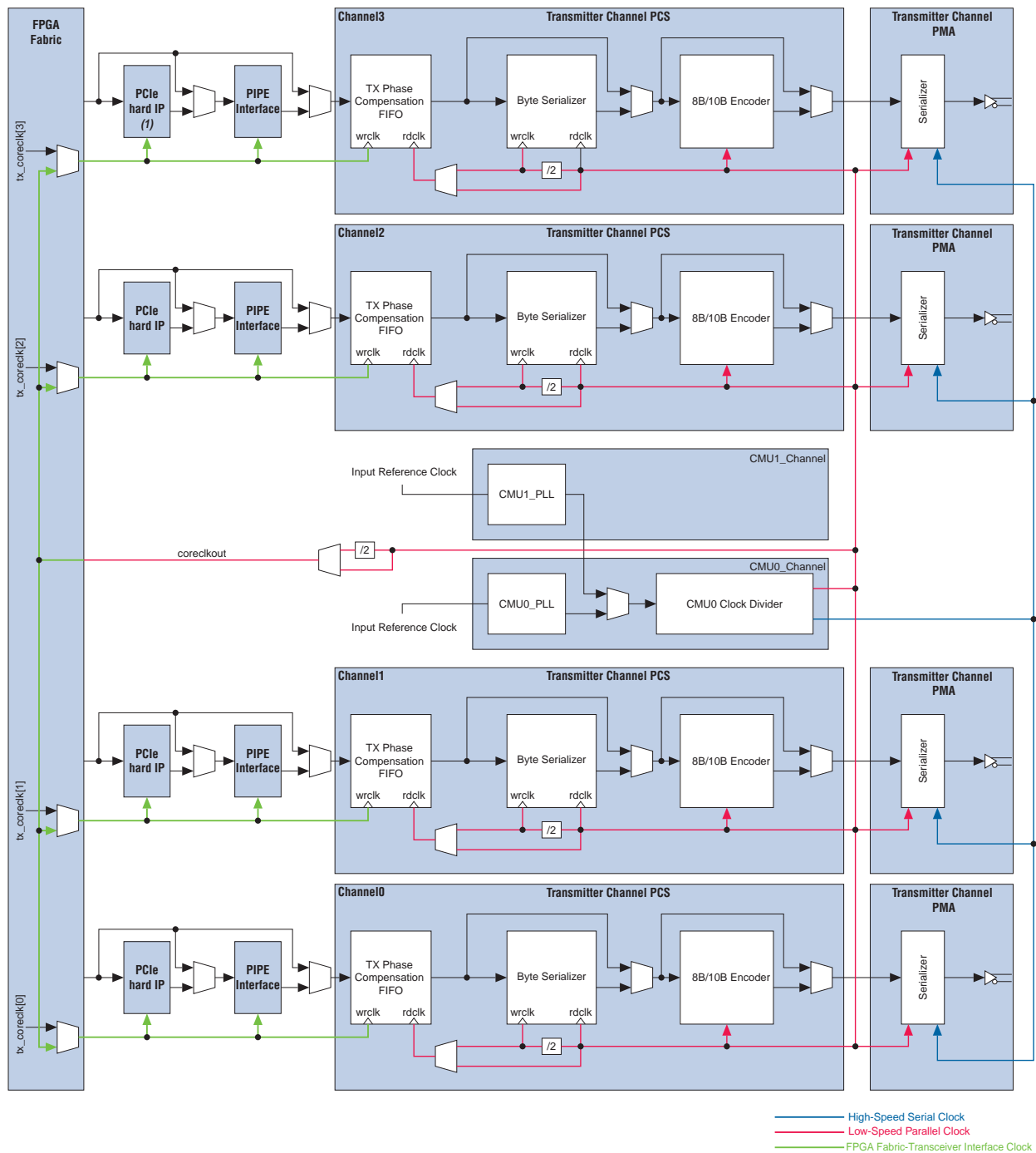
Figure 2-6. Transmitter Datapath Clocking in \times 4 Bonded Configurations
