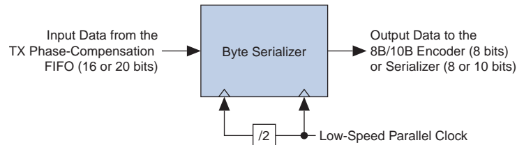
Figure 1-13. Byte Serializer Datapath for Arria II GX Devices
