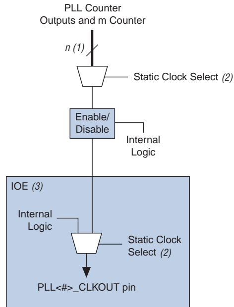
Figure 5-11. External PLL Output Clock Control Block Arria II Devices
