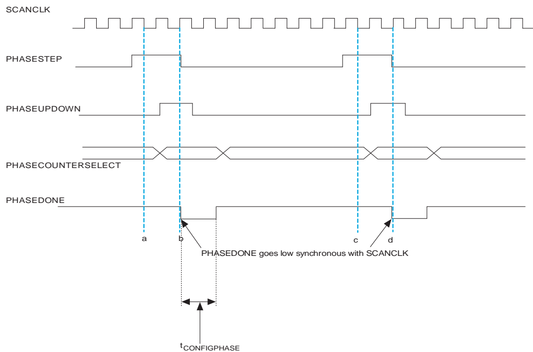
Figure 5-40. Dynamic Phase Shifting Waveform for Arria II Devices
