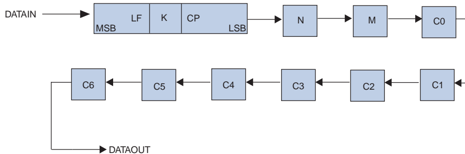
Figure 5-37. Scan Chain Order of PLL Components for Arria II GX PLLs
