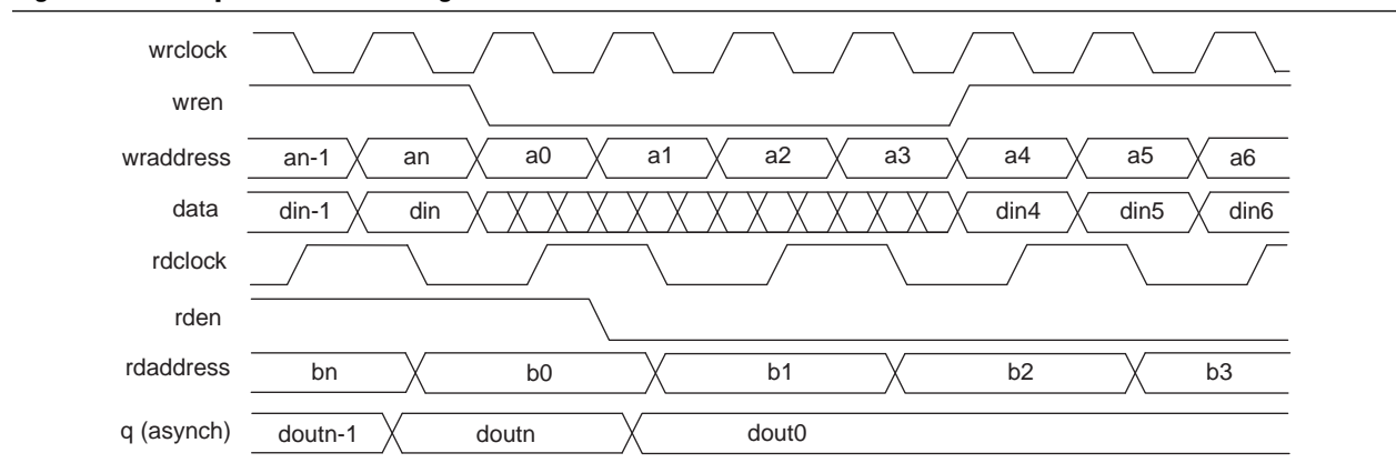
Figure 3-14. Simple Dual-Port Timing Waveforms for MLABs
