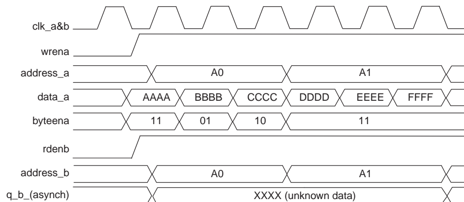
Figure 3–26. M9K and M144K Mixed-Port Read-During-Write: Don't Care Mode
