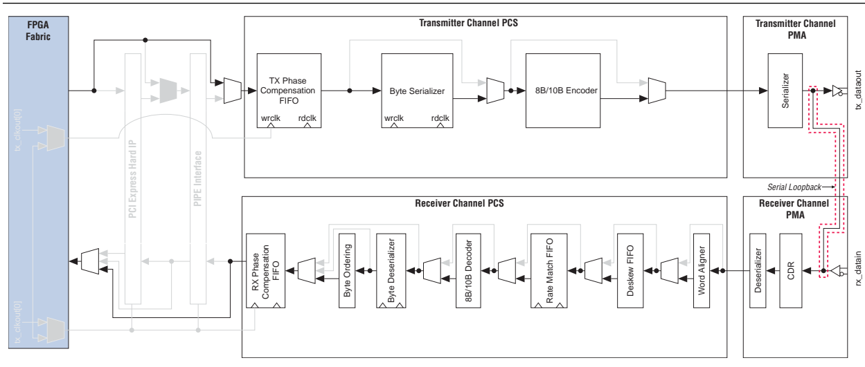
Figure 1-81. Serial Loopback Datapath
