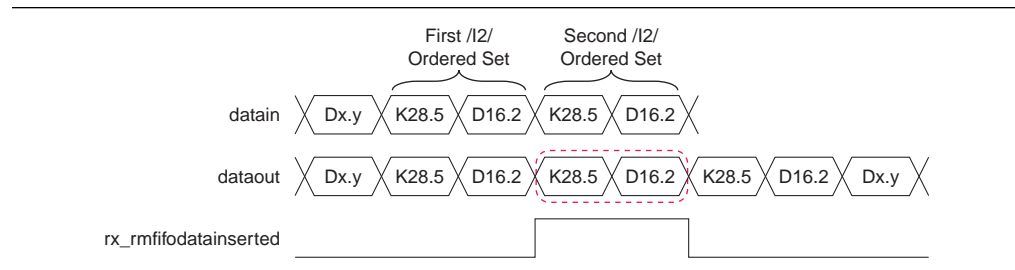
Figure 1-61. Example of Rate Match Insertion in GIGE Mode
