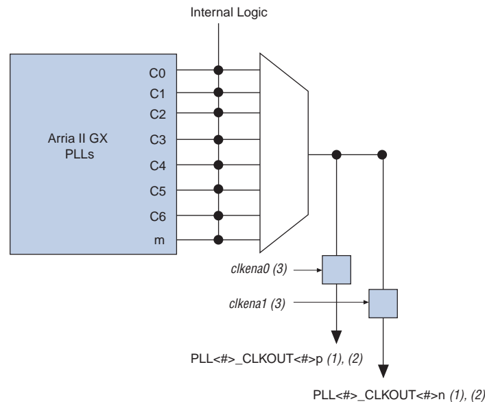
Figure 5-17. External Clock Outputs for Arria II GX PLLs
