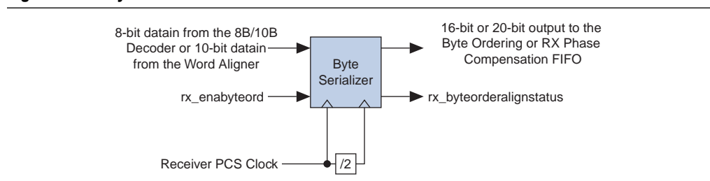
Figure 1-43. Byte Deserializer
