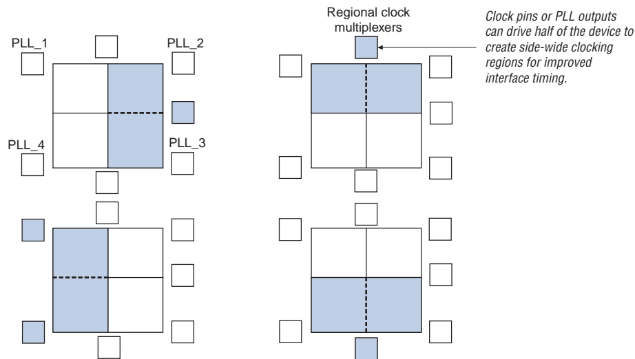
Figure 5-6. Device Dual-Regional Clock Region for Arria II GX Devices
