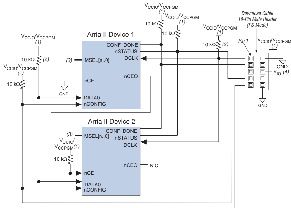
Figure 9-15. Multi-Device PS Configuration Using a USB-Blaster, EthernetBlaster, EthernetBlaster II, MasterBlaster, ByteBlaster II, or ByteBlasterMV Cable
