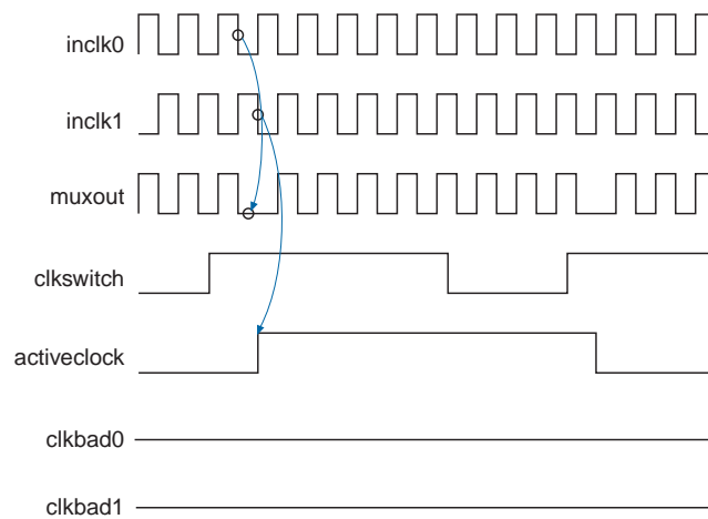
Figure 5-32. Clock Switchover with the clkswitch (Manual) Control for Arria II Devices (Note 1)
