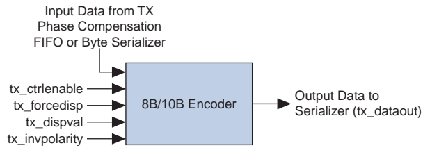
Figure 1-14. 8B/10B Encoder
