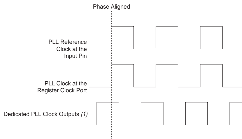
Figure 5-23. Phase Relationship Between PLL Clocks in Normal Mode for Arria II Devices
