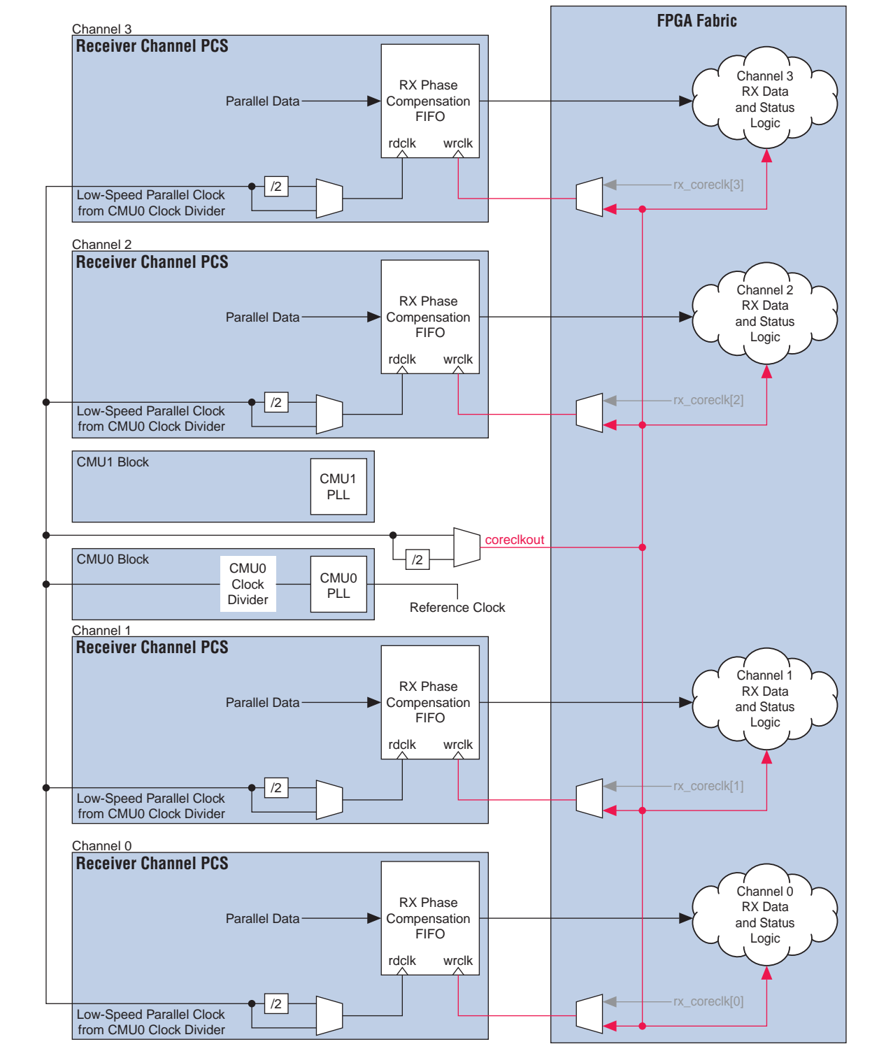
Figure 2-27. FPGA Fabric-Receiver Interface Clocking in an \times 4 Bonded Channel Configuration
