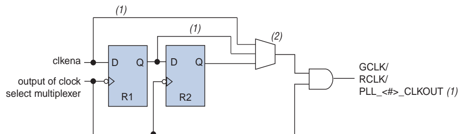
Figure 5-12. clkena Implementation for Arria II Devices
