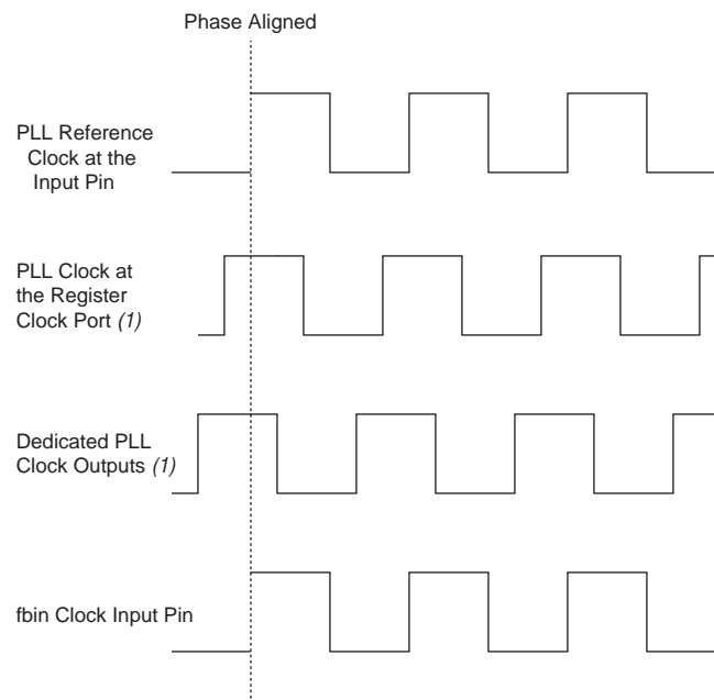
Figure 5-26. Phase Relationship Between the PLL Clocks in External Feedback Mode for Arria II Devices
