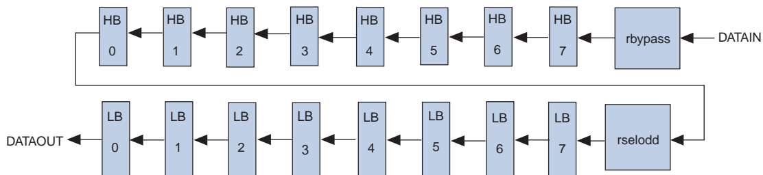
Figure 5-39. Scan Chain Bit-Order Sequence for Post-Scale Counters in Arria II PLLs
