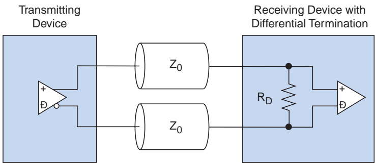
Figure 4–70. LVDS Input Differential On-Chip Termination
