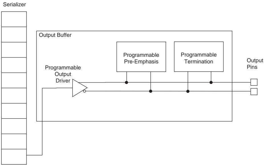
Figure 2–6. Output Buffer
