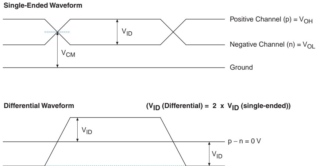
Figure 2–7. V_{OD} Differential
