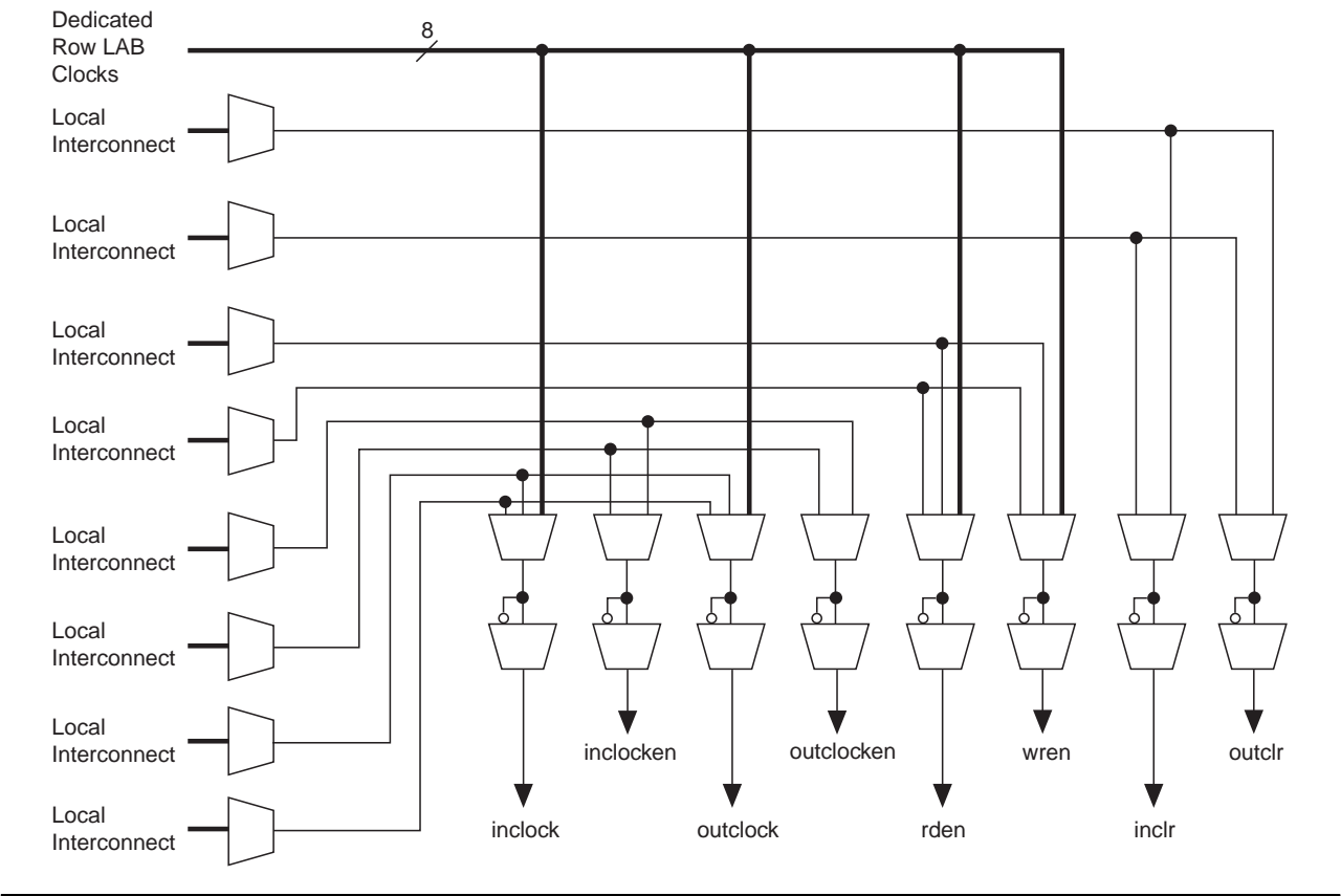
Figure 4–14. M512 RAM Block Control Signals
