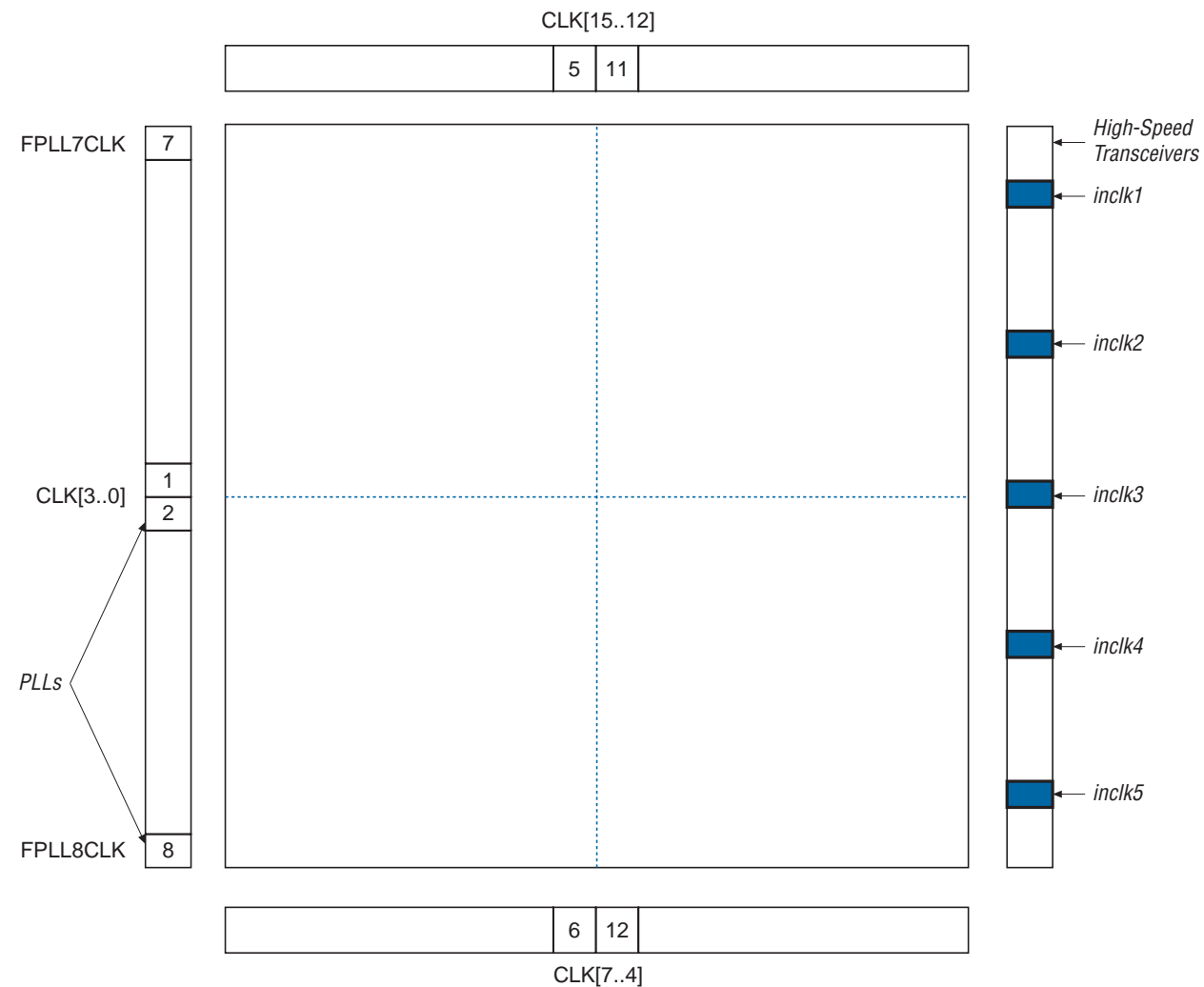
Figure 4–48. PLL Floorplan
