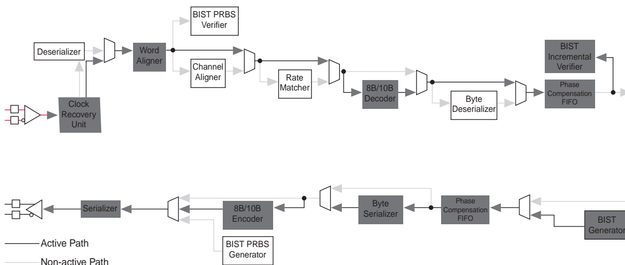
Figure 2–25. BIST Incremental Data Path
