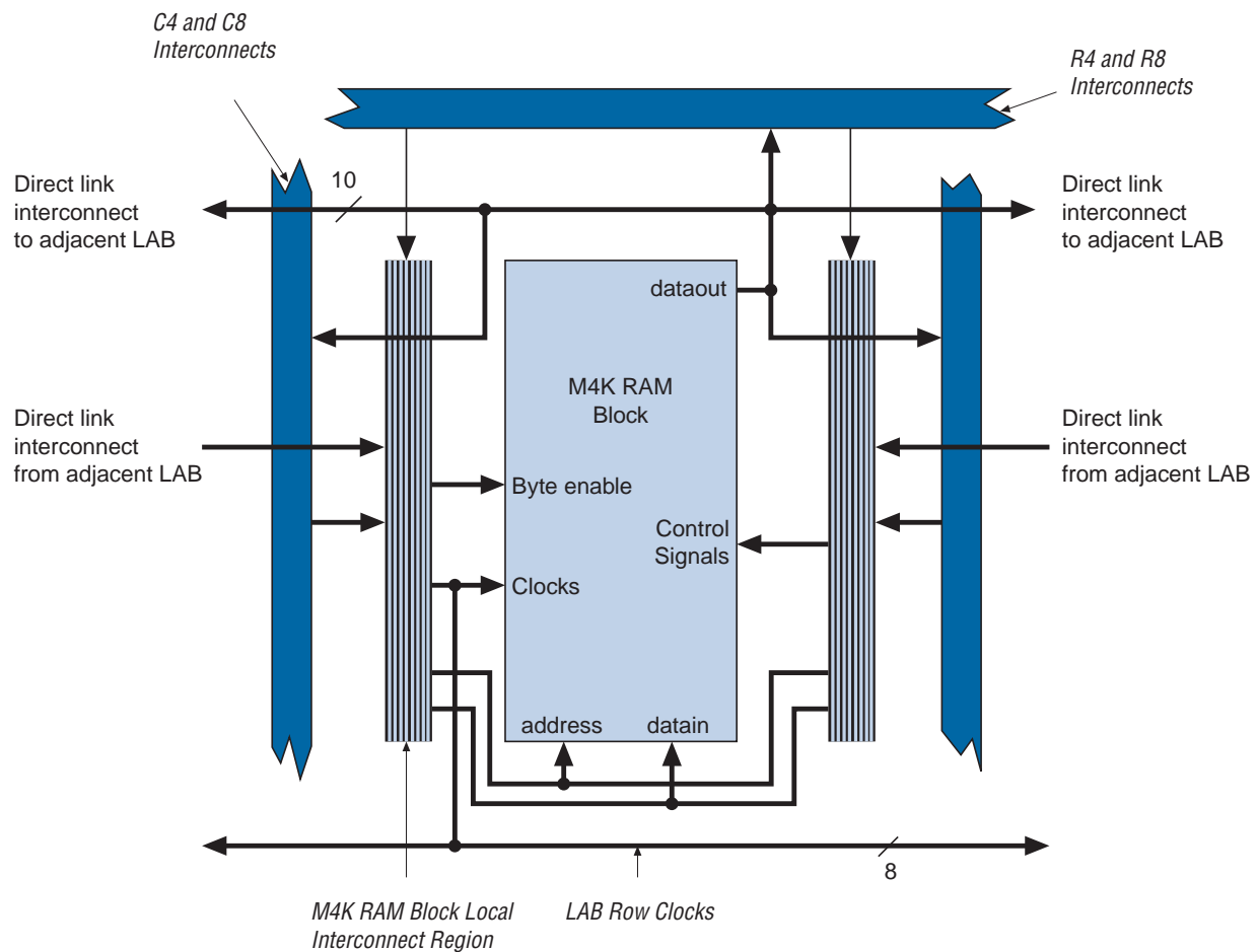
Figure 4–17. M4K RAM Block LAB Row Interface
