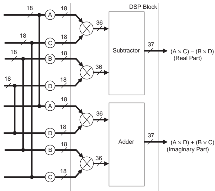
Figure 4-37. Two-Multipliers Adder Mode Implementing Complex Multiply
