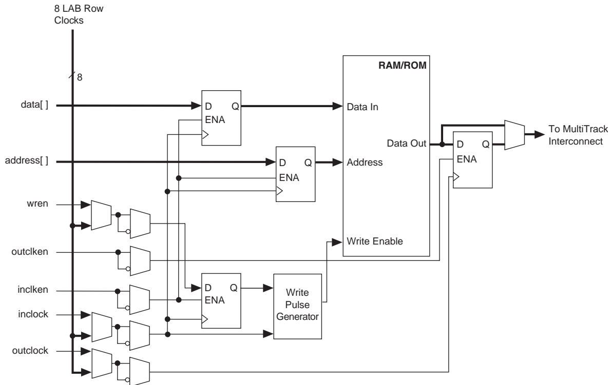
Figure 4–27. Single-Port Mode
