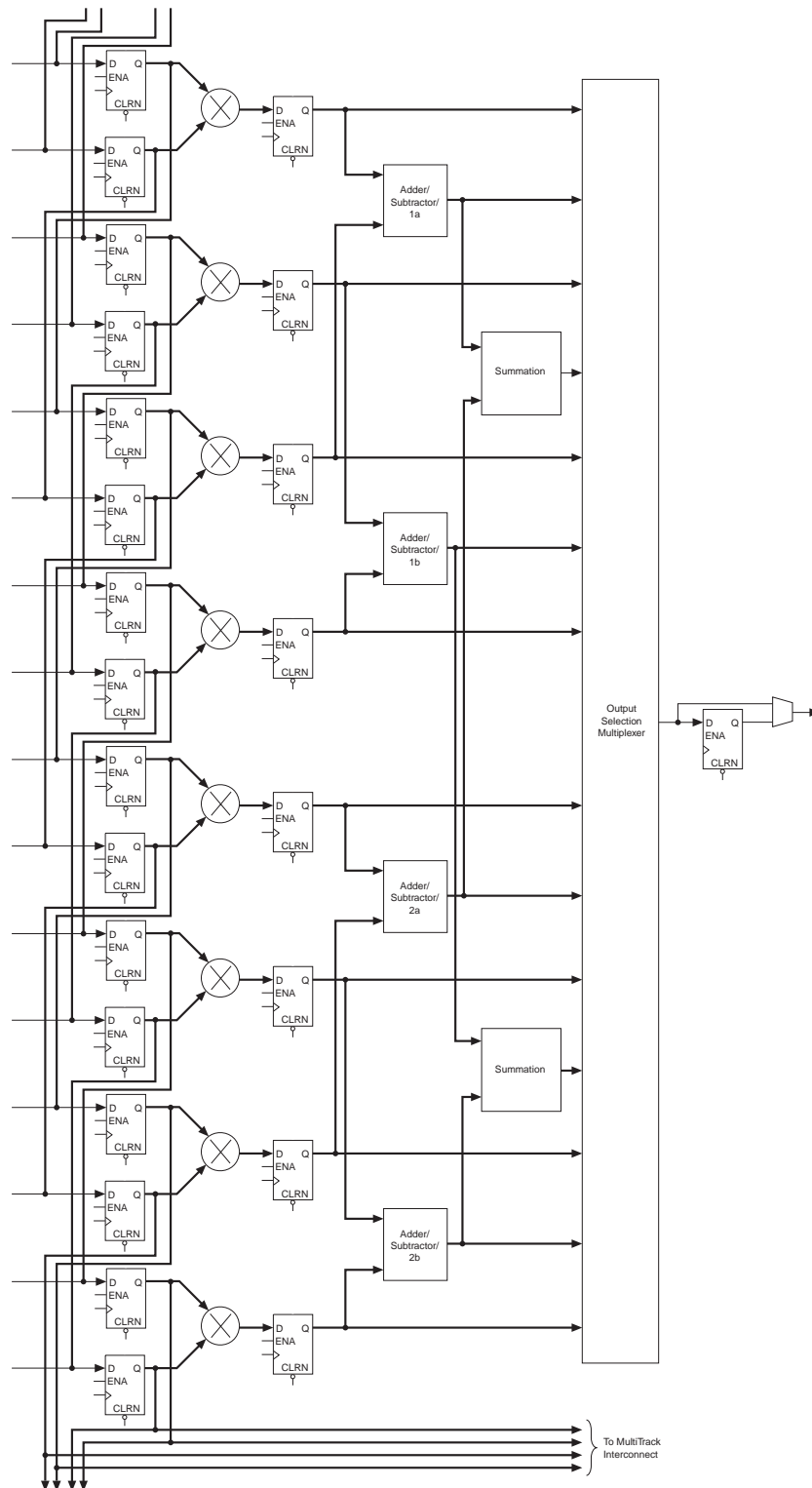
Figure 4-30. DSP Block Diagram for 9 \times 9 -Bit Configuration
