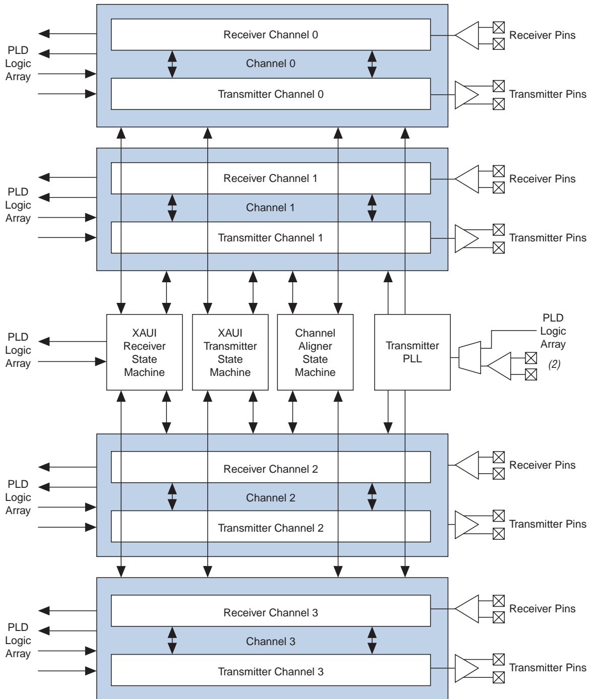
Figure 2–1. Stratix GX Transceiver Block Note (1)
