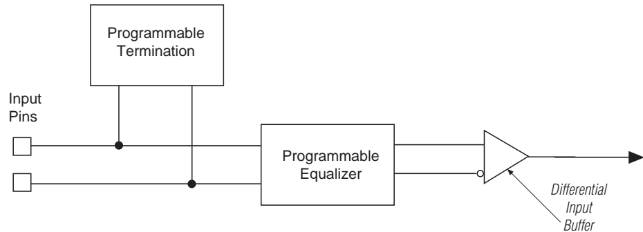
Figure 2–10. Receiver Input Buffer
