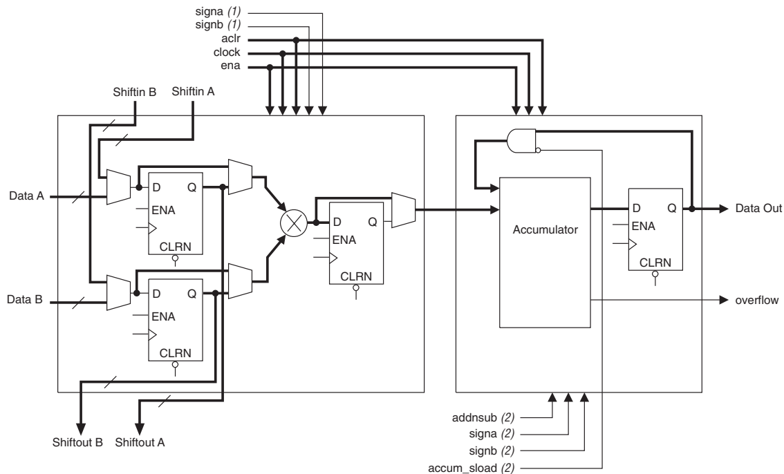
Figure 4–36. Multiply-Accumulate Mode
