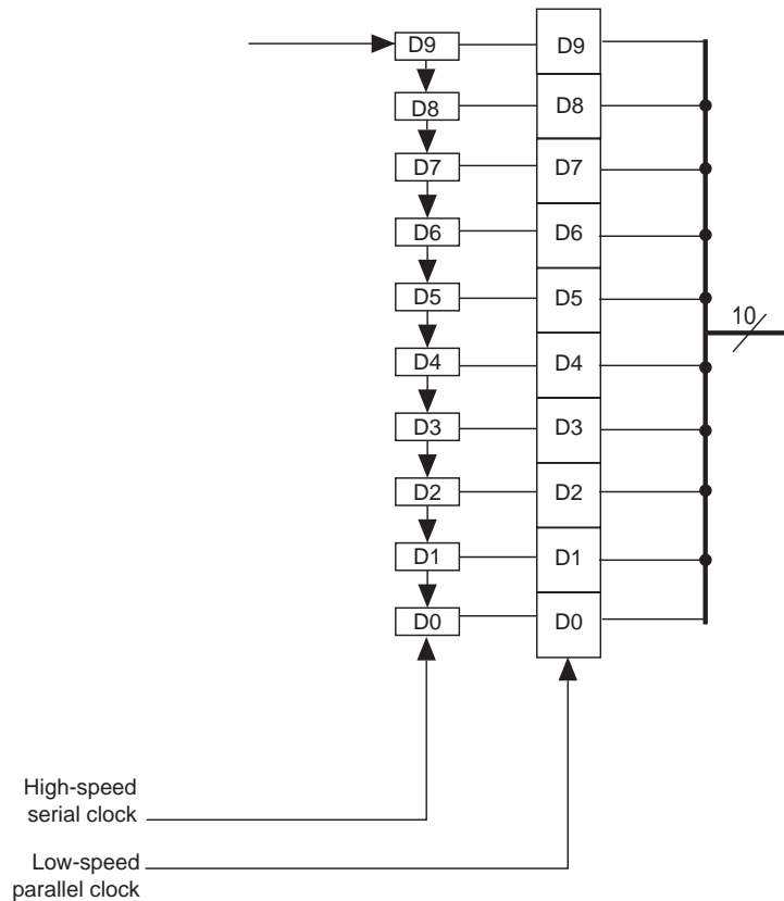
Figure 2–14. Deserializer
