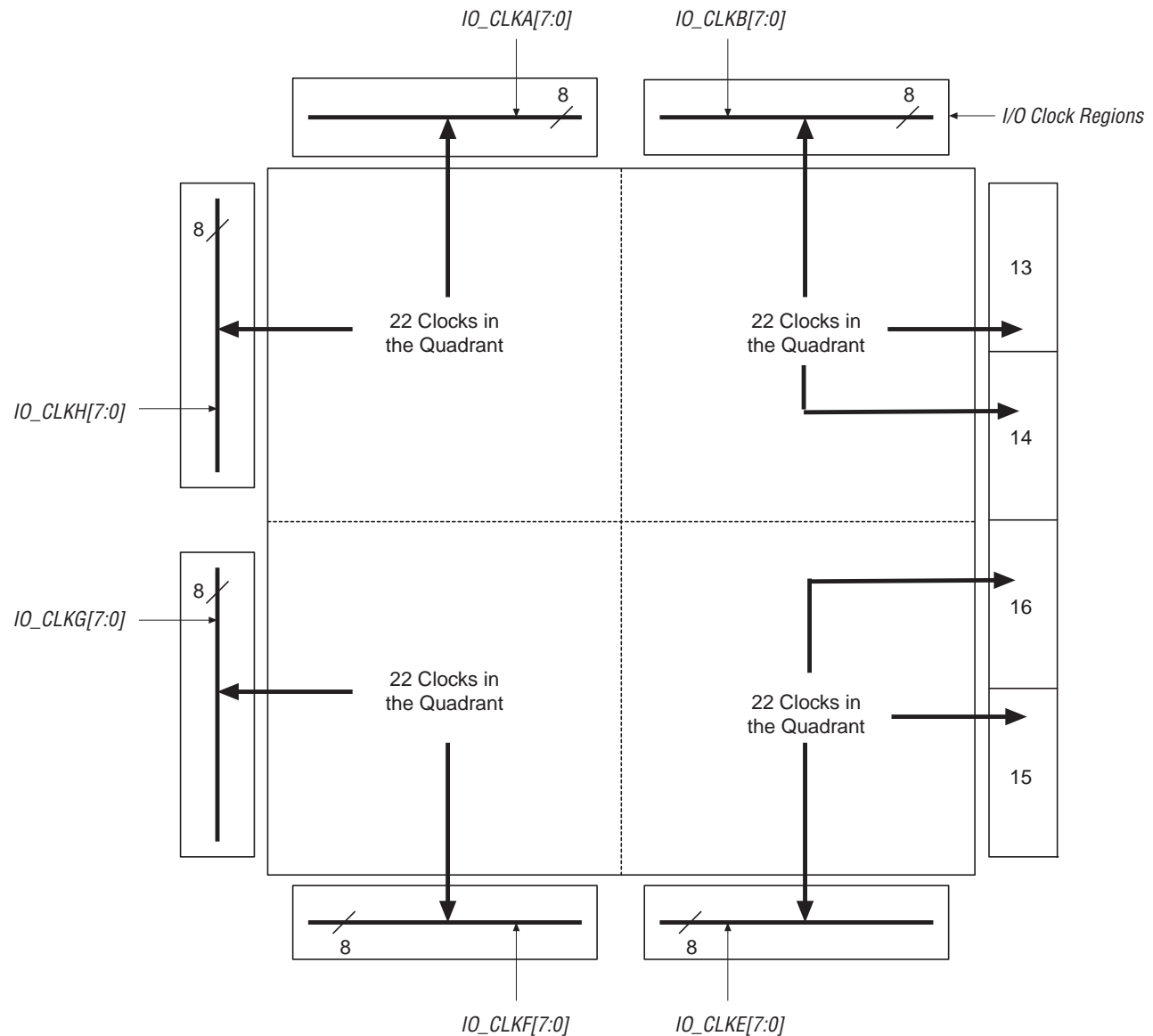
Figure 4–46. EP1SGX25 & EP1SGX10 Device I/O Clock Groups
