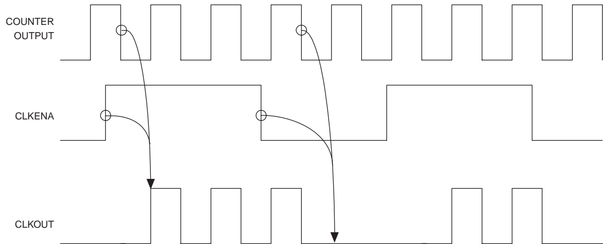
Figure 4–56. extclkena Signals
