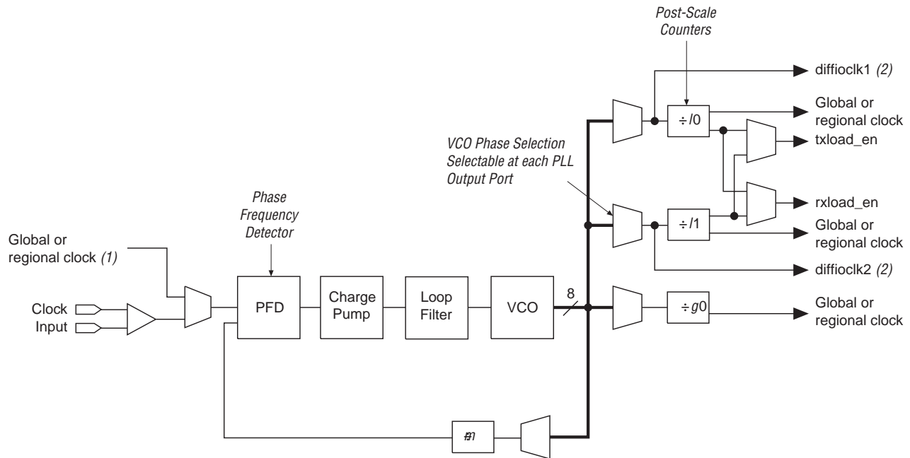
Figure 4–57. Stratix GX Device Fast PLL
