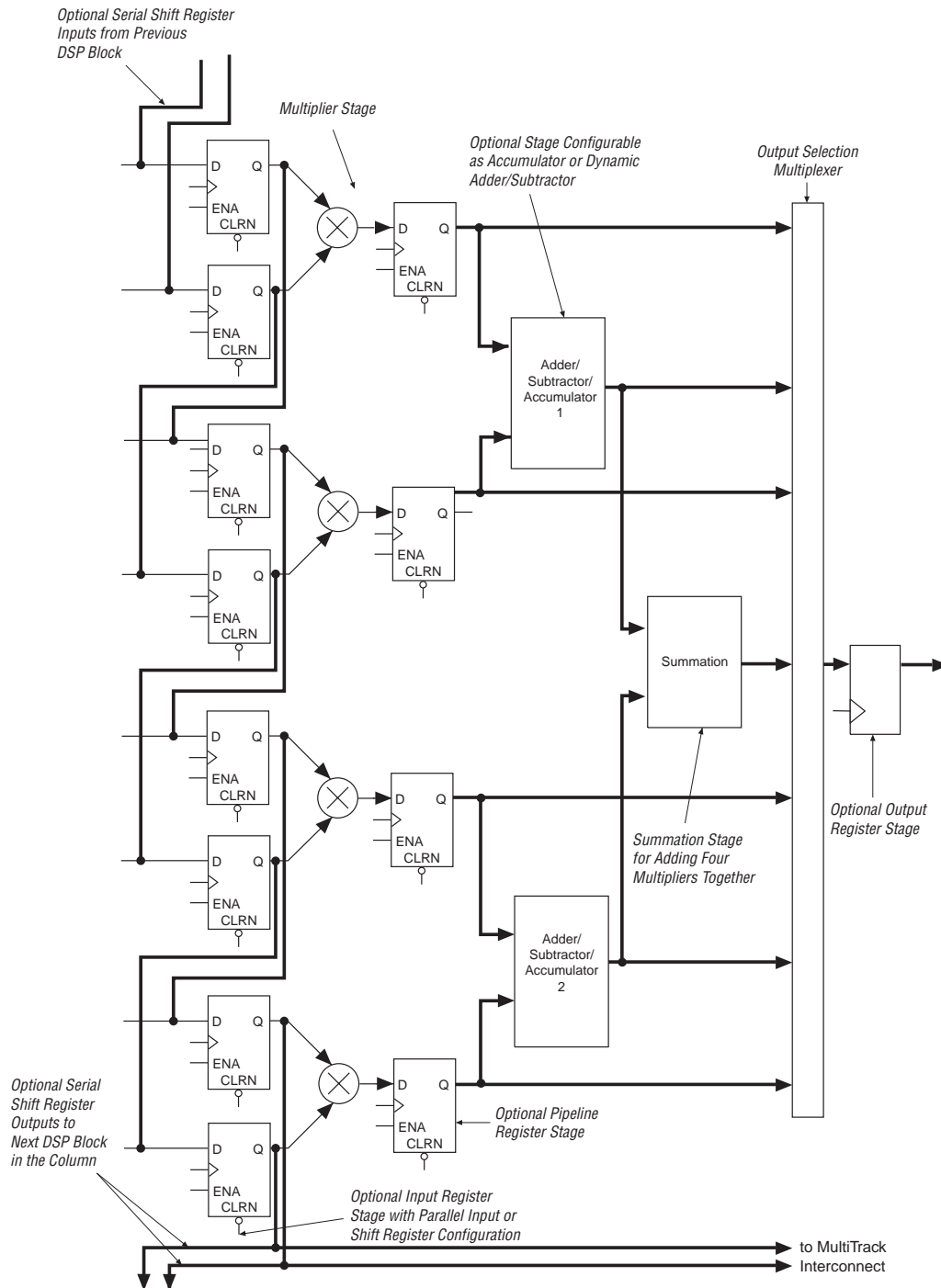
Figure 4–29. DSP Block Diagram for 18 \times 18 -Bit Configuration
