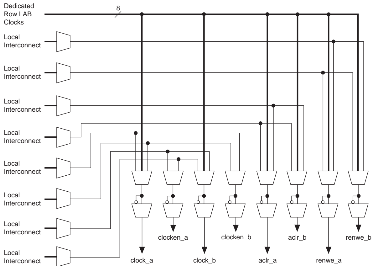
Figure 4–18. M-RAM Block Control Signals
