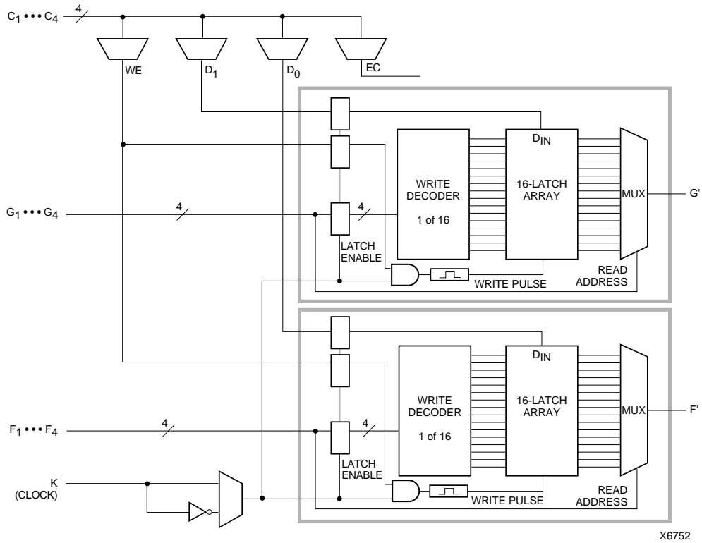
Figure 3: 16x2 (or 16x1) Edge-Triggered Single-Port RAM
