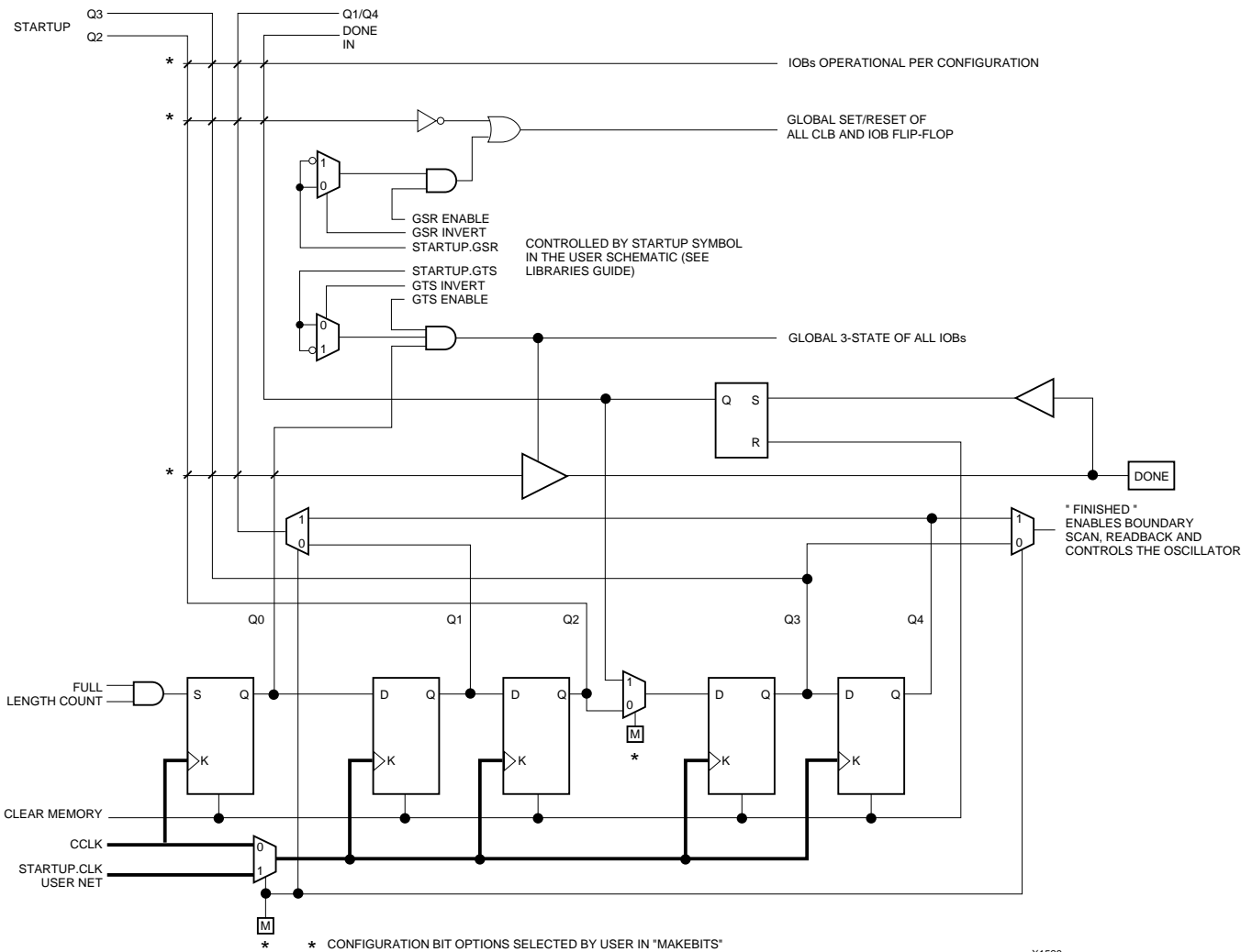
Figure 50: Start-up Logic
