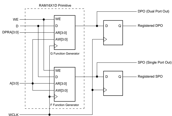
Figure 6: XC4000-Series Dual-Port RAM, Simple Model
