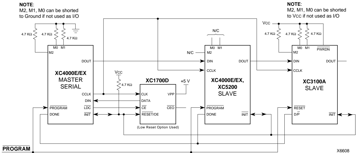
Figure 55: Slave Serial Mode Circuit Diagram
