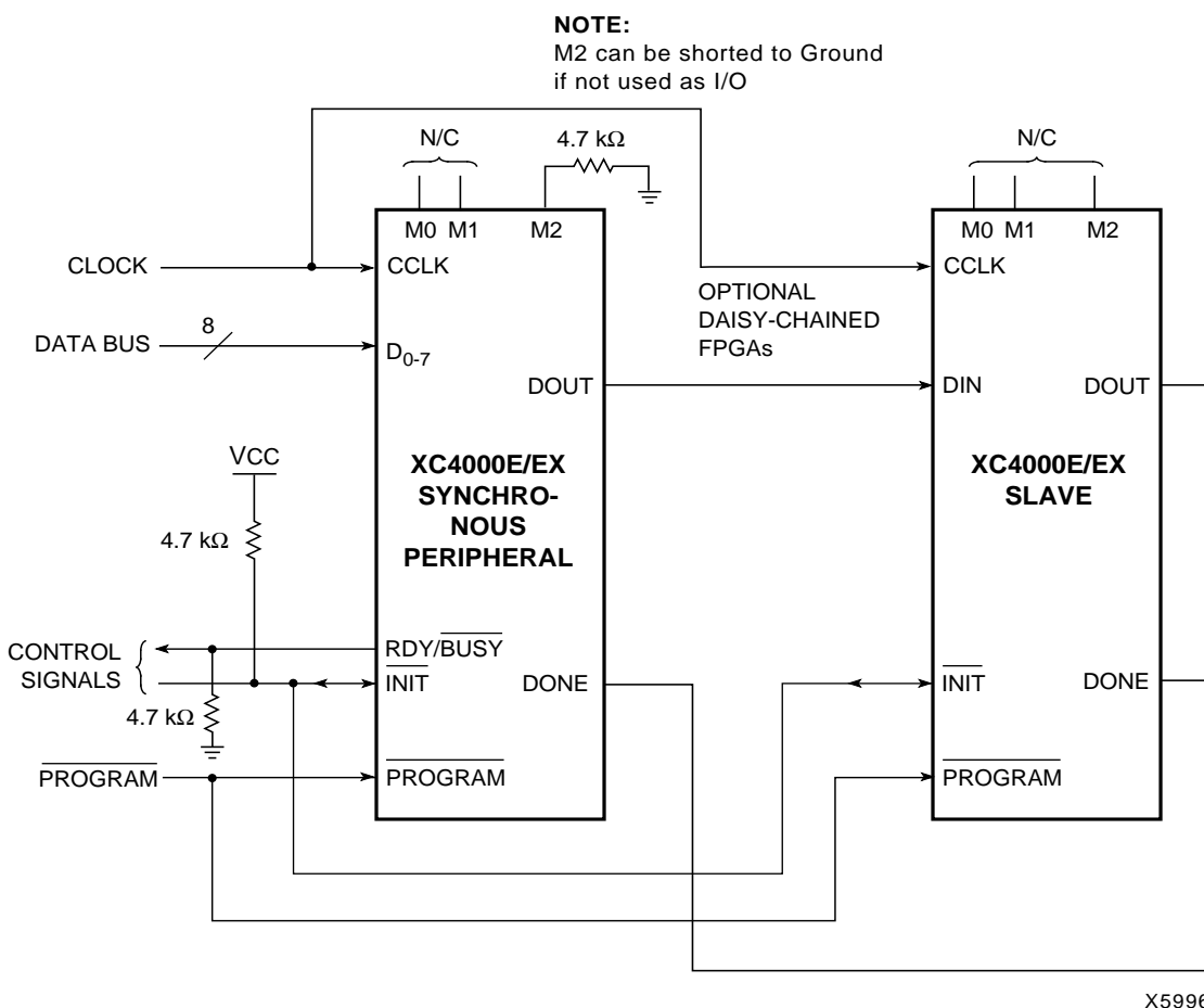
Figure 59: Synchronous Peripheral Mode Circuit Diagram
