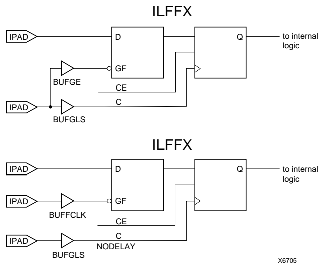
Figure 18: Examples Using XC4000EX Fast Capture Latch
