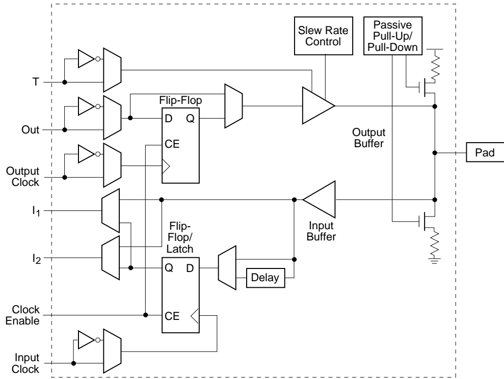
Figure 16: Simplified Block Diagram of XC4000E IOB
