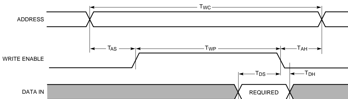
Figure 8: Level-Sensitive RAM Write Timing
