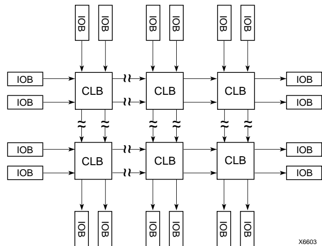
Figure 31: XC4000EX Direct Interconnect
