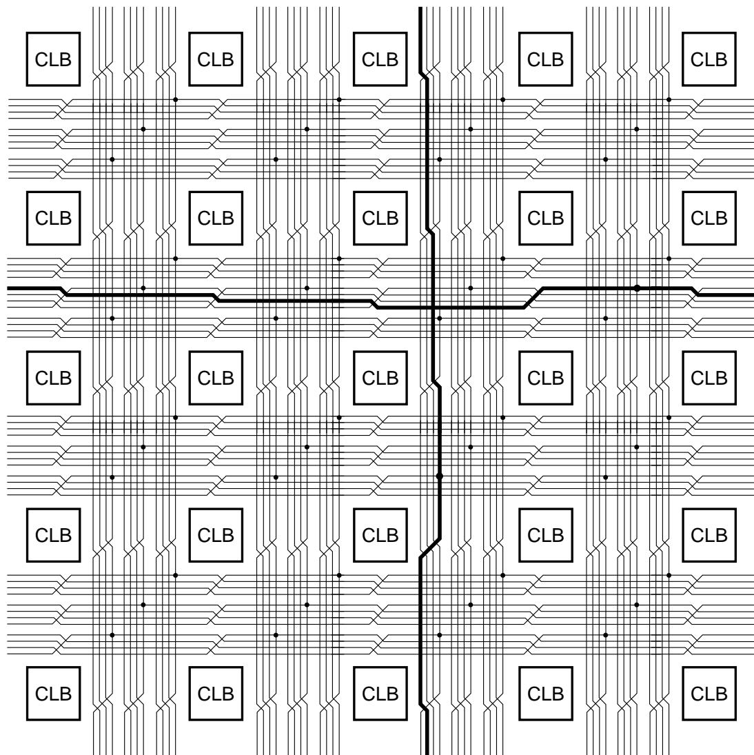
Figure 30: Quad Lines (XC4000EX only)
