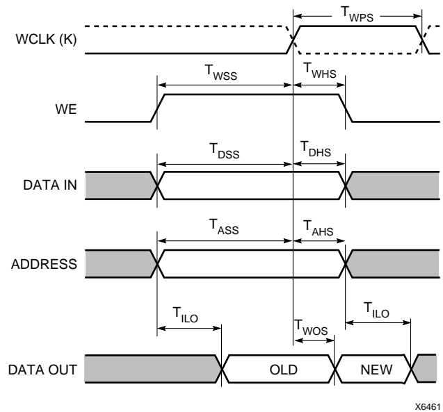
Figure 5: Edge-Triggered RAM Write Timing
