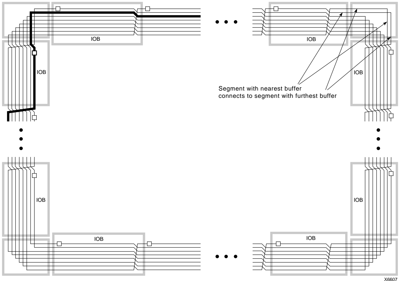
Figure 34: XC4000EX Octal I/O Routing
