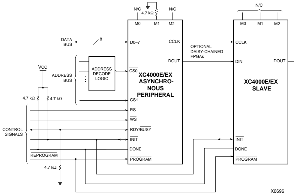
Figure 61: Asynchronous Peripheral Mode Circuit Diagram
