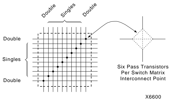
Figure 28: Programmable Switch Matrix (PSM)
