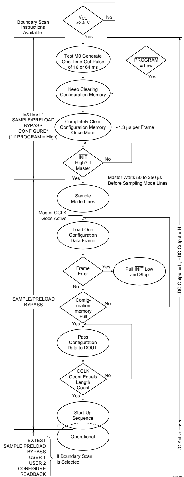
Figure 48: Power-up Configuration Sequence
