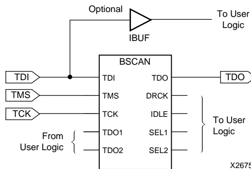
Figure 45: Boundary Scan Schematic Example
