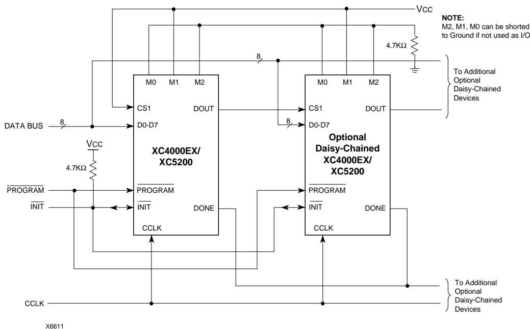
Figure 63: Express Mode Circuit Diagram
