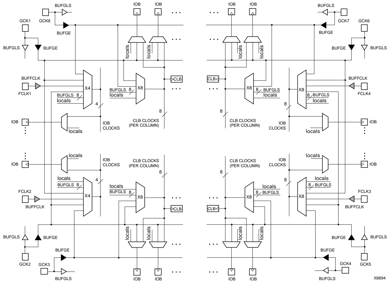
Figure 36: XC4000EX Global Net Distribution
