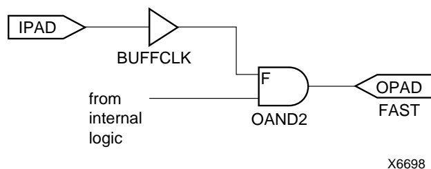
Figure 20: Fast Pin-to-Pin Path in XC4000E
