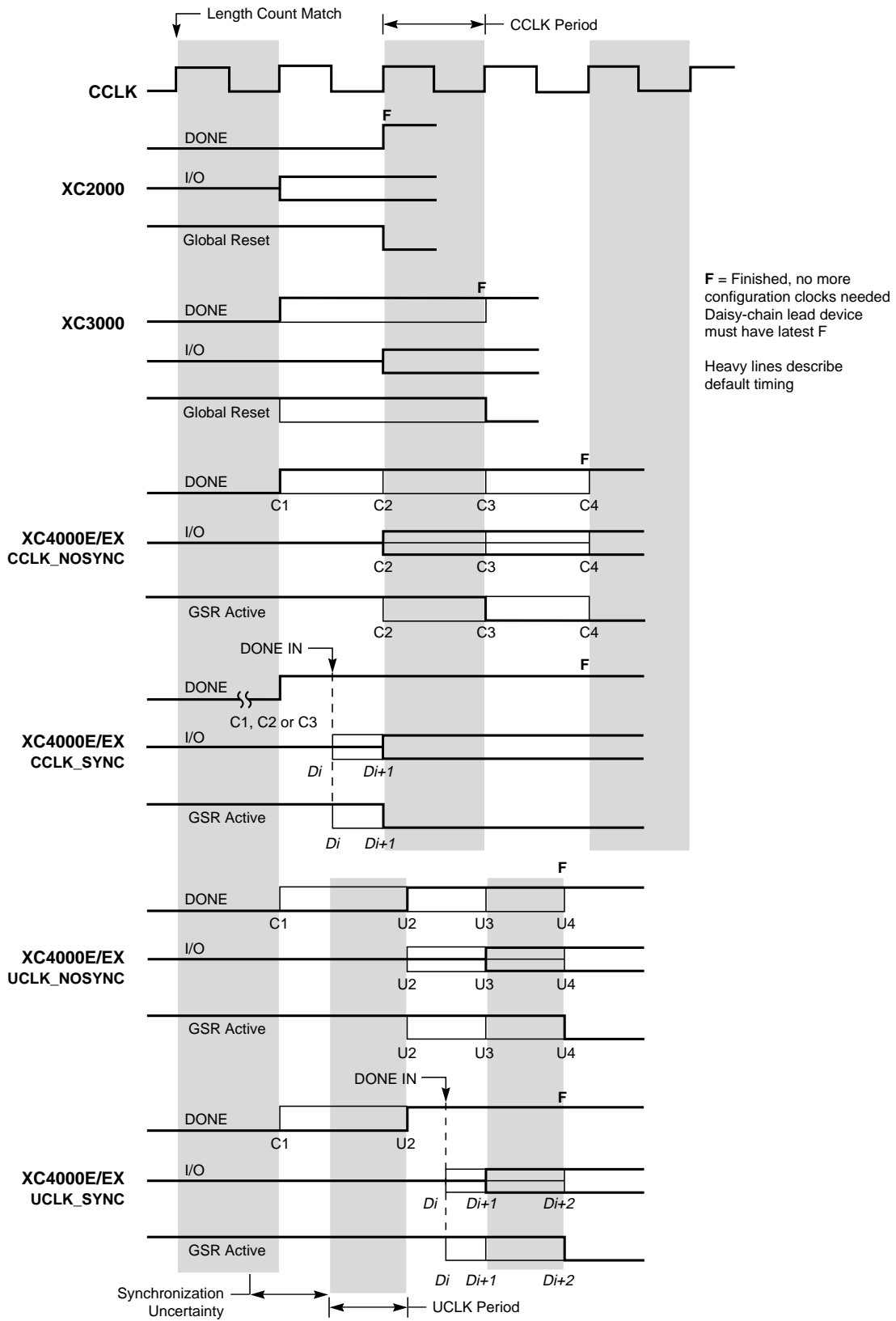
Figure 49: Start-up Timing
