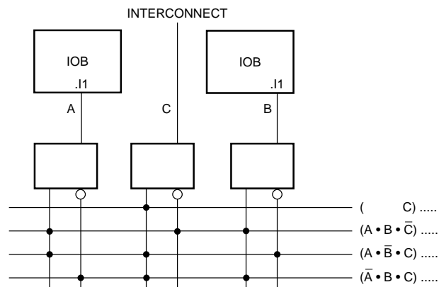
Figure 24: XC4000-Series Edge Decoding Example
