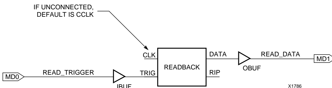
Figure 51: Readback Schematic Example
