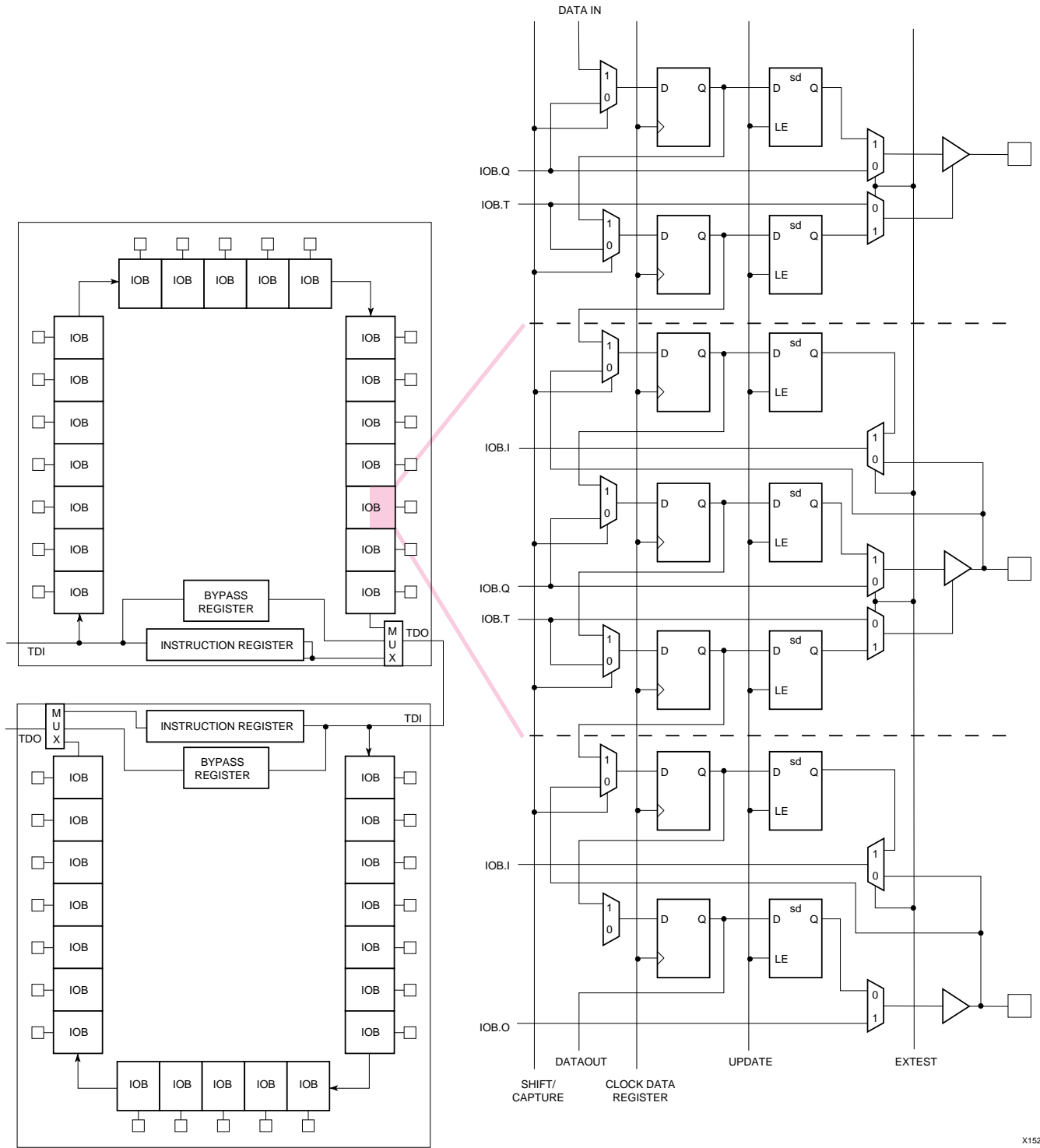
Figure 43: XC4000-Series Boundary Scan Logic
