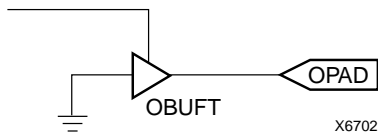
Figure 19: Open-Drain Output
