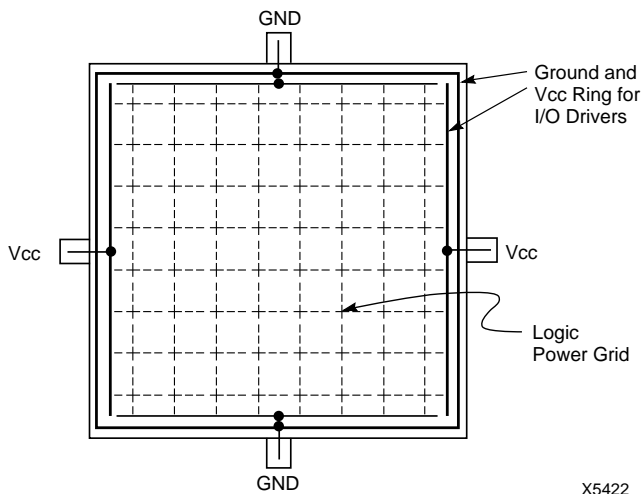
Figure 41: XC4000-Series Power Distribution
