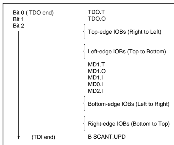
Figure 44: Boundary Scan Bit Sequence
