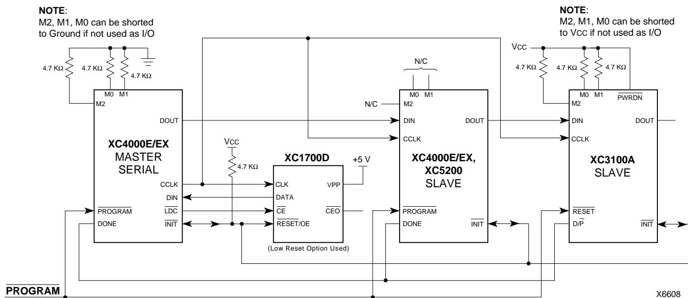
Figure 53: Master Serial Mode Circuit Diagram
