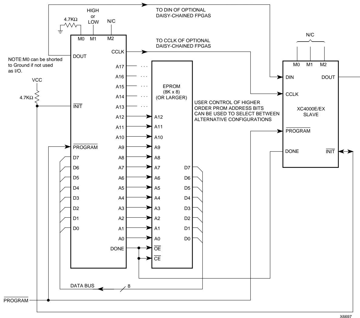
Figure 57: Master Parallel Mode Circuit Diagram
