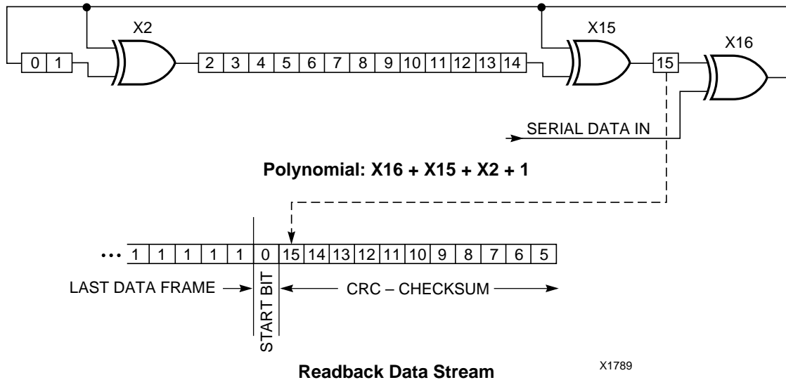
Figure 47: Circuit for Generating CRC-16
