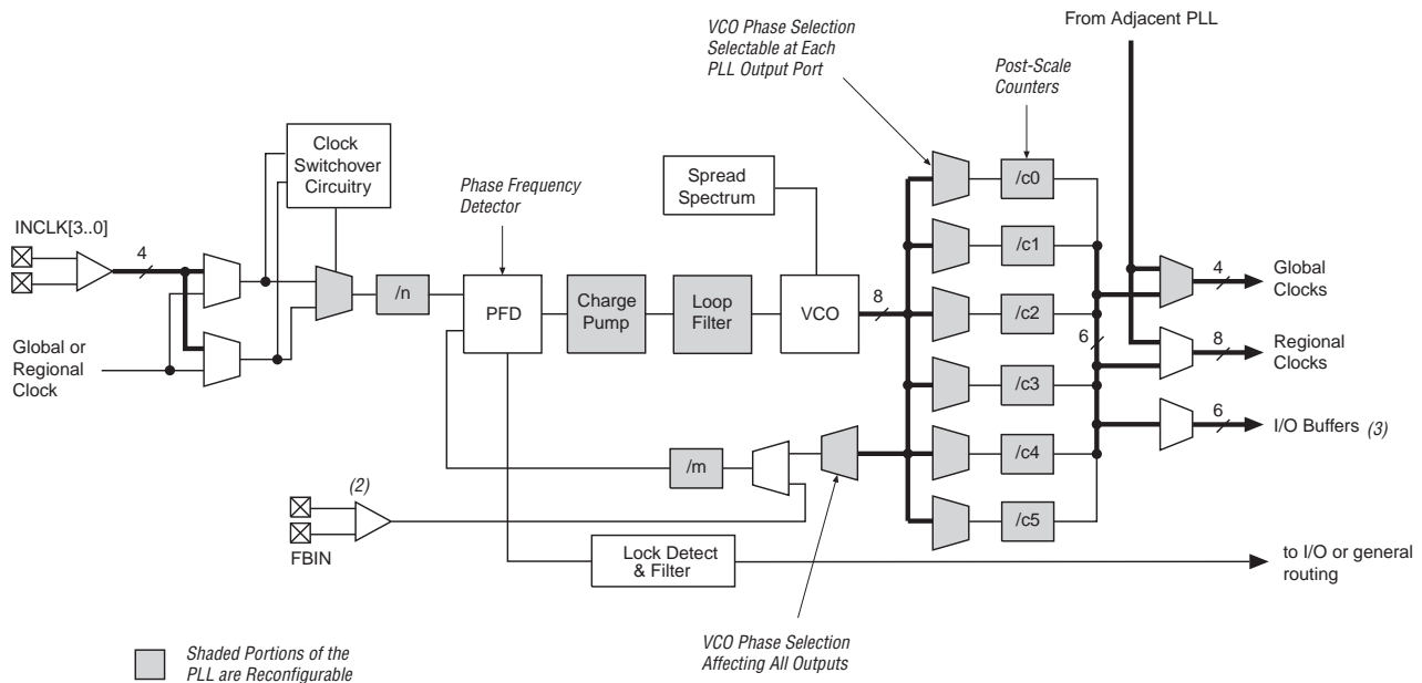
Figure 2–74. Stratix II GX Enhanced PLL Note (1)
