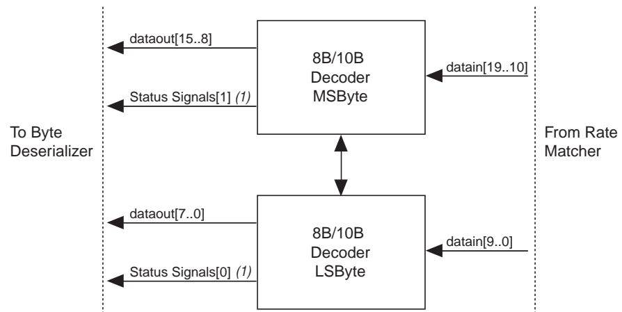
Figure 2–21. 8B/10B Decoder
