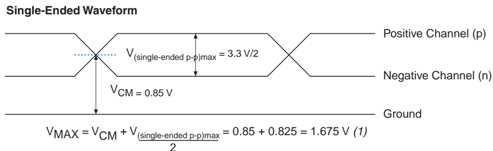
Figure 4–5. Maximum Receiver Input Pin Voltage
