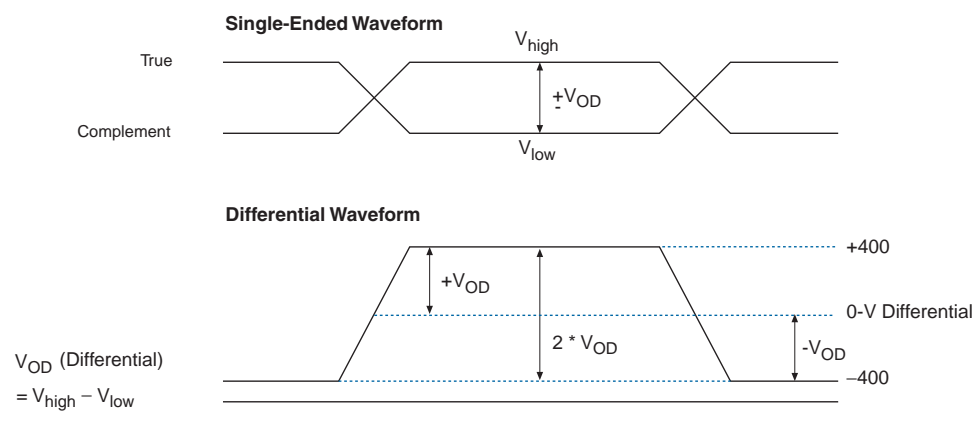
Figure 2–9. Differential Signaling
