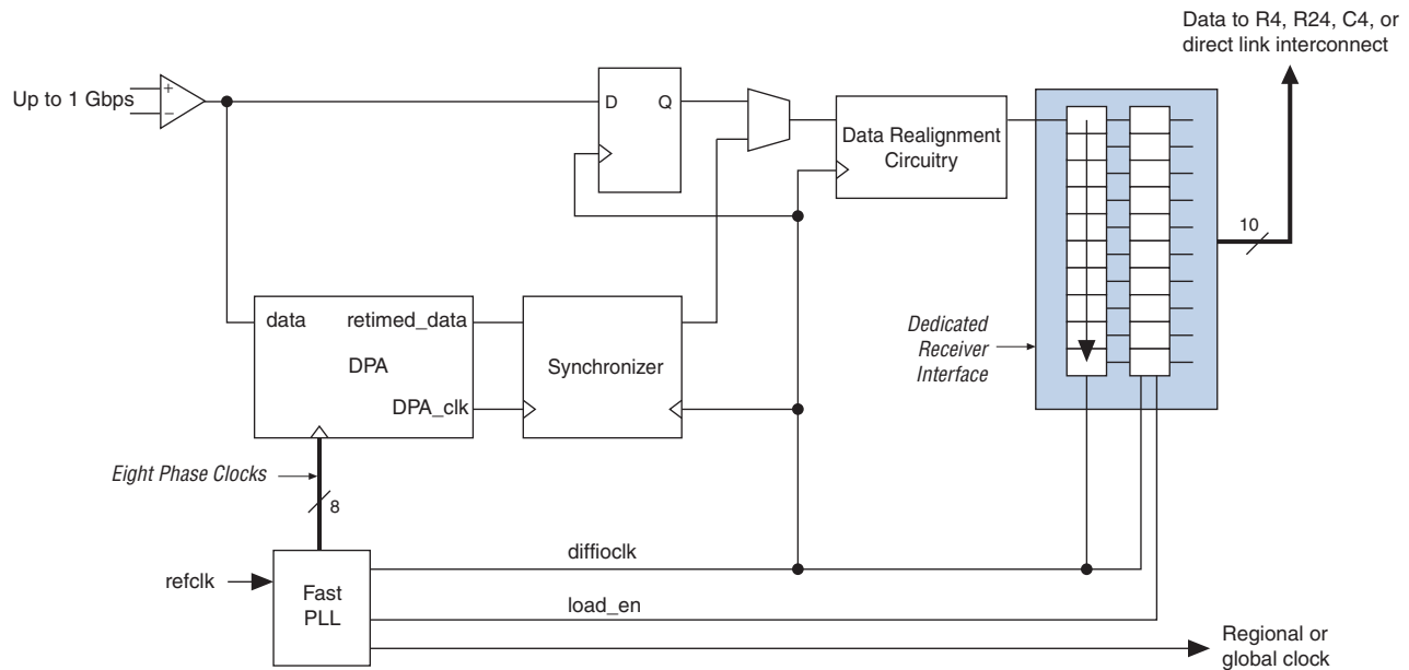
Figure 2–89. Stratix II GX Receiver Channel
