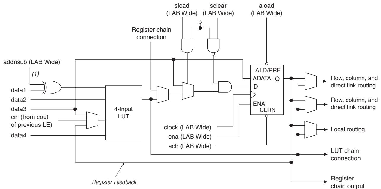
Figure 2-6. LE in Normal Mode
