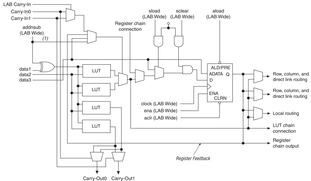
Figure 2-7. LE in Dynamic Arithmetic Mode
