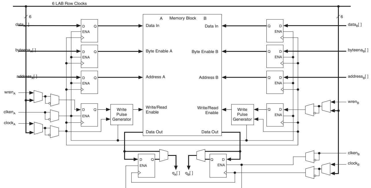
Figure 2-18. Input/Output Clock Mode in True Dual-Port Mode Notes (1), (2)
