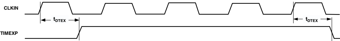
Figure 11. Timer
