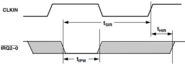
Figure 10. Interrupts
