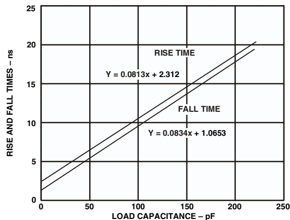
Figure 32. Typical Output Rise Time (20%–80%, V_{DDEXT} = \text{Min} ) vs. Load Capacitance
