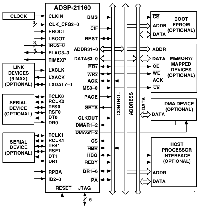
Figure 1. Single-Processor System
