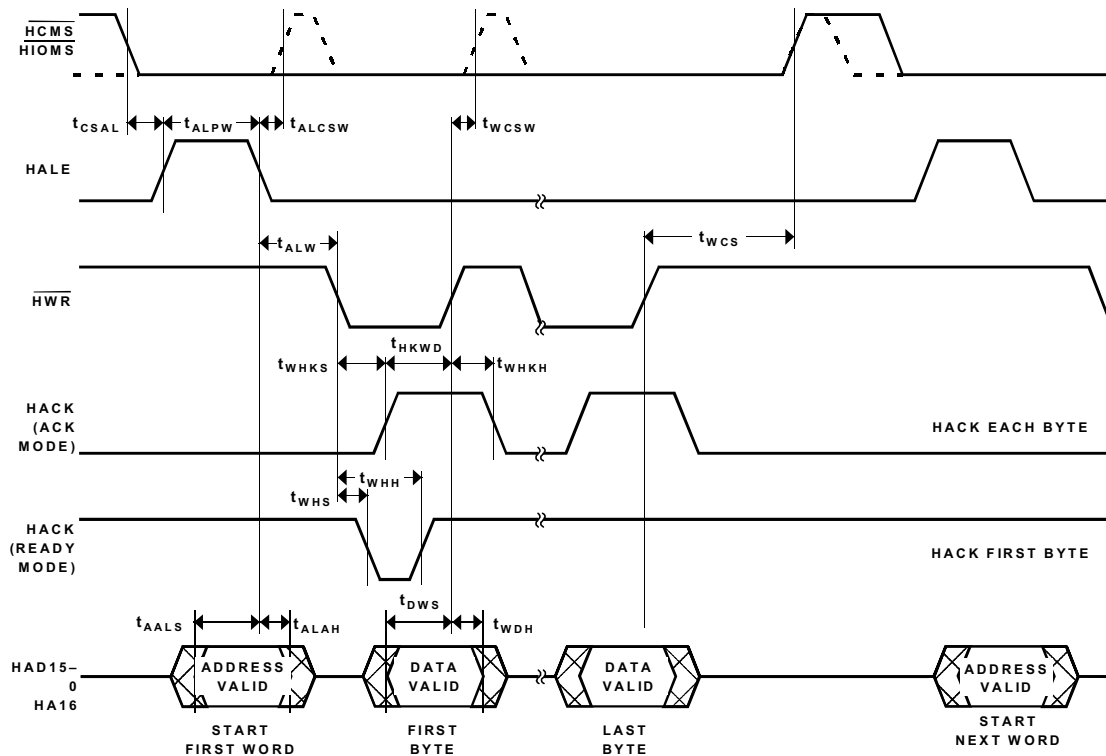
Figure 17. Host Port ALE Mode Write Cycle Timing
