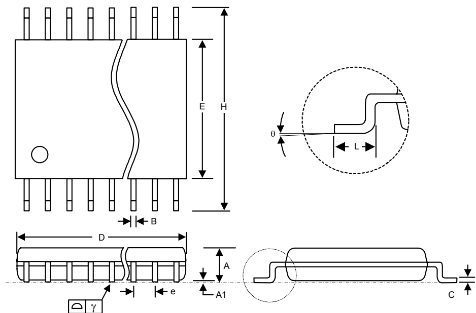
Figure 19. 24-Pin Thin Shrink Small Outline Package (TSSOP)
