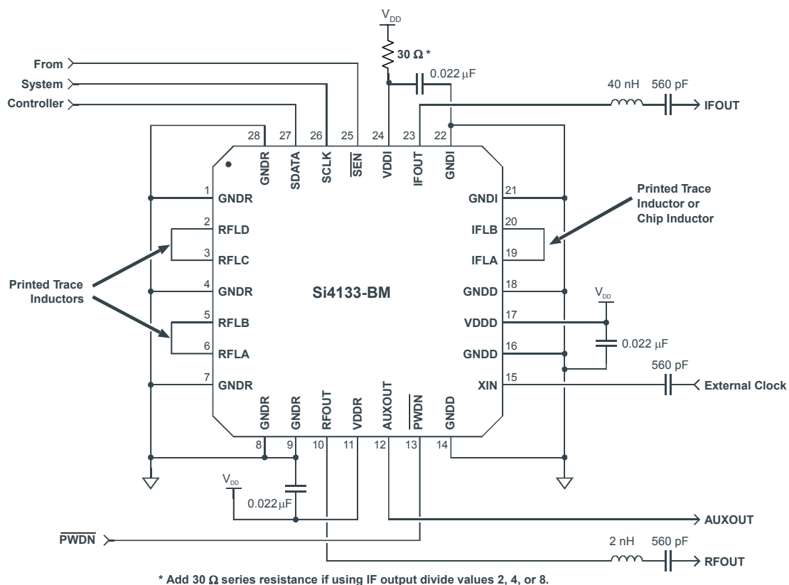
Figure 14. Si4133-BM
