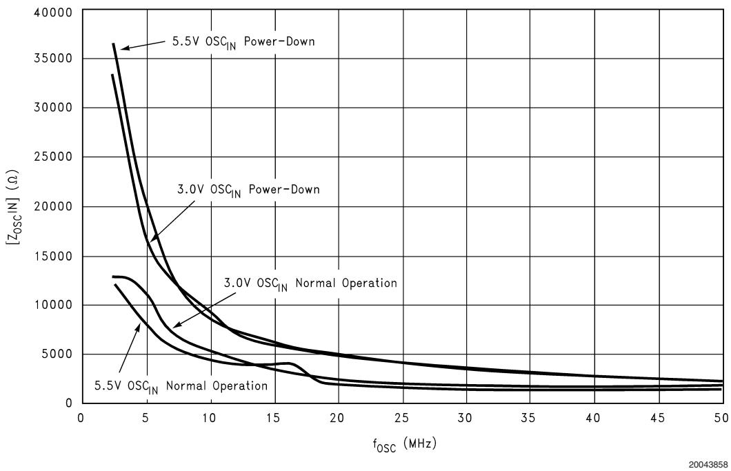
LMX231xU OSC in Input Impedance vs Frequency
