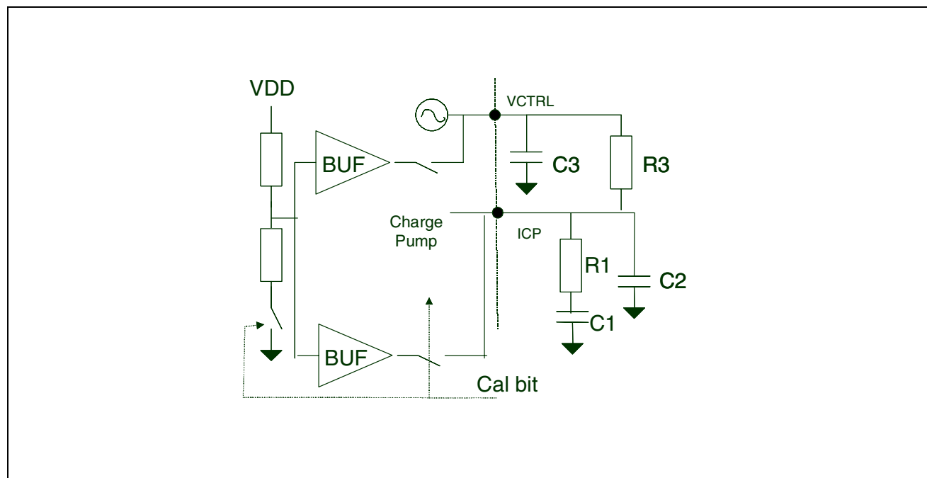
Figure 15. Loop Filter Connection
