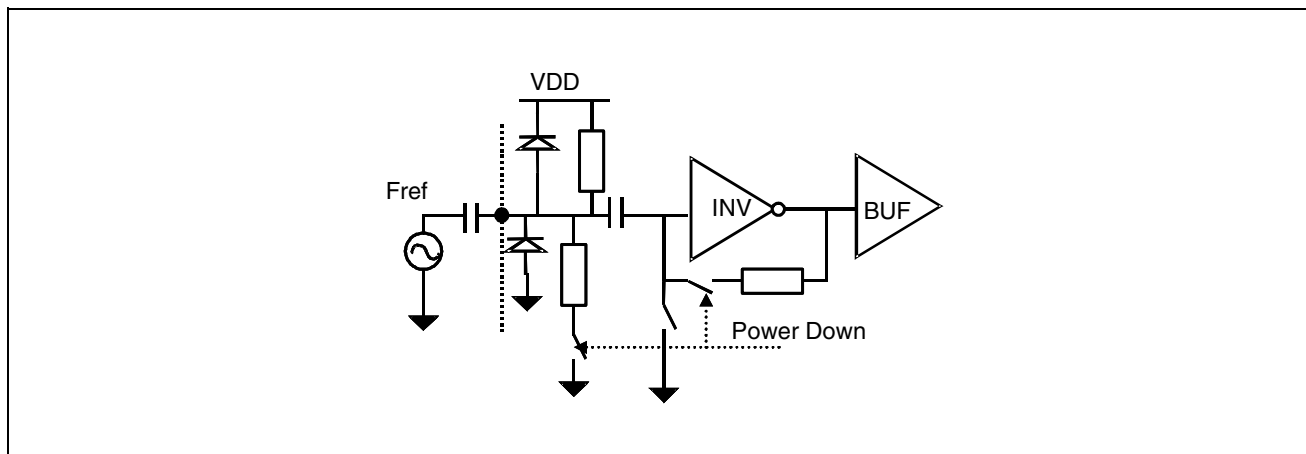
Figure 12. Reference Frequency Input Buffer
