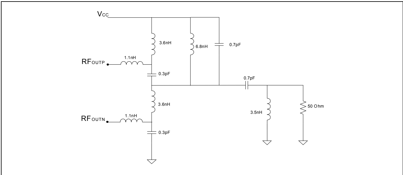
Figure 24. LC lumped balun and matching network
