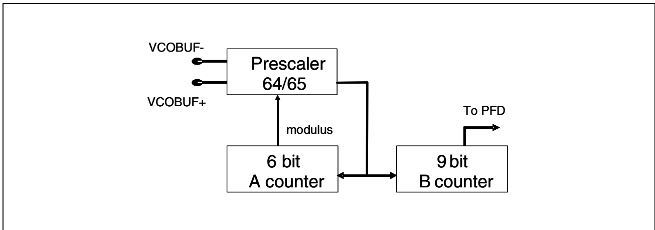
Figure 13. VCO Divider Diagram
