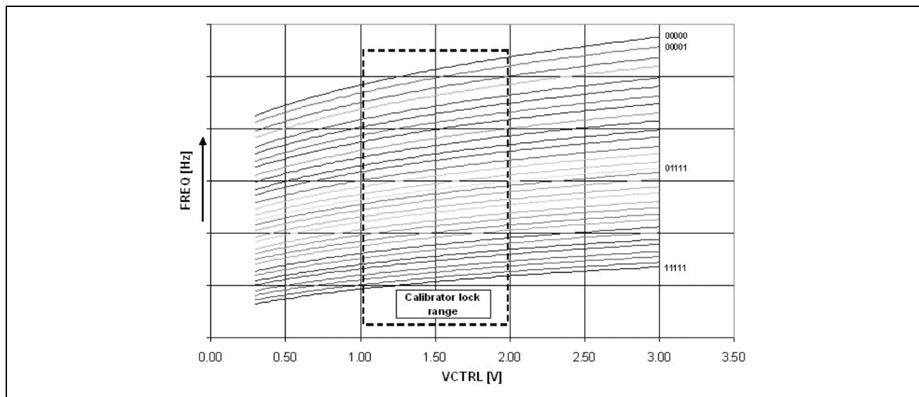
Figure 16. VCO Sub-Bands Frequency Characteristics
