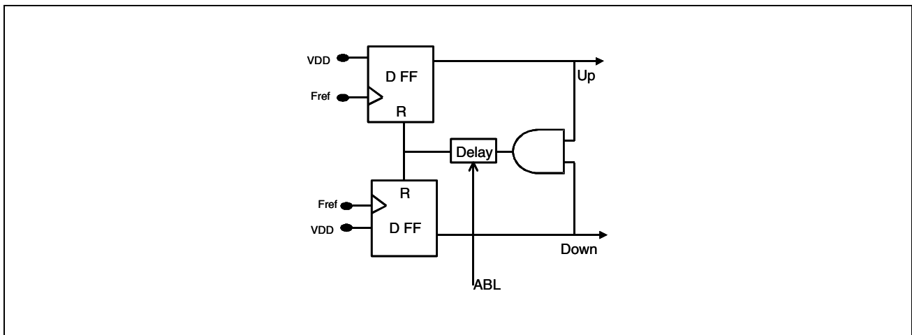
Figure 14. PFD Diagram
