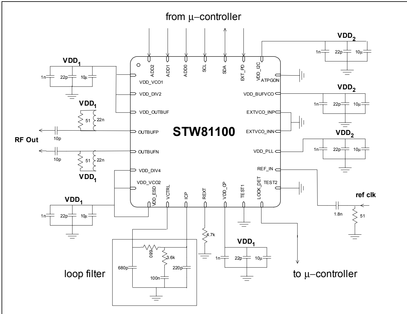
Figure 31. Application diagram
