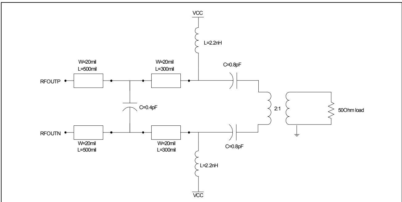
Figure 25. Microstrip line and lumped matching network
