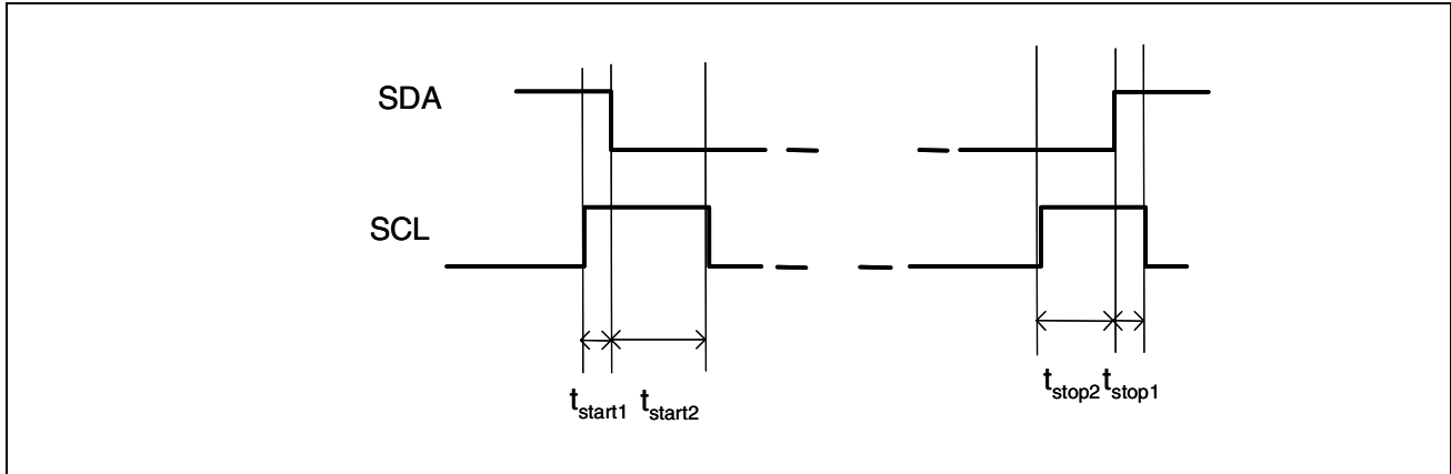
Figure 21. Start and Stop
