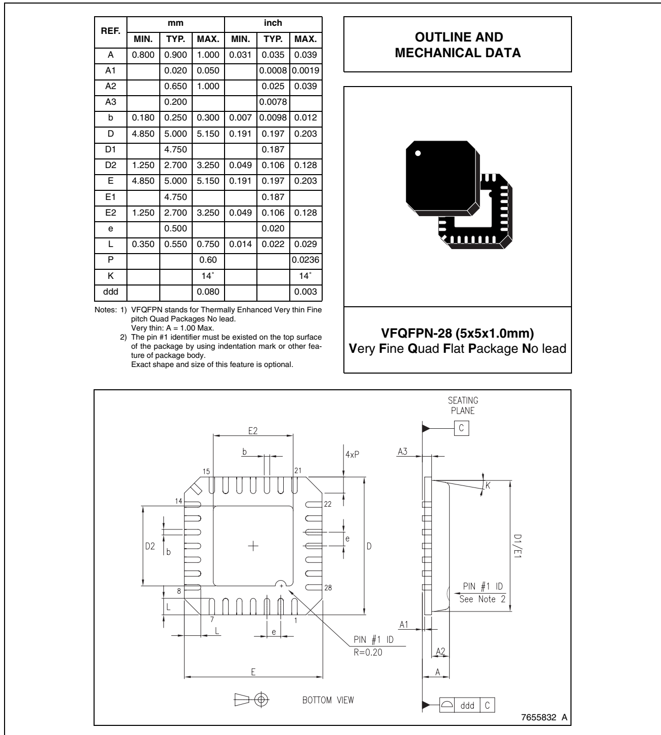
Figure 32. VFQFPN28 Mechanical Data & Package Dimensions
