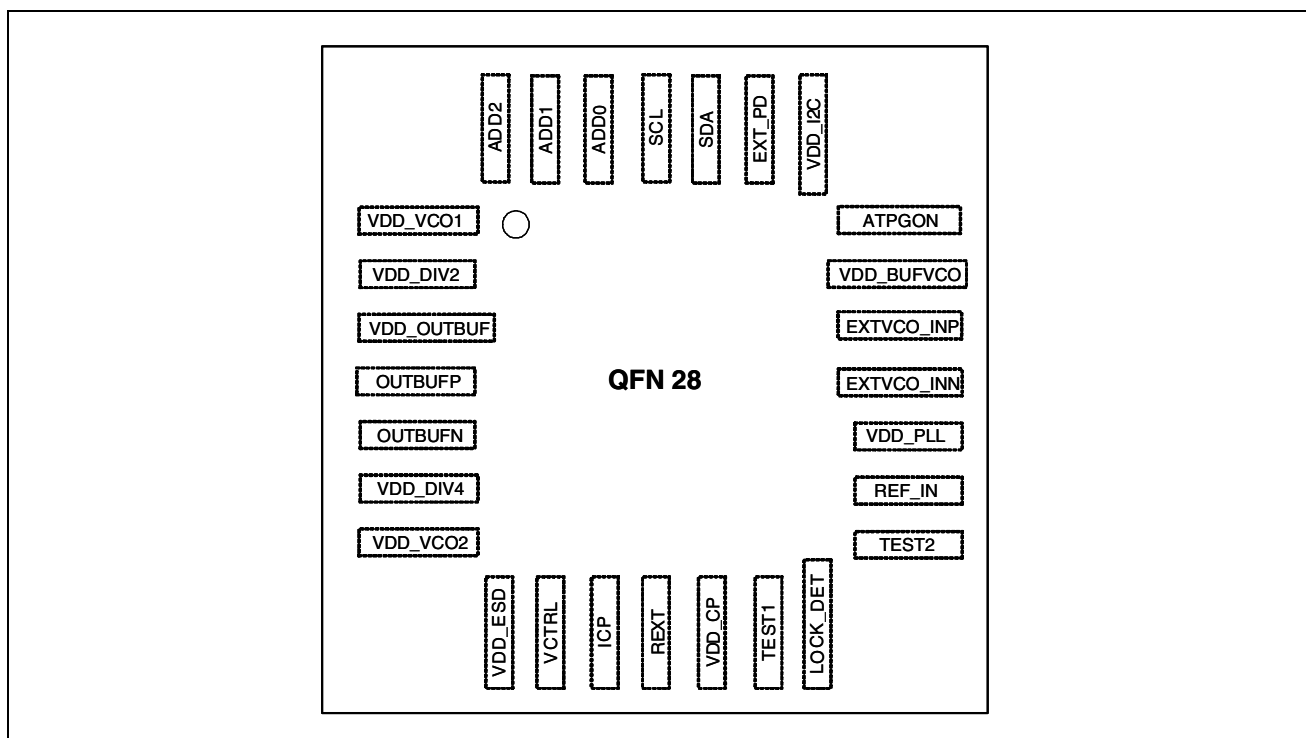
Figure 3. Pin Connections
