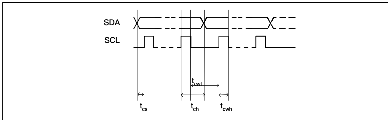
Figure 20. Data and clock
