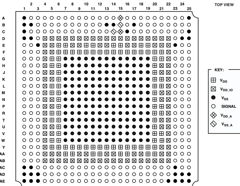
Figure 42. 625-Ball PBGA Pin Configurations (Top View, Summary)
