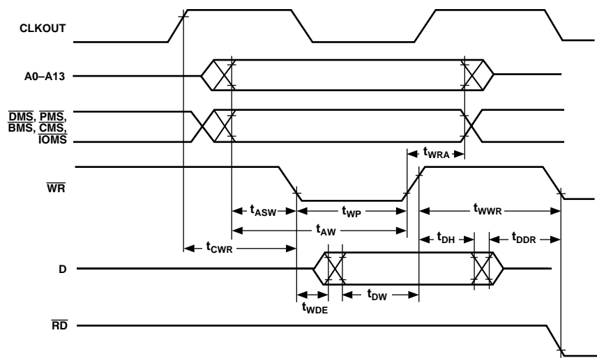
Figure 12. Memory Write
