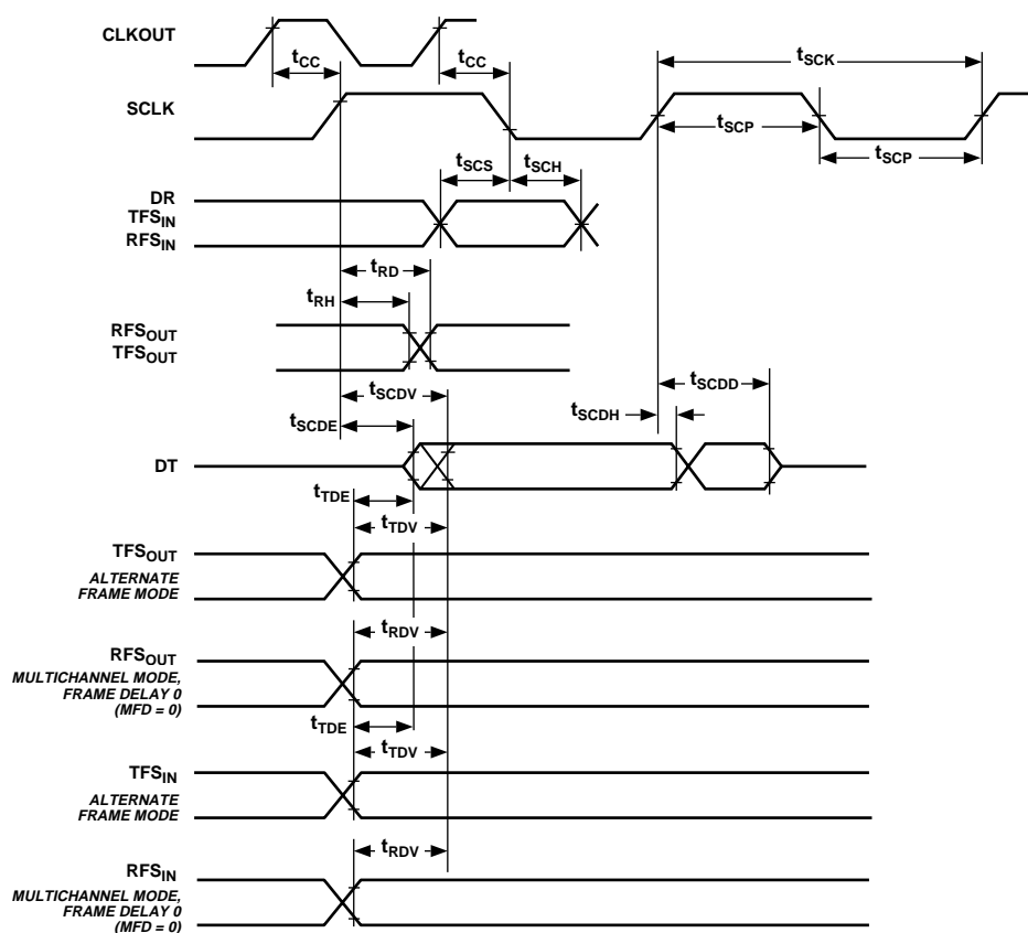
Figure 13. Serial Ports
