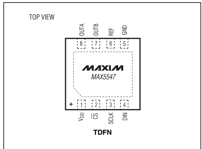
Pin Configuration
