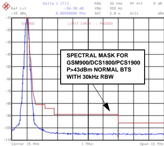
FIGURE 1. EDGE AT 11MHz, 78MSPS CLOCK (94+dBc @ \Delta f = +6 MHz)
