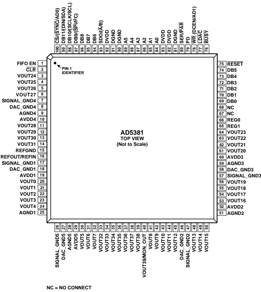
Figure 8. 100-Lead LQFP Pin Configuration
