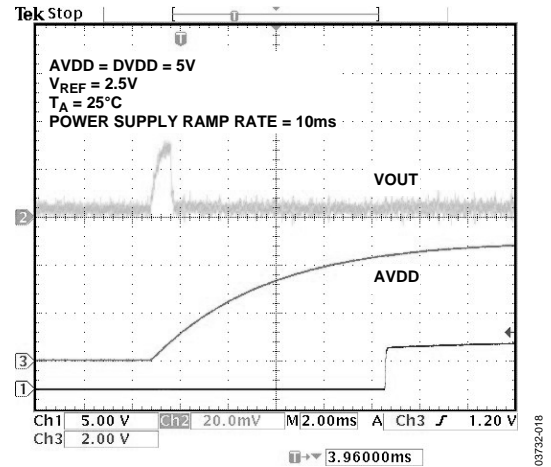
Figure 18. Power-Up Transient
