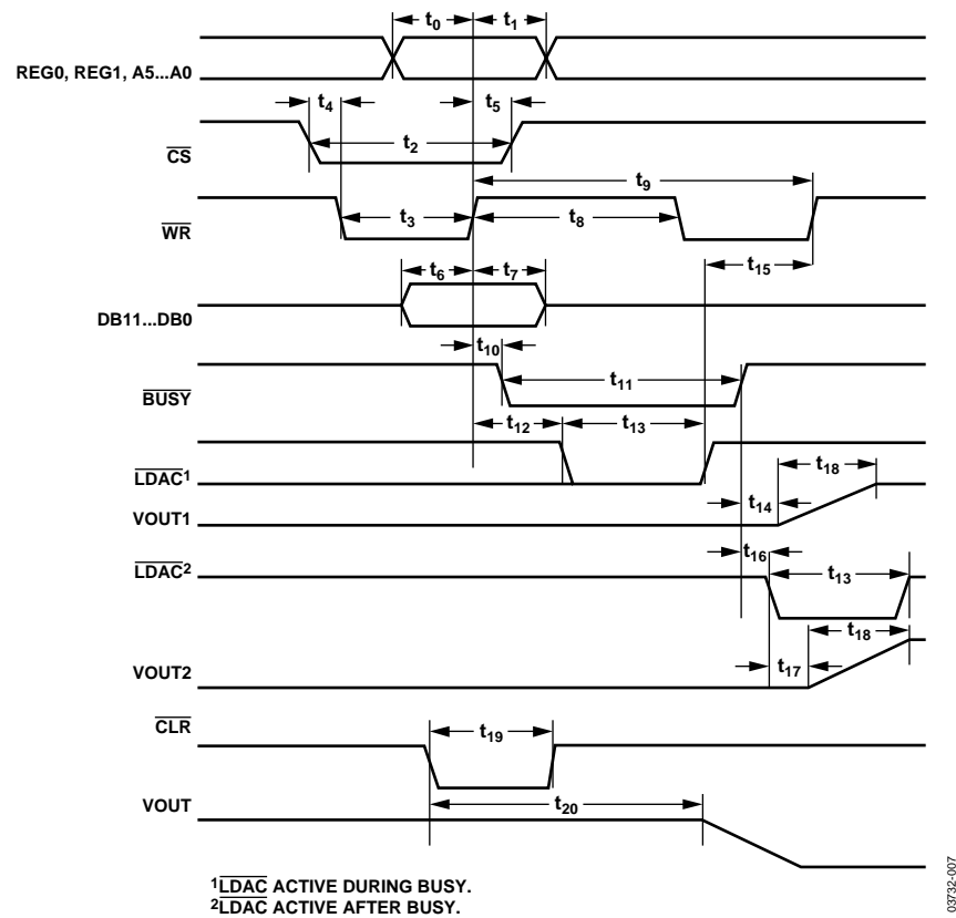
Figure 7. Parallel Interface Timing Diagram
